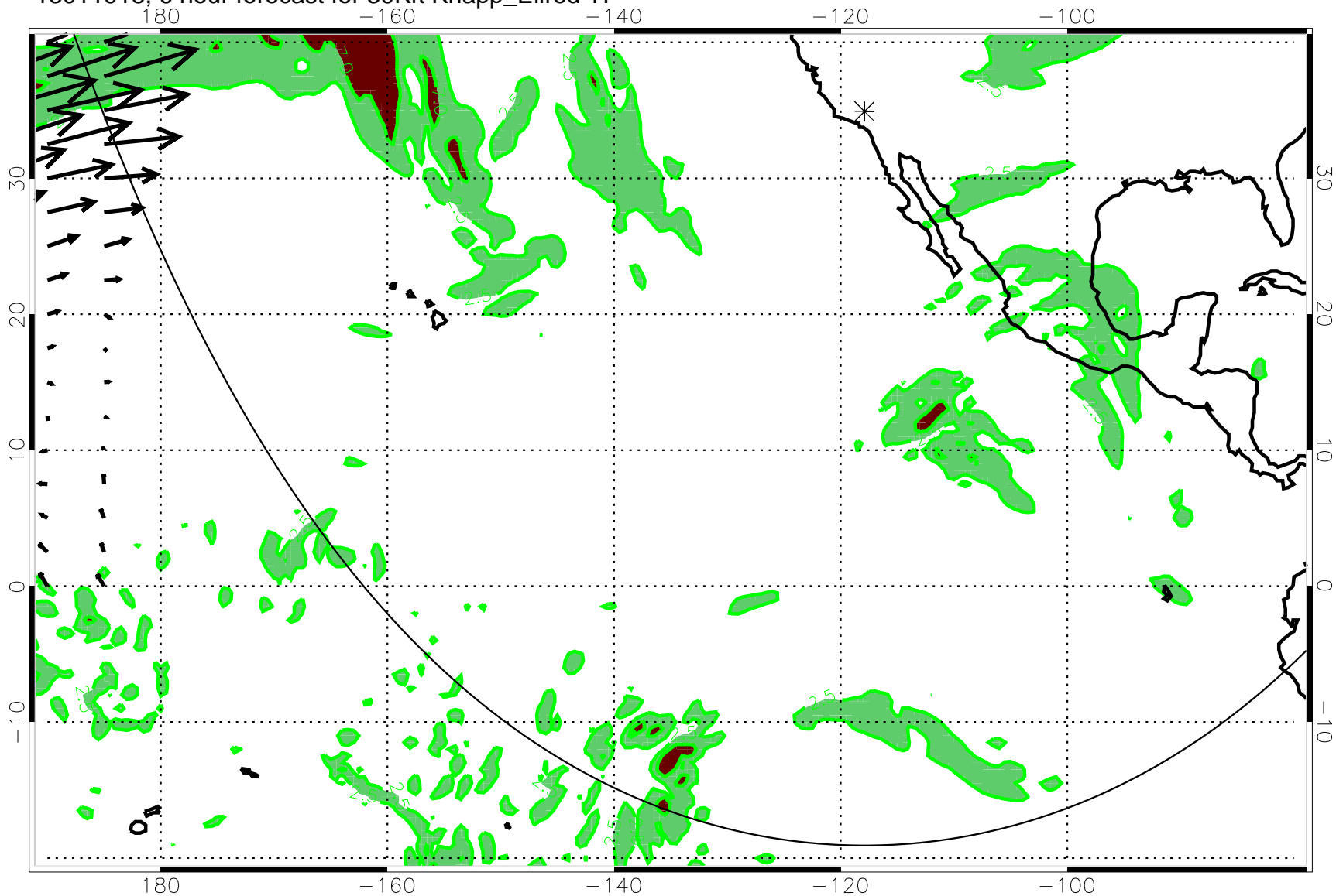
13011918, 6 hour forecast for 39Kft Knapp_Ellrod TI
