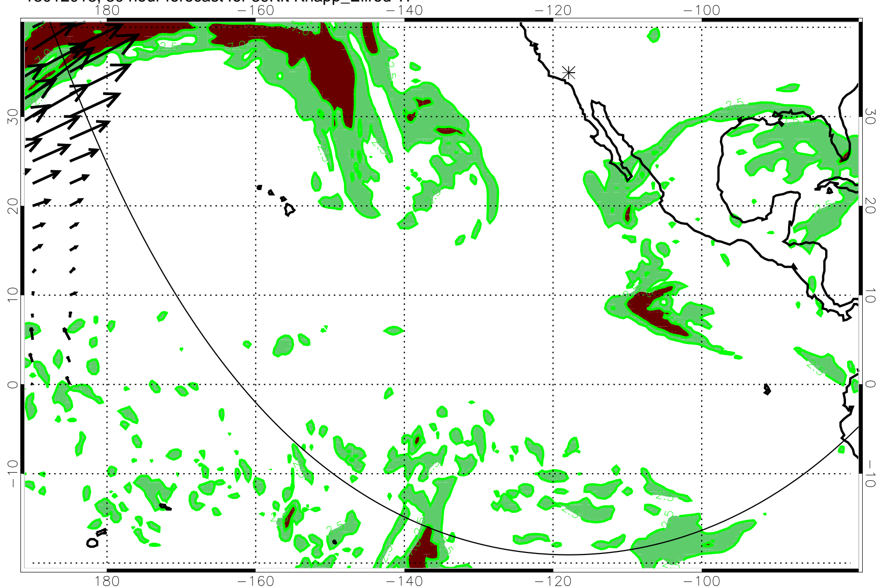
13012018, 30 hour forecast for 39Kft Knapp_Ellrod TI
