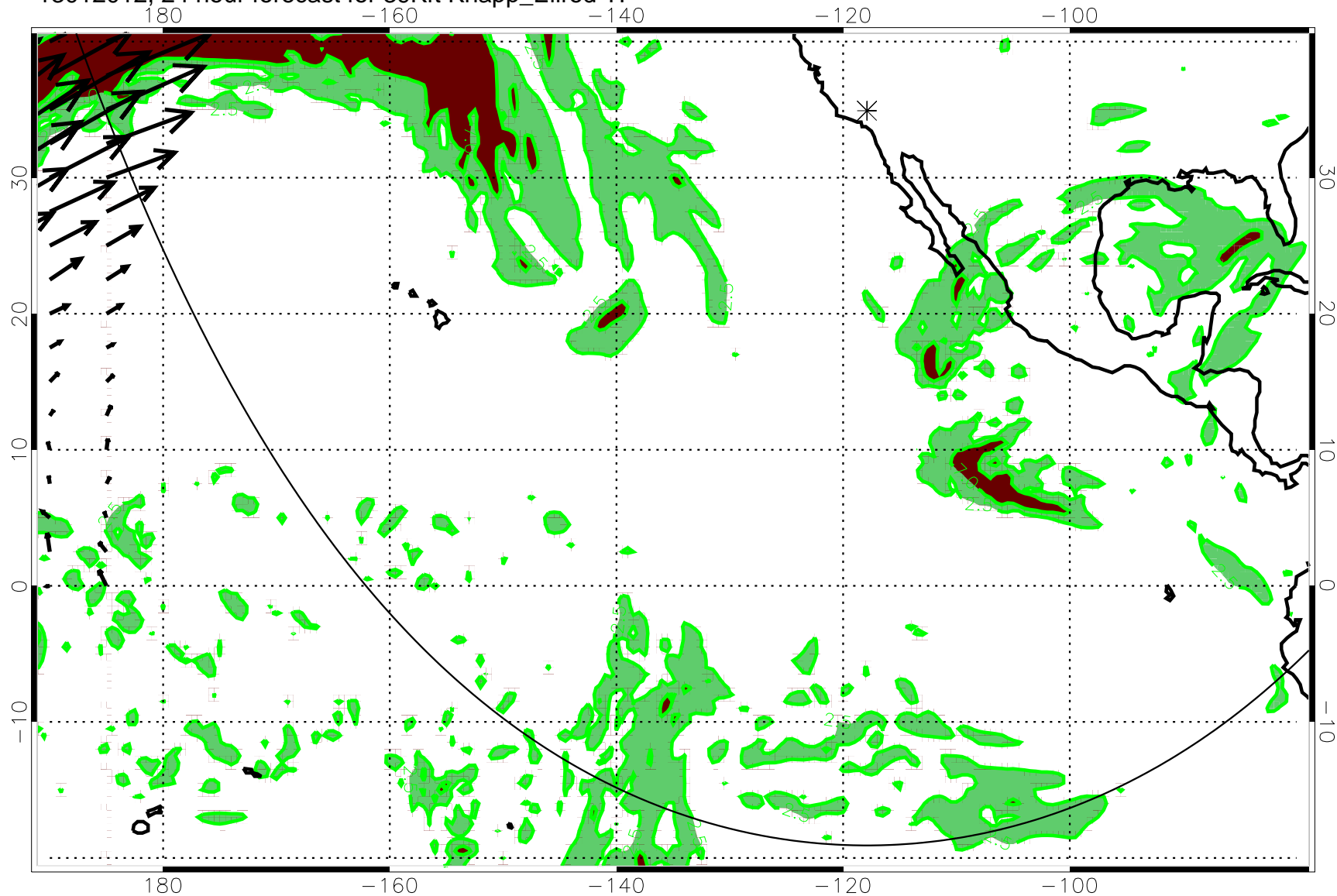
13012012, 24 hour forecast for 39Kft Knapp_Ellrod TI
