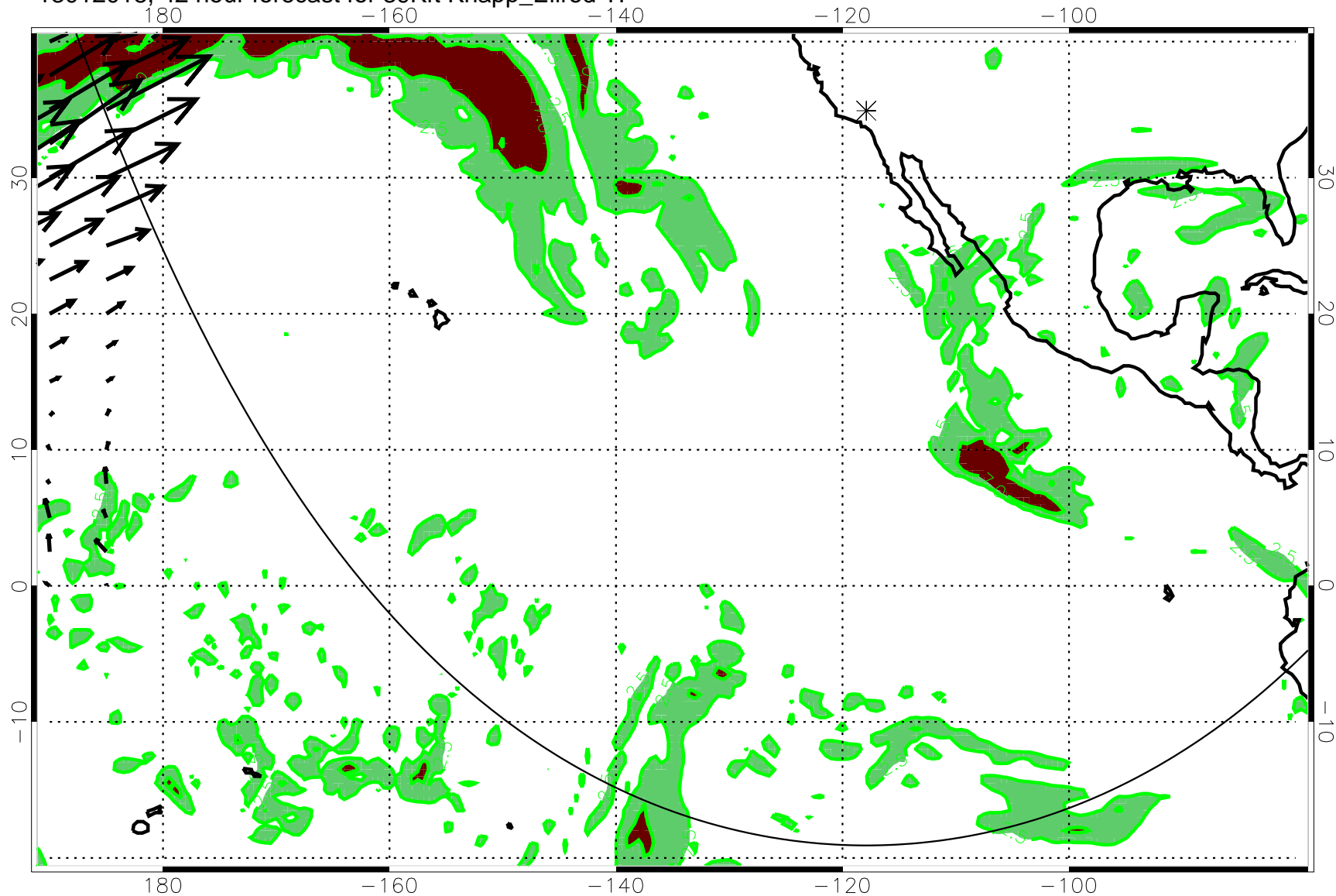
13012018, 42 hour forecast for 39Kft Knapp_Ellrod TI
