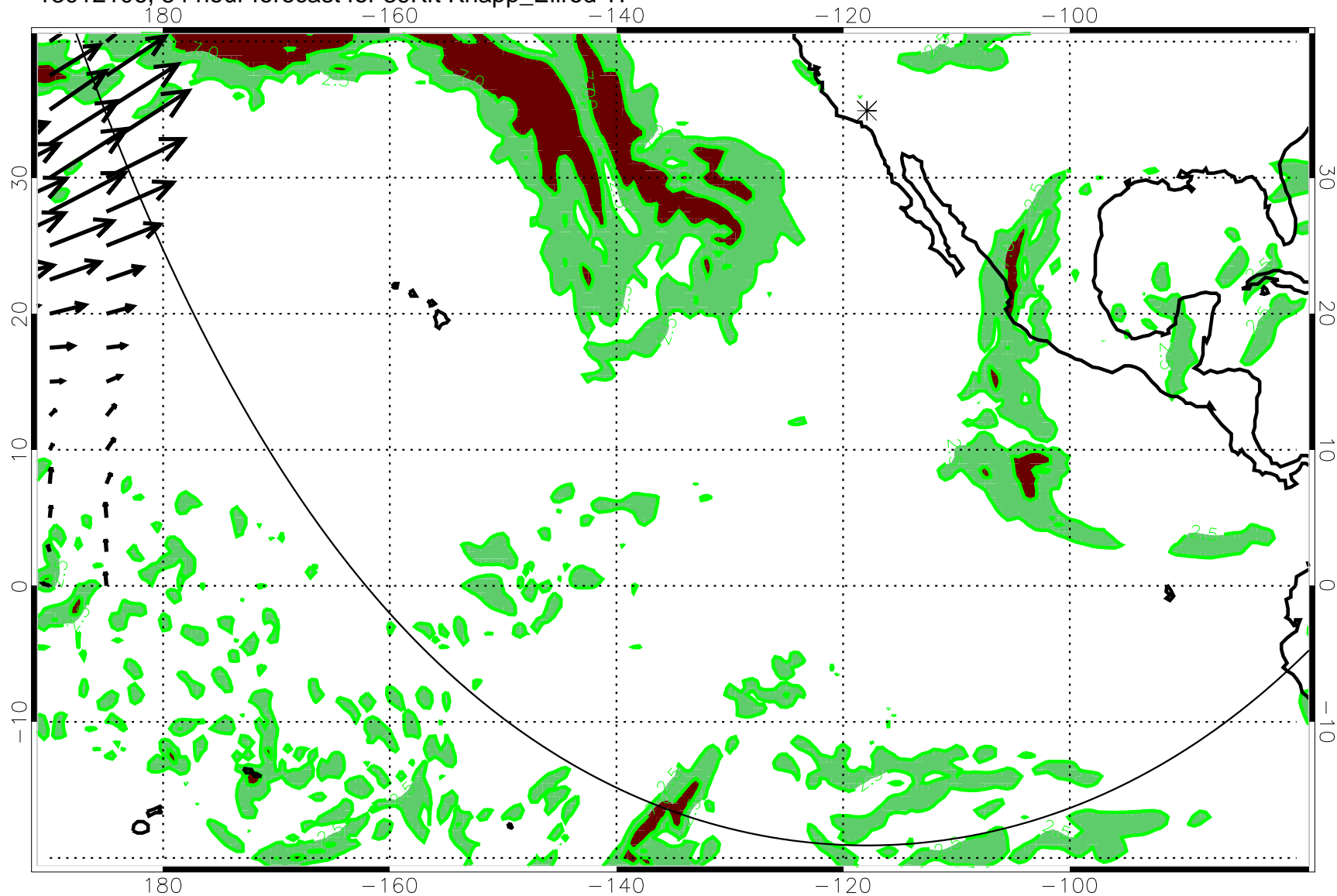
13012106, 54 hour forecast for 39Kft Knapp_Ellrod TI
