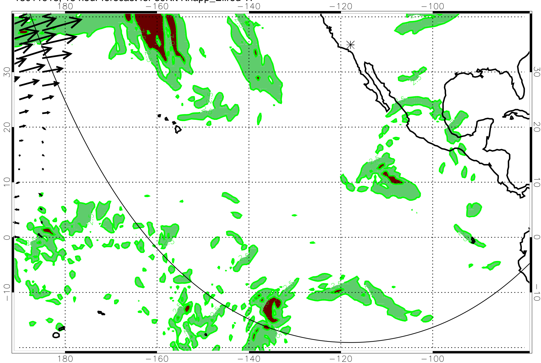
13011918, 18 hour forecast for 39Kft Knapp_Ellrod TI
