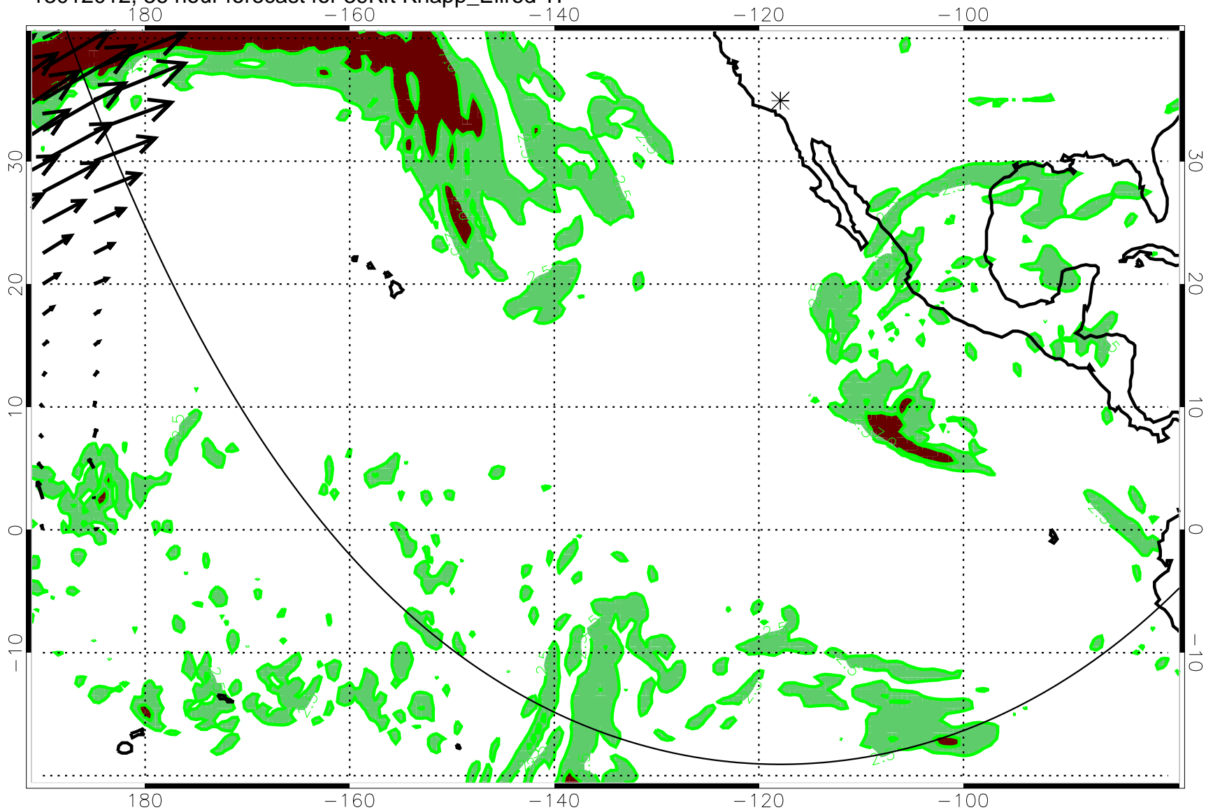
13012012, 36 hour forecast for 39Kft Knapp_Ellrod TI
