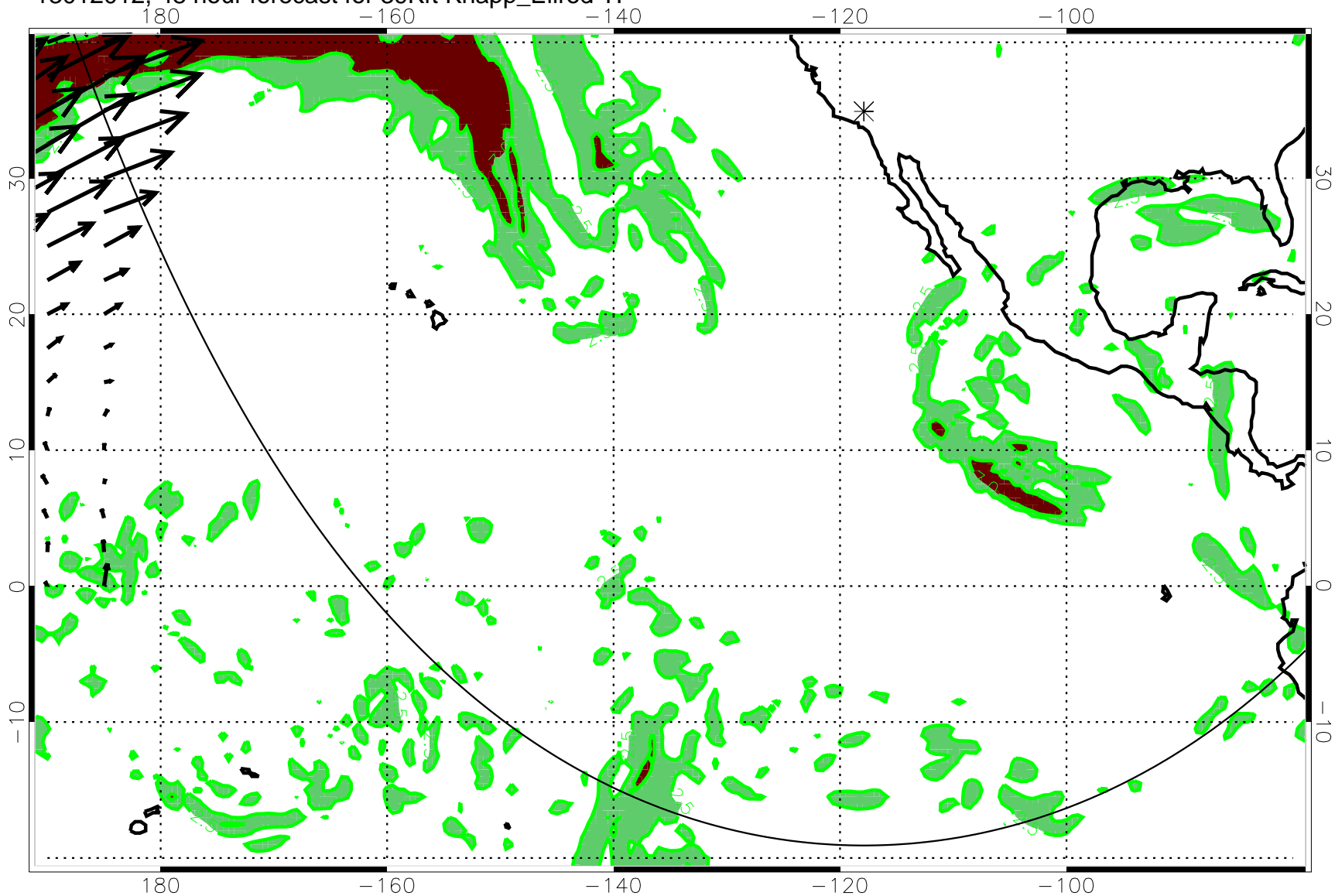
13012012, 48 hour forecast for 39Kft Knapp_Ellrod TI
