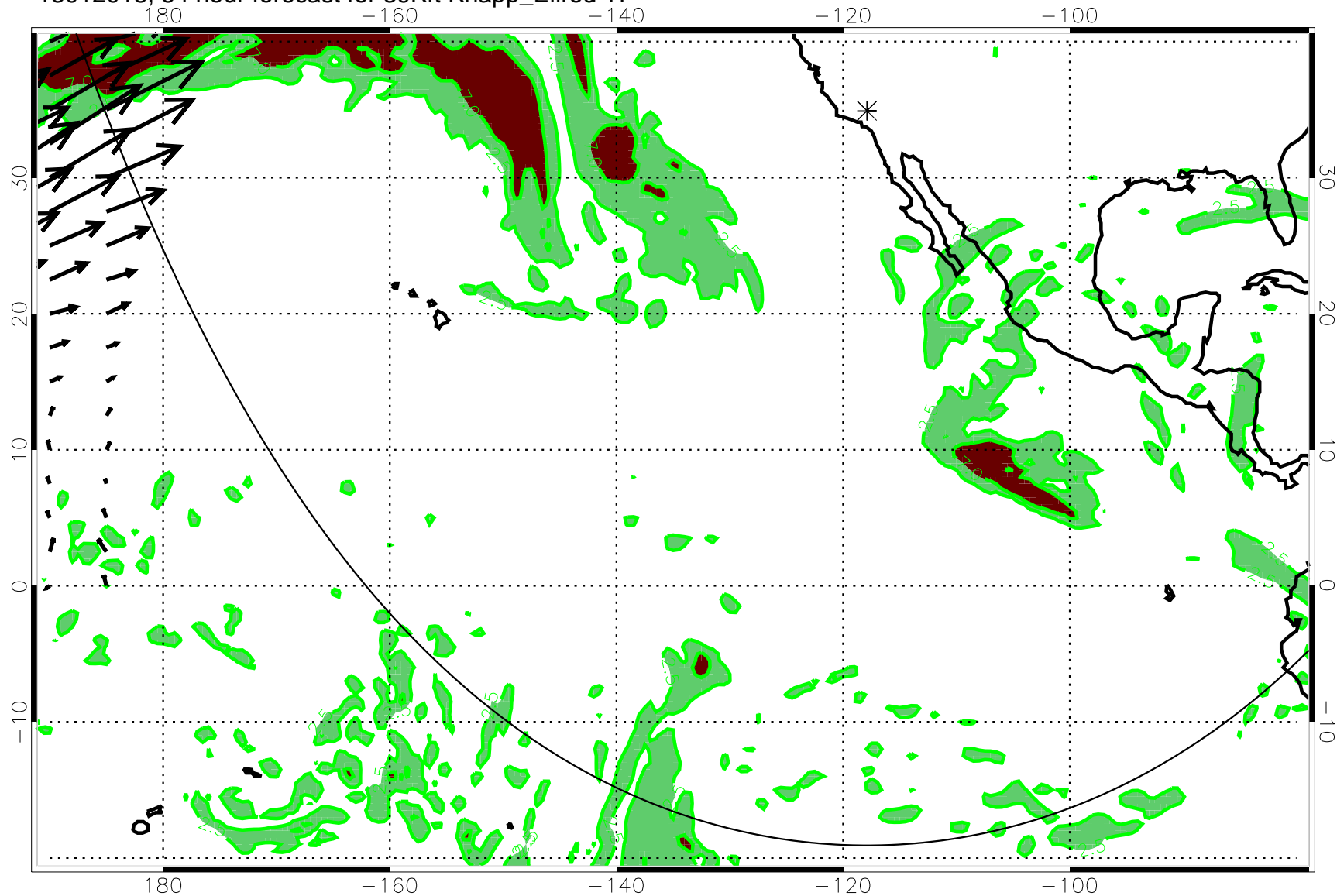
13012018, 54 hour forecast for 39Kft Knapp_Ellrod TI
