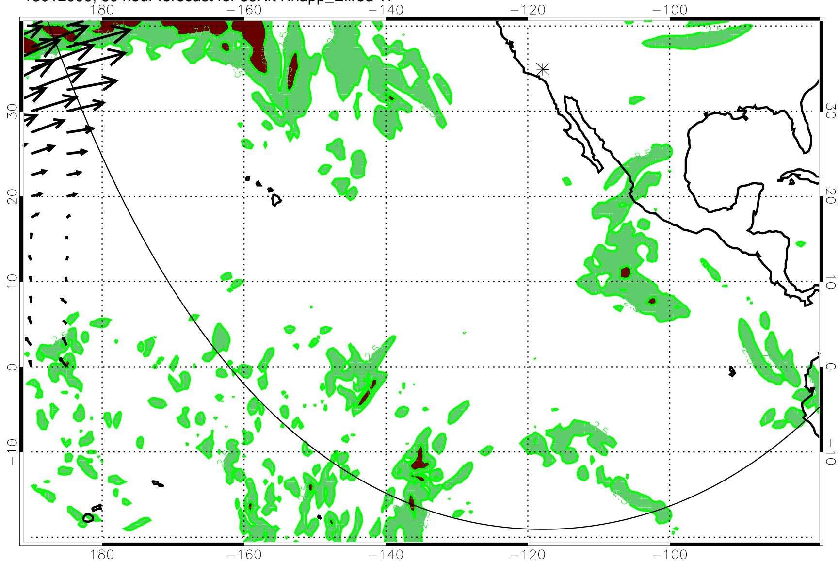
13012000, 60 hour forecast for 39Kft Knapp_Ellrod TI
