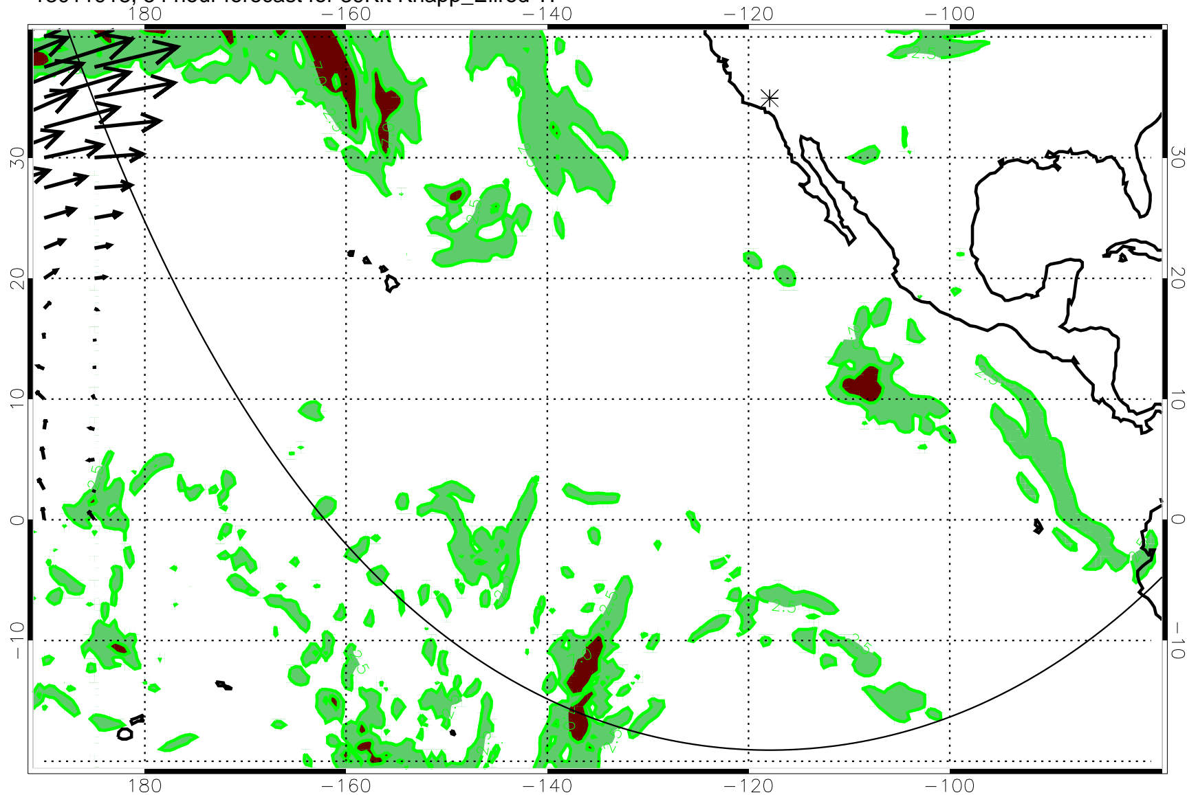
13011918, 54 hour forecast for 39Kft Knapp_Ellrod TI
