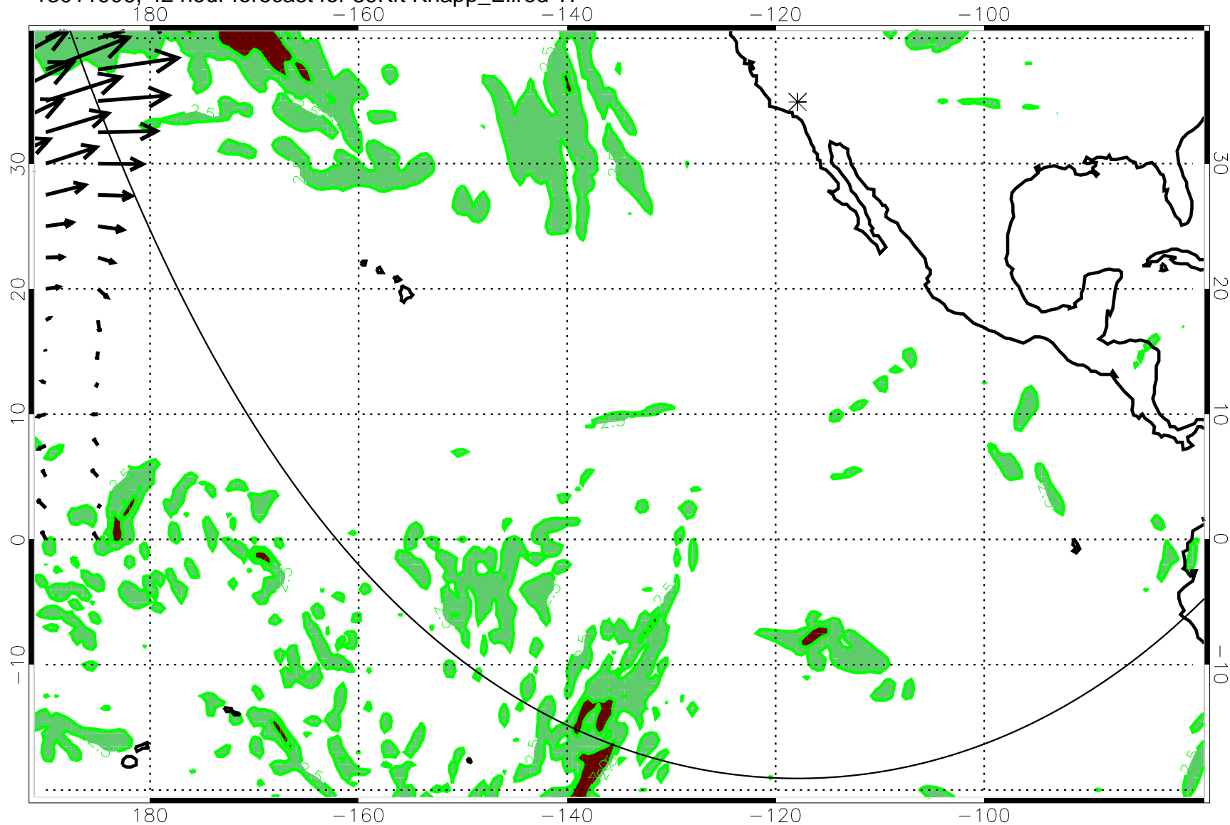
13011906, 42 hour forecast for 39Kft Knapp_Ellrod TI
