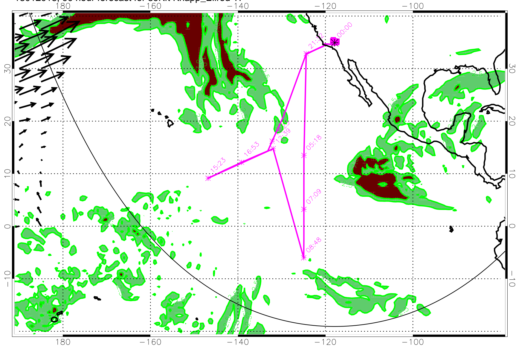
13012018, 90 hour forecast for 39Kft Knapp_Ellrod TI
