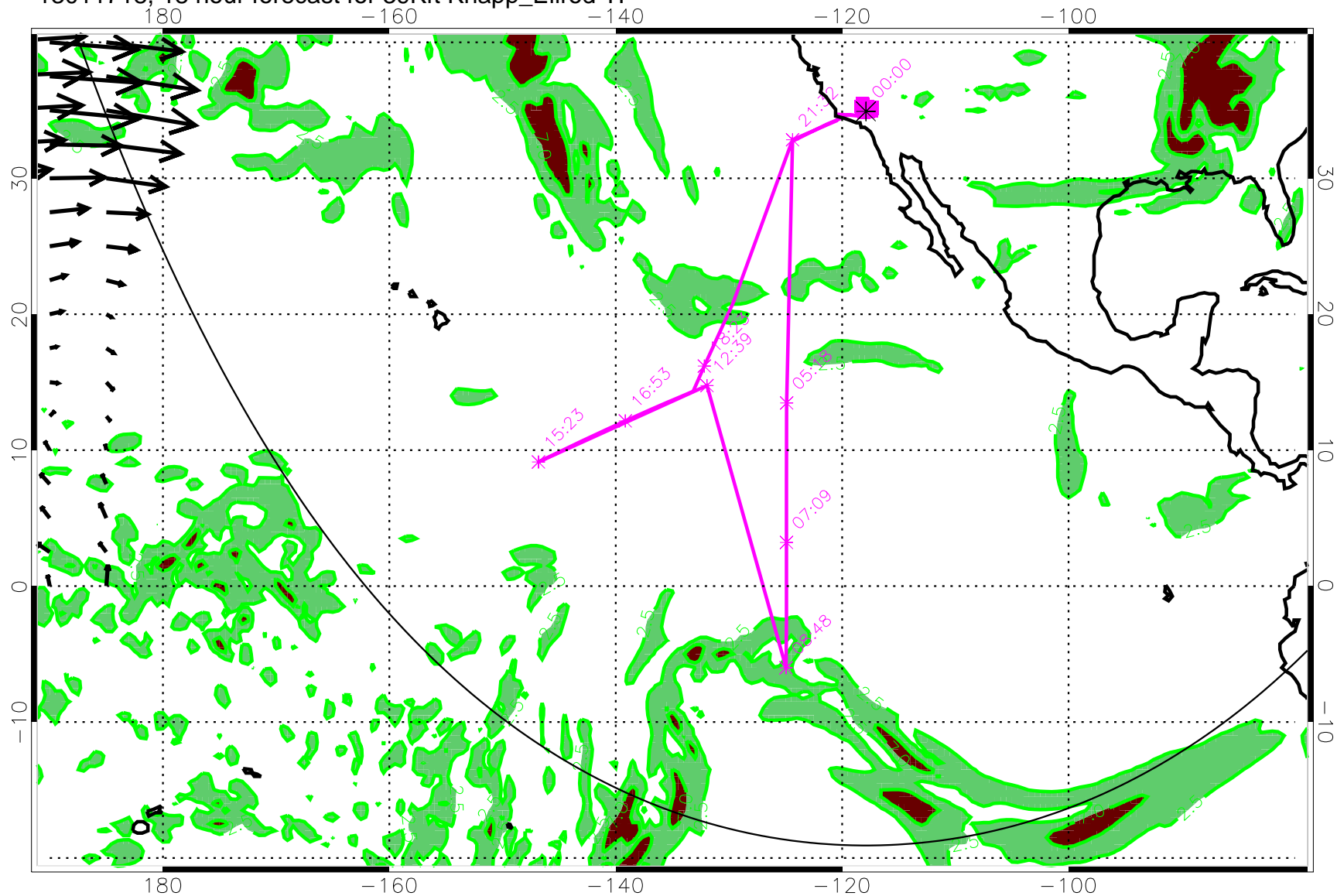
13011718, 18 hour forecast for 39Kft Knapp_Ellrod TI
