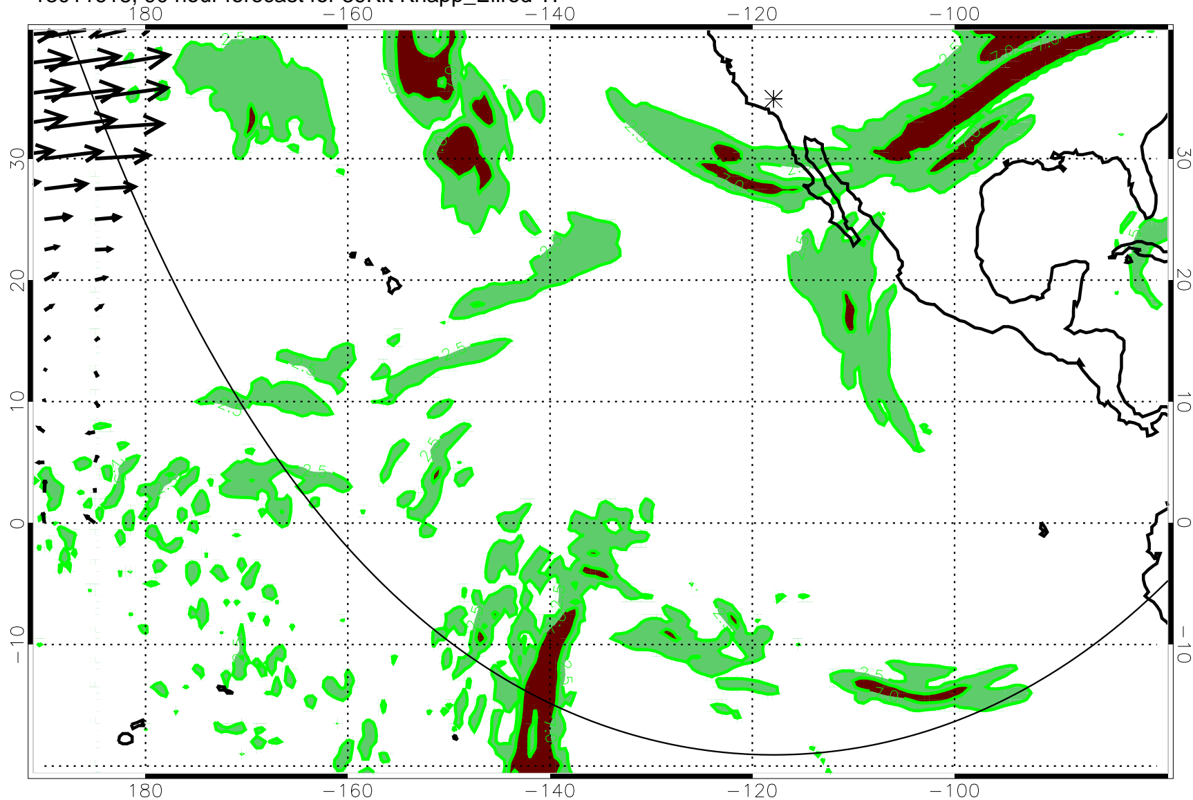
13011618, 90 hour forecast for 39Kft Knapp_Ellrod TI
