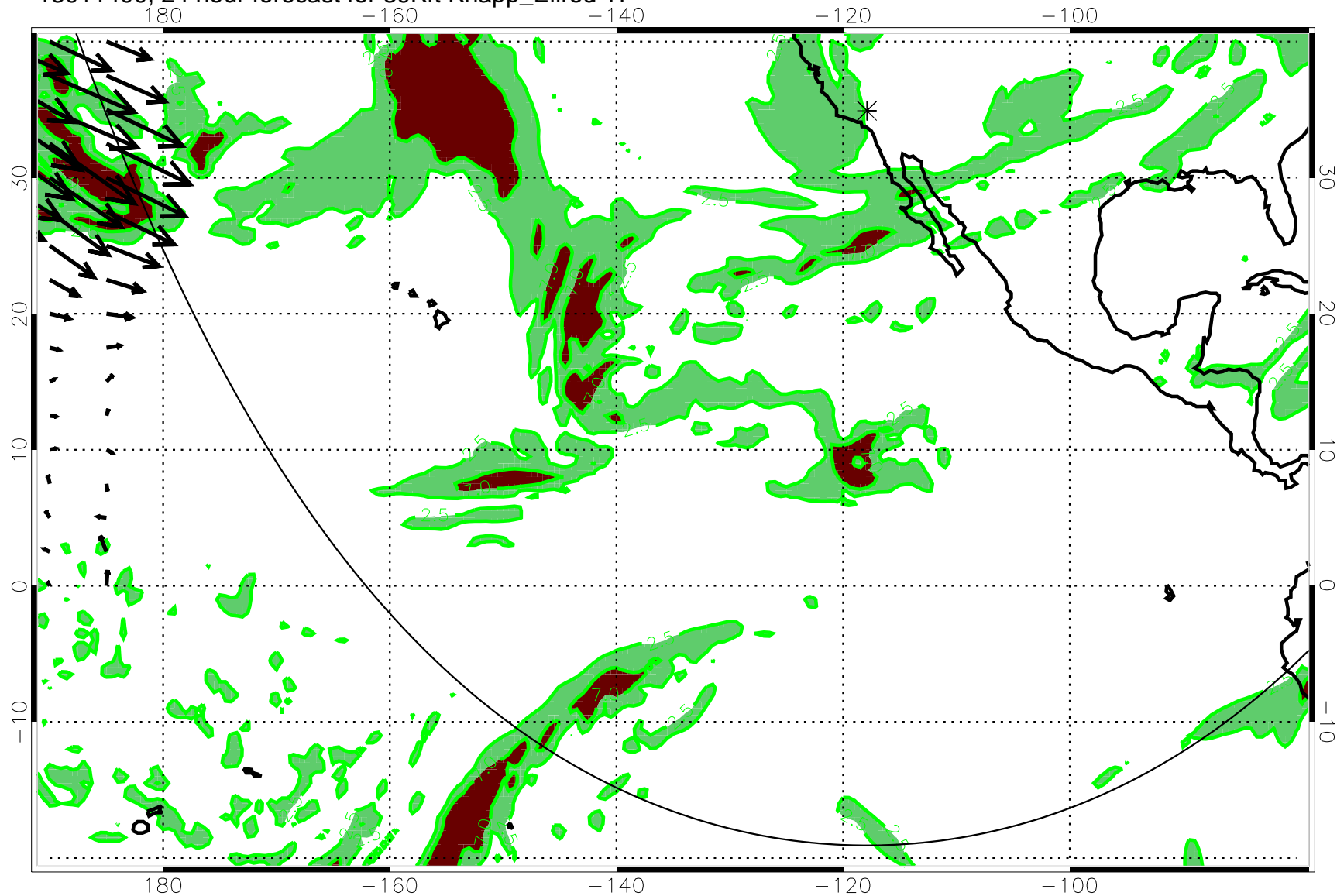
13011400, 24 hour forecast for 39Kft Knapp_Ellrod TI
