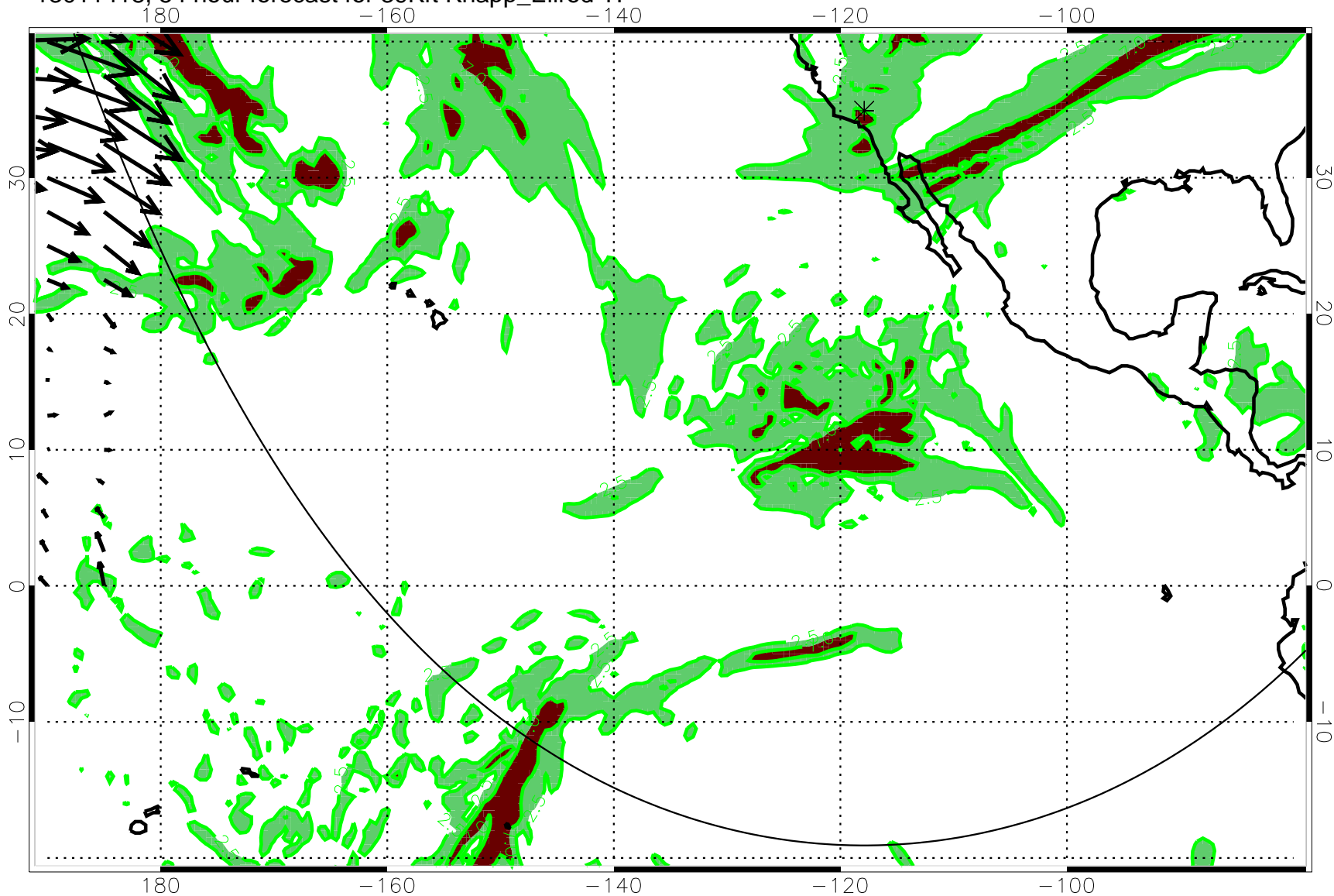
13011418, 54 hour forecast for 39Kft Knapp_Ellrod TI
