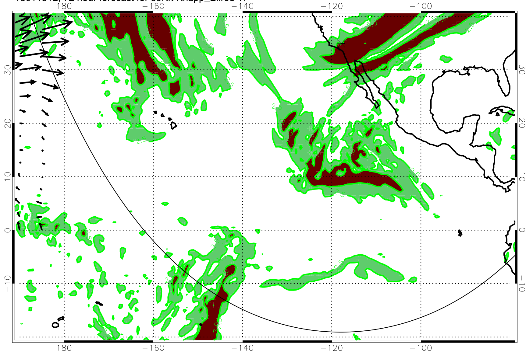
13011512, 72 hour forecast for 39Kft Knapp_Ellrod TI
