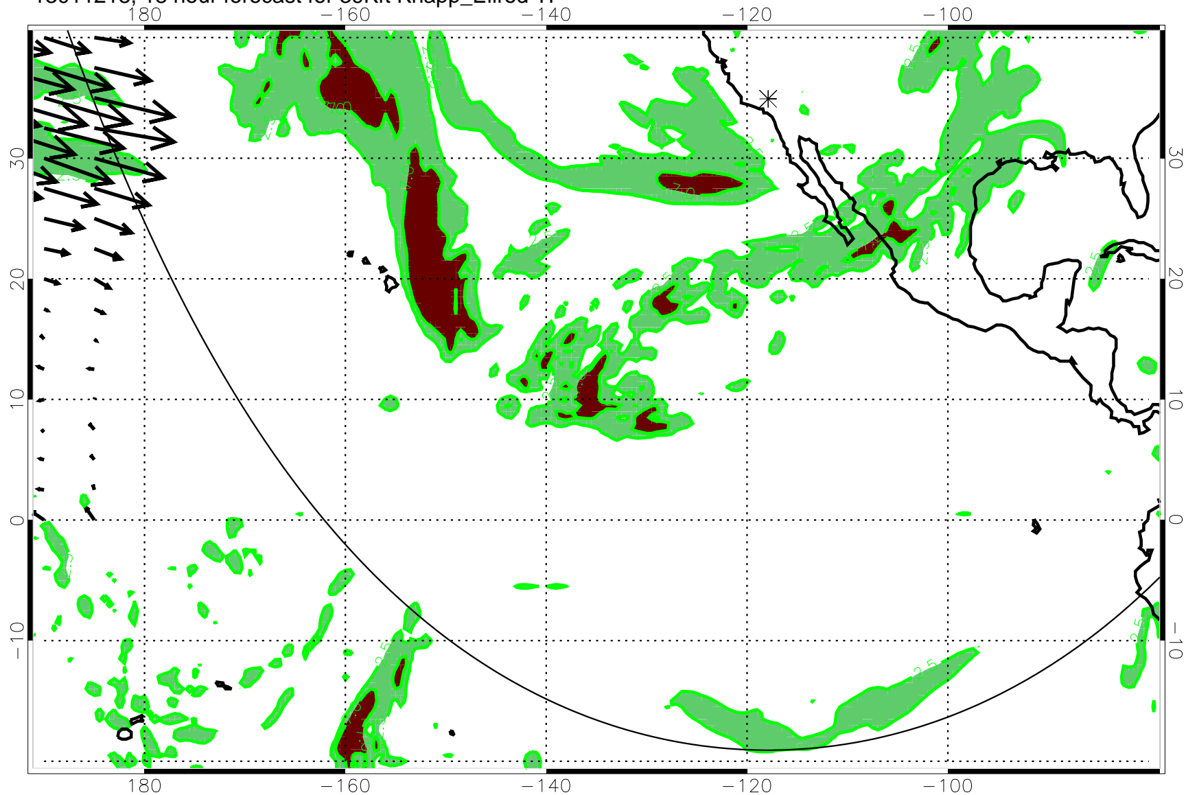
13011218, 18 hour forecast for 39Kft Knapp_Ellrod TI
