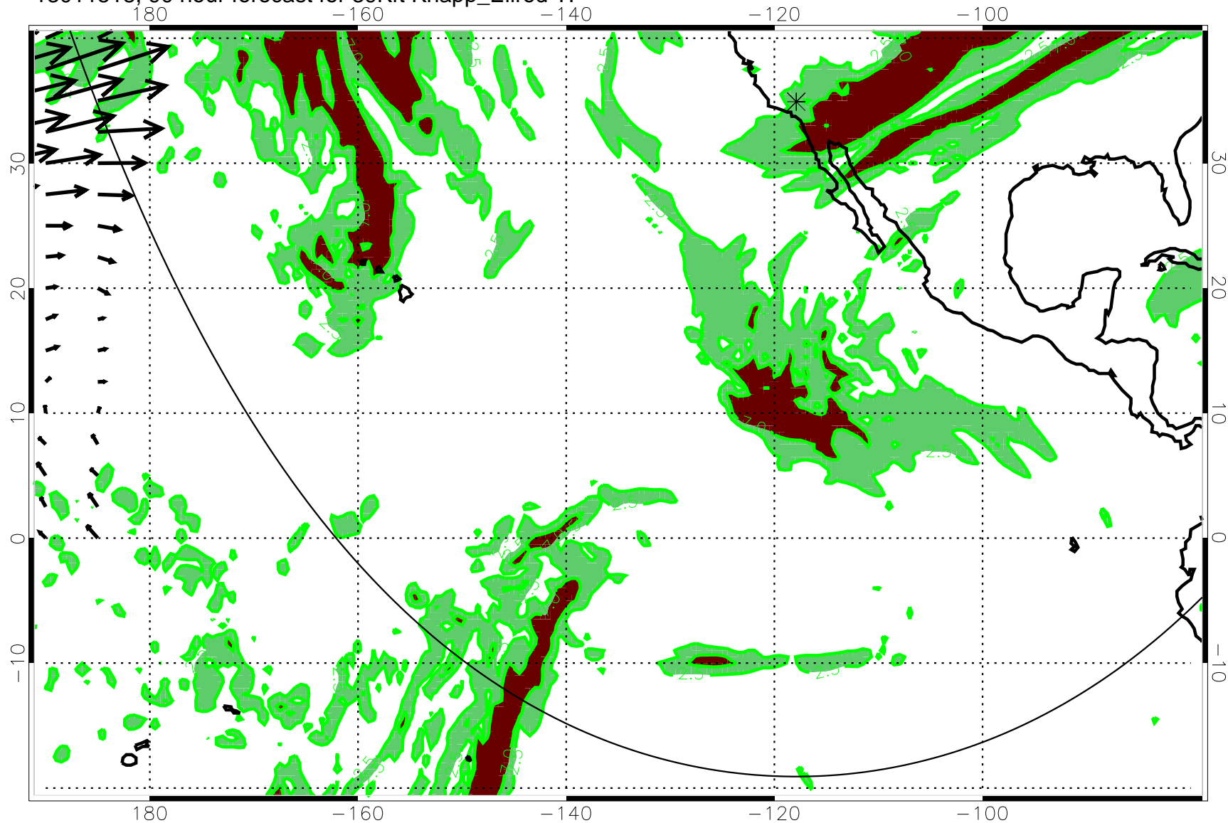
13011518, 90 hour forecast for 39Kft Knapp_Ellrod TI
