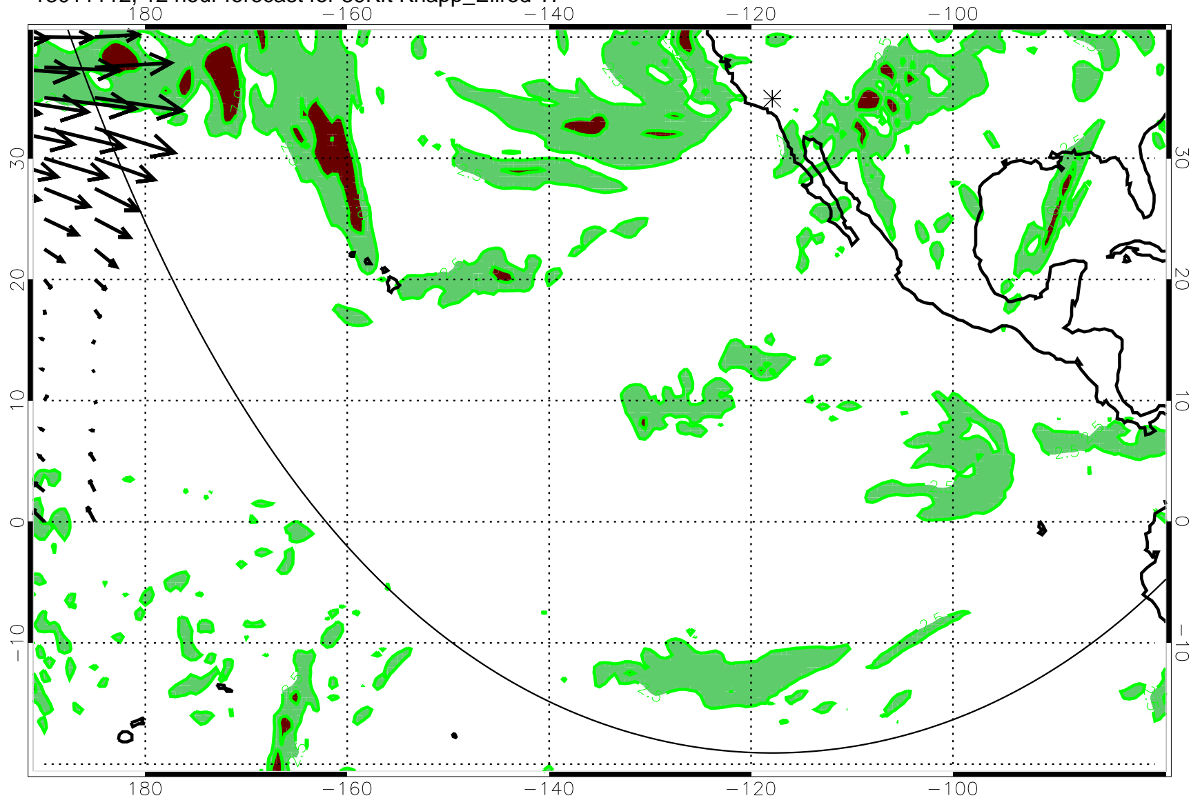
13011112, 12 hour forecast for 39Kft Knapp_Ellrod TI
