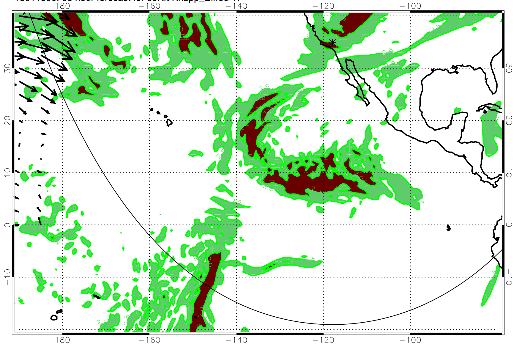
13011500, 96 hour forecast for 39Kft Knapp_Ellrod TI
