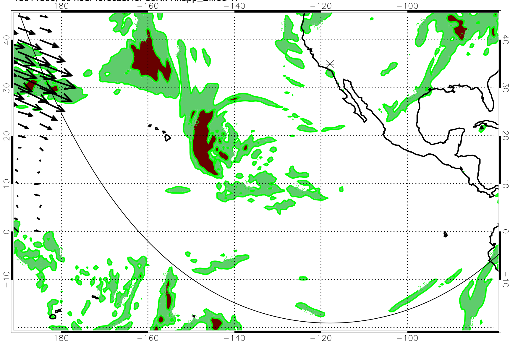
13011306, 66 hour forecast for 39Kft Knapp_Ellrod TI
