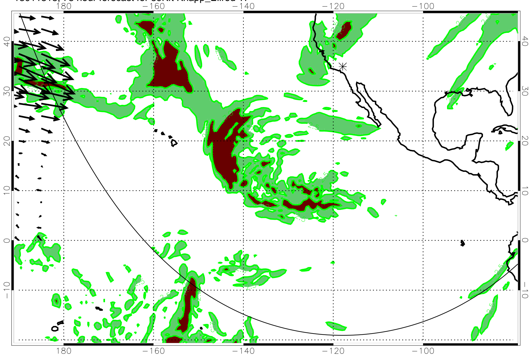
13011318, 78 hour forecast for 39Kft Knapp_Ellrod TI
