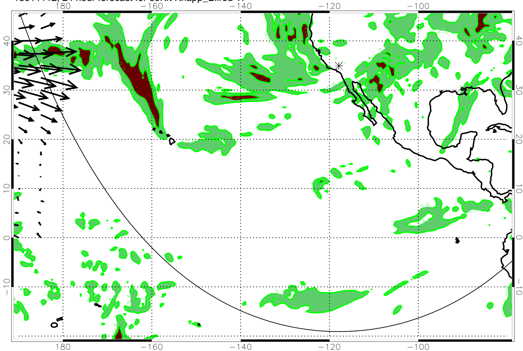
13011112, 24 hour forecast for 39Kft Knapp_Ellrod TI
