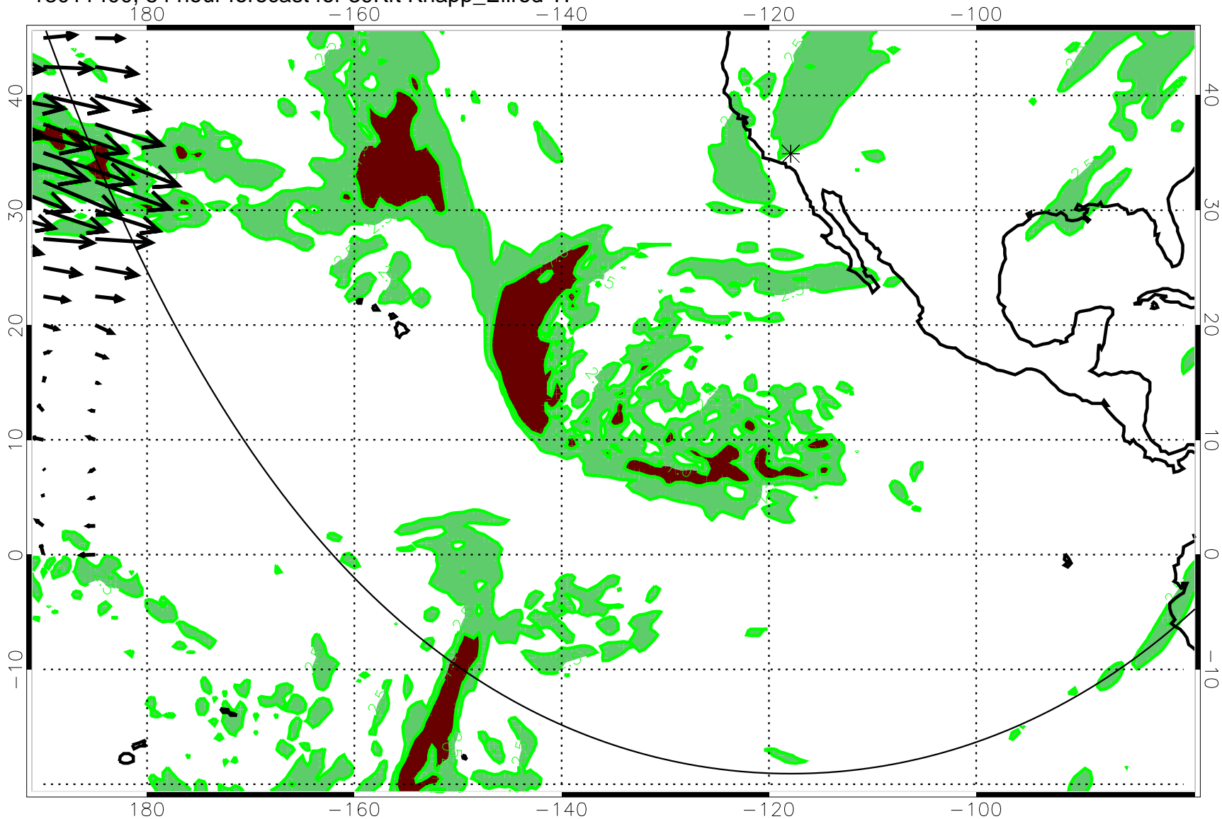
13011400, 84 hour forecast for 39Kft Knapp_Ellrod TI
