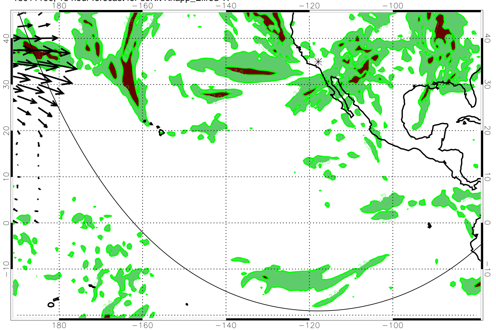
13011106, 18 hour forecast for 39Kft Knapp_Ellrod TI
