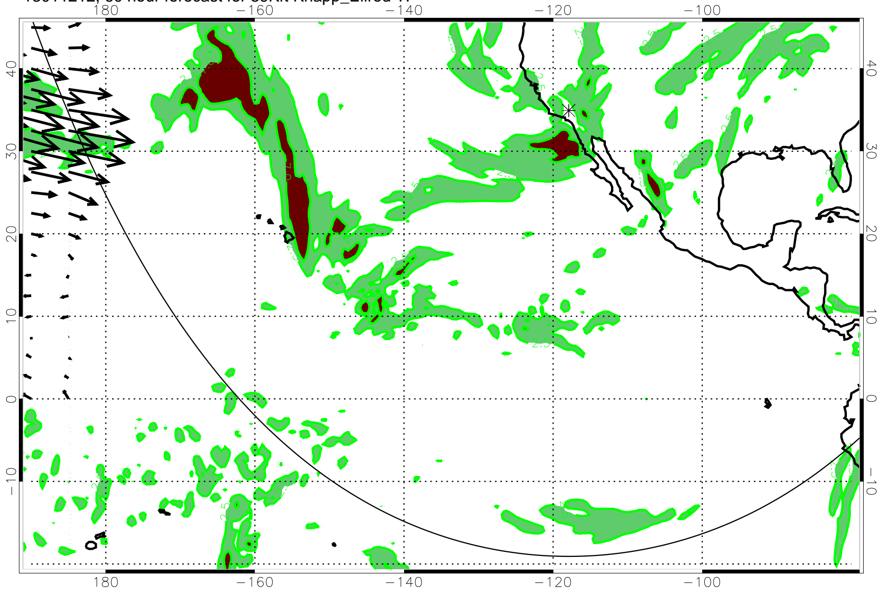
13011212, 60 hour forecast for 39Kft Knapp_Ellrod TI
