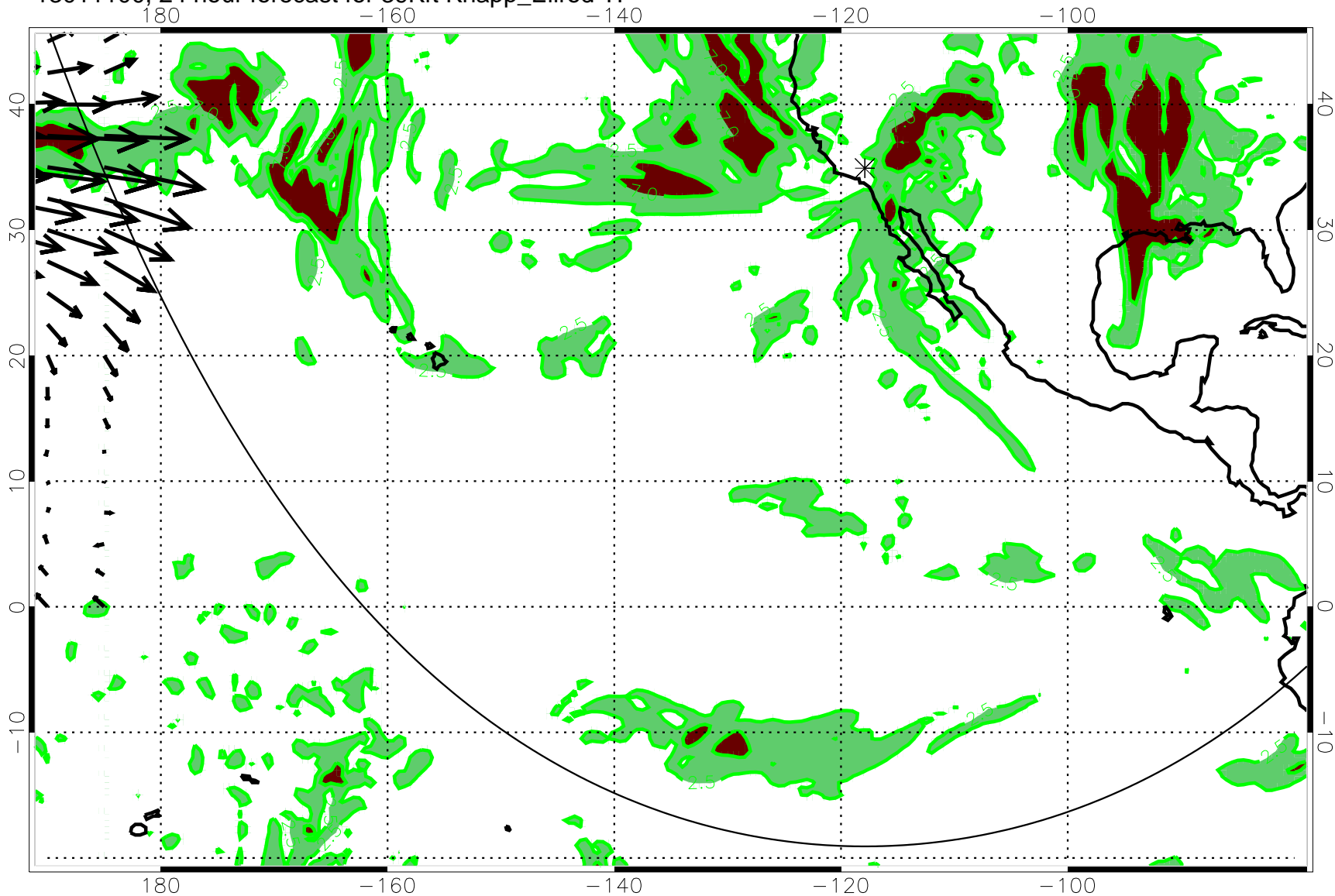
13011100, 24 hour forecast for 39Kft Knapp_Ellrod TI
