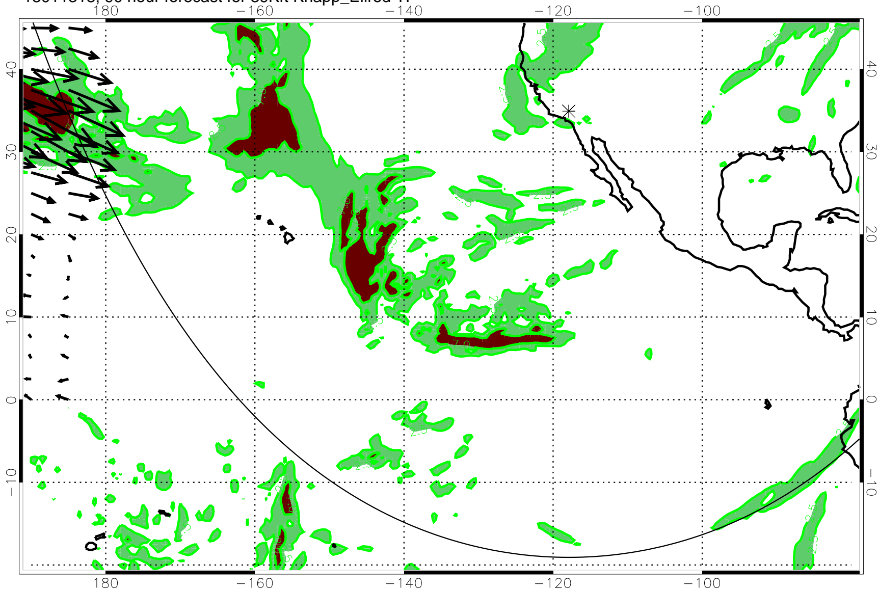
13011318, 90 hour forecast for 39Kft Knapp_Ellrod TI
