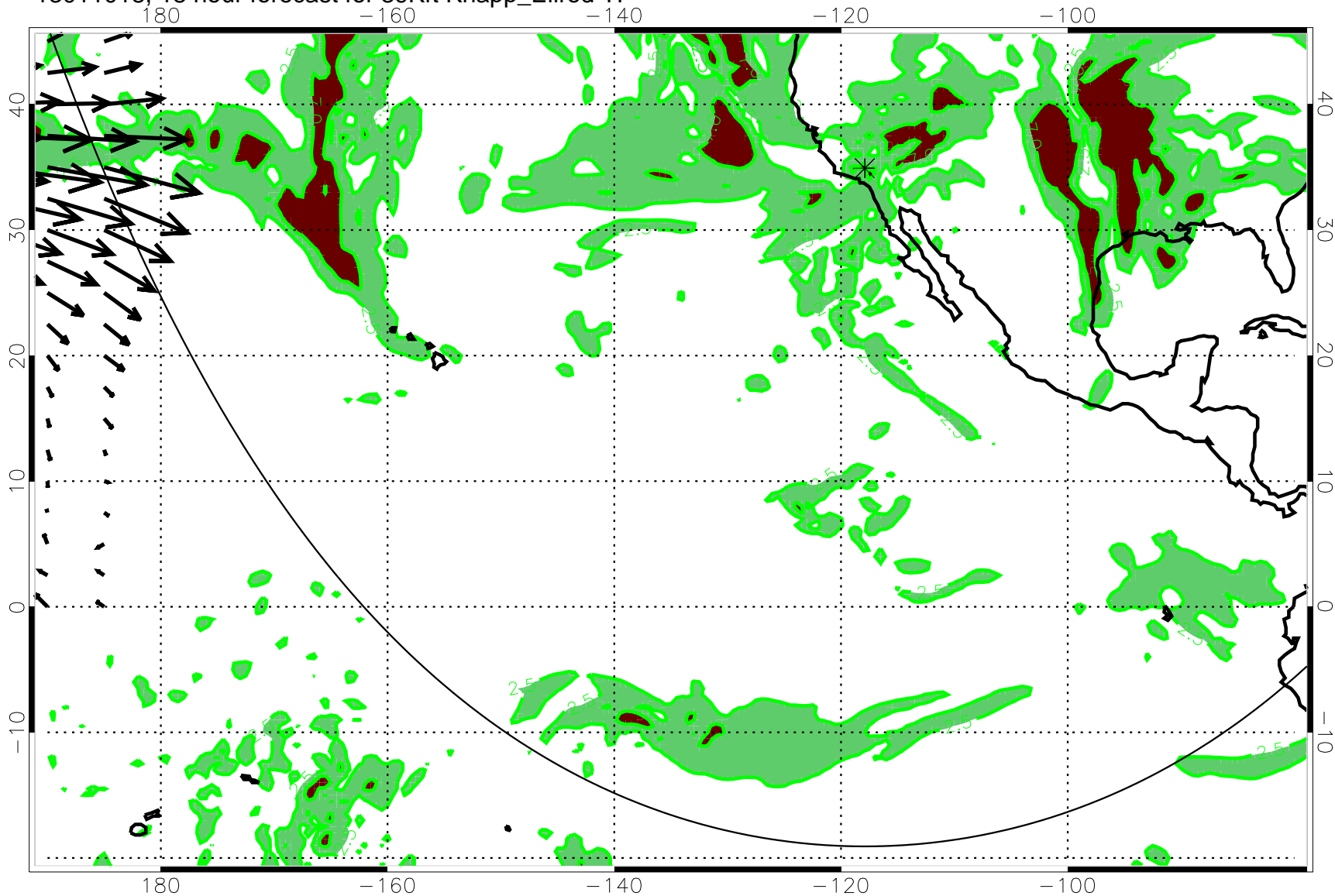
13011018, 18 hour forecast for 39Kft Knapp_Ellrod TI
