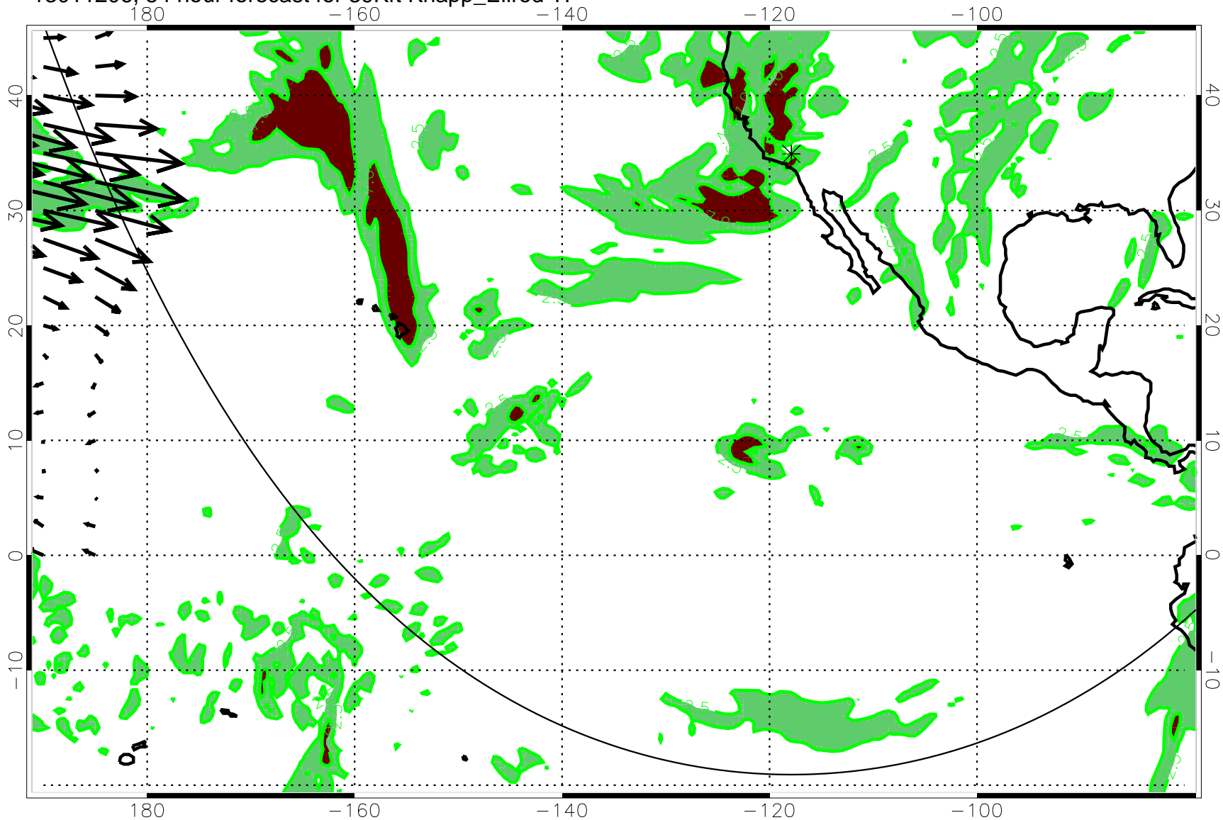
13011206, 54 hour forecast for 39Kft Knapp_Ellrod TI
