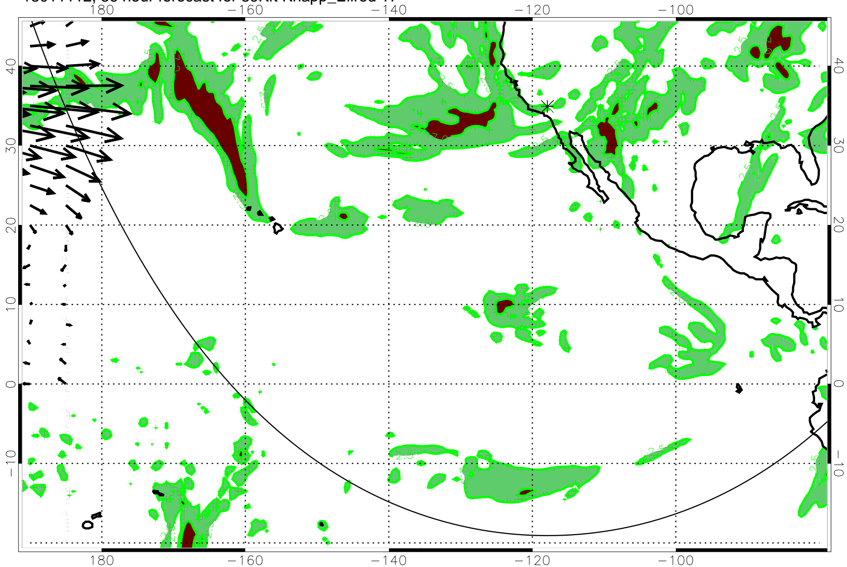
13011112, 36 hour forecast for 39Kft Knapp_Ellrod TI
