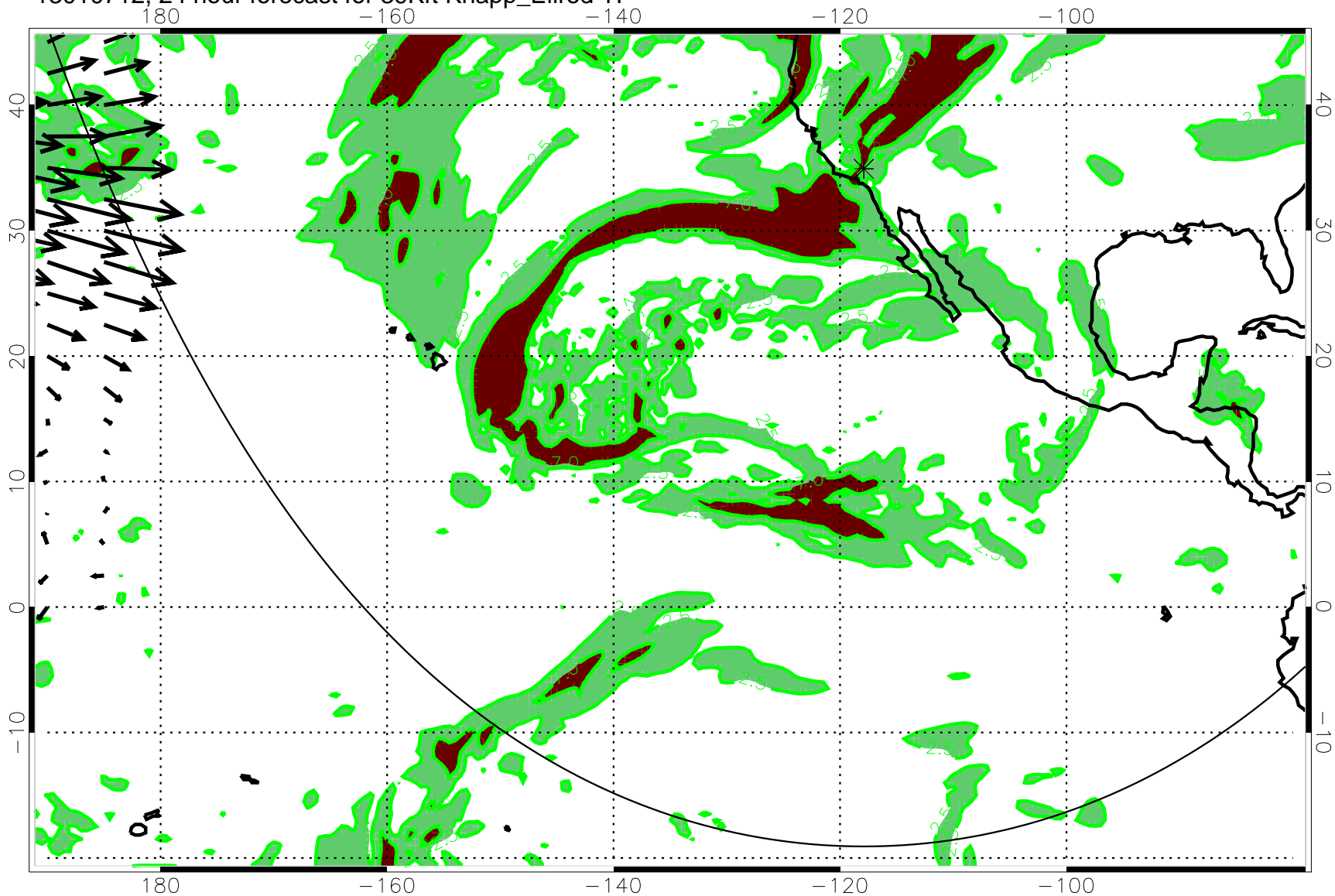
13010712, 24 hour forecast for 39Kft Knapp_Ellrod TI
