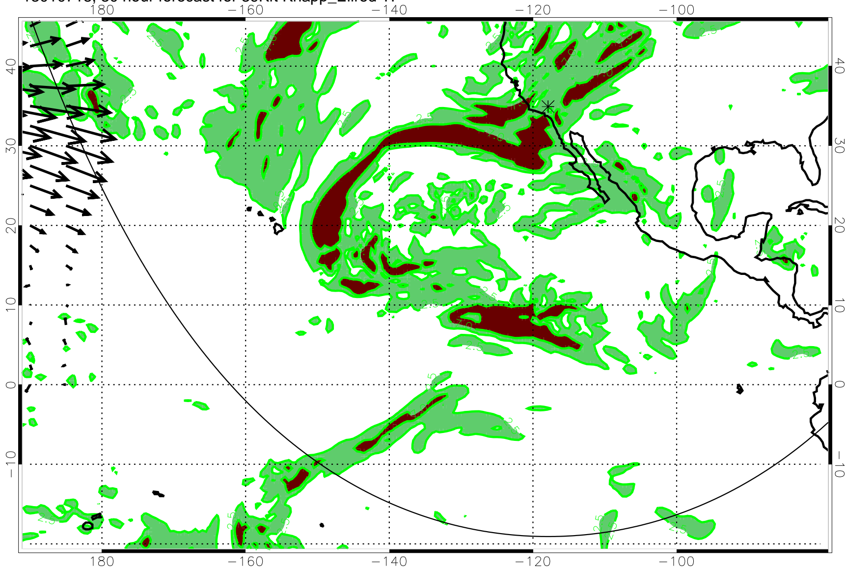
13010718, 30 hour forecast for 39Kft Knapp_Ellrod TI
