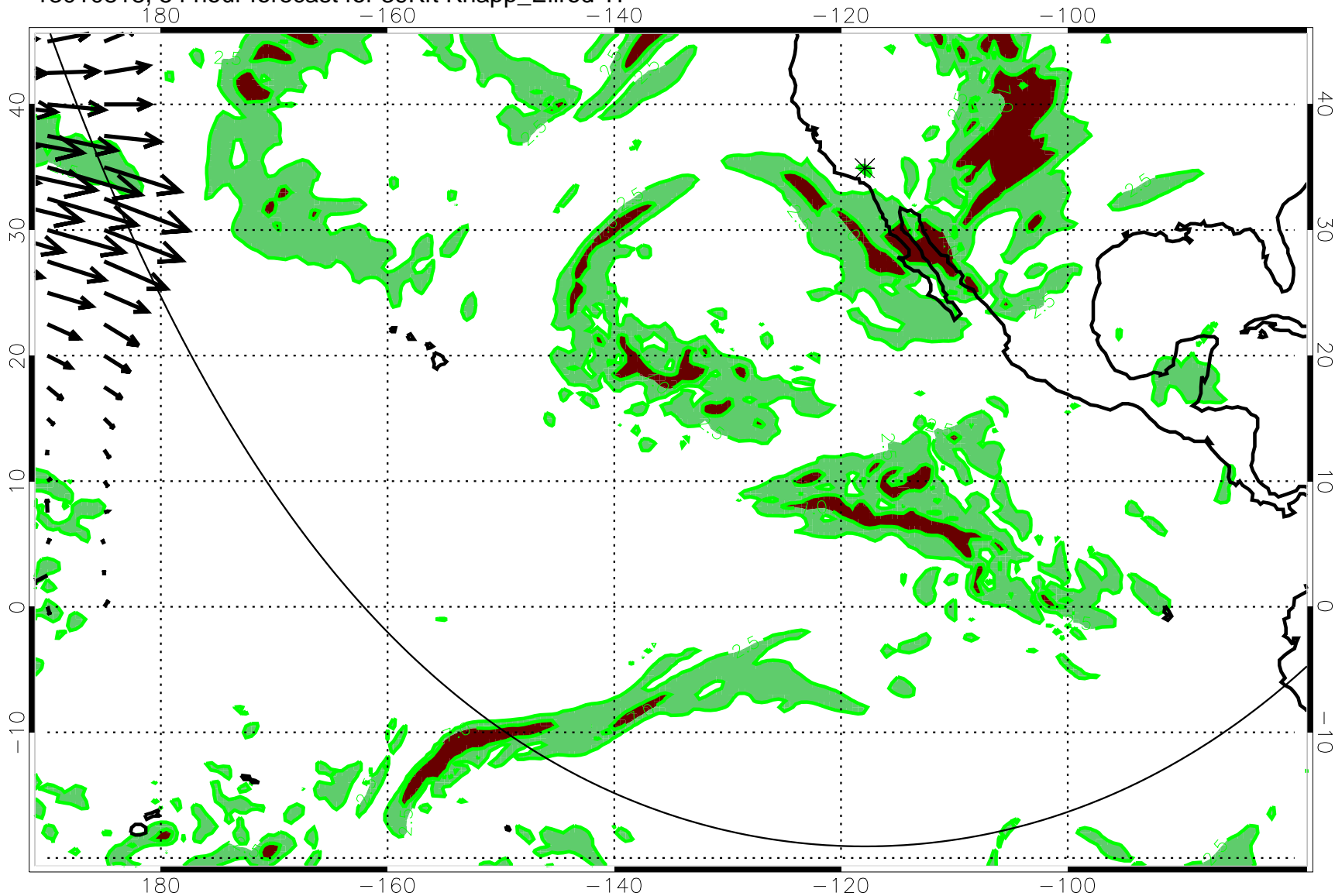
13010818, 54 hour forecast for 39Kft Knapp_Ellrod TI
