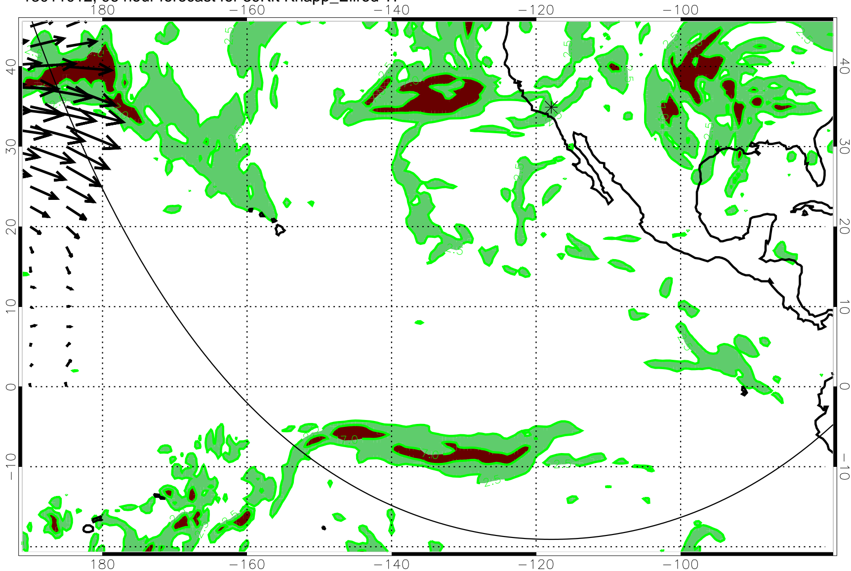
13011012, 96 hour forecast for 39Kft Knapp_Ellrod TI
