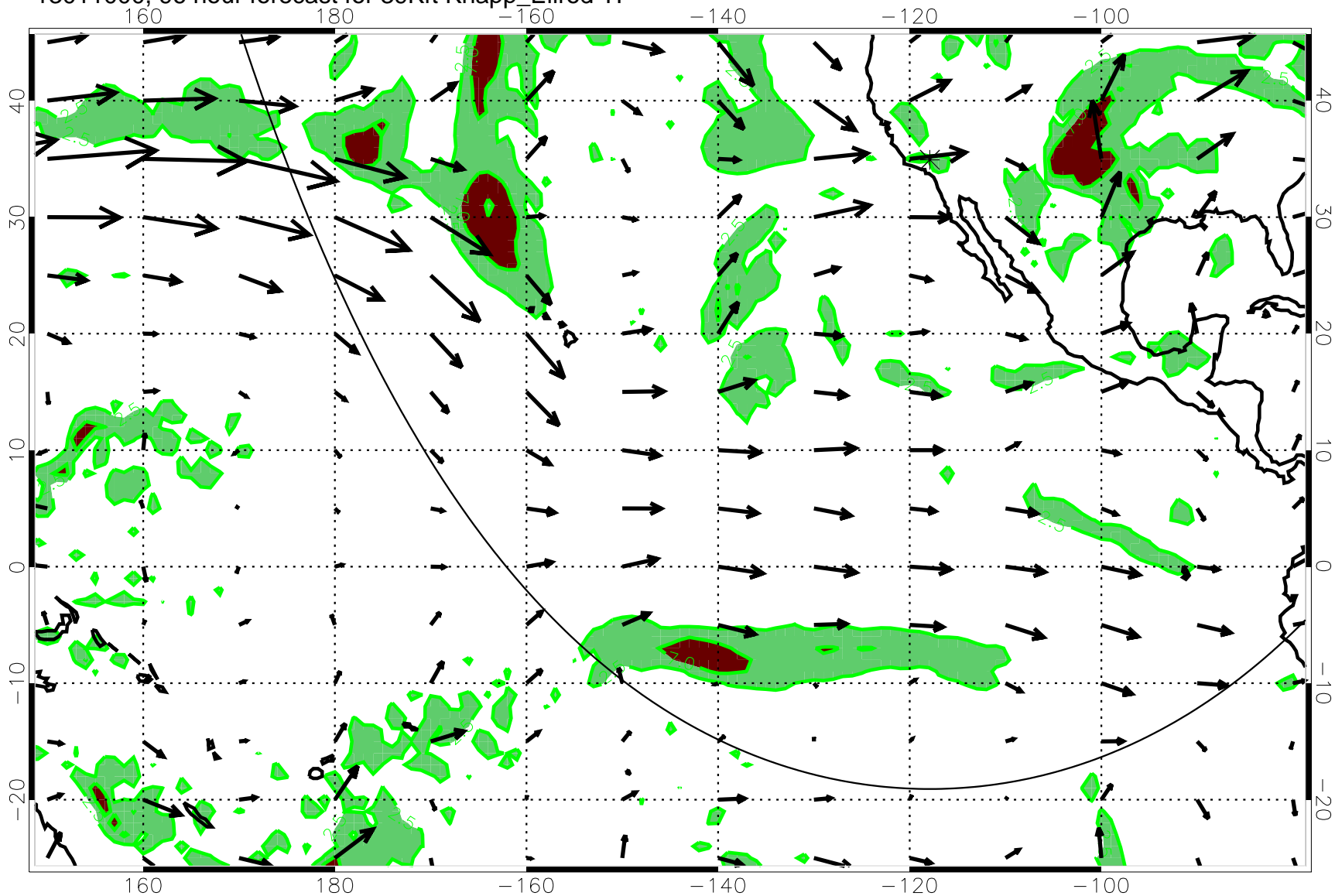
13011000, 96 hour forecast for 39Kft Knapp_Ellrod T1
