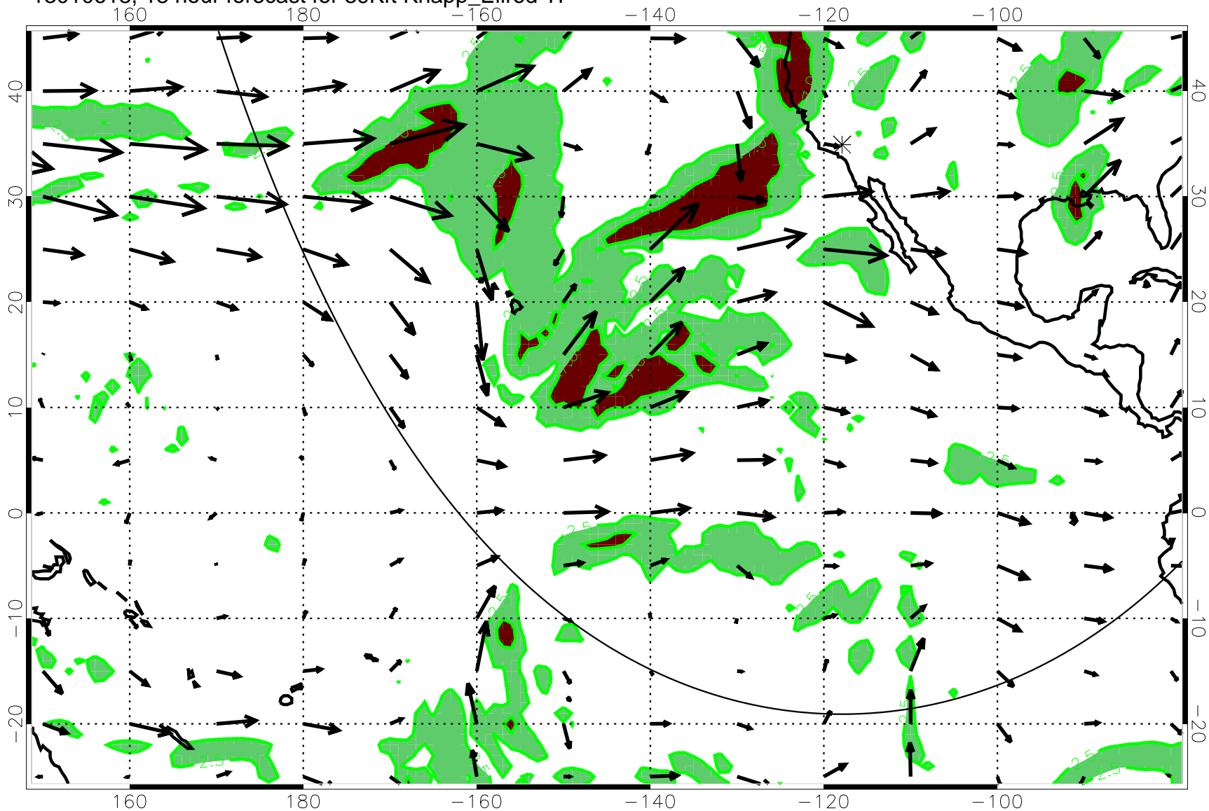
13010618, 18 hour forecast for 39Kft Knapp_Ellrod T1
