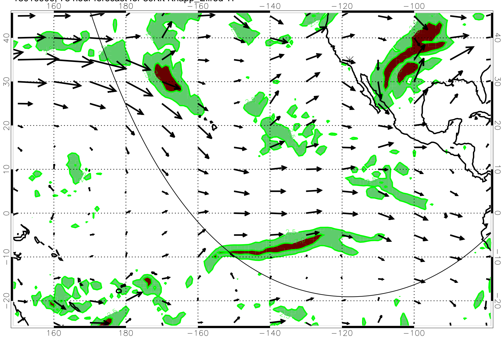
13010906, 78 hour forecast for 39Kft Knapp_Ellrod T1
