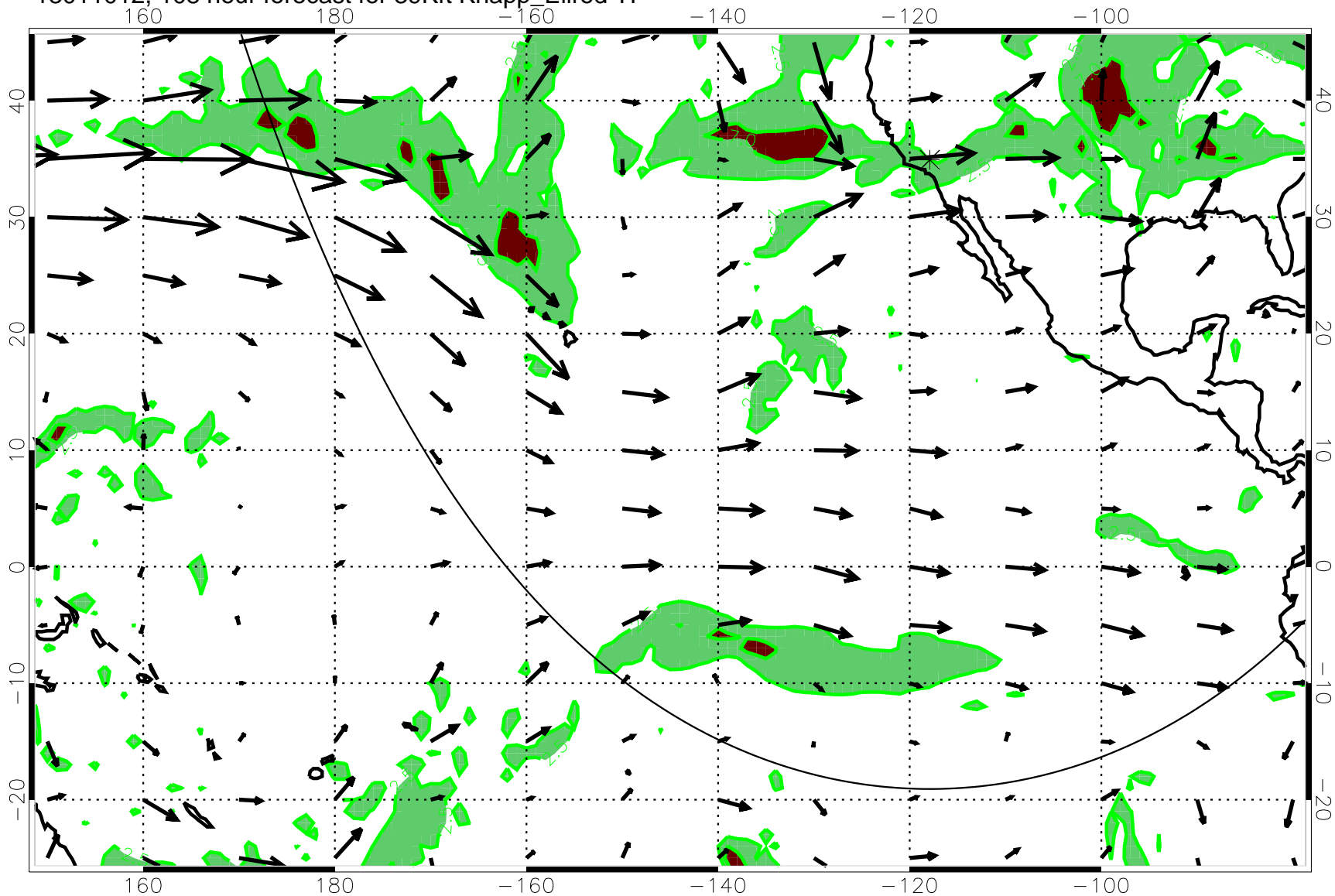
13011012, 108 hour forecast for 39Kft Knapp_Ellrod T1
