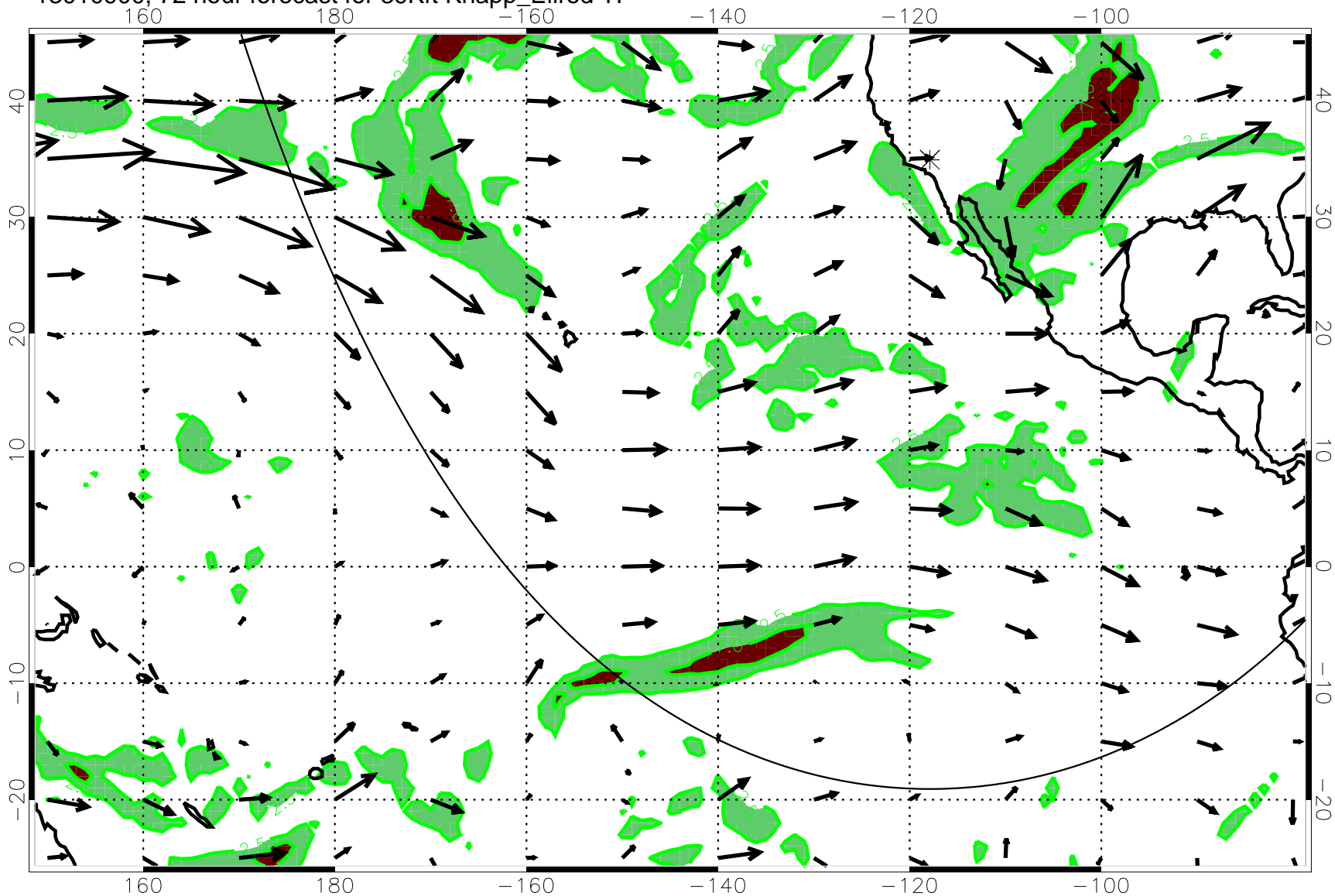
13010900, 72 hour forecast for 39Kft Knapp_Ellrod T1
