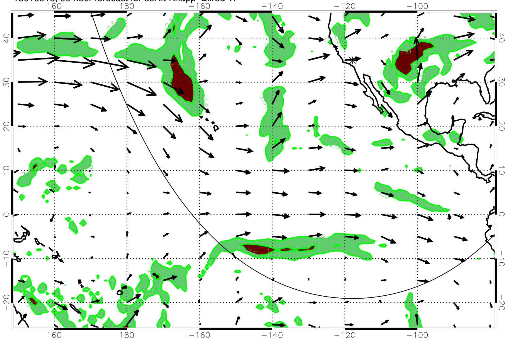
13010918, 90 hour forecast for 39Kft Knapp_Ellrod T1
