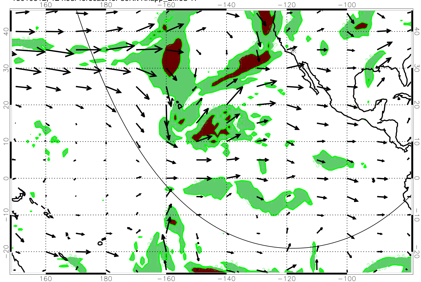
13010612, 12 hour forecast for 39Kft Knapp_Ellrod TI
