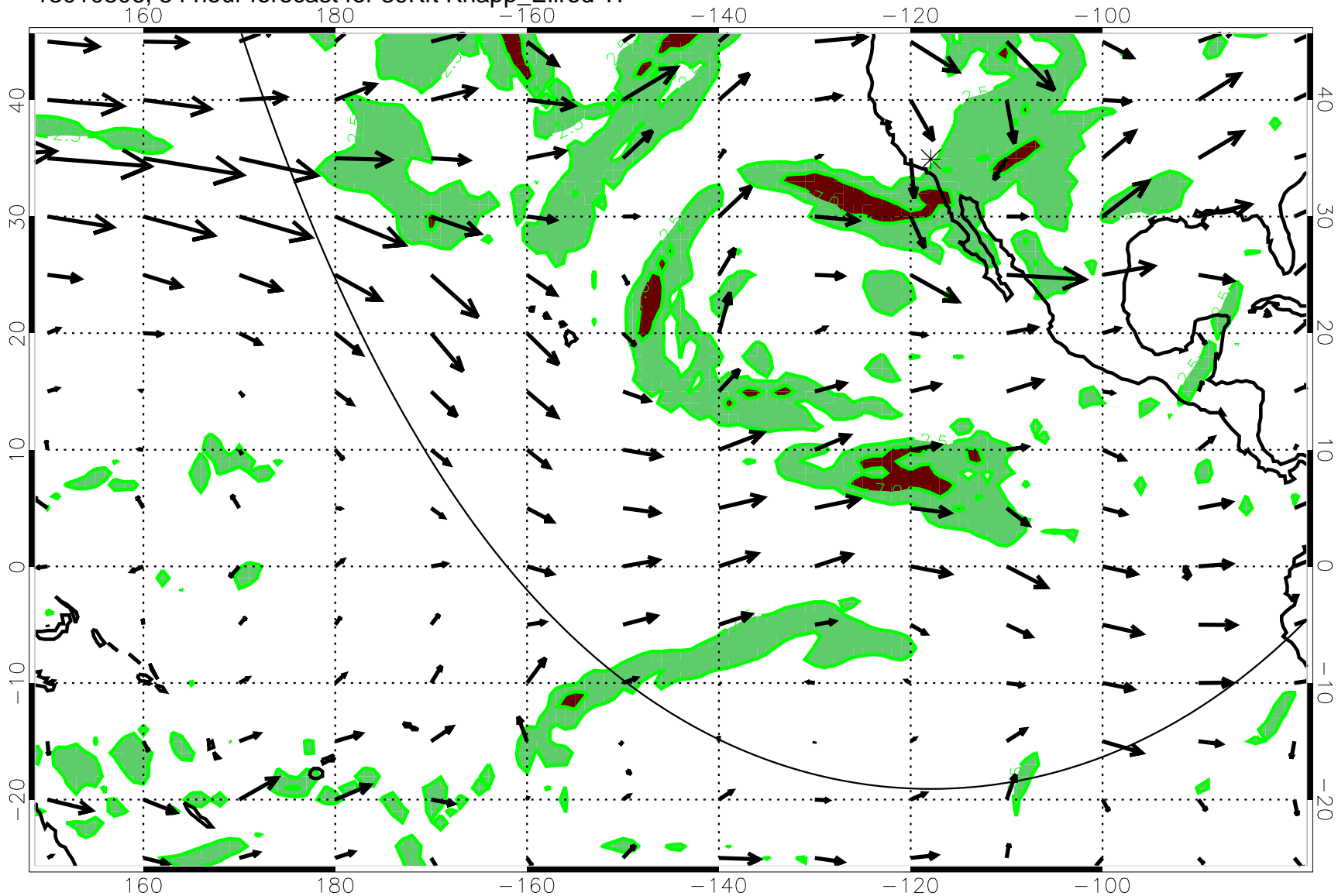
13010806, 54 hour forecast for 39Kft Knapp_Ellrod T1
