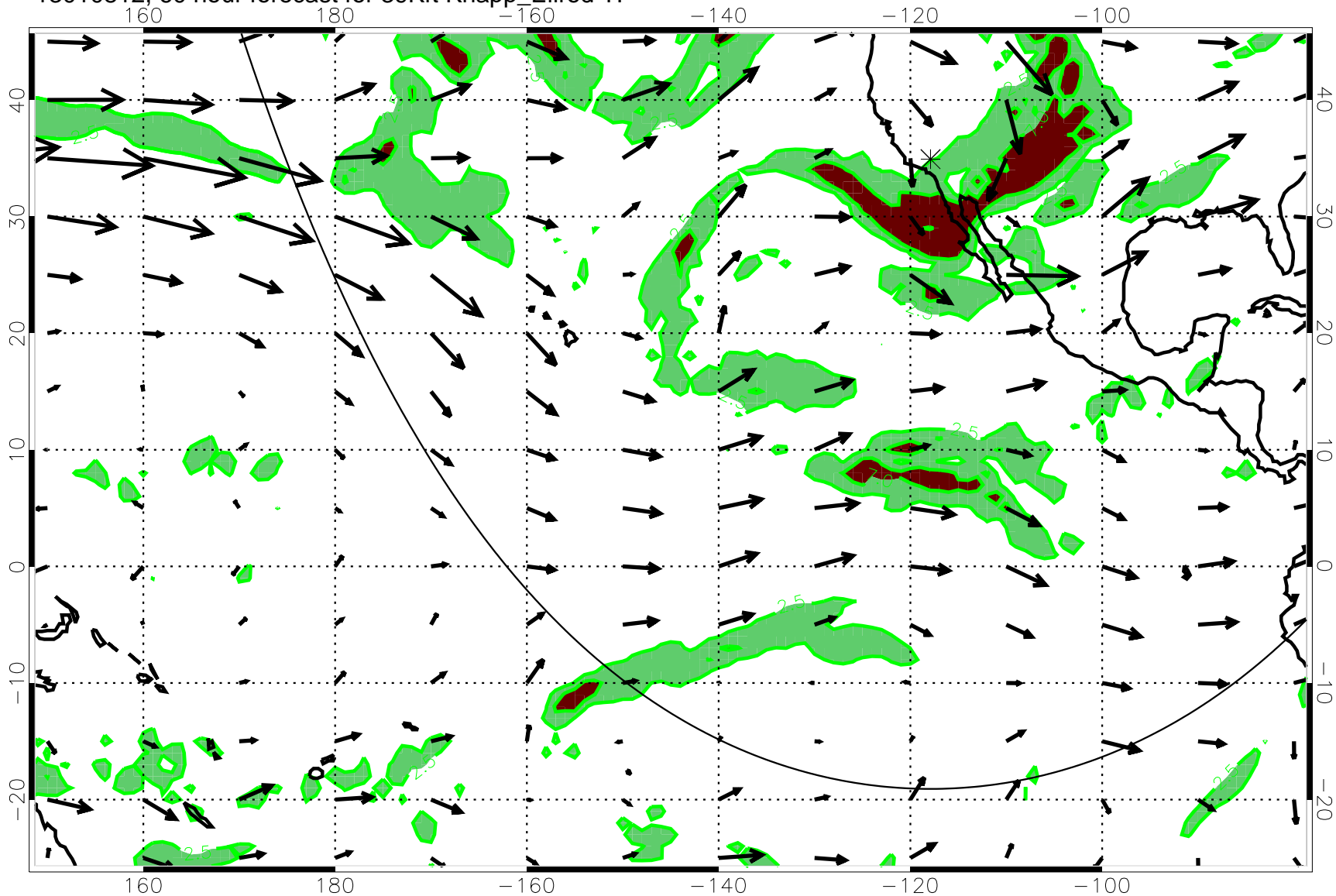
13010812, 60 hour forecast for 39Kft Knapp_Ellrod T1
