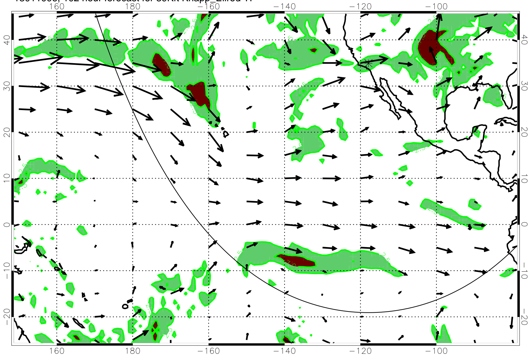
13011006, 102 hour forecast for 39Kft Knapp_Ellrod T1
