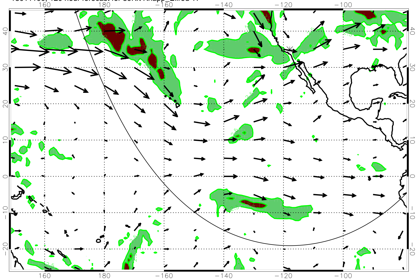
13011100, 120 hour forecast for 39Kft Knapp_Ellrod T1
