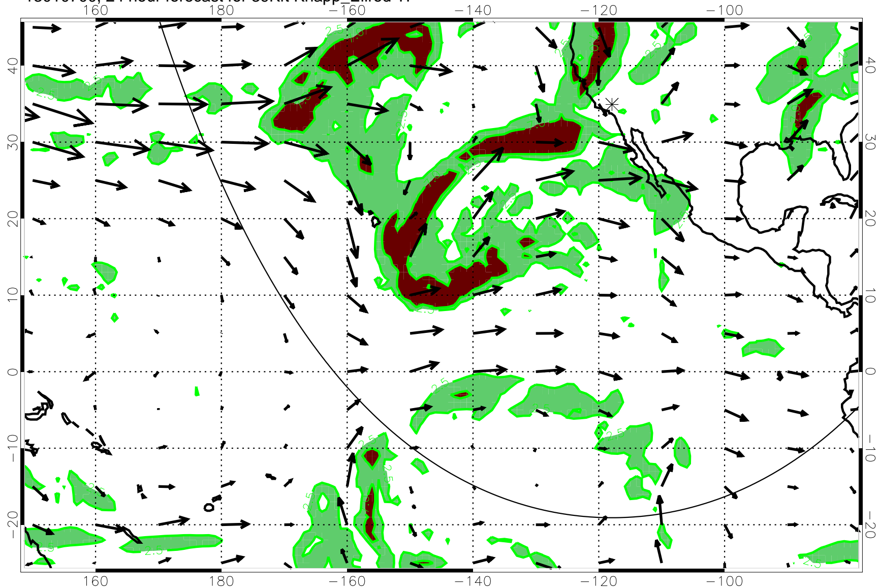
13010700, 24 hour forecast for 39Kft Knapp_Ellrod TI
