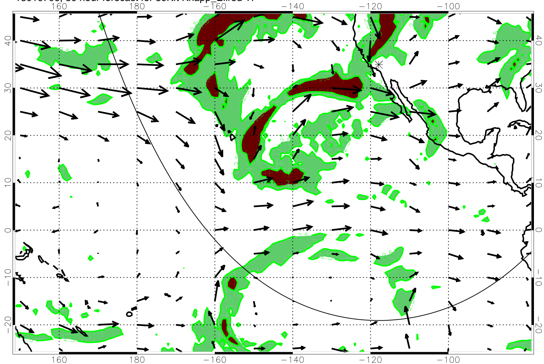
13010706, 30 hour forecast for 39Kft Knapp_Ellrod TI
