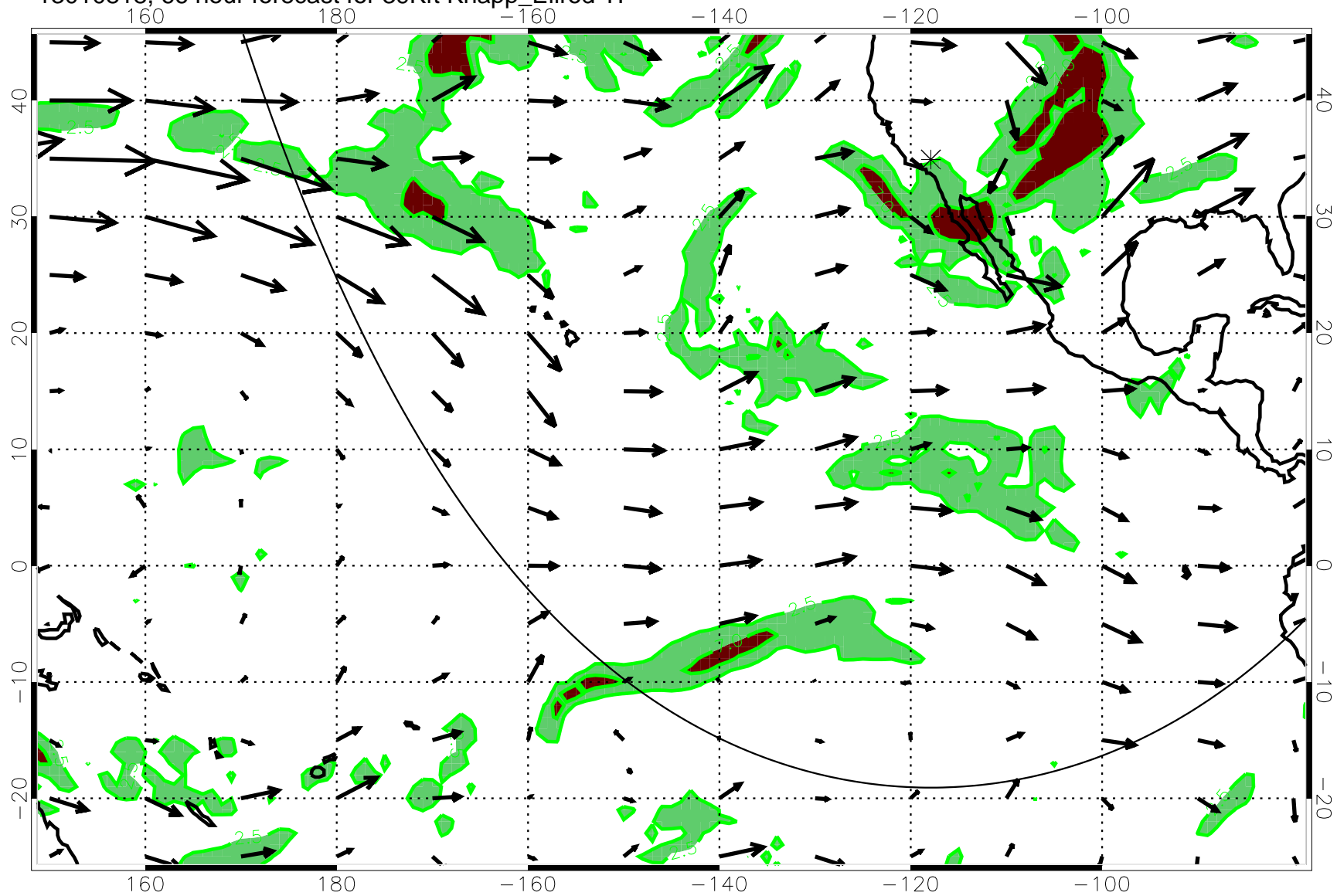
13010818, 66 hour forecast for 39Kft Knapp_Ellrod T1
