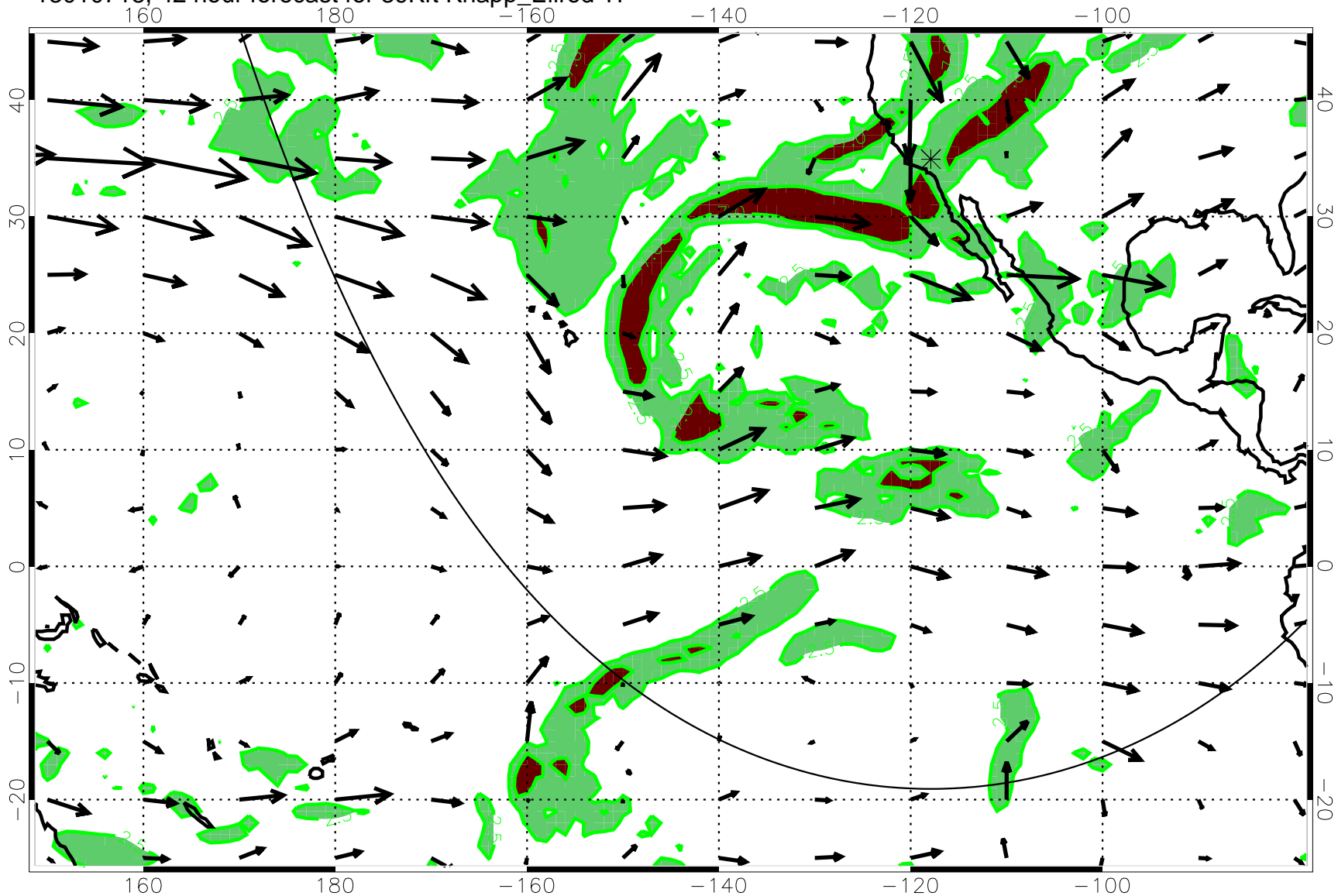
13010718, 42 hour forecast for 39Kft Knapp_Ellrod TI
