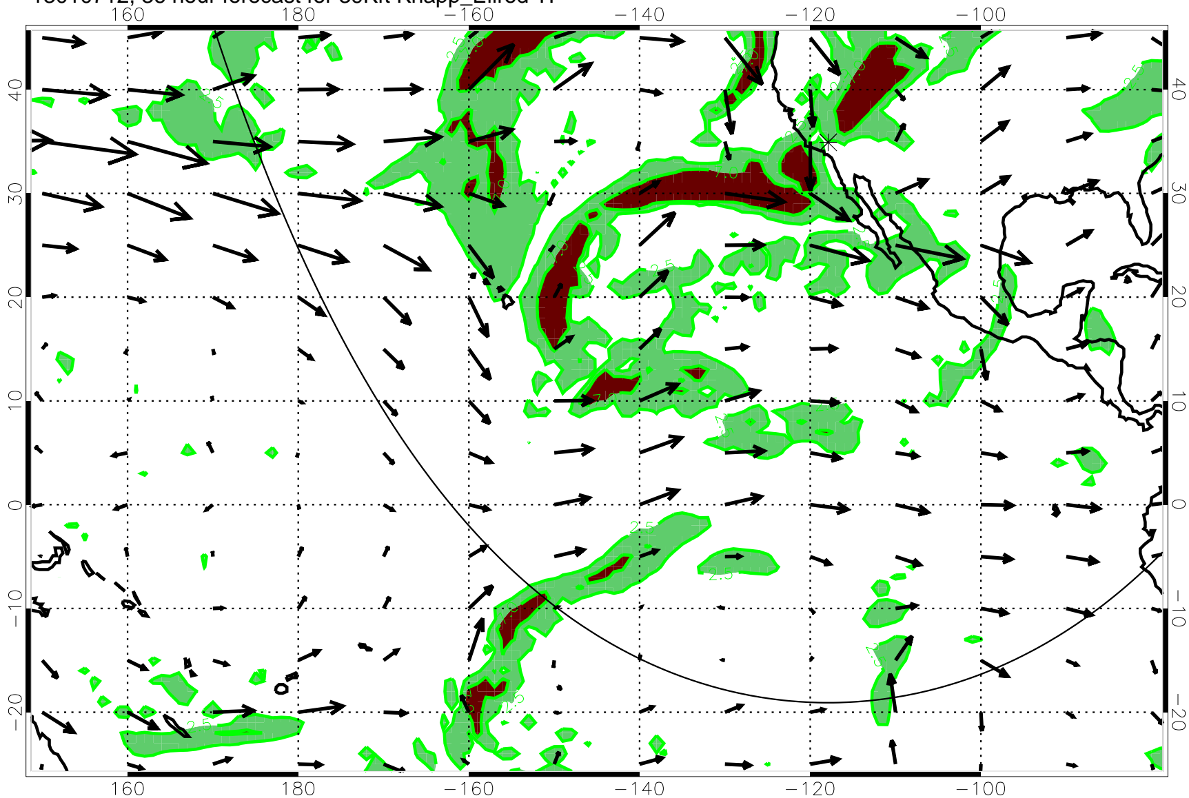
13010712, 36 hour forecast for 39Kft Knapp_Ellrod TI
