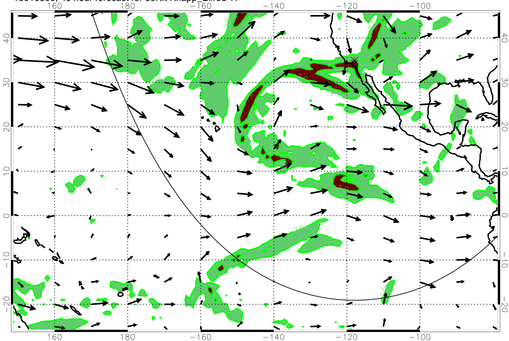
13010800, 48 hour forecast for 39Kft Knapp_Ellrod T1
