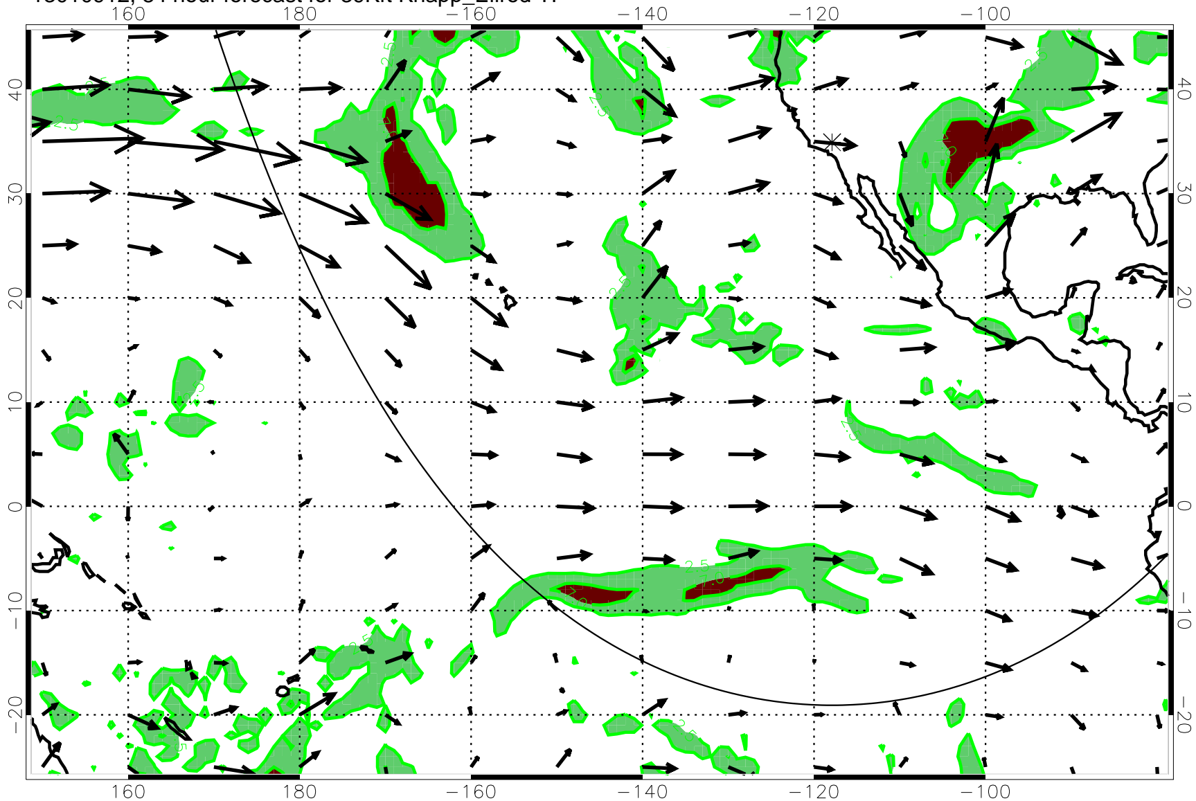
13010912, 84 hour forecast for 39Kft Knapp_Ellrod T1
