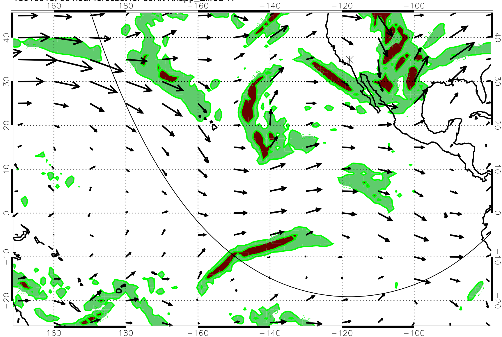
13010818, 90 hour forecast for 39Kft Knapp_Ellrod T1
