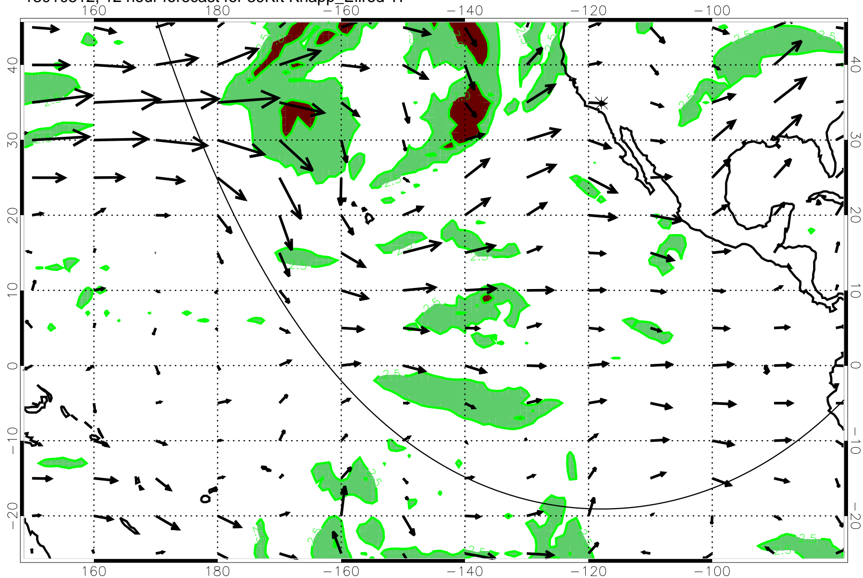
13010512, 12 hour forecast for 39Kft Knapp_Ellrod TI
