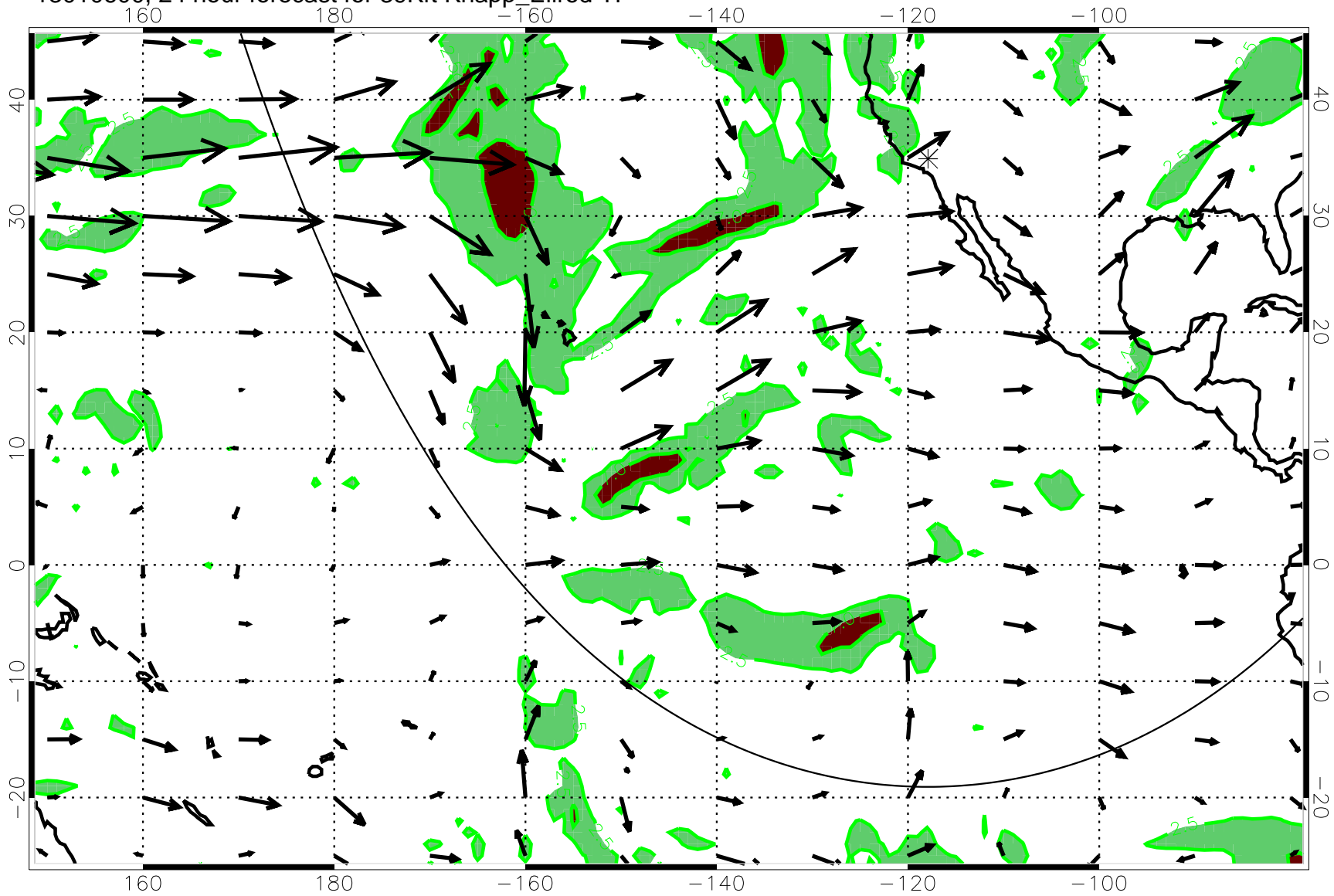
13010600, 24 hour forecast for 39Kft Knapp_Ellrod TI
