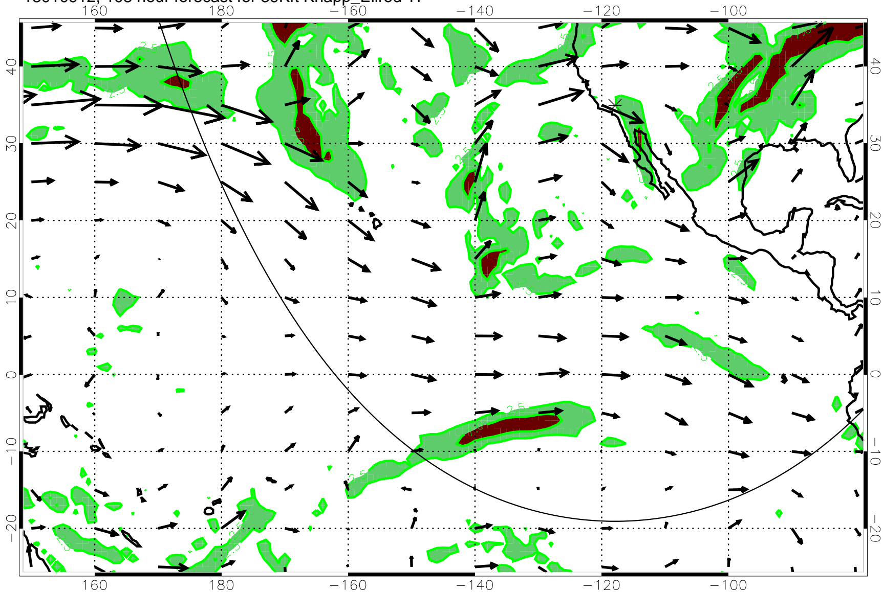
13010912, 108 hour forecast for 39Kft Knapp_Ellrod T1
