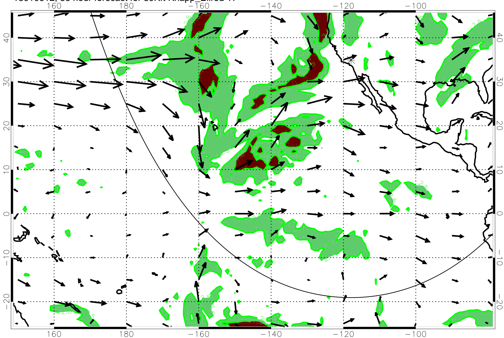
13010612, 36 hour forecast for 39Kft Knapp_Ellrod T1
