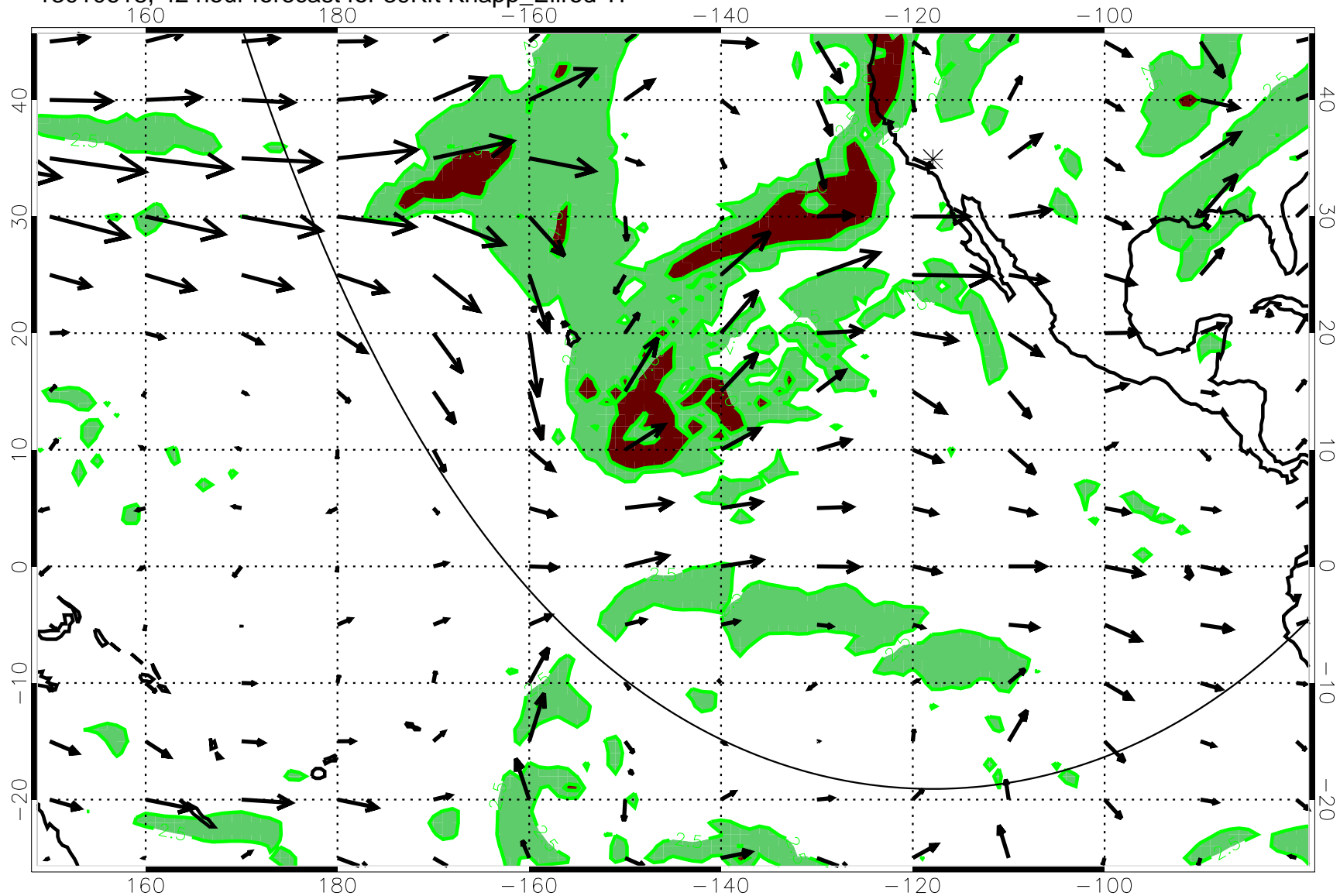
13010618, 42 hour forecast for 39Kft Knapp_Ellrod T1
