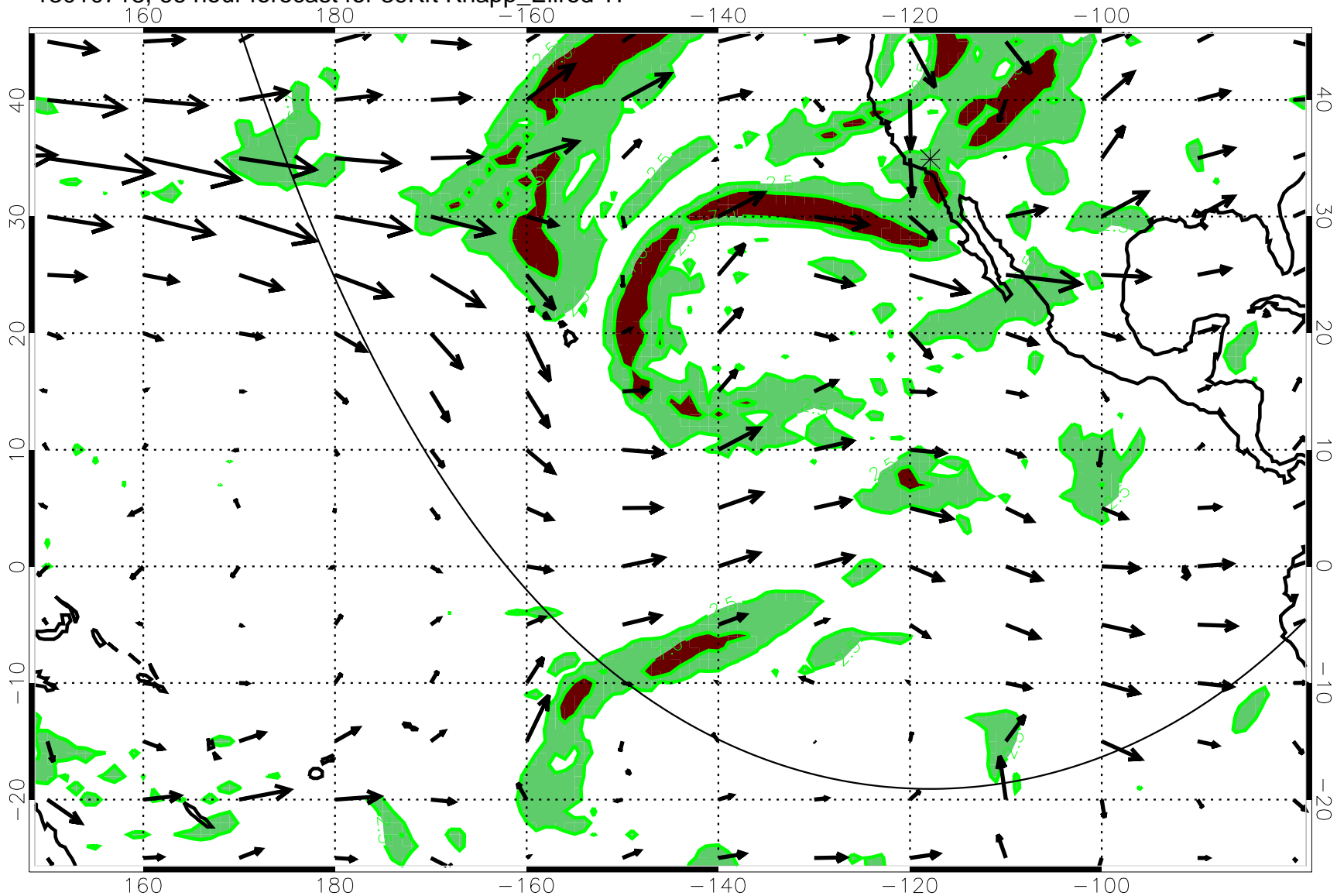
13010718, 66 hour forecast for 39Kft Knapp_Ellrod T1
