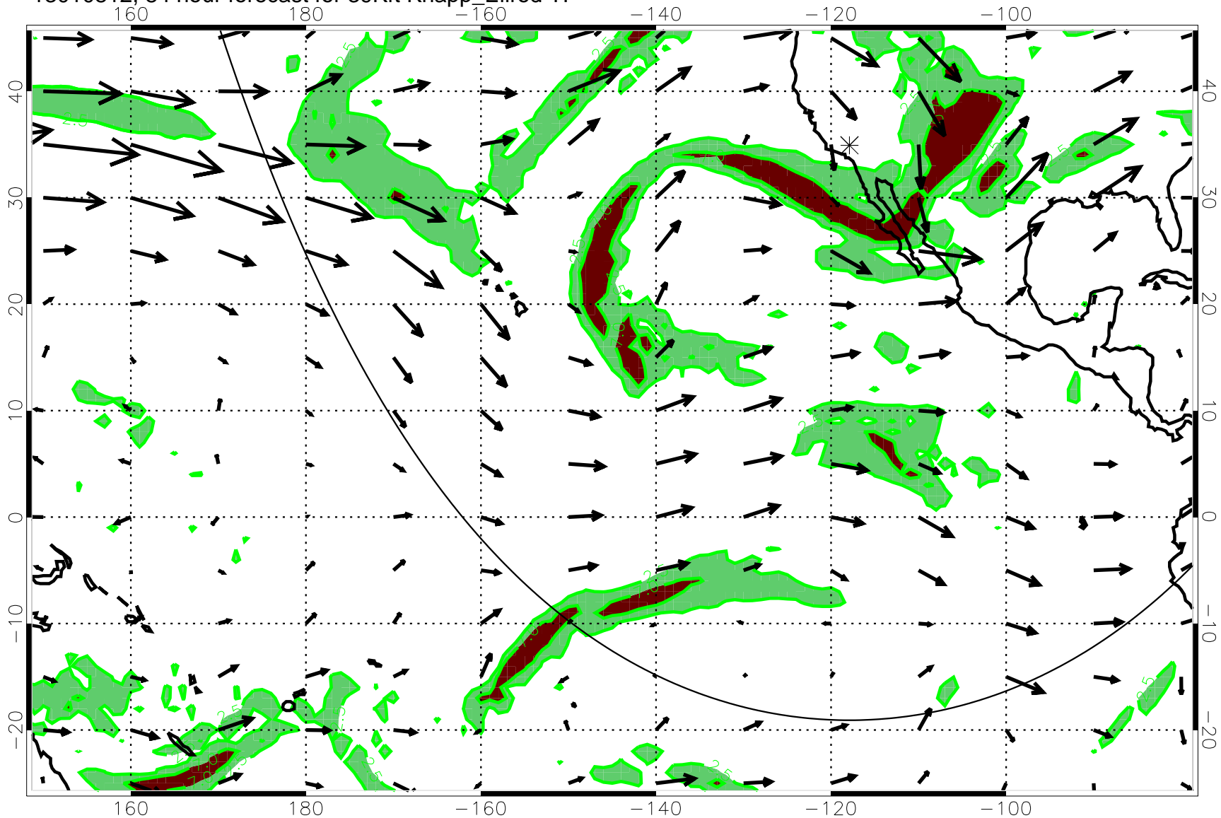
13010812, 84 hour forecast for 39Kft Knapp_Ellrod T1
