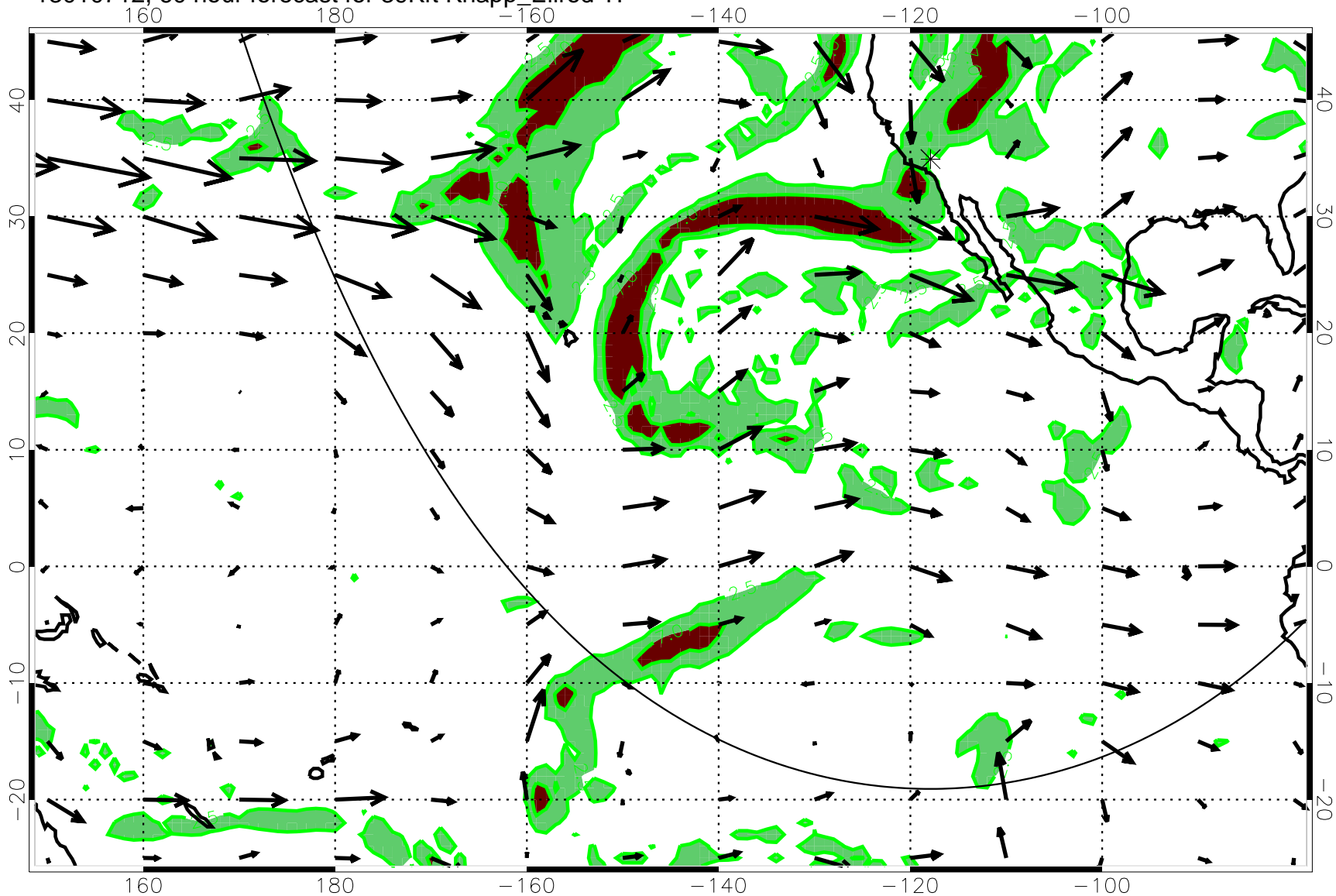
13010712, 60 hour forecast for 39Kft Knapp_Ellrod TI
