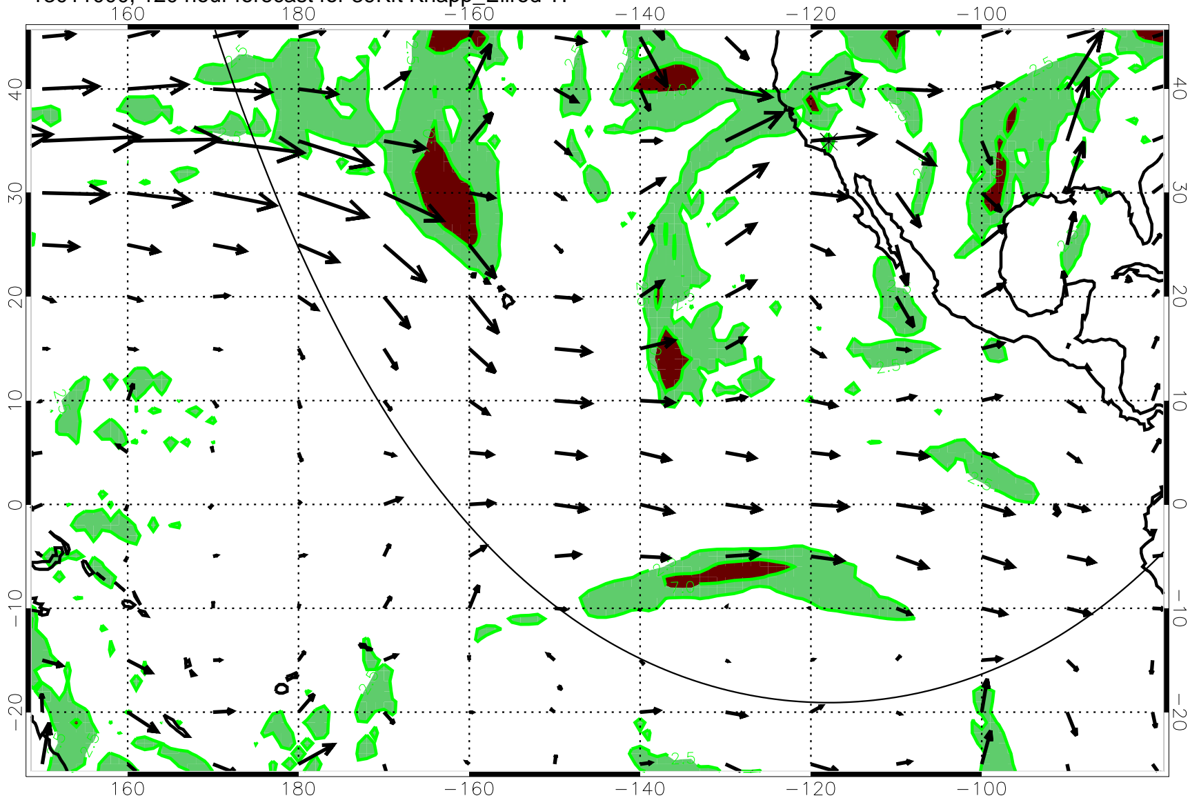
13011000, 120 hour forecast for 39Kft Knapp_Ellrod T1
