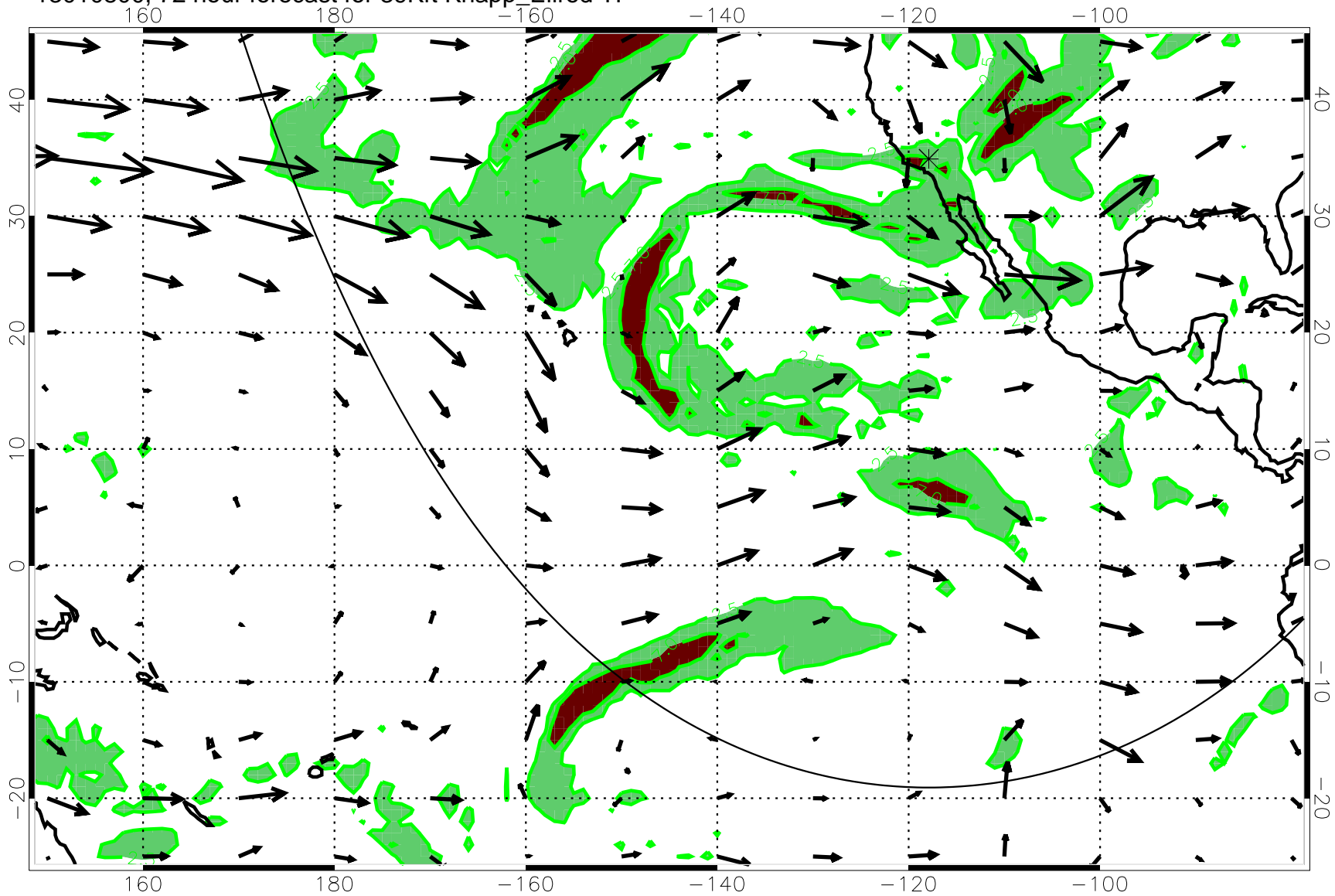
13010800, 72 hour forecast for 39Kft Knapp_Ellrod T1
