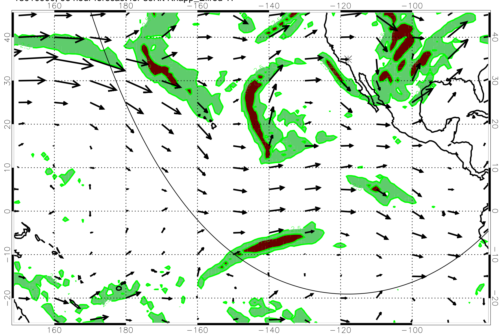
13010900, 96 hour forecast for 39Kft Knapp_Ellrod T1
