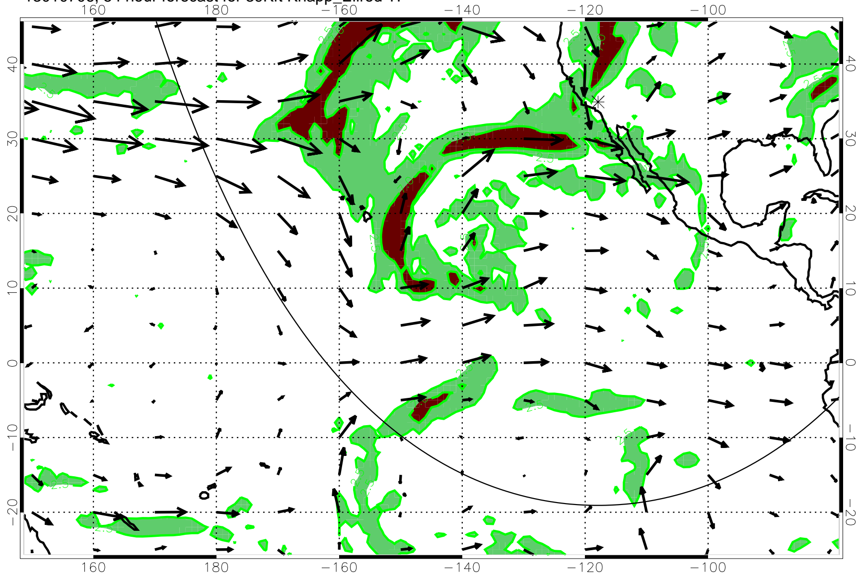
13010706, 54 hour forecast for 39Kft Knapp_Ellrod T1
