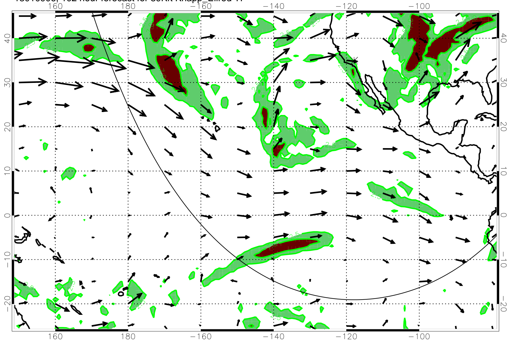
13010906, 102 hour forecast for 39Kft Knapp_Ellrod T1
