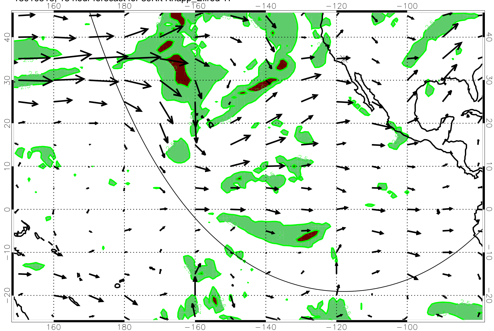
13010518, 18 hour forecast for 39Kft Knapp_Ellrod T1
