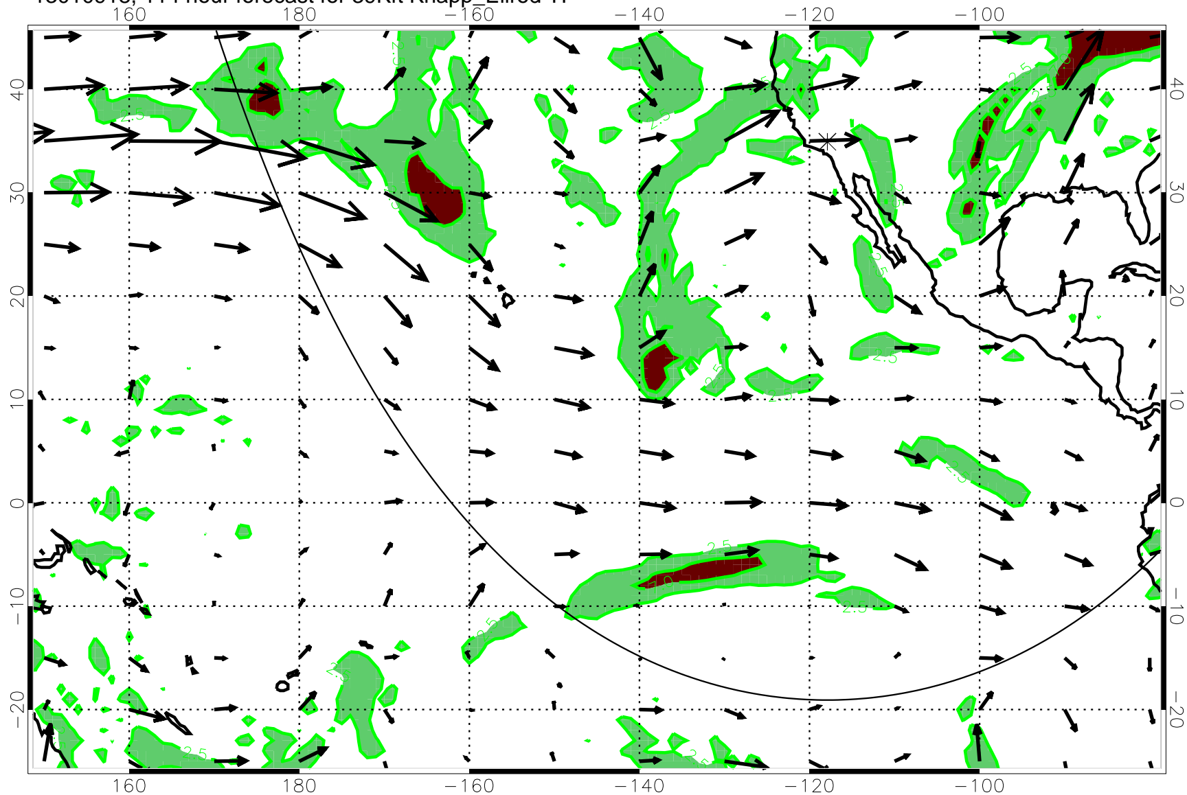
13010918, 114 hour forecast for 39Kft Knapp_Ellrod T1
