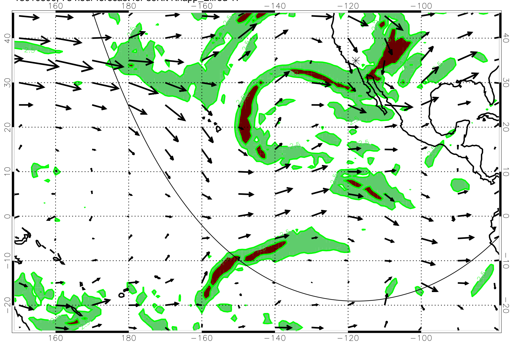
13010806, 78 hour forecast for 39Kft Knapp_Ellrod T1
