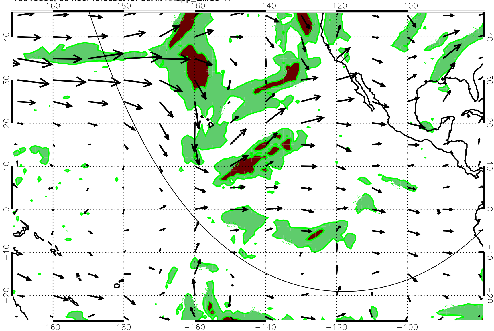
13010606, 30 hour forecast for 39Kft Knapp_Ellrod T1
