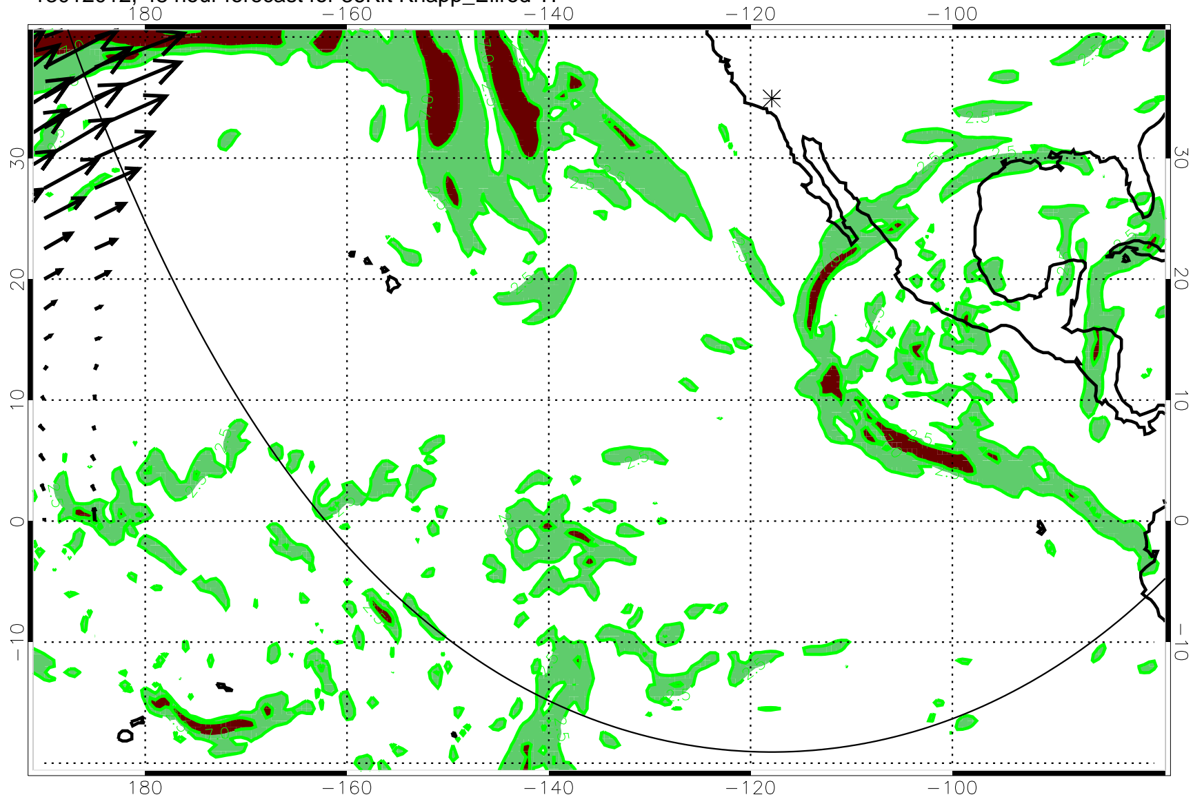
13012012, 48 hour forecast for 36Kft Knapp_Ellrod TI
