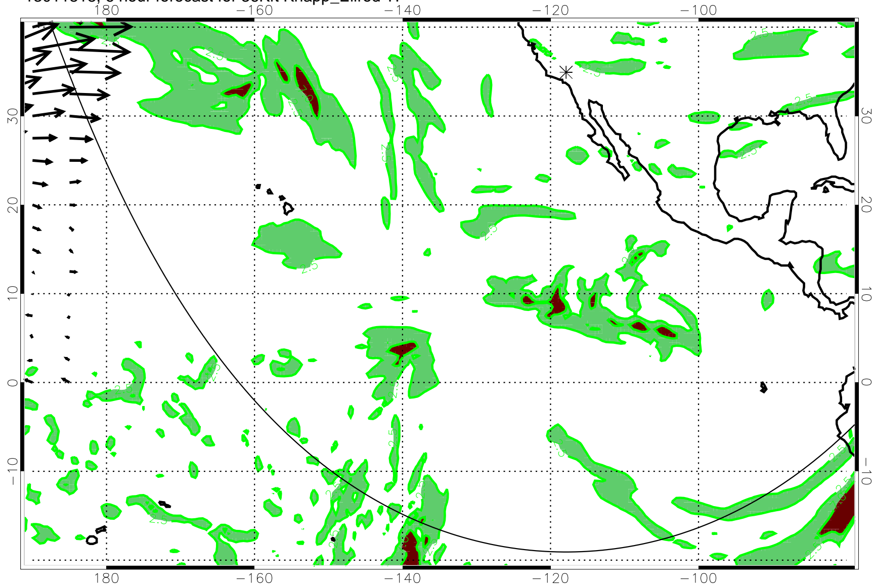
13011818, 6 hour forecast for 36Kft Knapp_Ellrod TI
