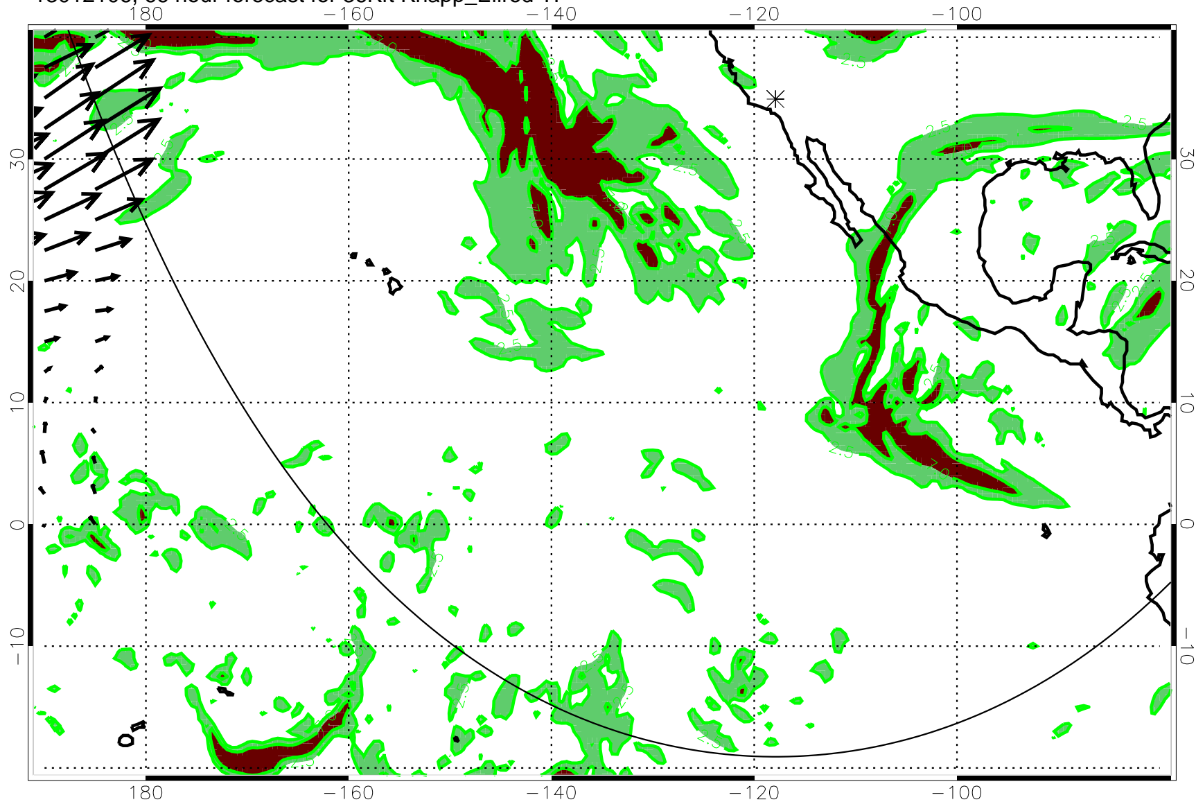
13012106, 66 hour forecast for 36Kft Knapp_Ellrod TI
