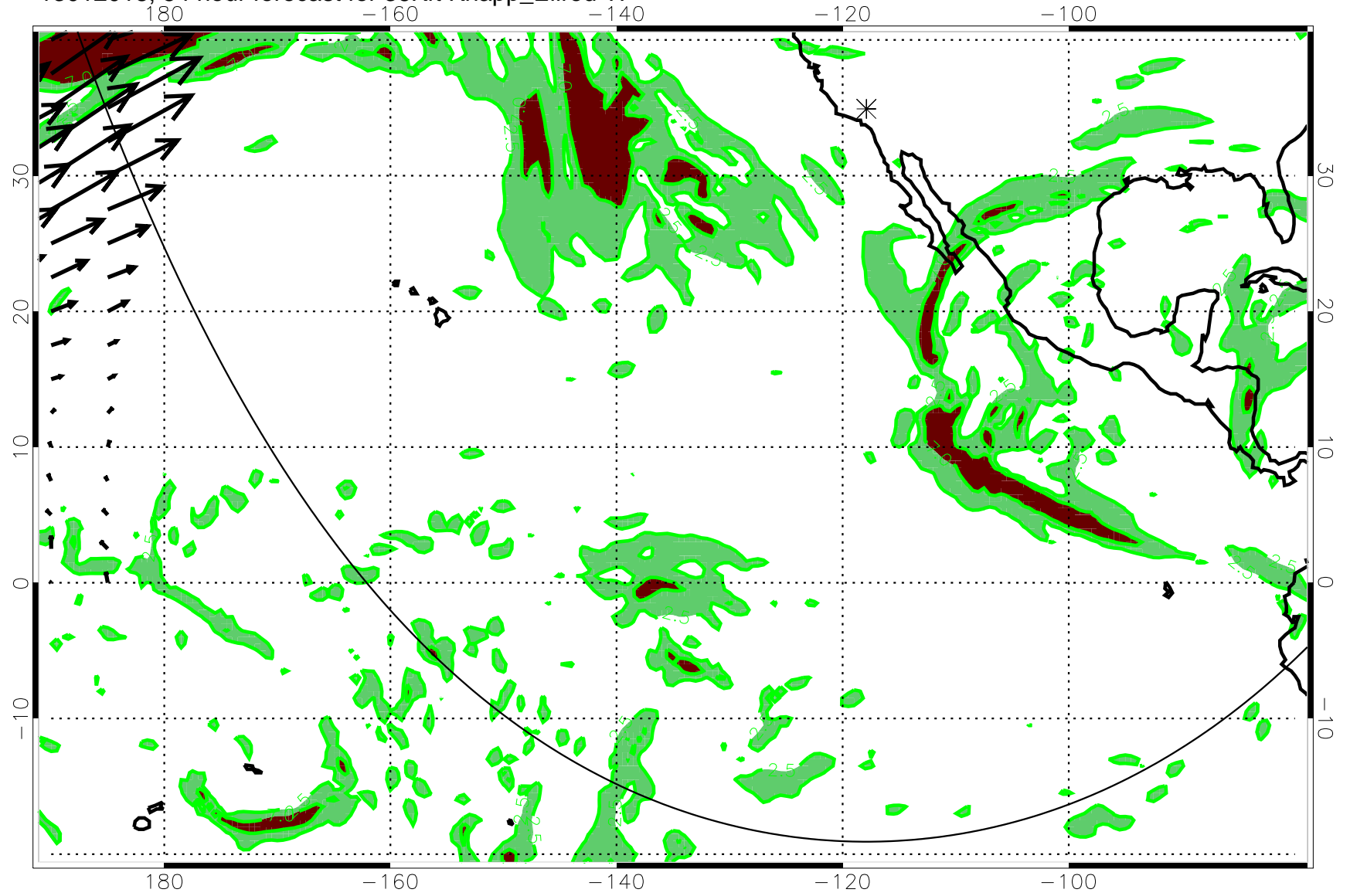
13012018, 54 hour forecast for 36Kft Knapp_Ellrod TI
