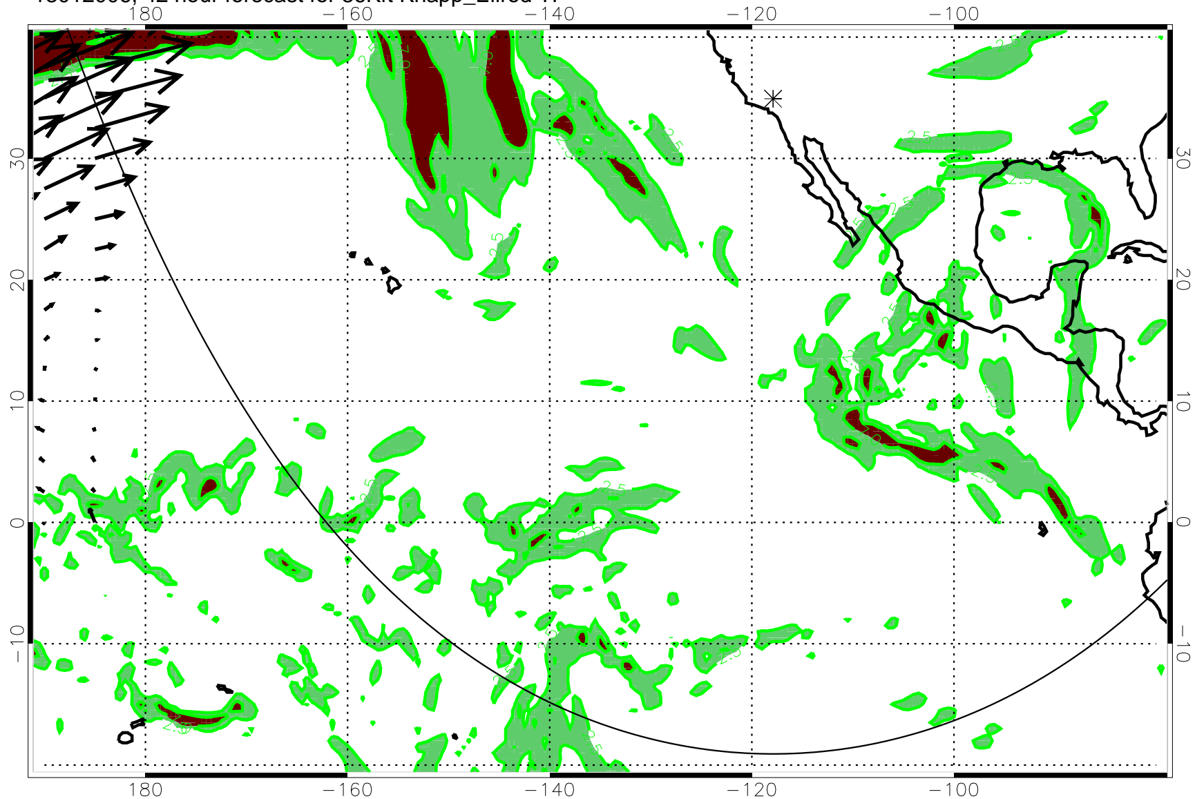
13012006, 42 hour forecast for 36Kft Knapp_Ellrod TI
