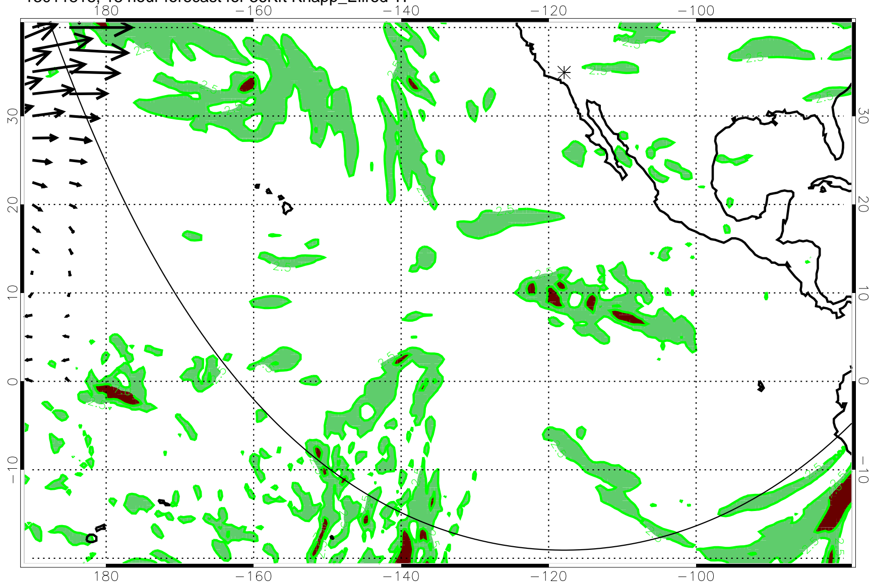
13011818, 18 hour forecast for 36Kft Knapp_Ellrod TI
