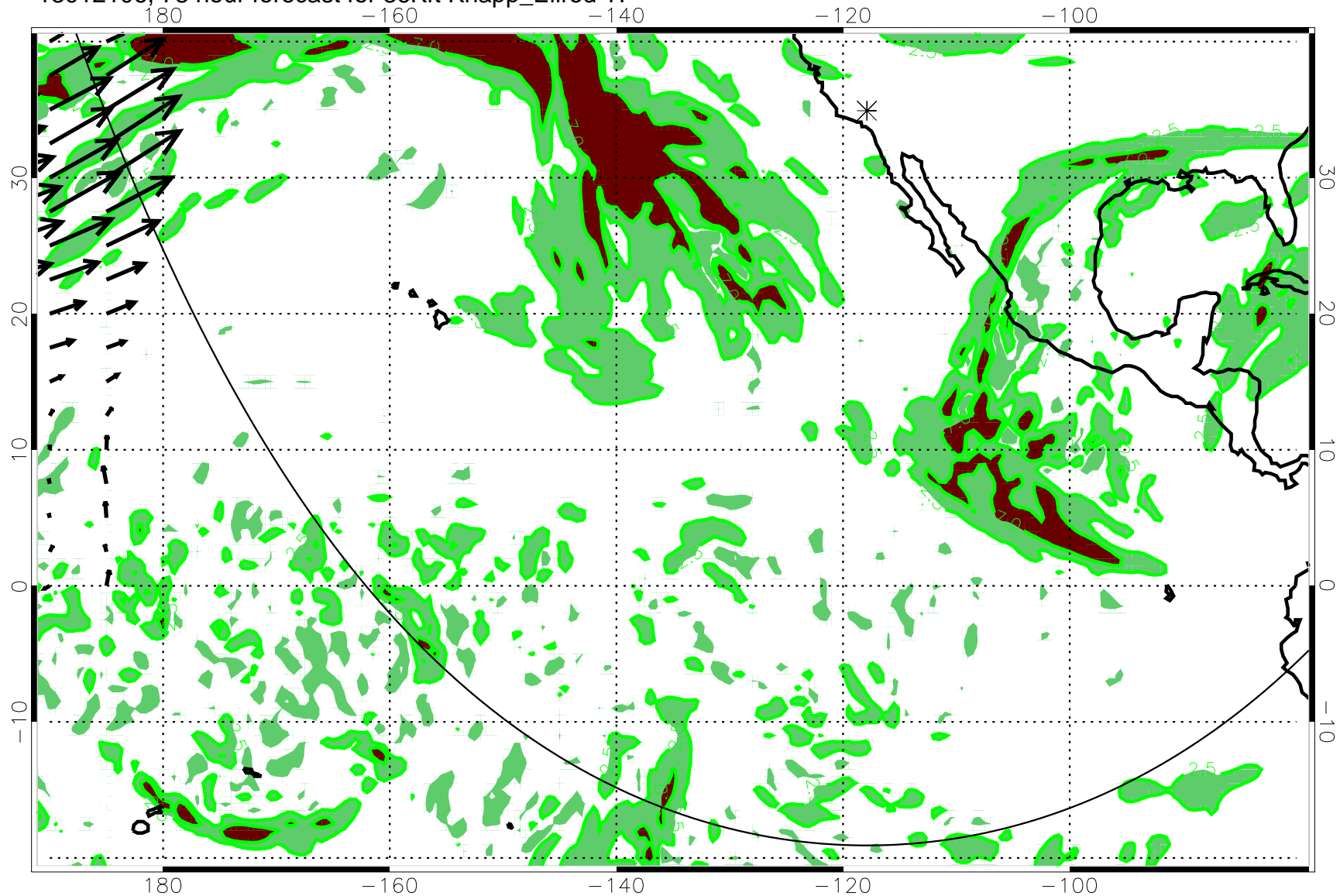
13012106, 78 hour forecast for 36Kft Knapp_Ellrod TI
