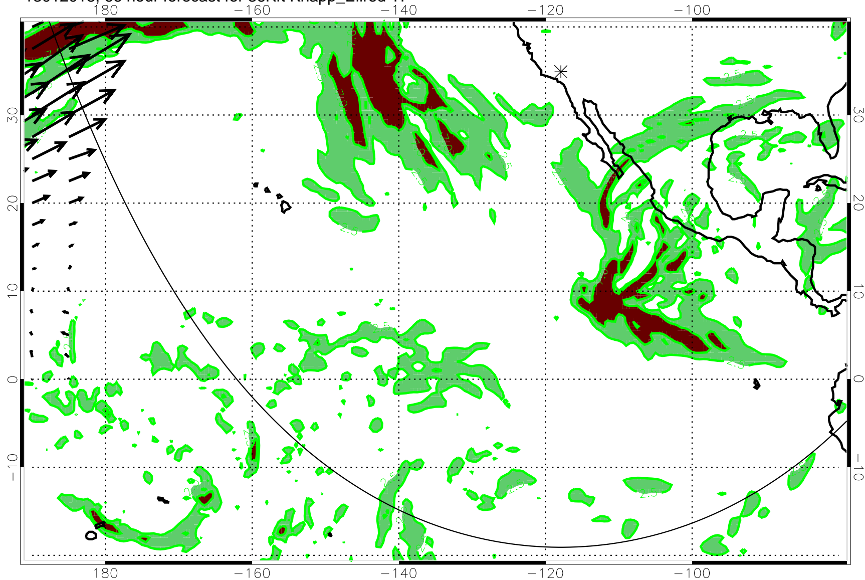
13012018, 66 hour forecast for 36Kft Knapp_Ellrod TI
