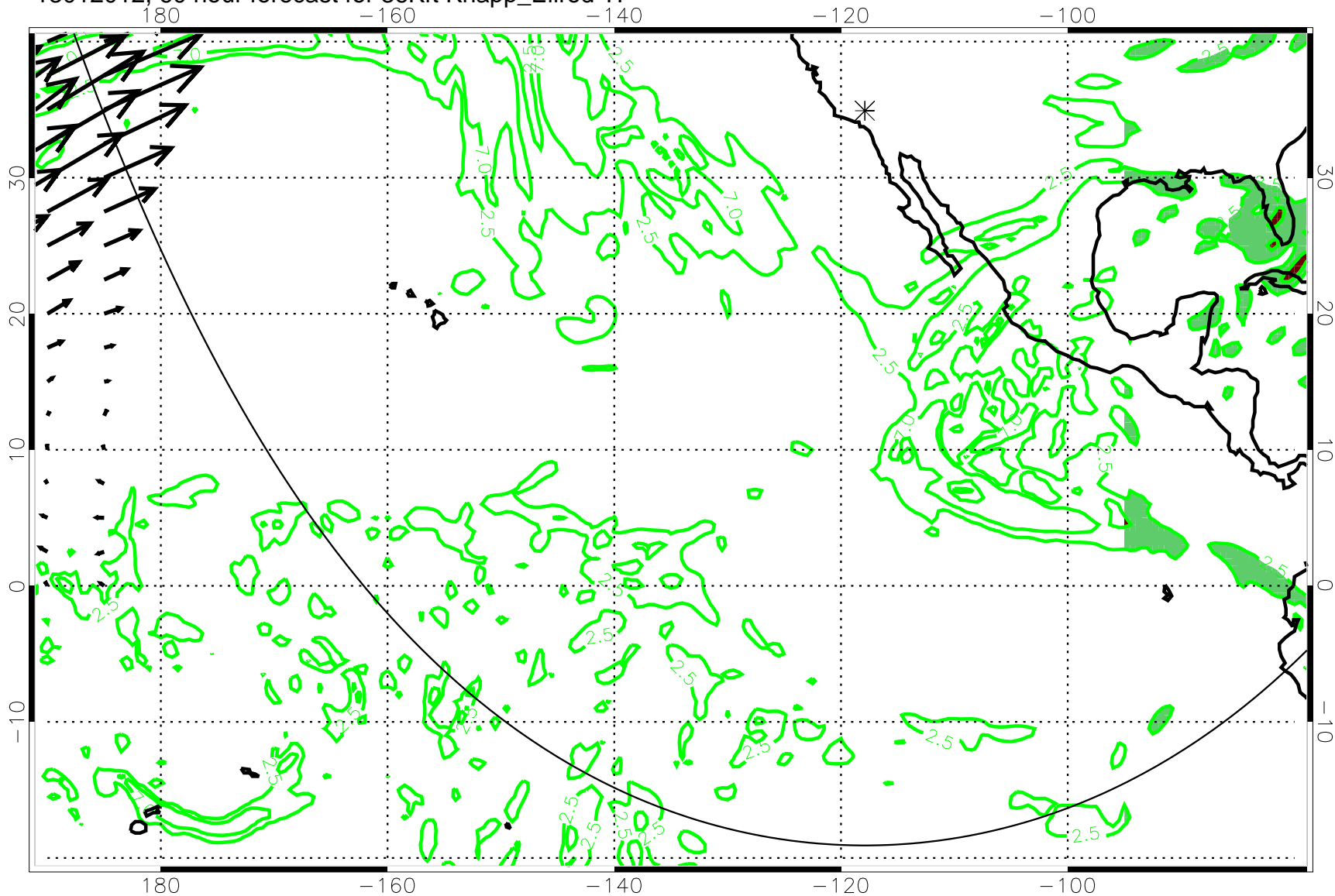
13012012, 60 hour forecast for 36Kft Knapp_Ellrod TI
