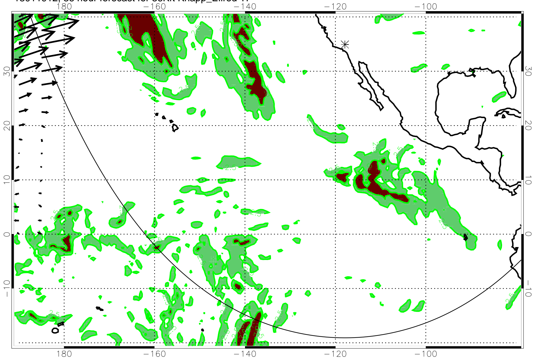
13011912, 36 hour forecast for 36Kft Knapp_Ellrod TI
