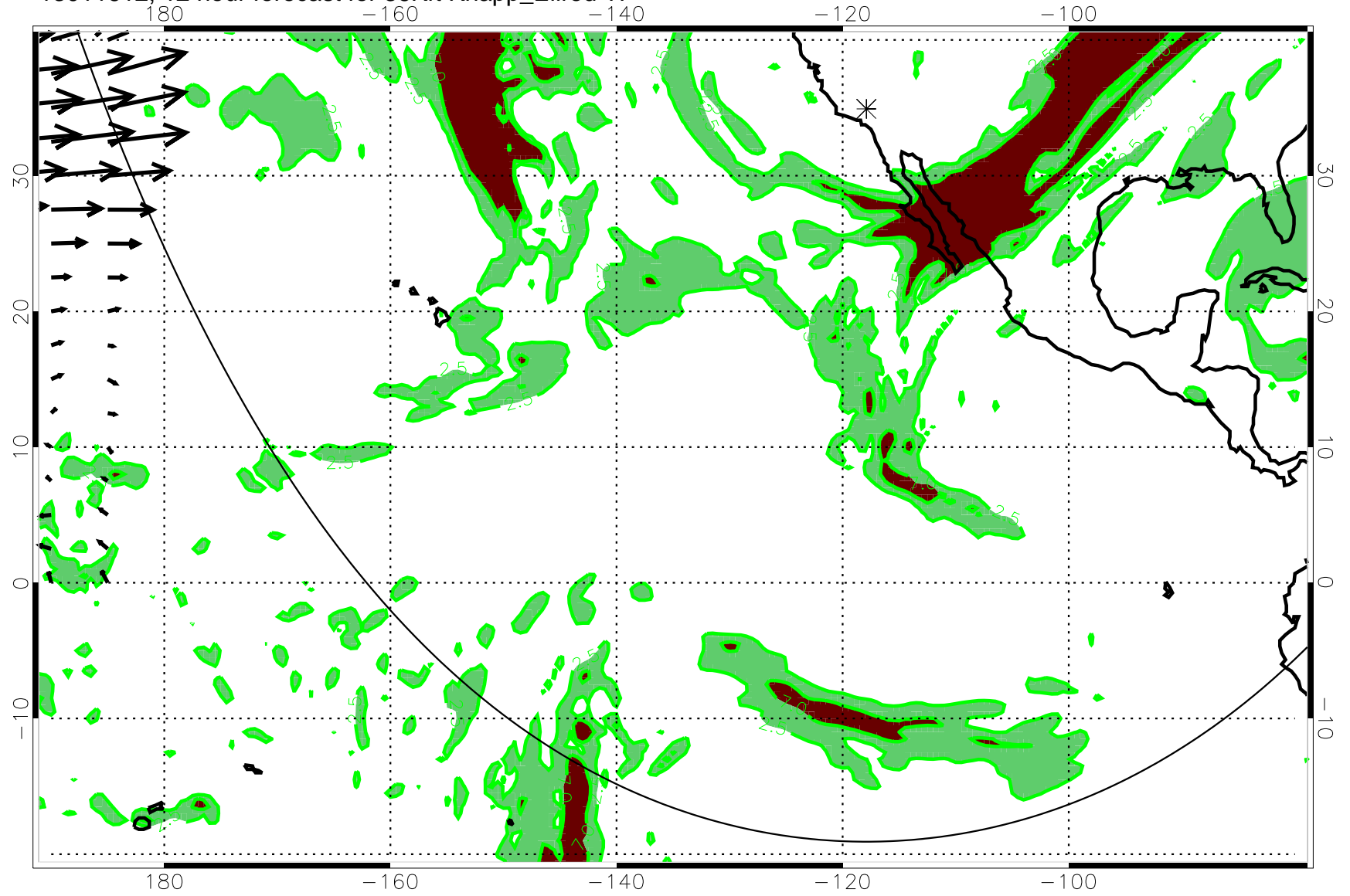
13011612, 12 hour forecast for 36Kft Knapp_Ellrod TI
