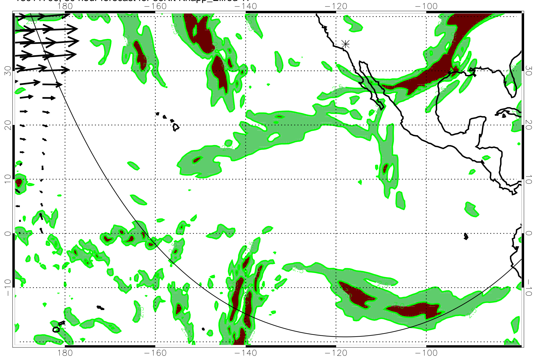
13011706, 30 hour forecast for 36Kft Knapp_Ellrod TI
