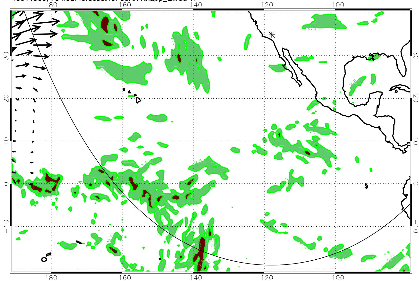
13011906, 78 hour forecast for 36Kft Knapp_Ellrod TI
