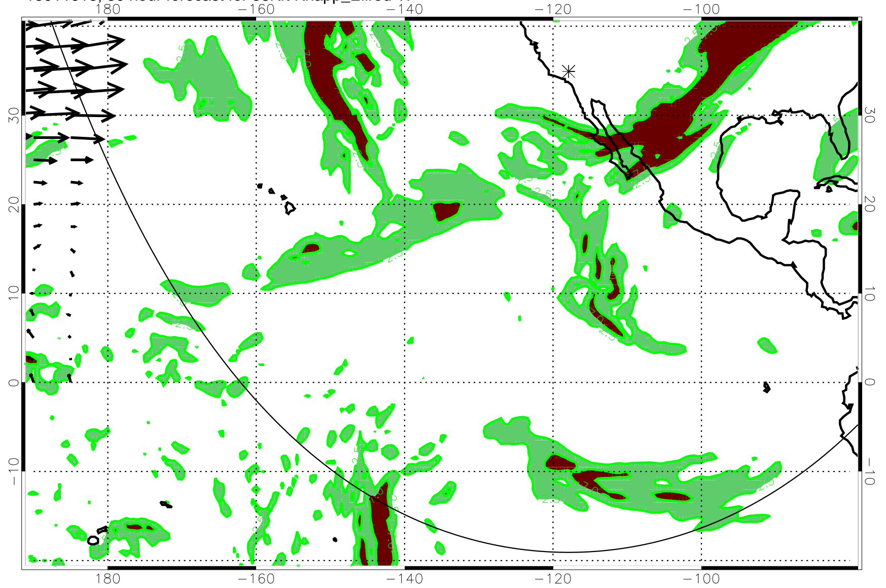
13011618, 30 hour forecast for 36Kft Knapp_Ellrod TI
