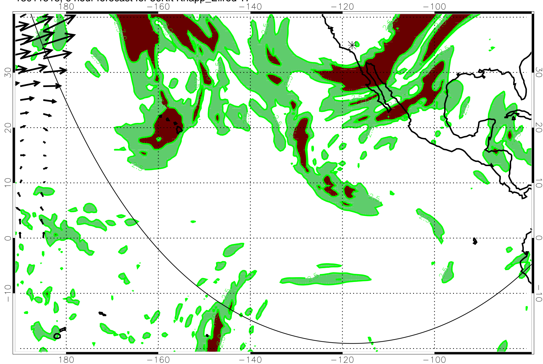
13011518, 6 hour forecast for 36Kft Knapp_Ellrod TI
