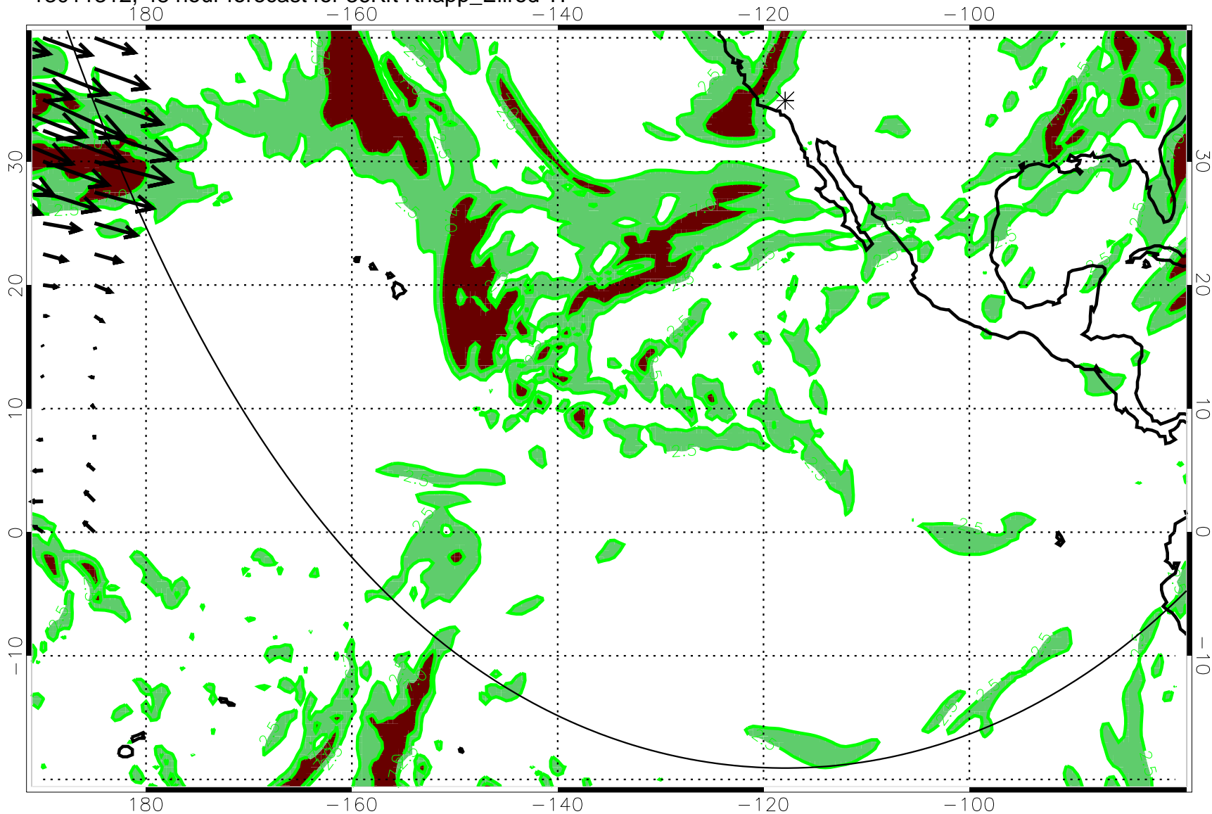
13011312, 48 hour forecast for 36Kft Knapp_Ellrod TI
