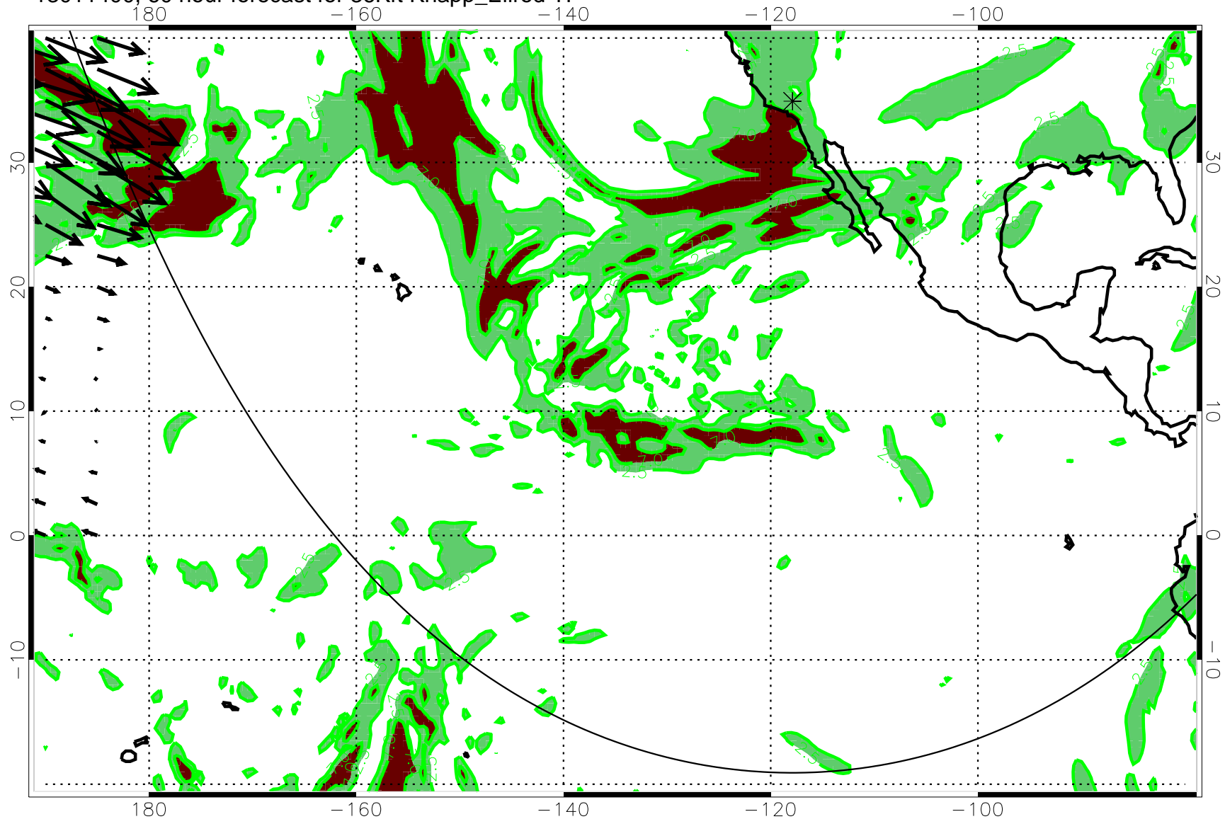
13011400, 60 hour forecast for 36Kft Knapp_Ellrod TI
