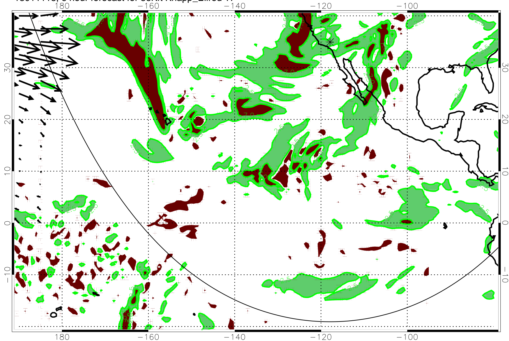
13011118, 6 hour forecast for 36Kft Knapp_Ellrod TI
