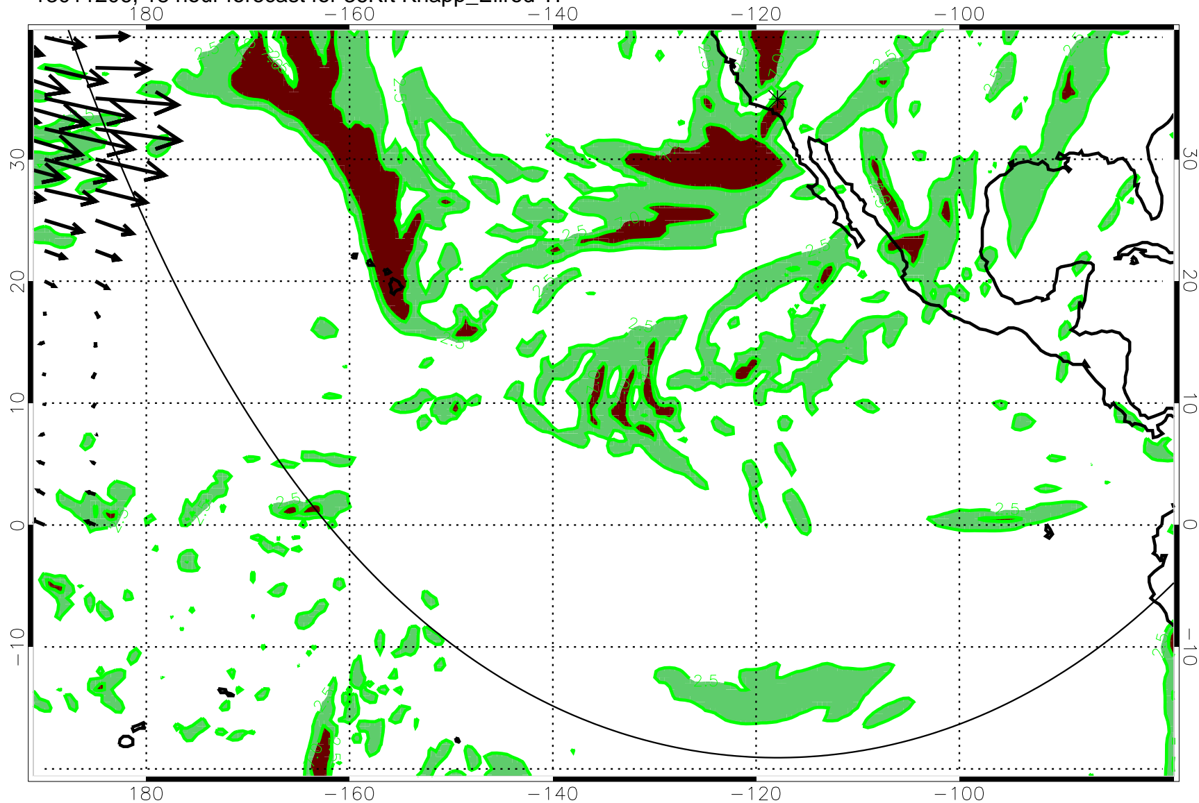
13011206, 18 hour forecast for 36Kft Knapp_Ellrod TI
