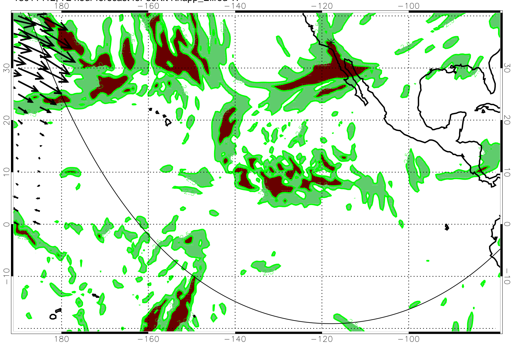
13011412, 72 hour forecast for 36Kft Knapp_Ellrod TI
