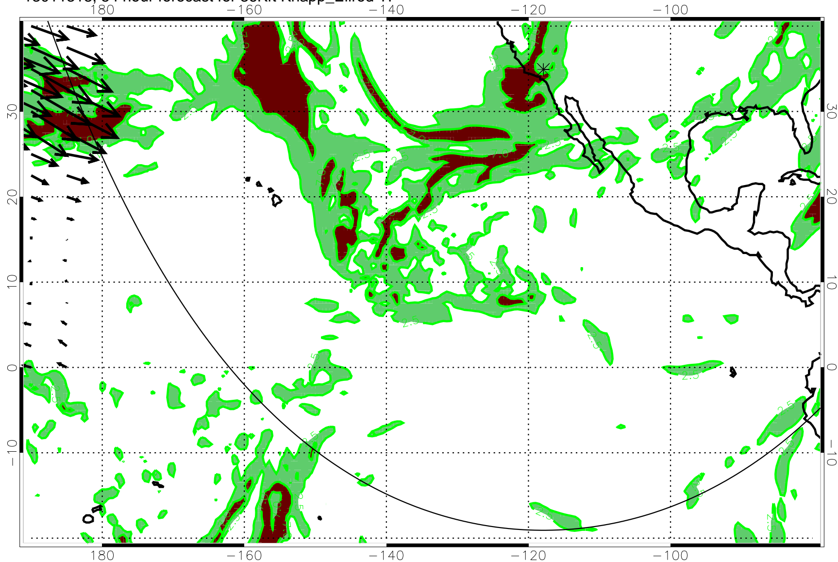
13011318, 54 hour forecast for 36Kft Knapp_Ellrod TI
