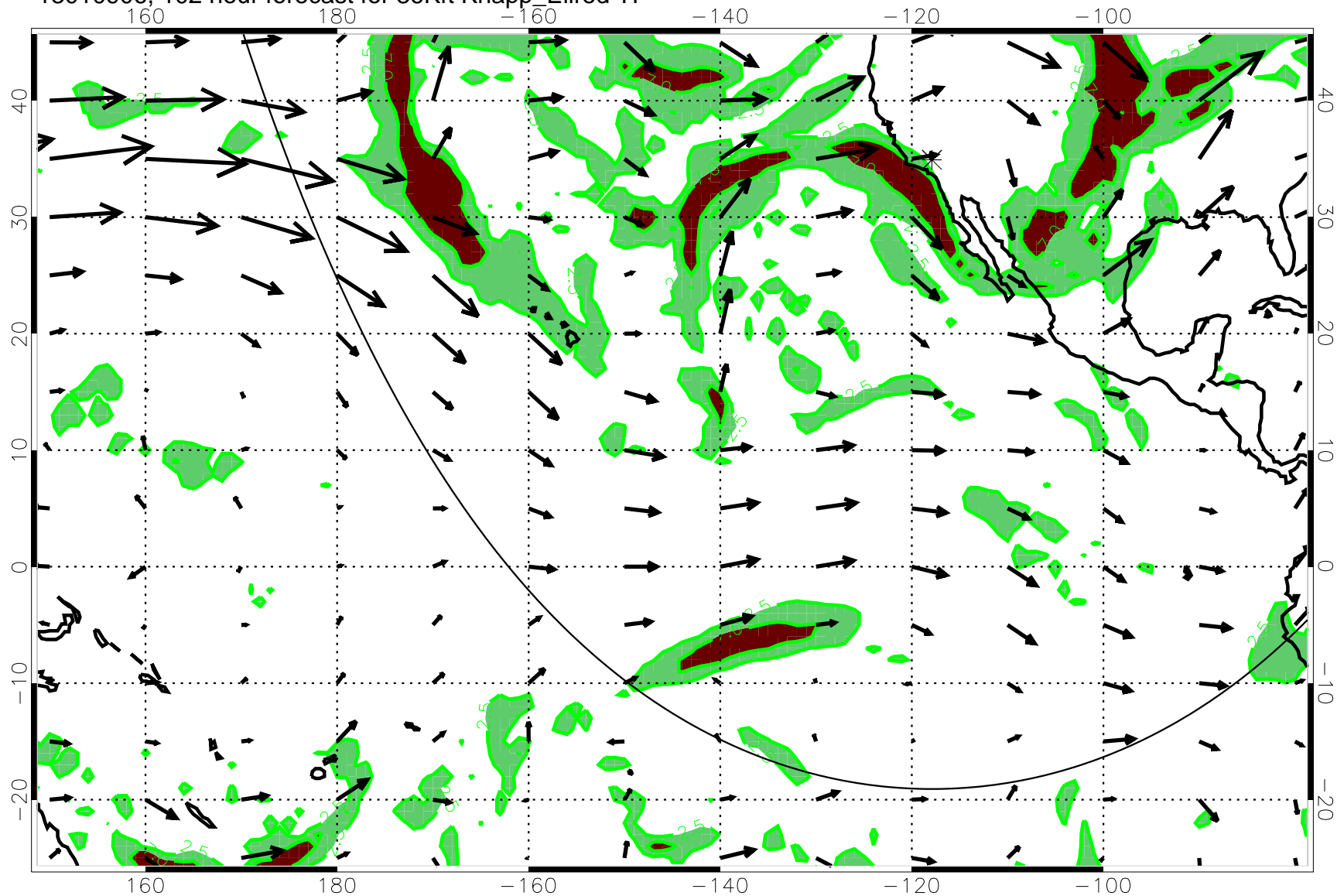
13010906, 102 hour forecast for 36Kft Knapp_Ellrod T1
