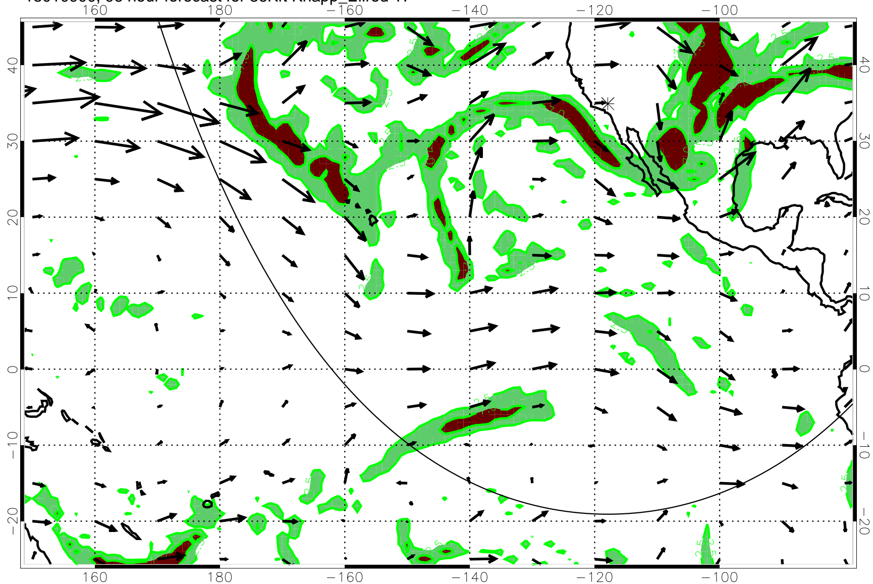
13010900, 96 hour forecast for 36Kft Knapp_Ellrod T1
