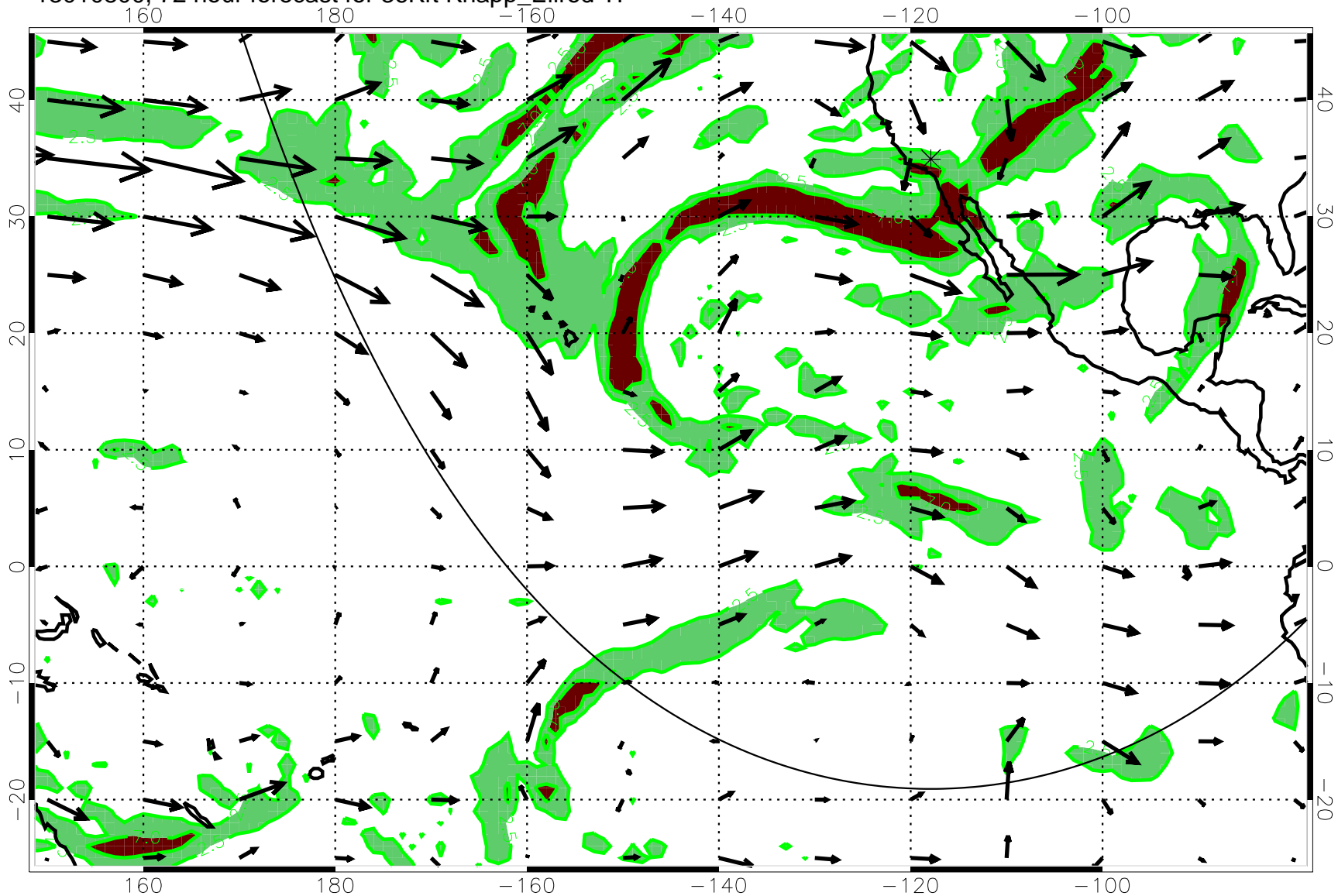
13010800, 72 hour forecast for 36Kft Knapp_Ellrod T1
