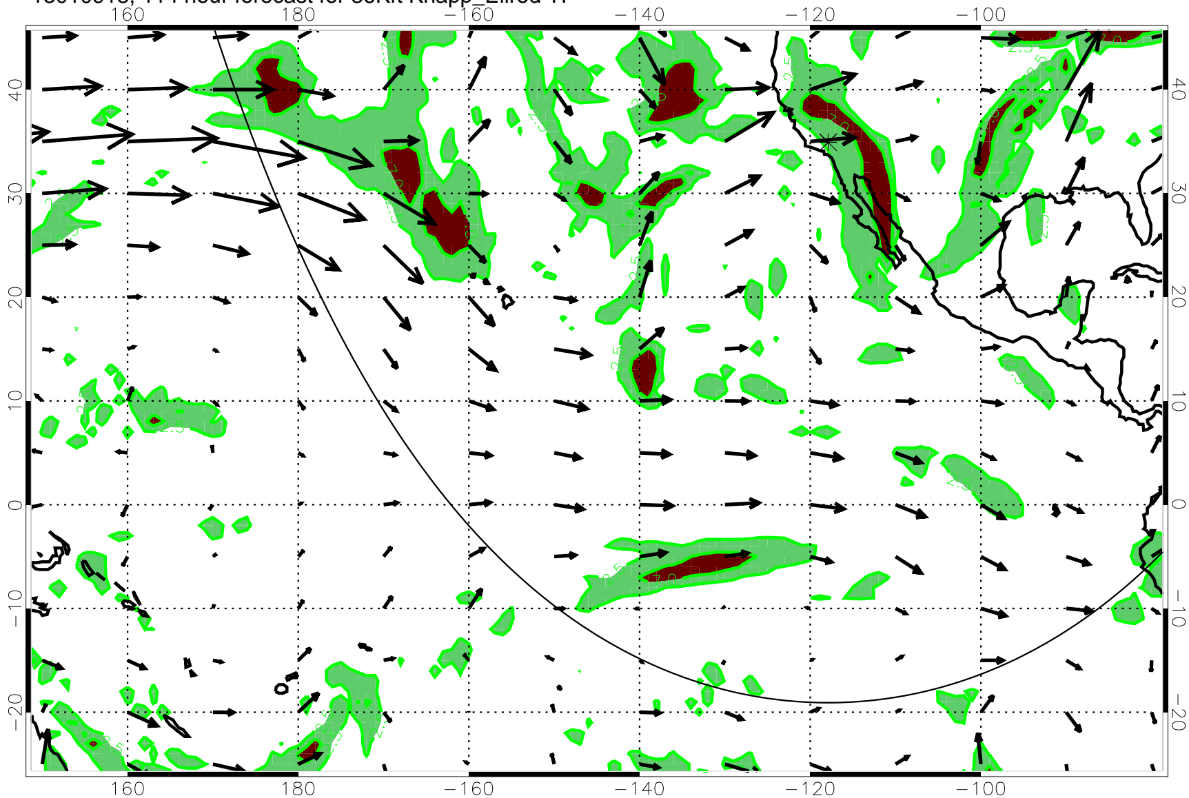
13010918, 114 hour forecast for 36Kft Knapp_Ellrod T1
