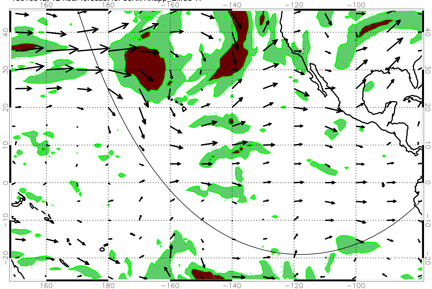
13010512, 12 hour forecast for 36Kft Knapp_Ellrod T1
