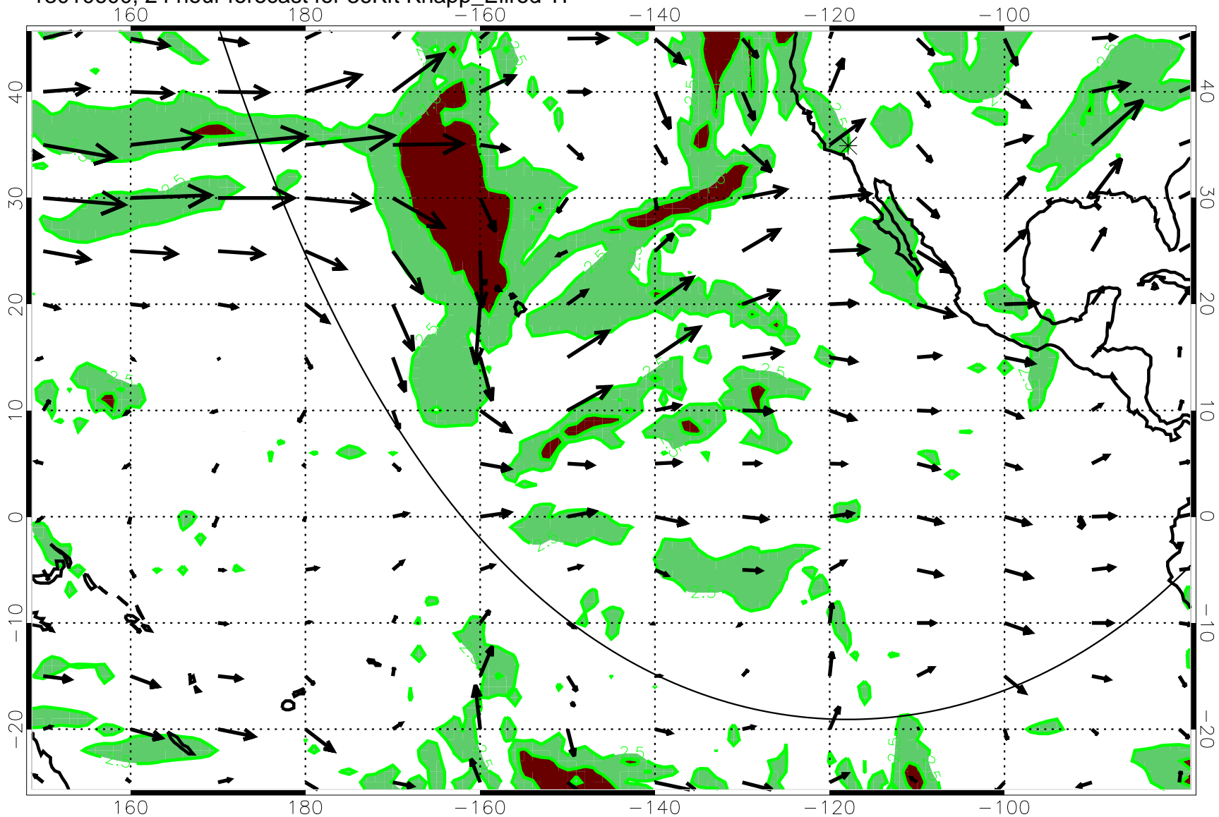
13010600, 24 hour forecast for 36Kft Knapp_Ellrod T1
