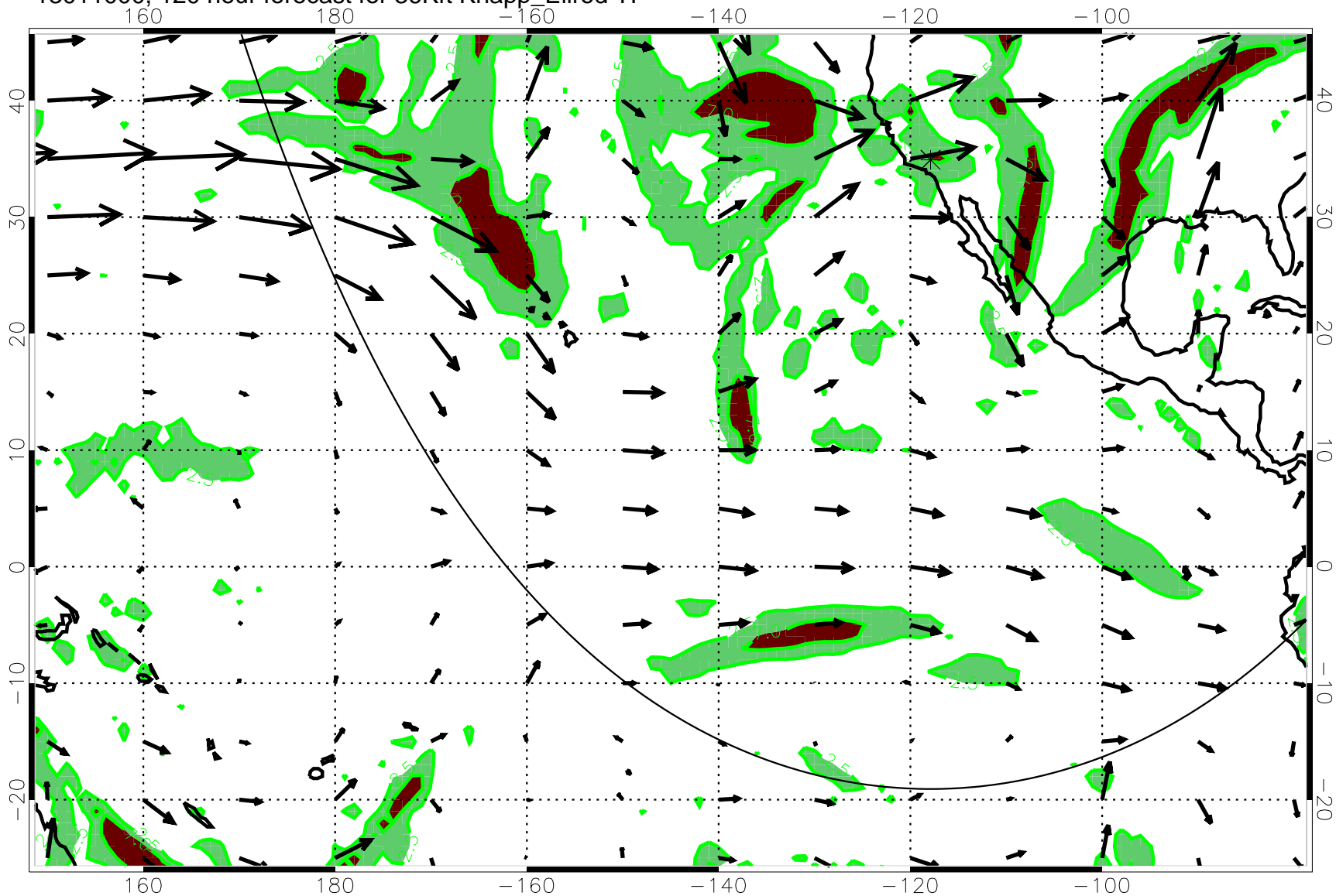
13011000, 120 hour forecast for 36Kft Knapp_Ellrod T1
