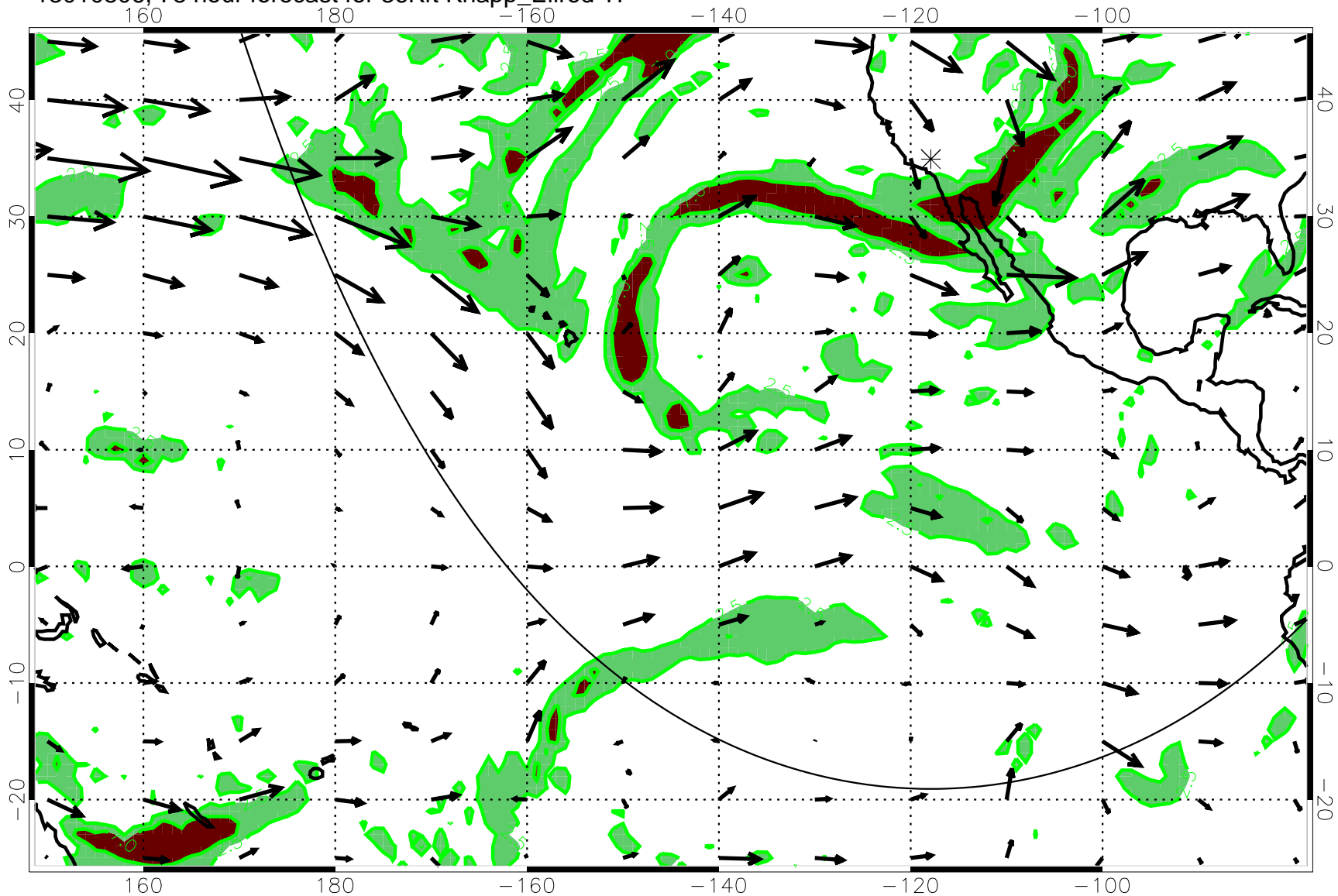
13010806, 78 hour forecast for 36Kft Knapp_Ellrod TI
