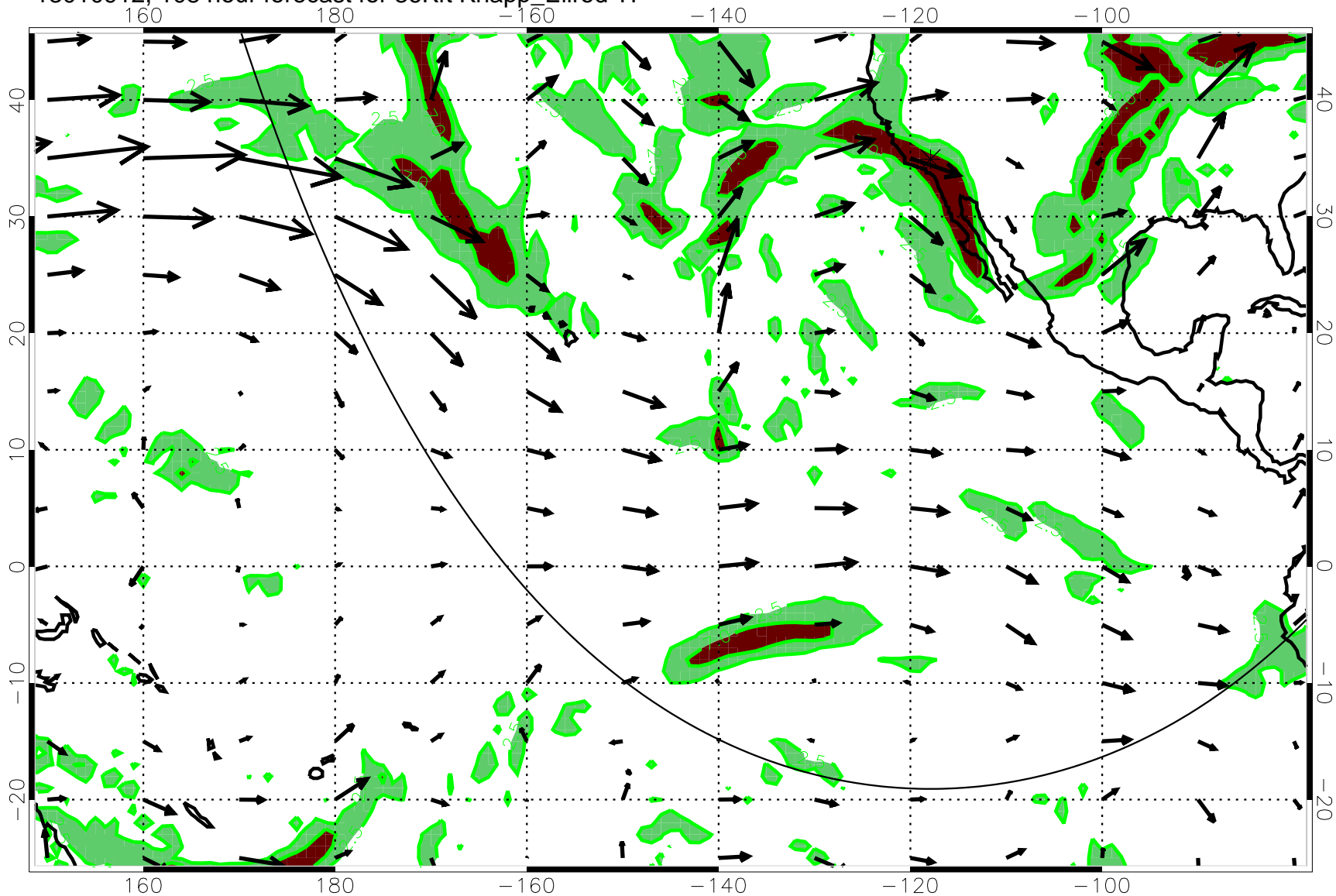
13010912, 108 hour forecast for 36Kft Knapp_Ellrod T1
