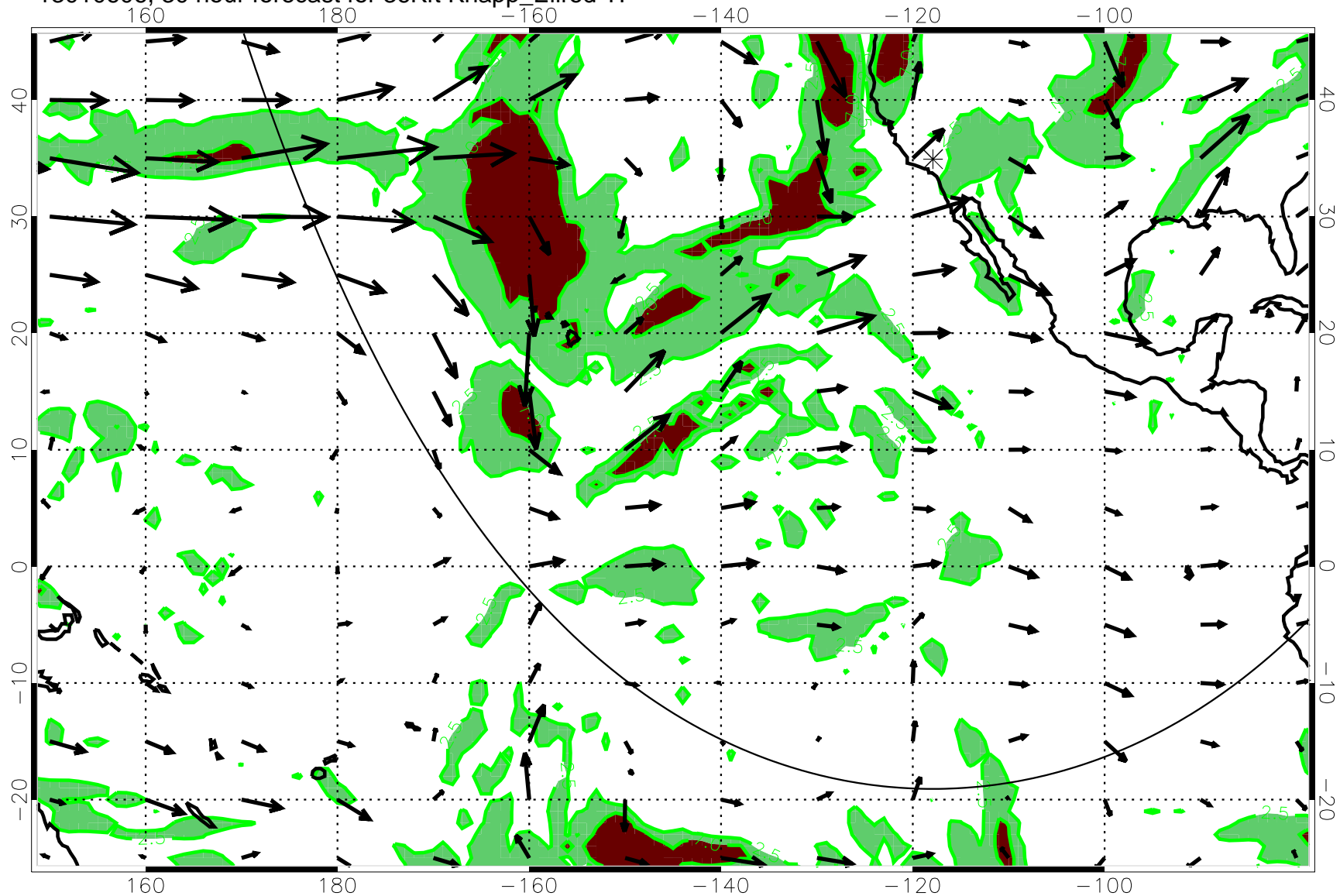
13010606, 30 hour forecast for 36Kft Knapp_Ellrod T1
