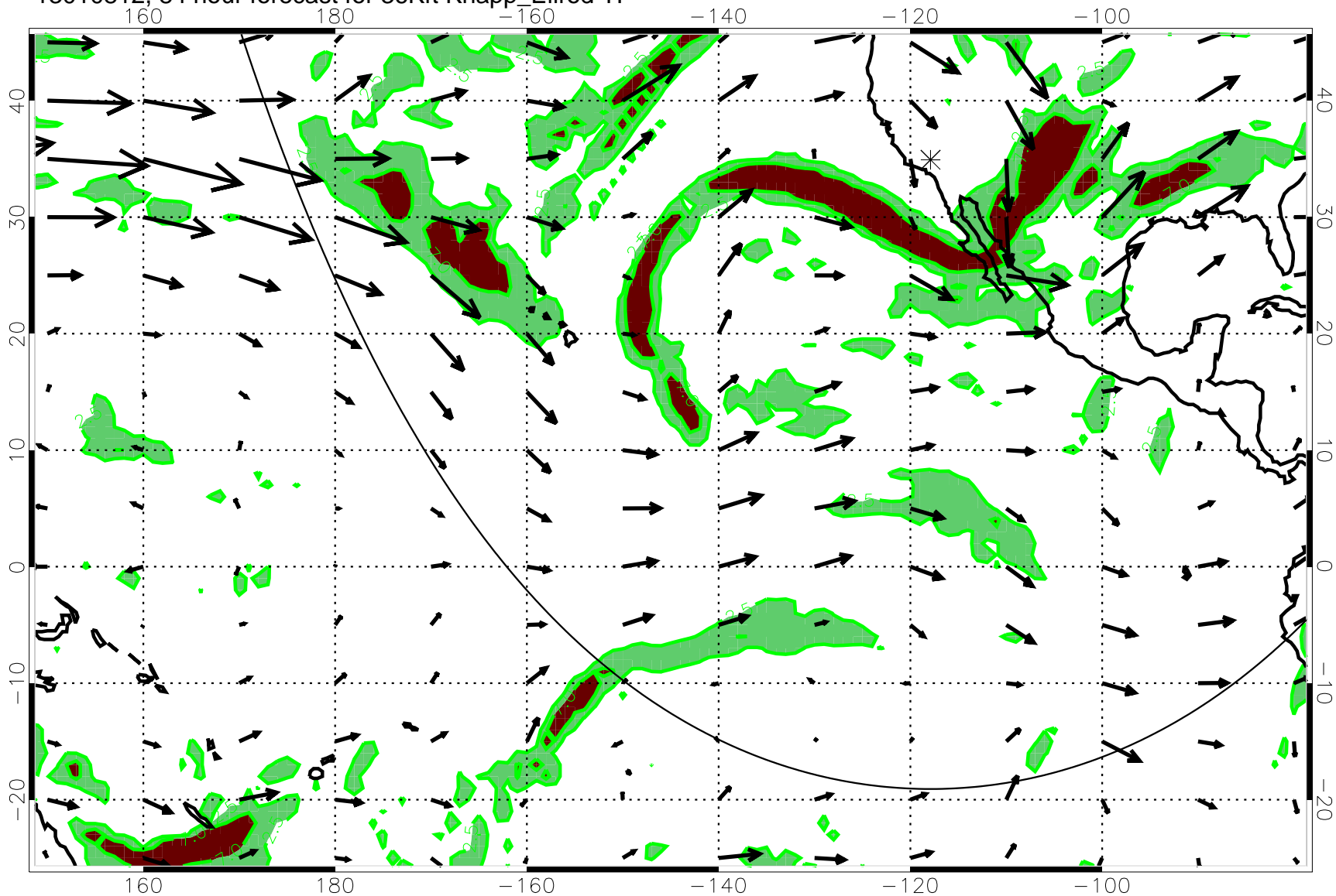
13010812, 84 hour forecast for 36Kft Knapp_Ellrod T1
