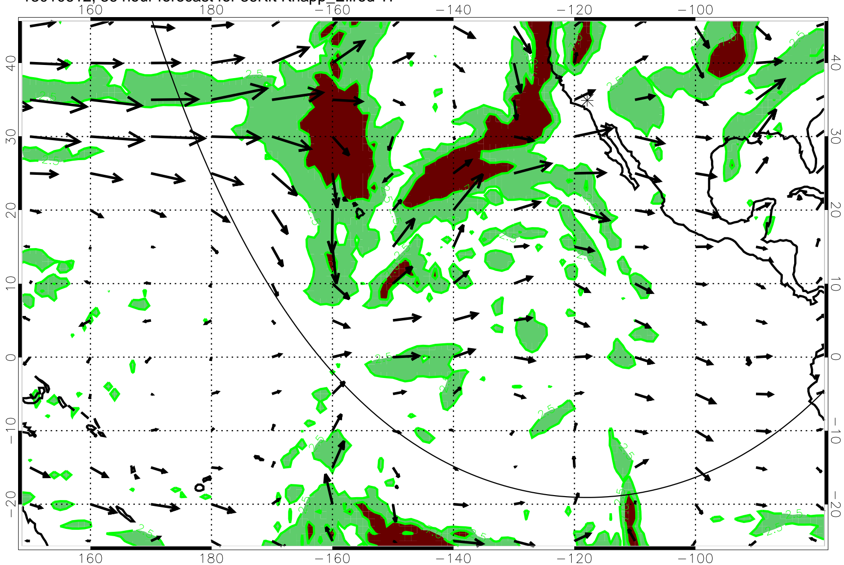
13010612, 36 hour forecast for 36Kft Knapp_Ellrod TI
