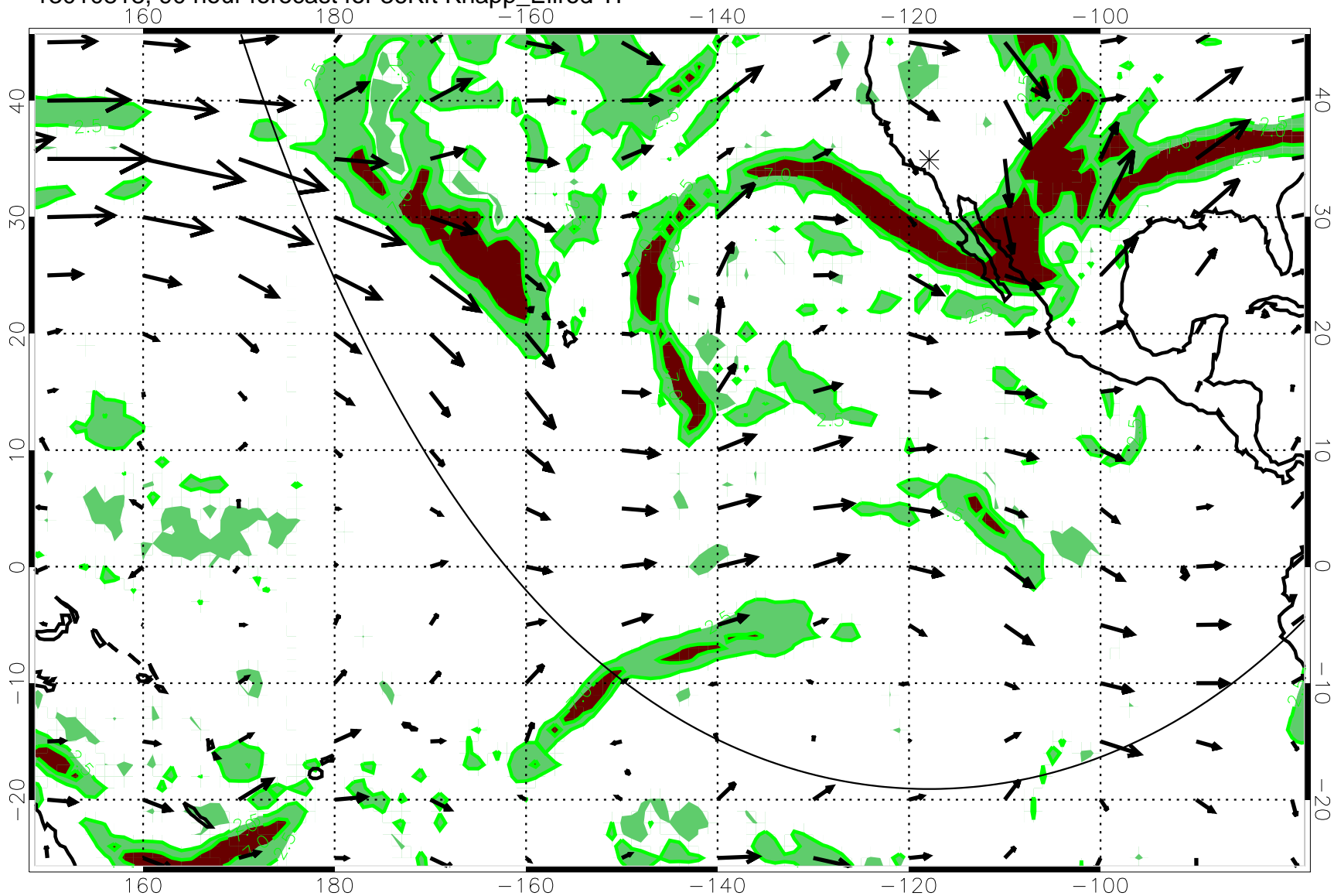
13010818, 90 hour forecast for 36Kft Knapp_Ellrod T1
