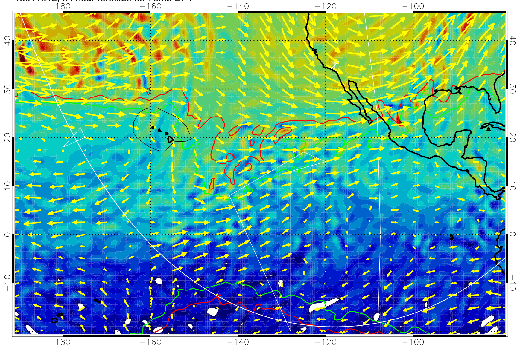
13011312, 84 hour forecast for 70mb EPV
