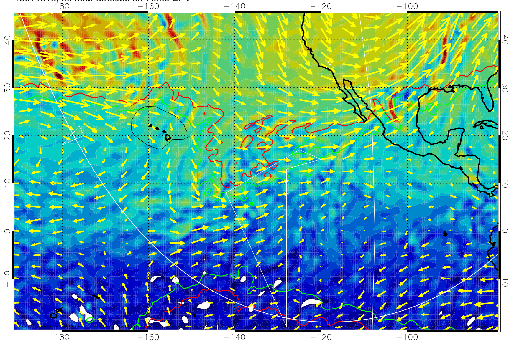
13011318, 90 hour forecast for 70mb EPV
