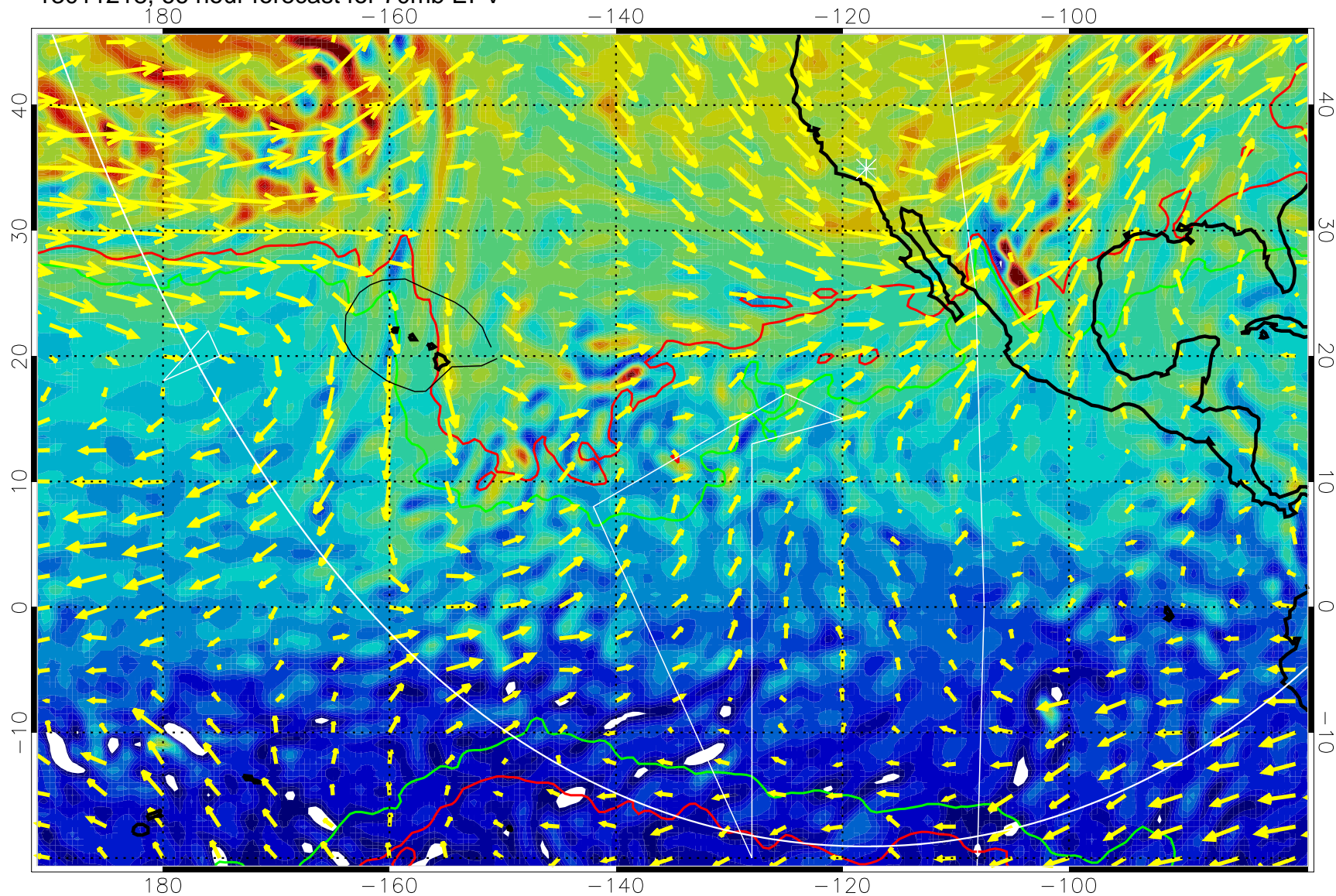
13011218, 66 hour forecast for 70mb EPV
