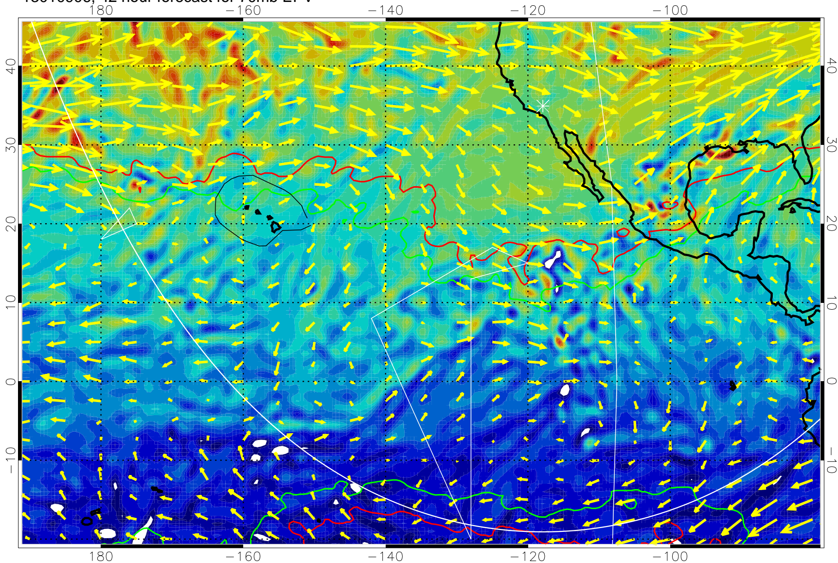
13010906, 42 hour forecast for 70mb EPV
