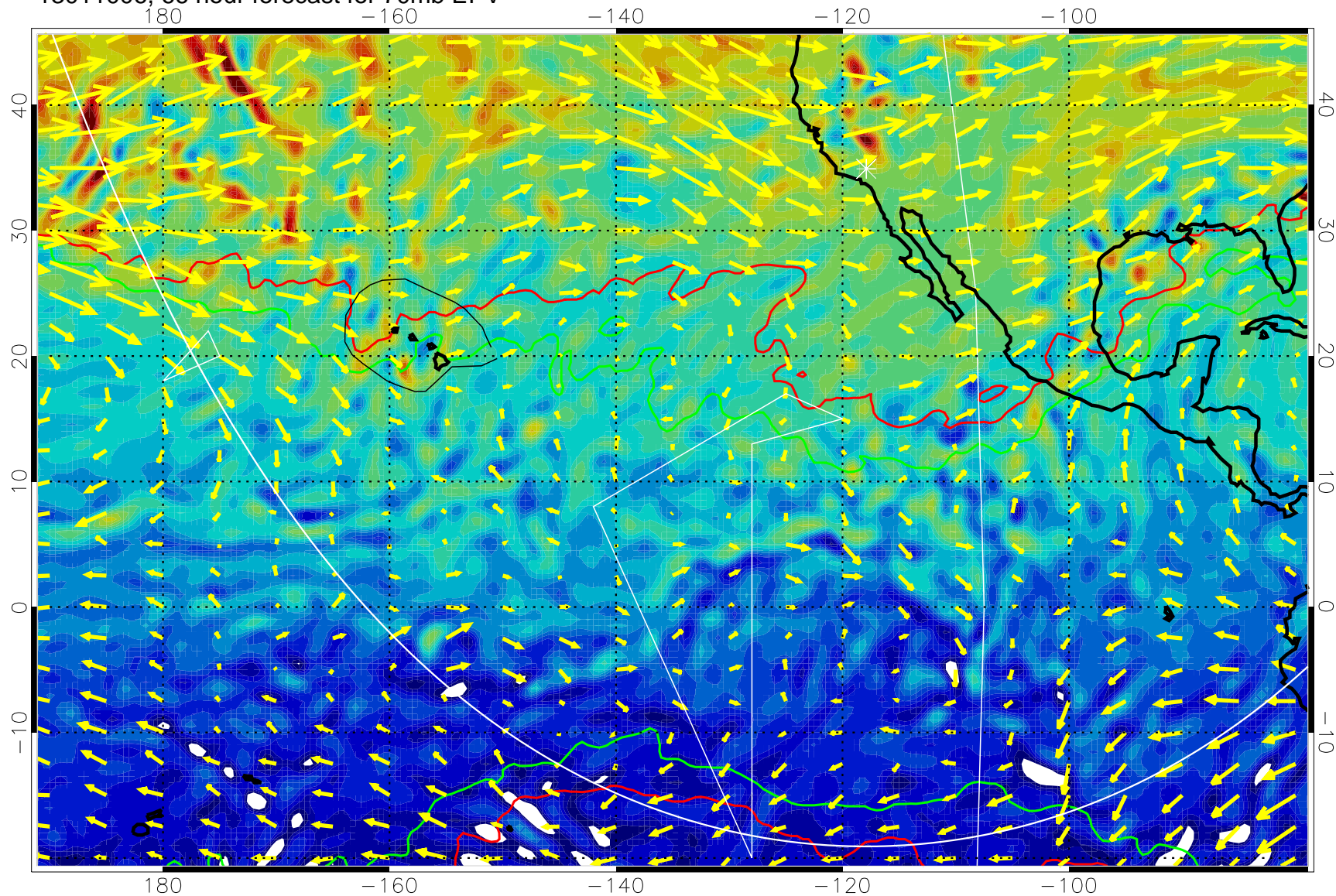
13011006, 66 hour forecast for 70mb EPV
