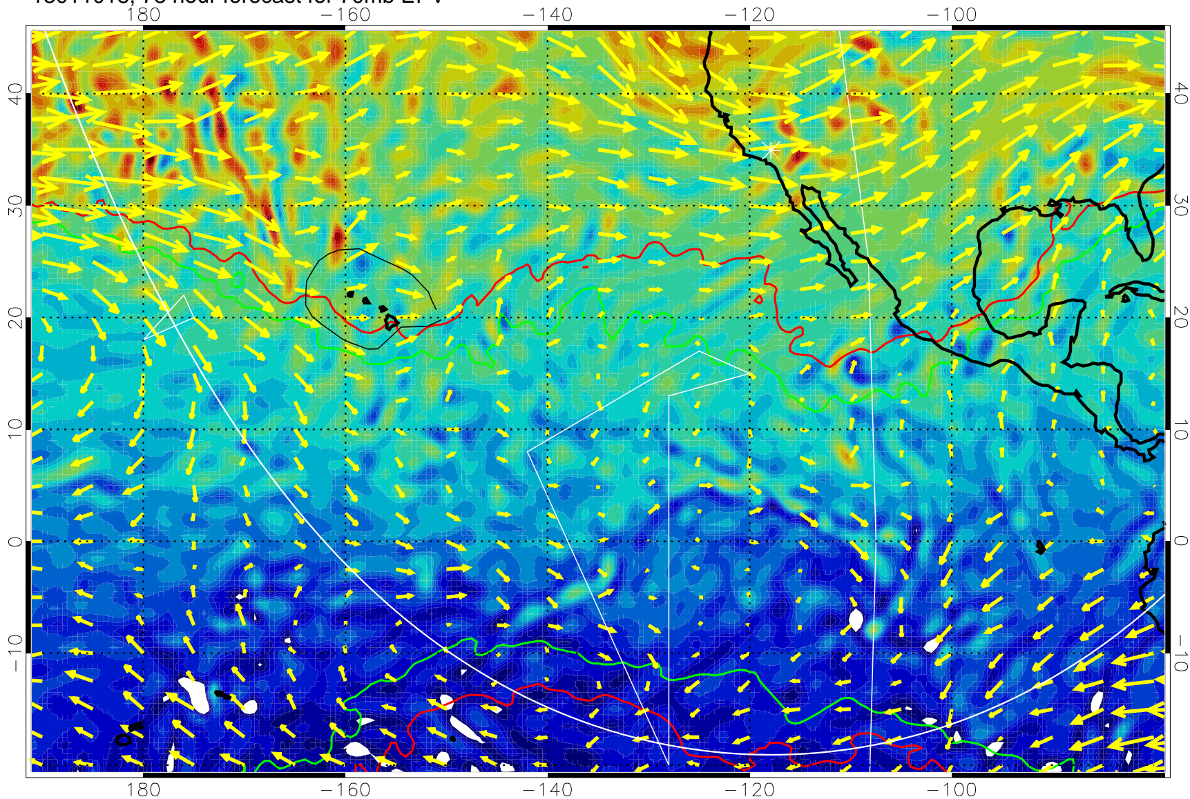
13011018, 78 hour forecast for 70mb EPV
