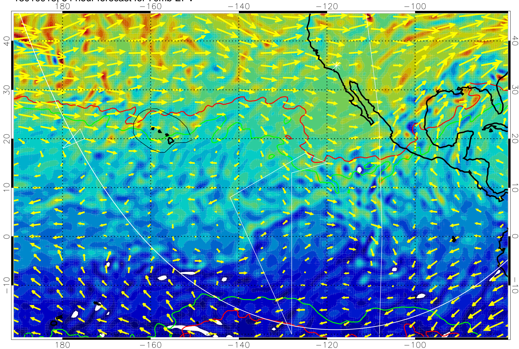
13010918, 54 hour forecast for 70mb EPV
