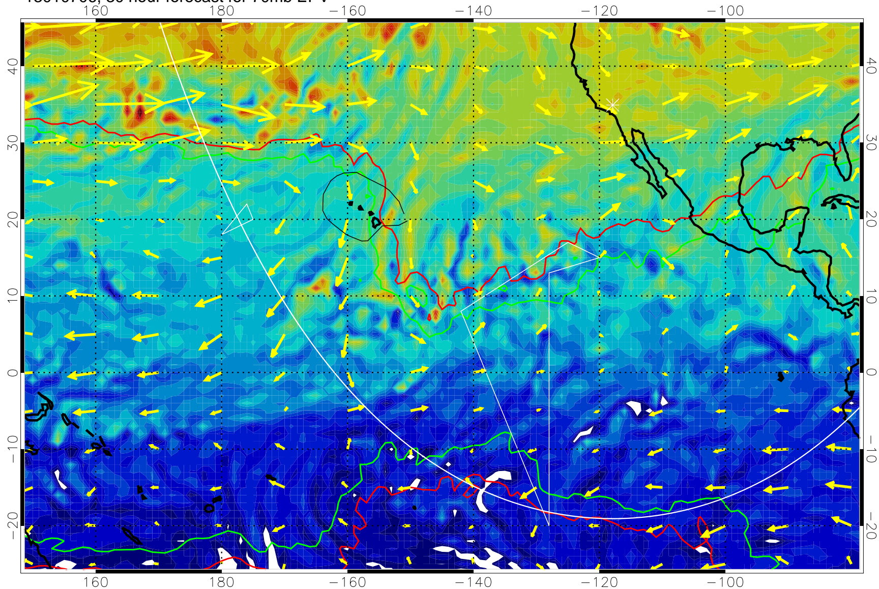
13010706, 30 hour forecast for 70mb EPV
