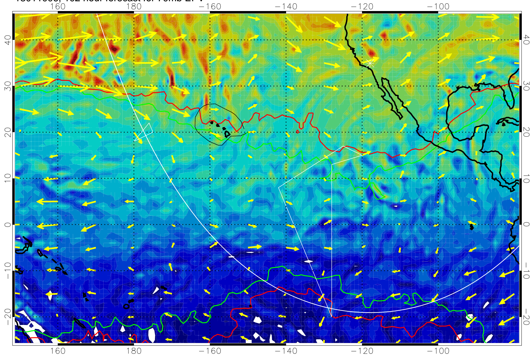
13011006, 102 hour forecast for 70mb EPV
