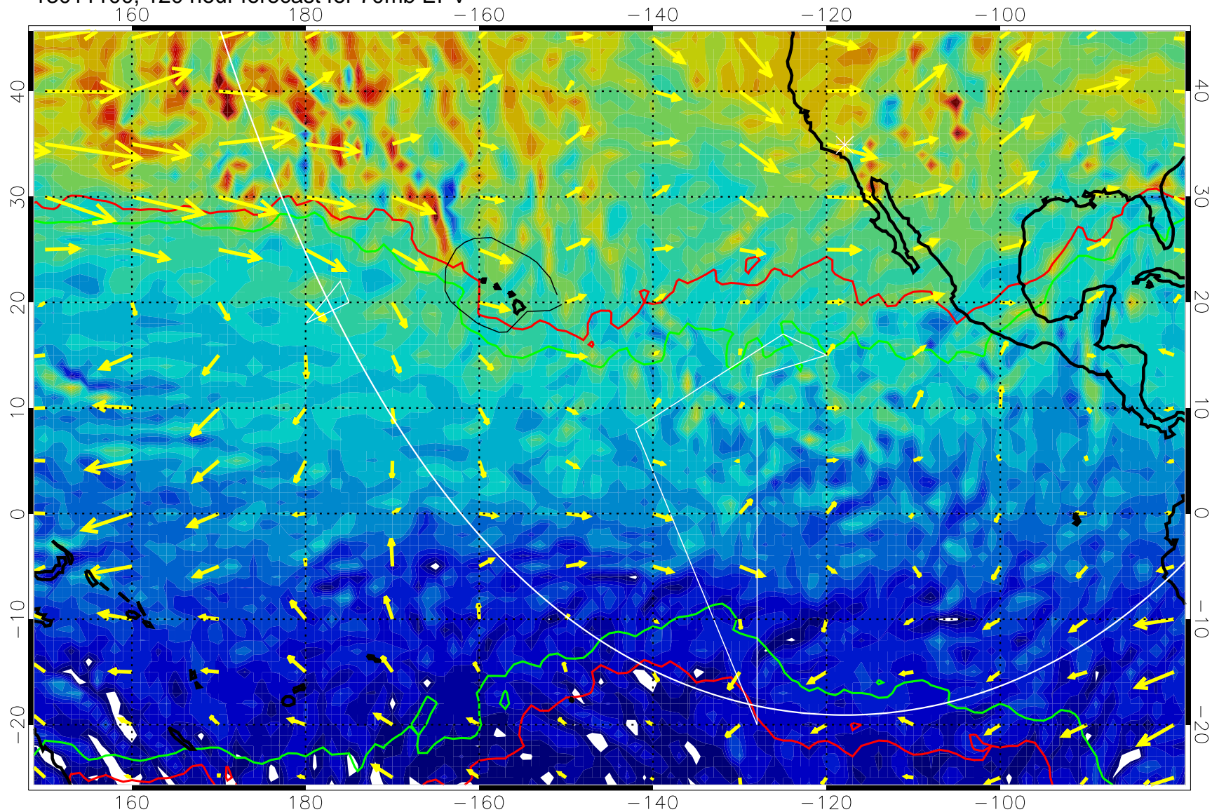
13011100, 120 hour forecast for 70mb EPV
