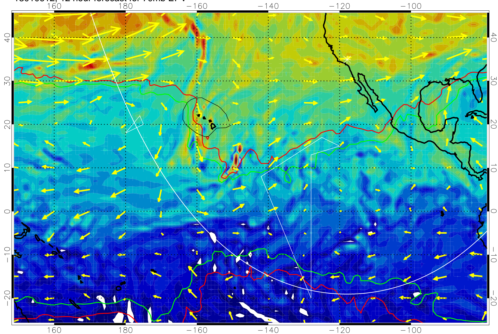
13010612, 12 hour forecast for 70mb EPV
