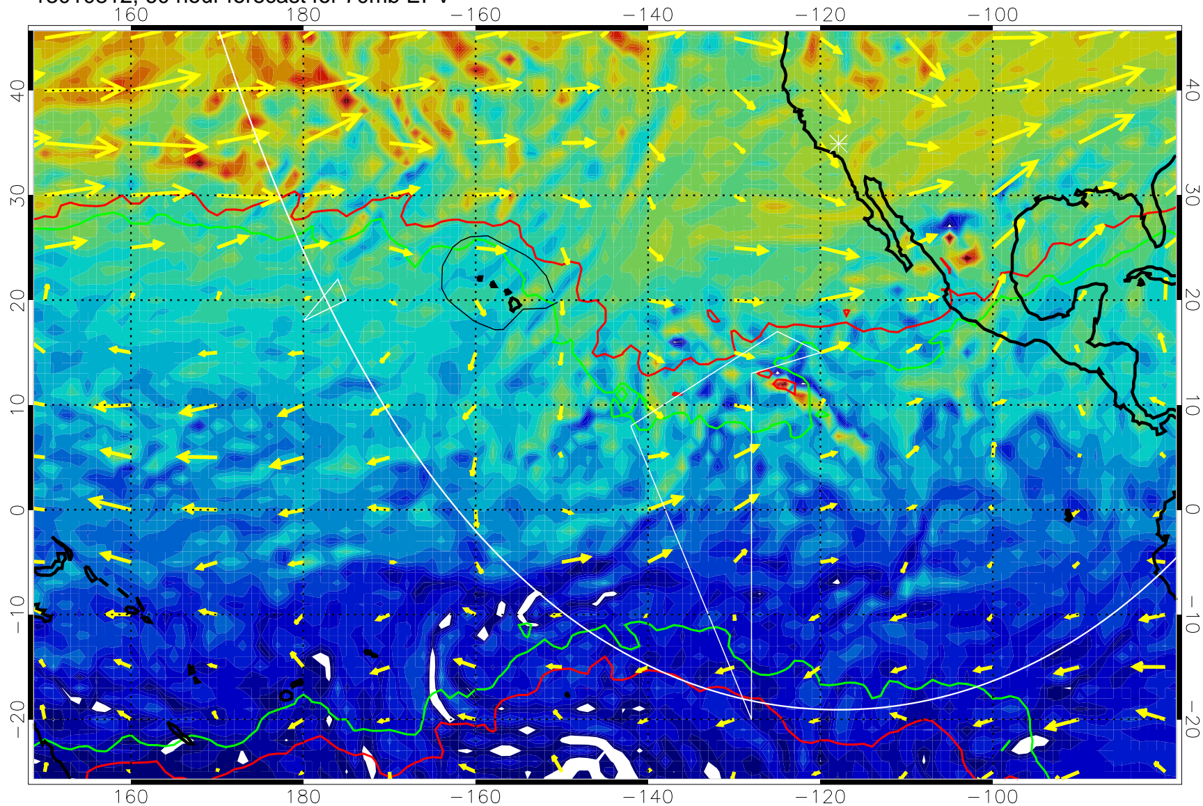
13010812, 60 hour forecast for 70mb EPV
