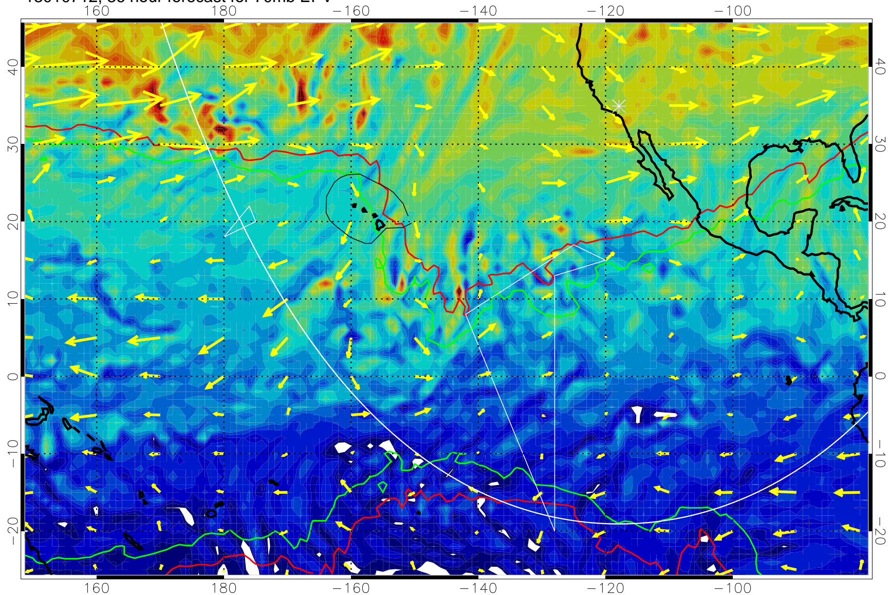
13010712, 36 hour forecast for 70mb EPV
