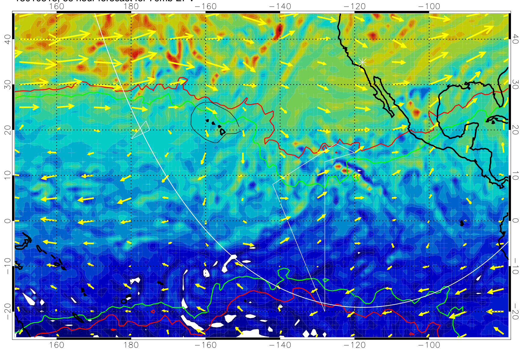
13010818, 66 hour forecast for 70mb EPV
