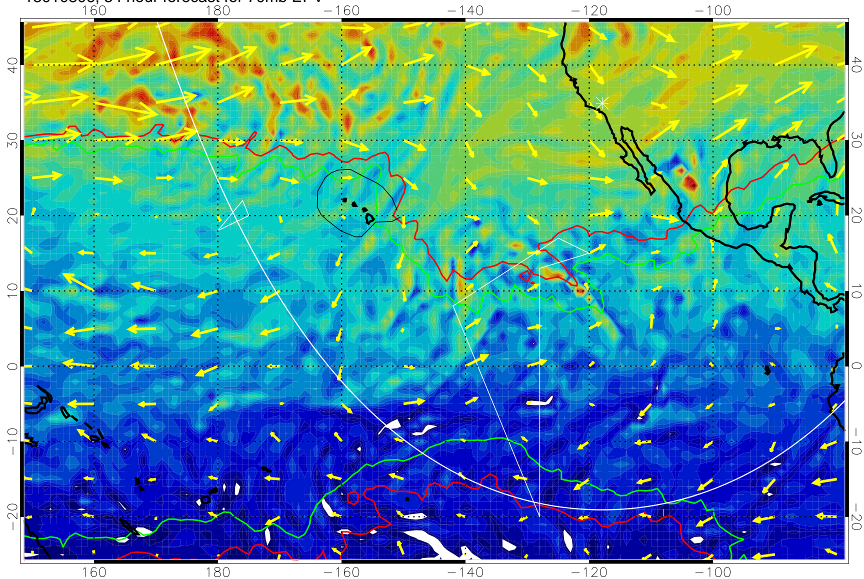
13010806, 54 hour forecast for 70mb EPV
