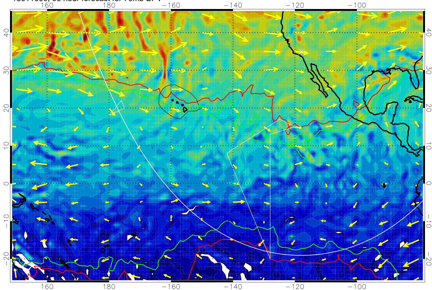
13011000, 96 hour forecast for 70mb EPV
