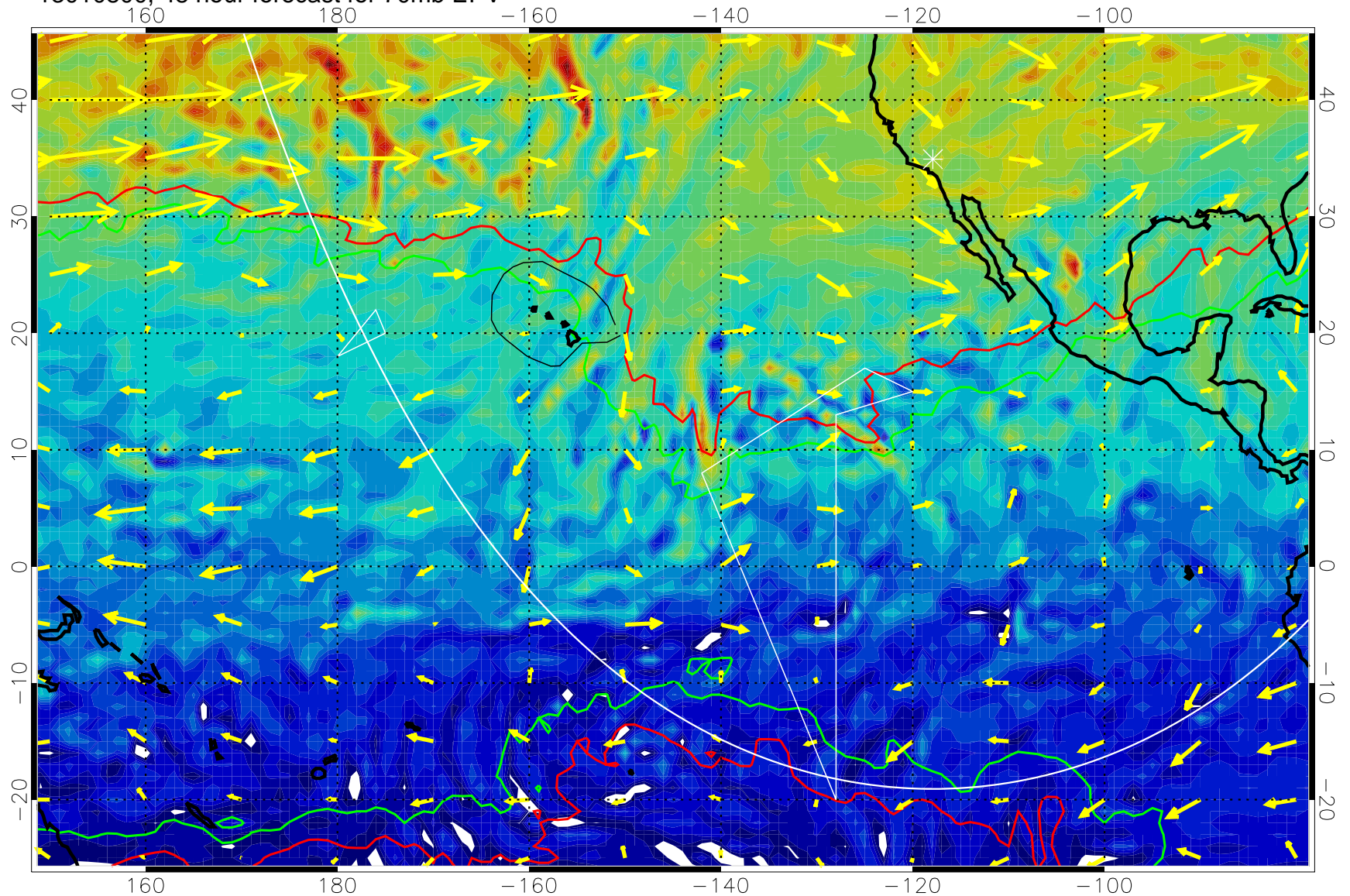
13010800, 48 hour forecast for 70mb EPV
