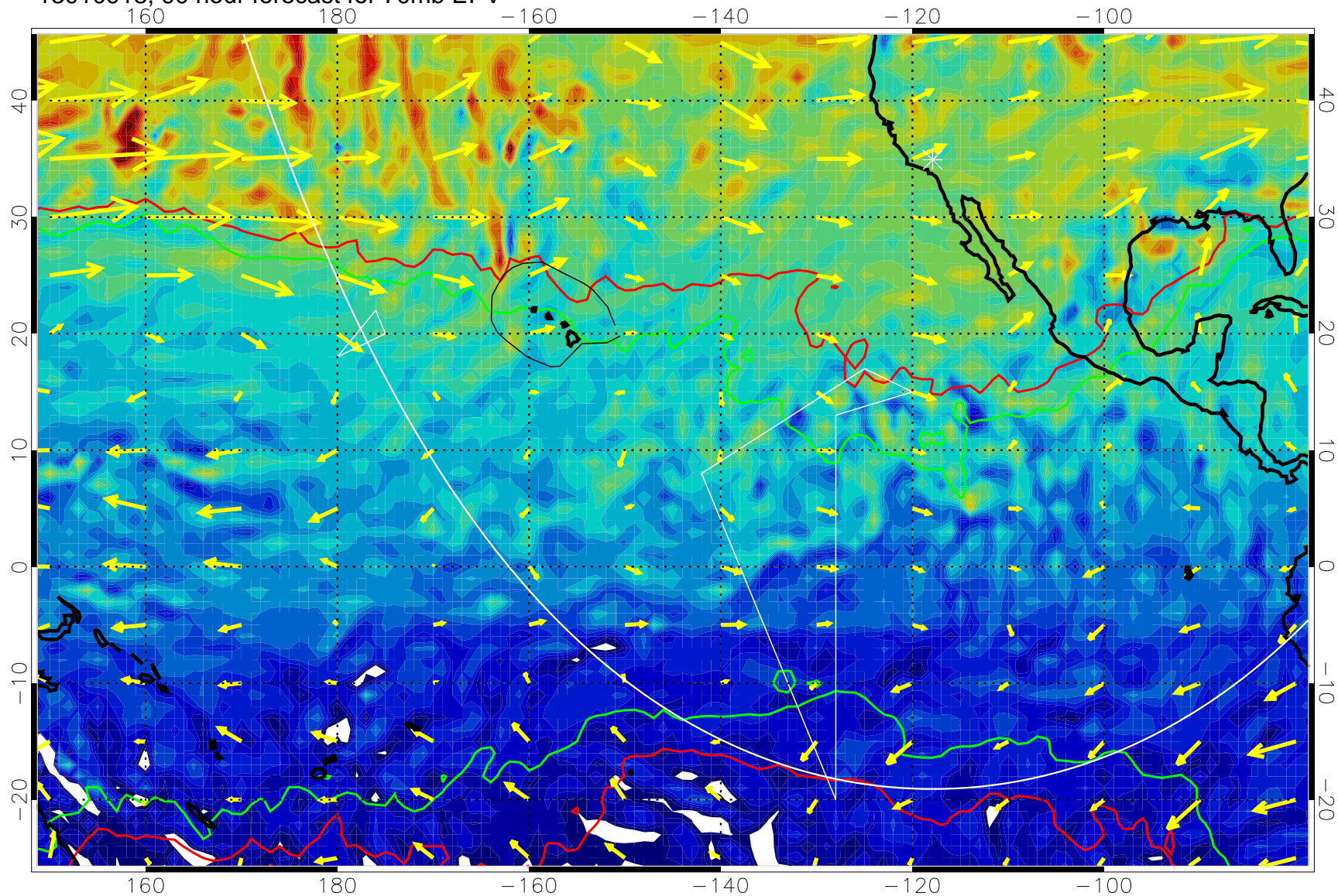
13010918, 90 hour forecast for 70mb EPV
