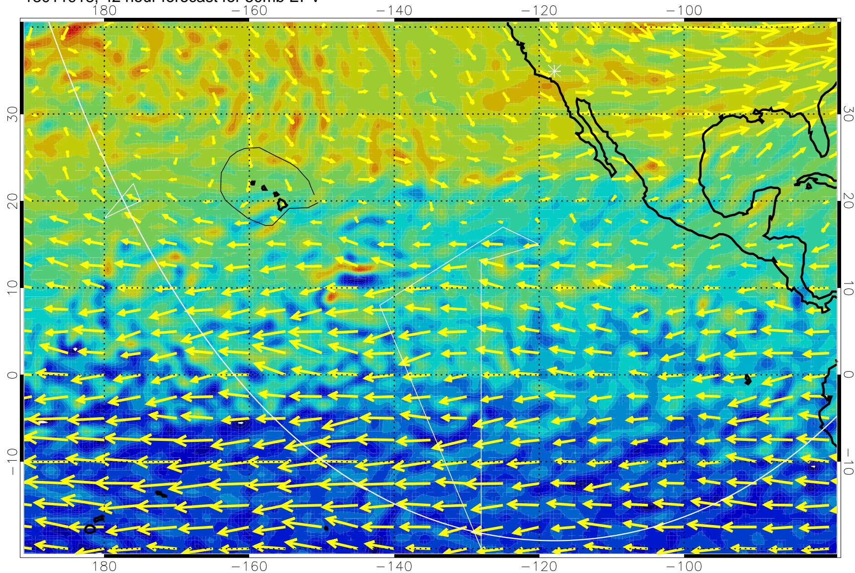
13011918, 42 hour forecast for 50mb EPV
