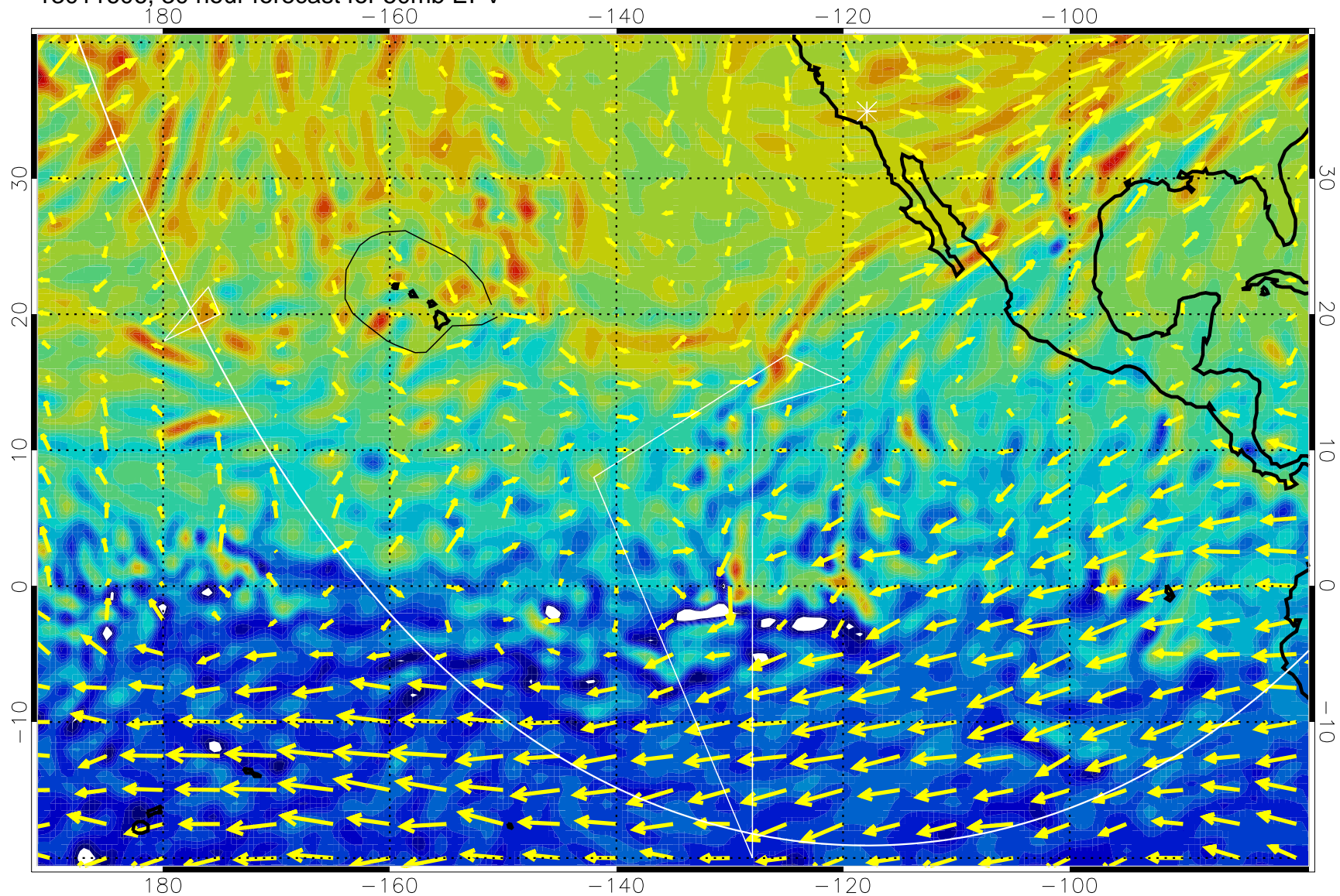
13011606, 30 hour forecast for 50mb EPV
