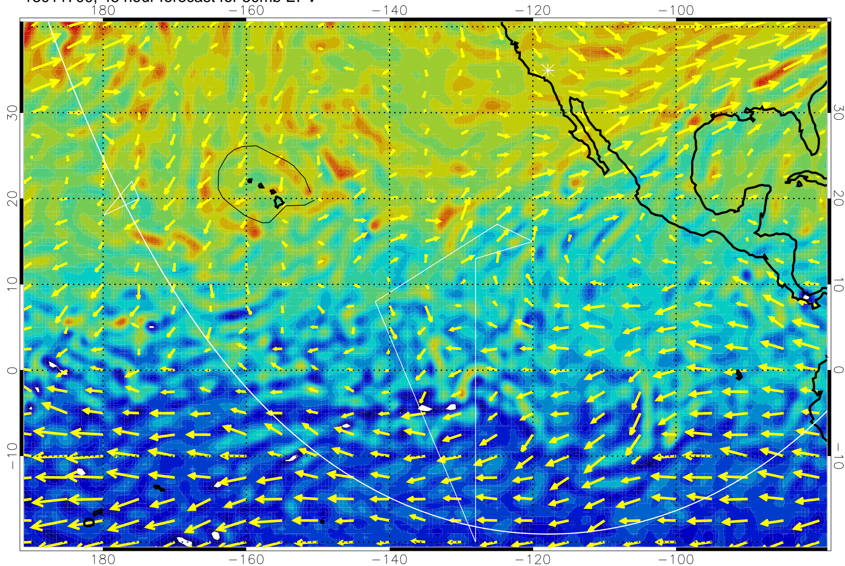
13011700, 48 hour forecast for 50mb EPV
