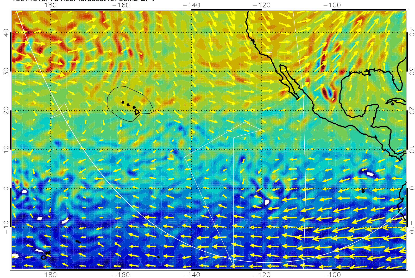
13011318, 78 hour forecast for 50mb EPV
