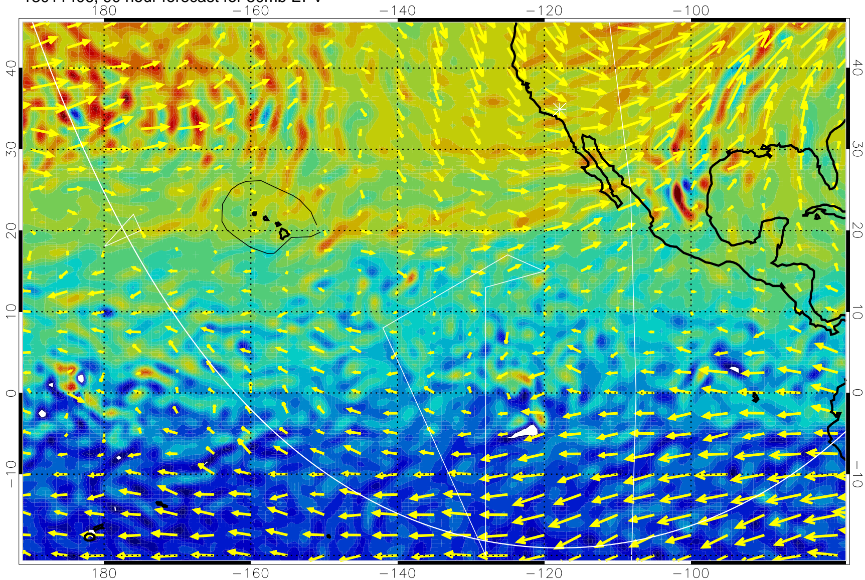
13011406, 90 hour forecast for 50mb EPV
