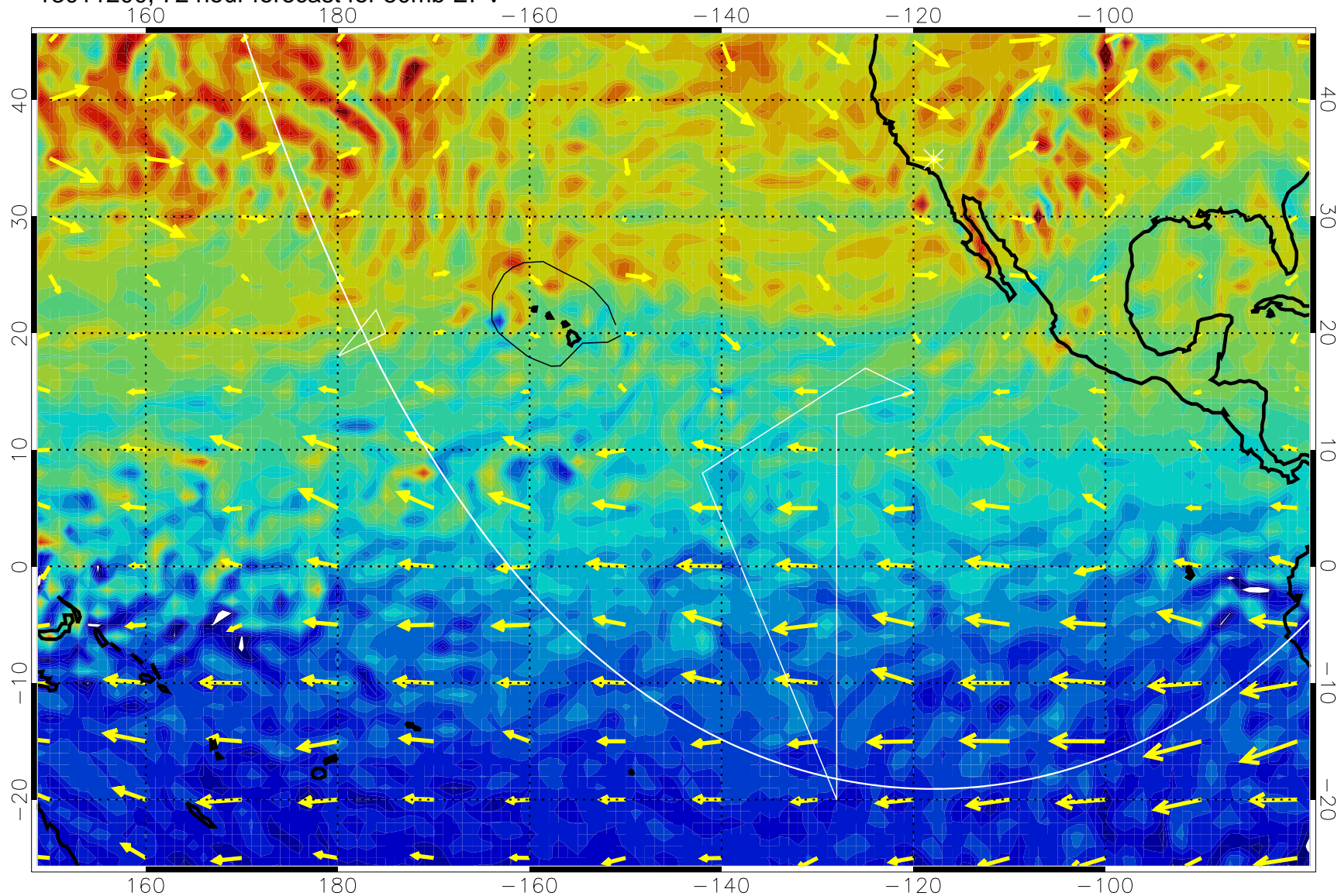
13011200, 72 hour forecast for 50mb EPV
