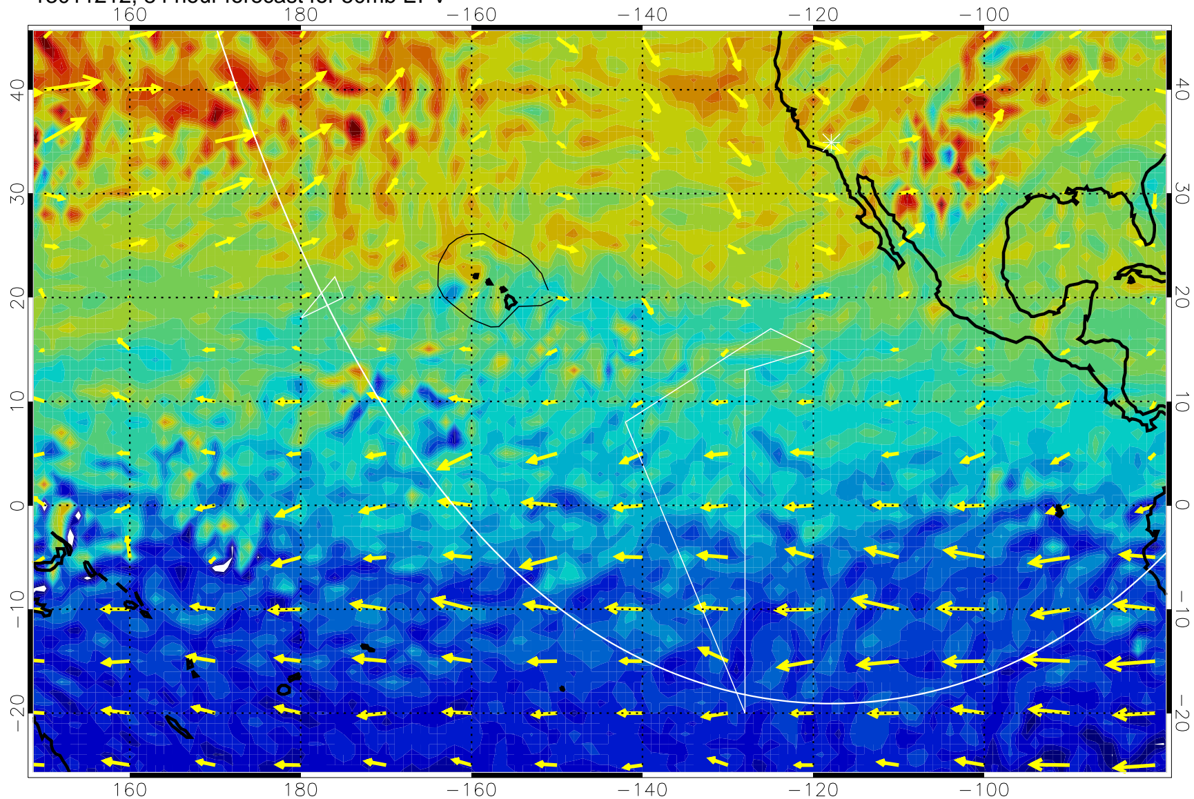
13011212, 84 hour forecast for 50mb EPV
