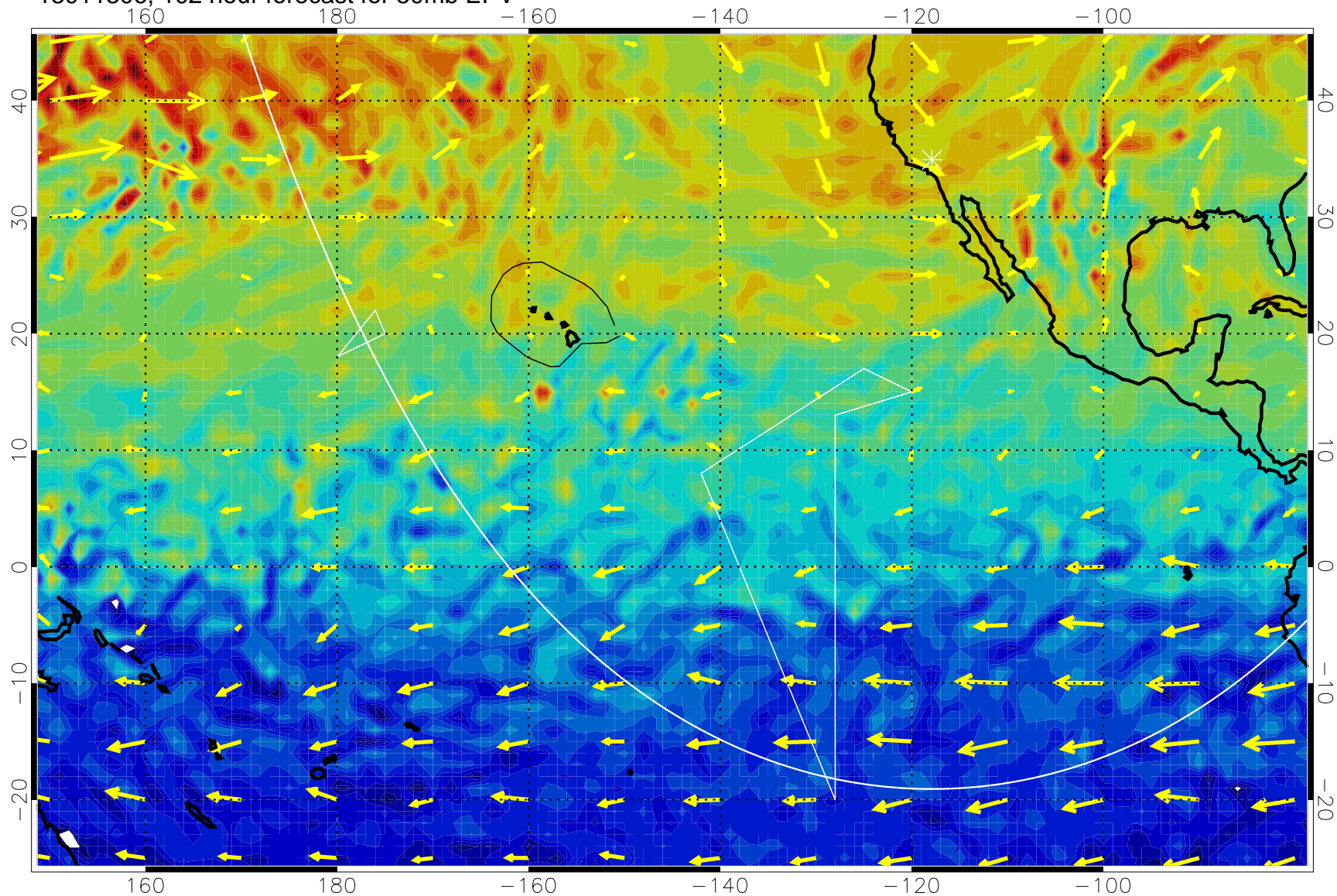
13011306, 102 hour forecast for 50mb EPV
