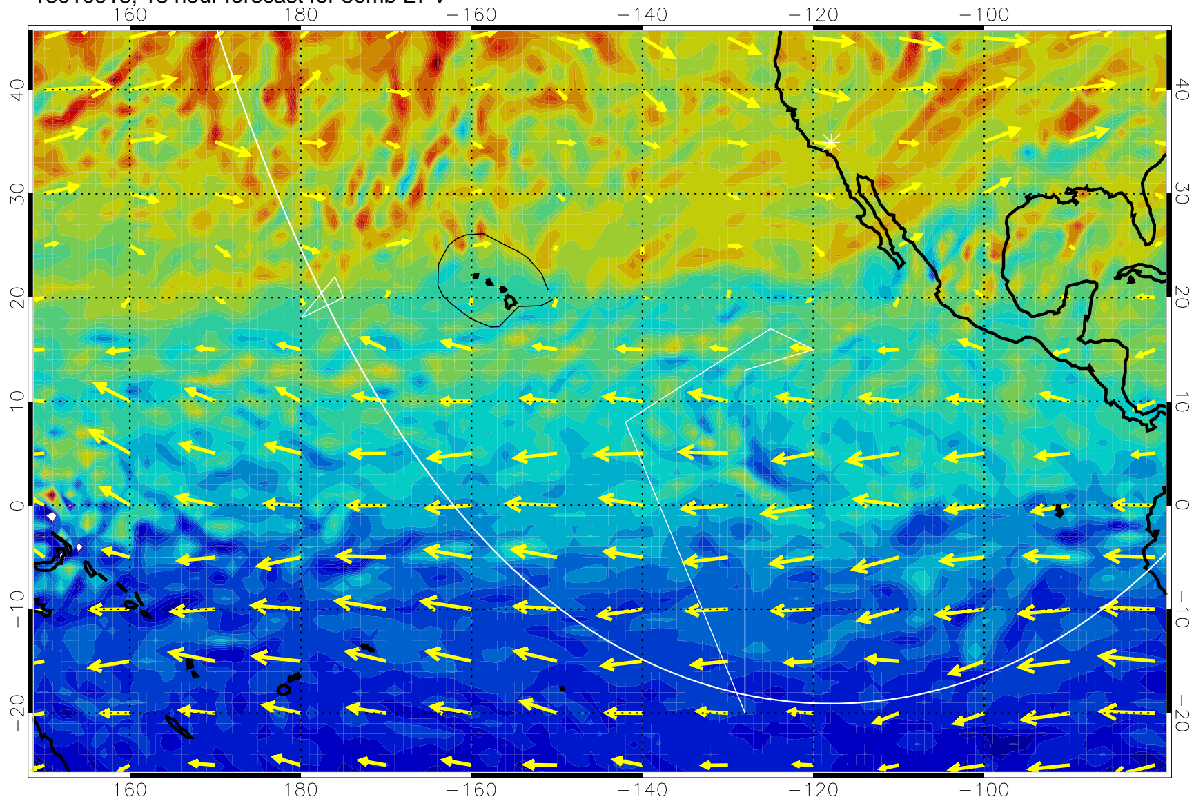
13010918, 18 hour forecast for 50mb EPV
