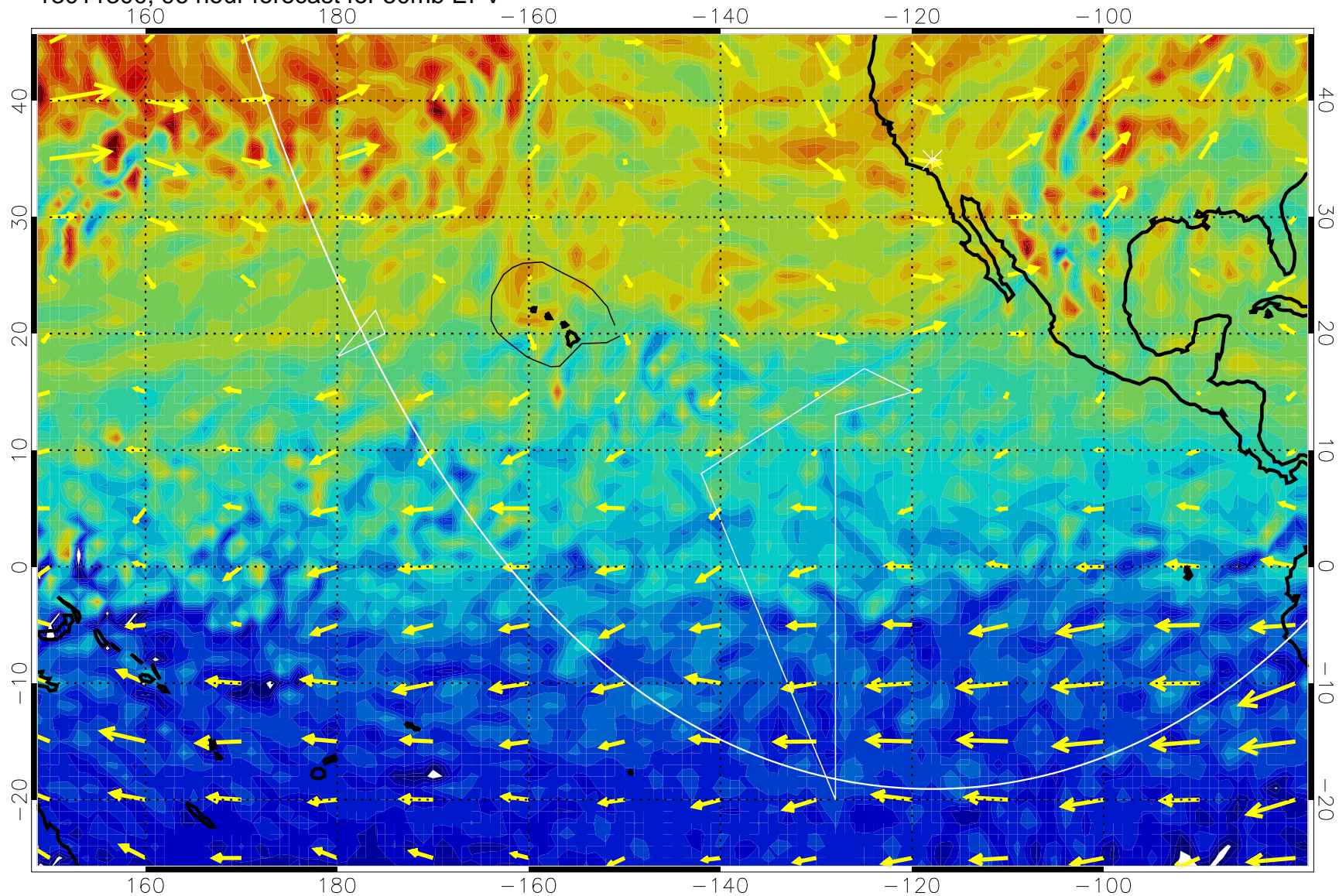
13011300, 96 hour forecast for 50mb EPV
