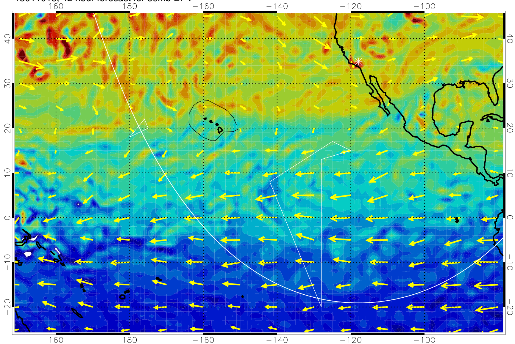
13011018, 42 hour forecast for 50mb EPV
