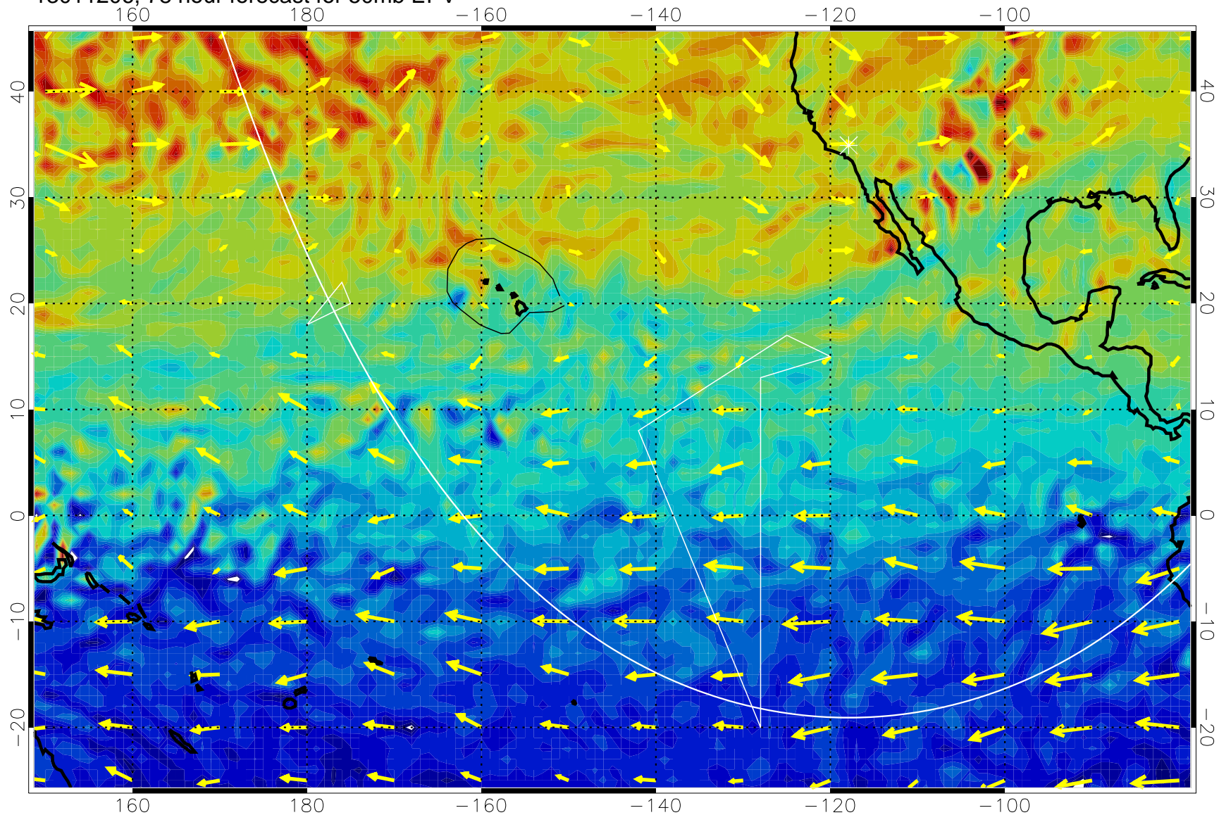
13011206, 78 hour forecast for 50mb EPV
