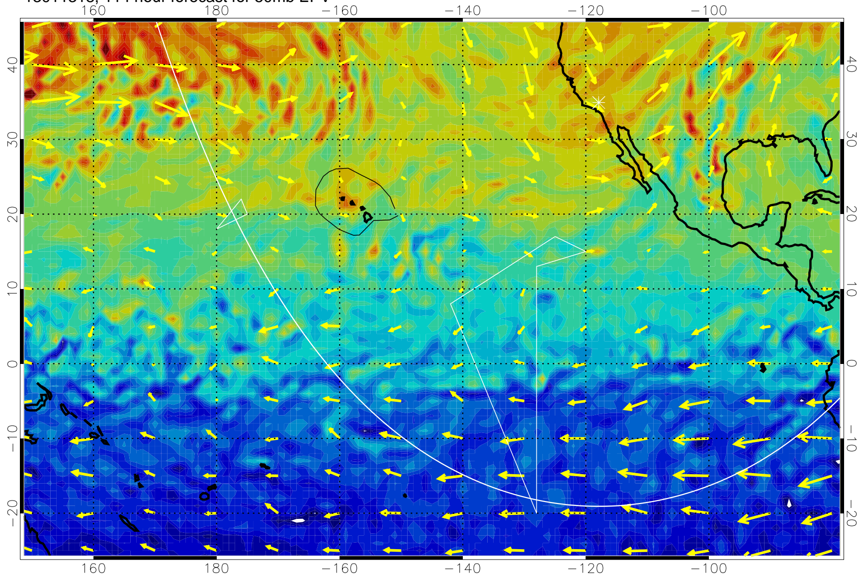
13011318, 114 hour forecast for 50mb EPV
