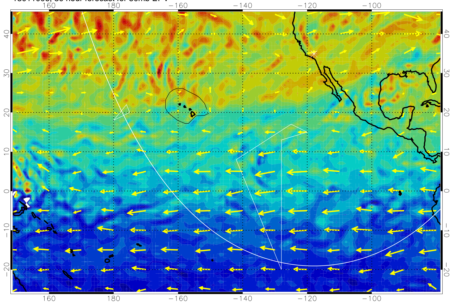
13011006, 30 hour forecast for 50mb EPV
