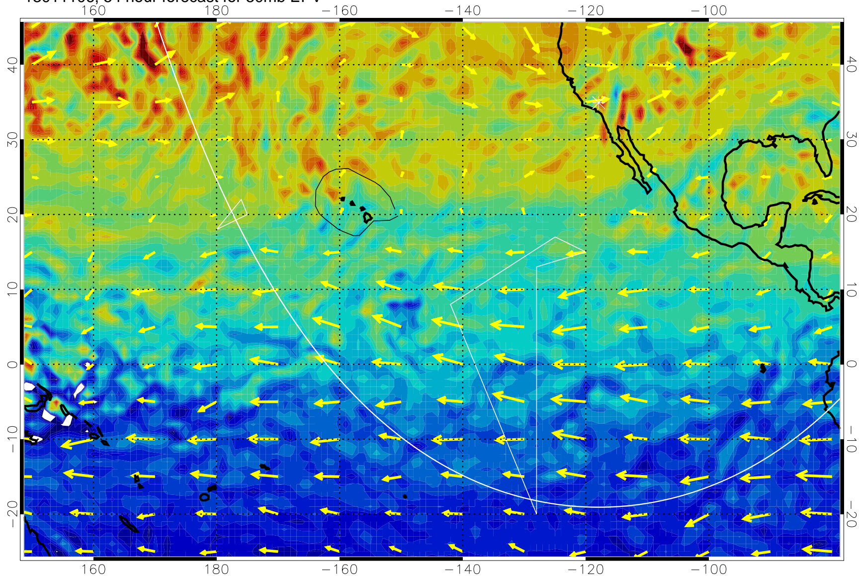
13011106, 54 hour forecast for 50mb EPV
