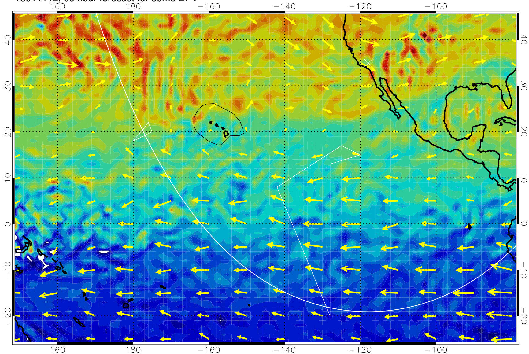
13011112, 60 hour forecast for 50mb EPV
