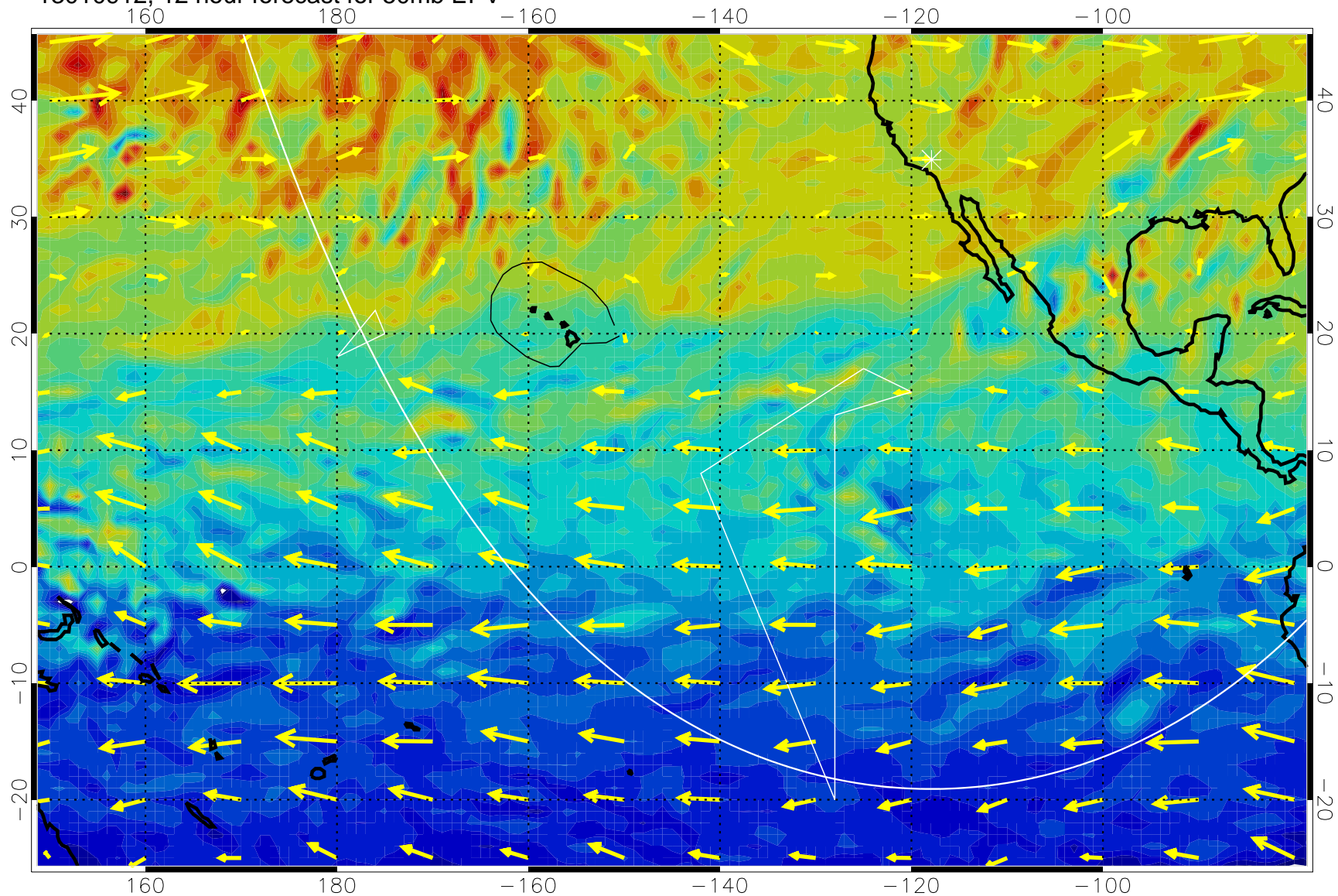
13010912, 12 hour forecast for 50mb EPV
