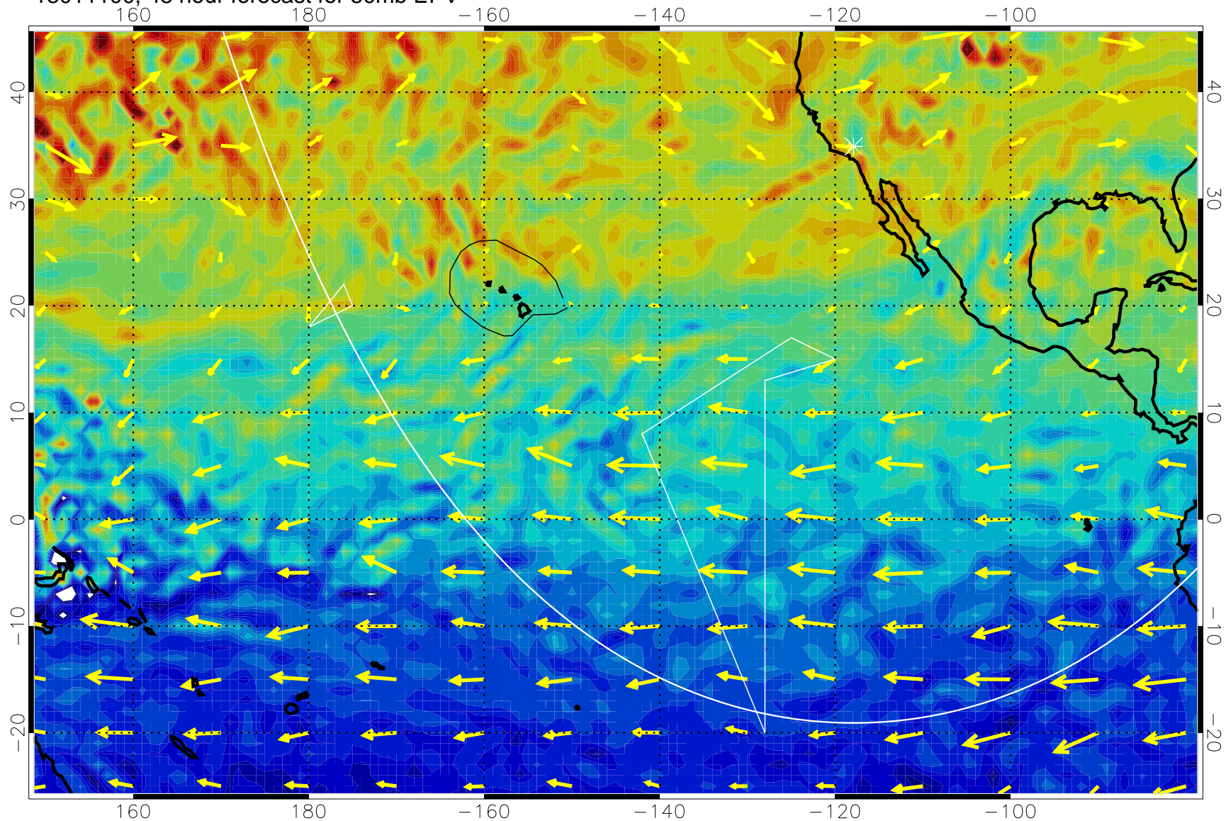
13011100, 48 hour forecast for 50mb EPV
