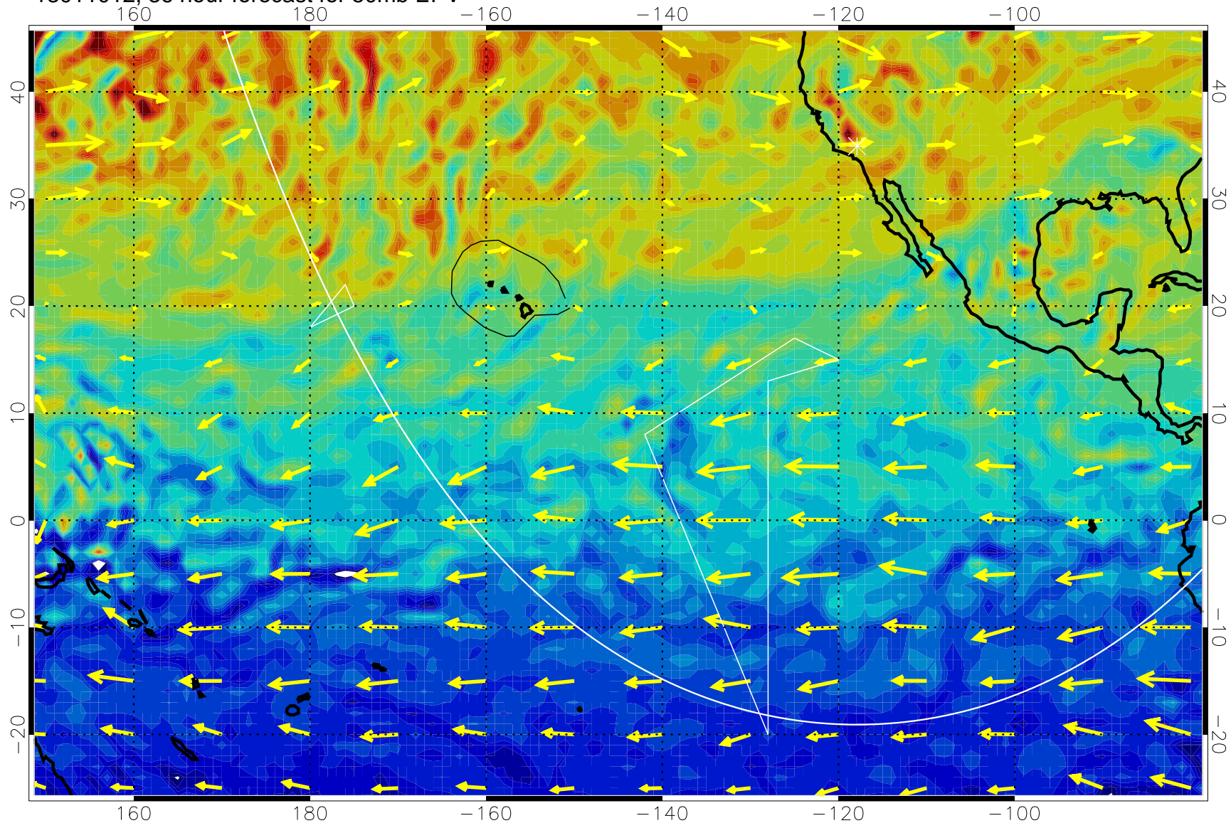
13011012, 36 hour forecast for 50mb EPV
