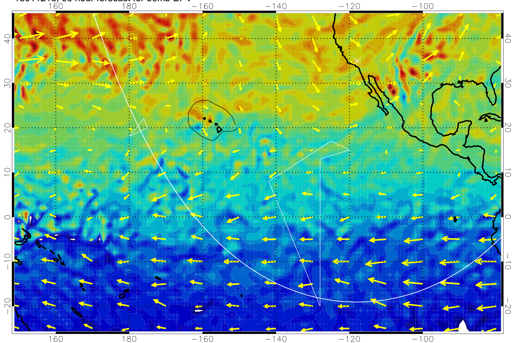
13011218, 90 hour forecast for 50mb EPV
