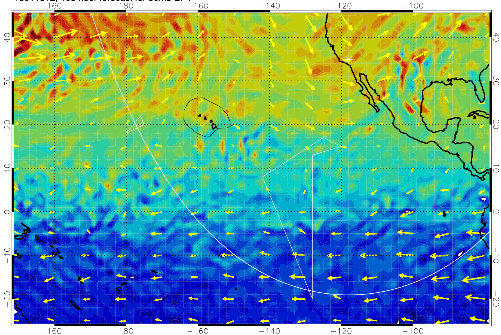
13011312, 108 hour forecast for 50mb EPV
