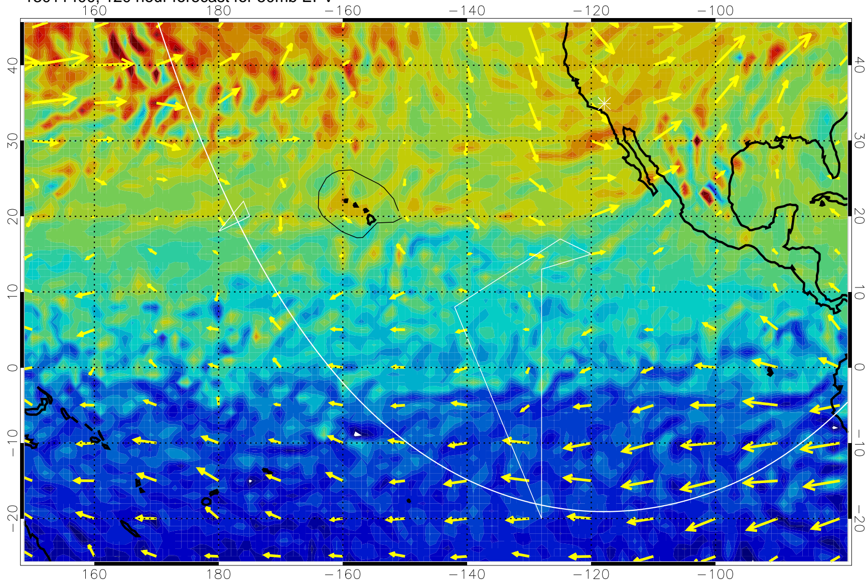
13011400, 120 hour forecast for 50mb EPV
