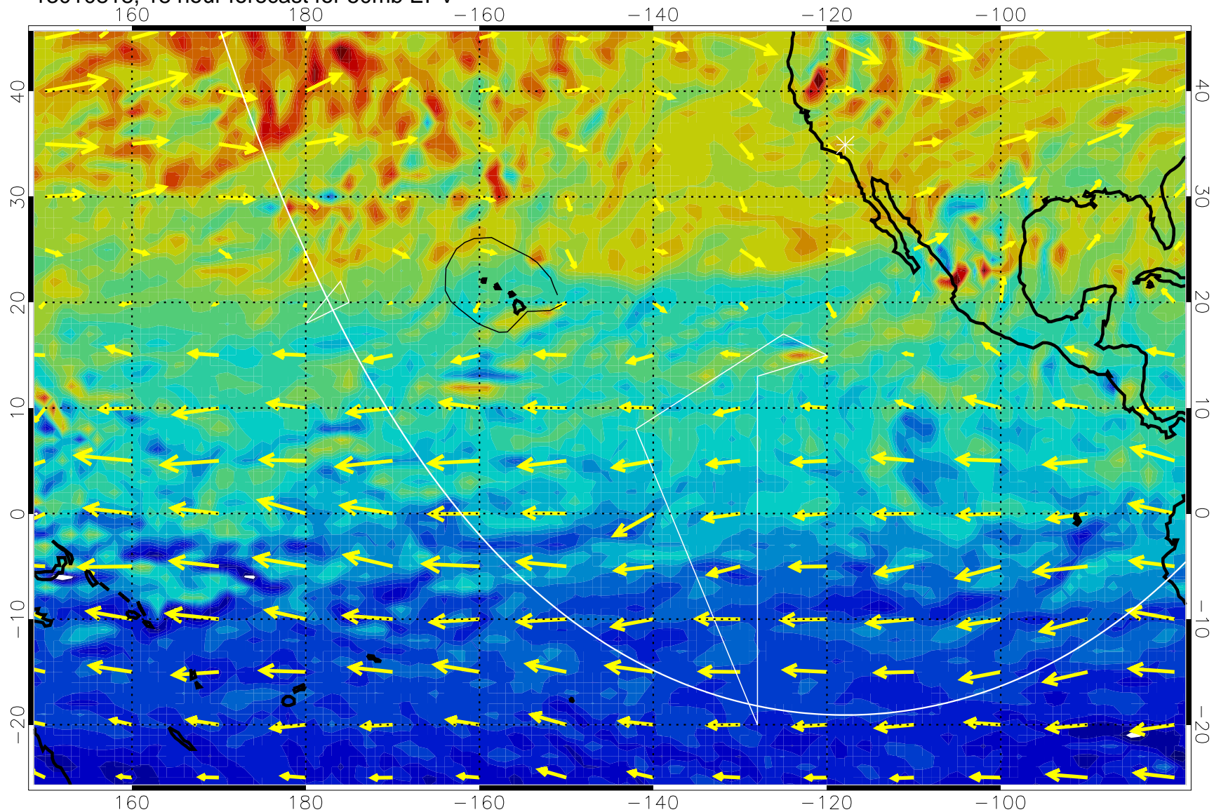
13010818, 18 hour forecast for 50mb EPV
