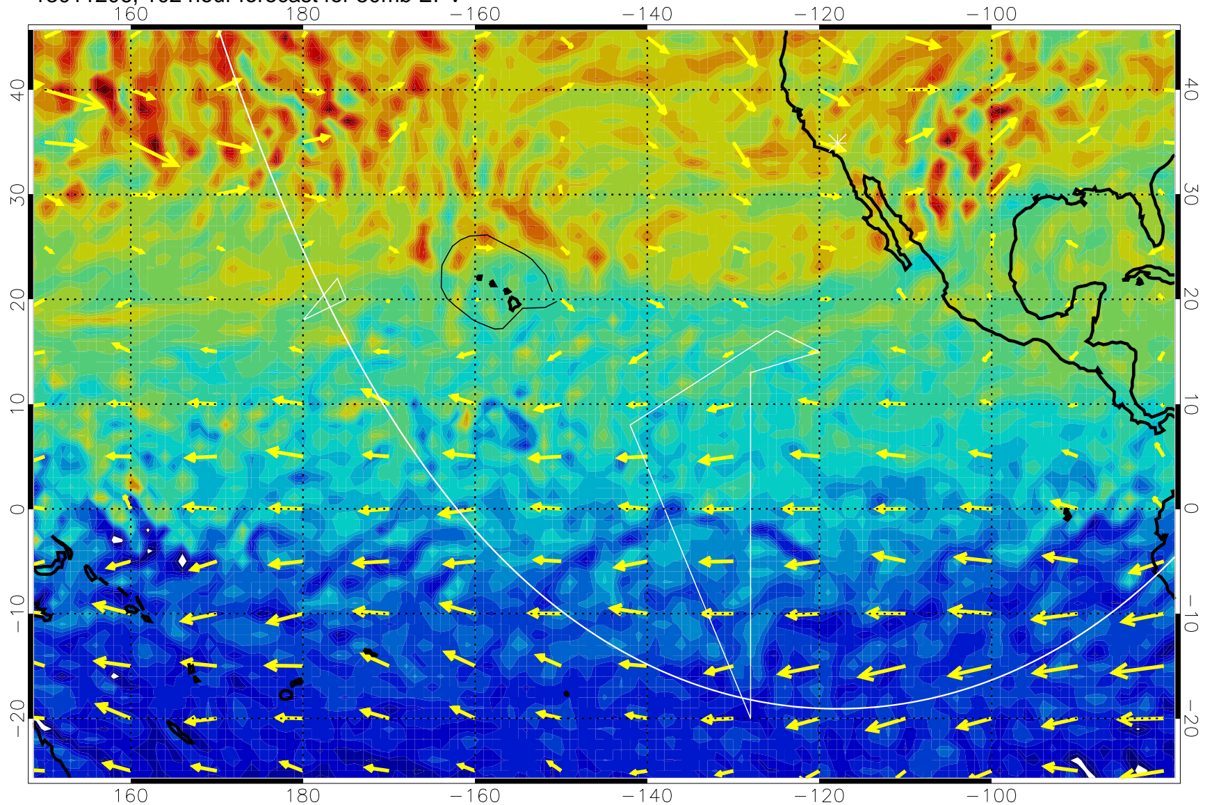
13011206, 102 hour forecast for 50mb EPV
