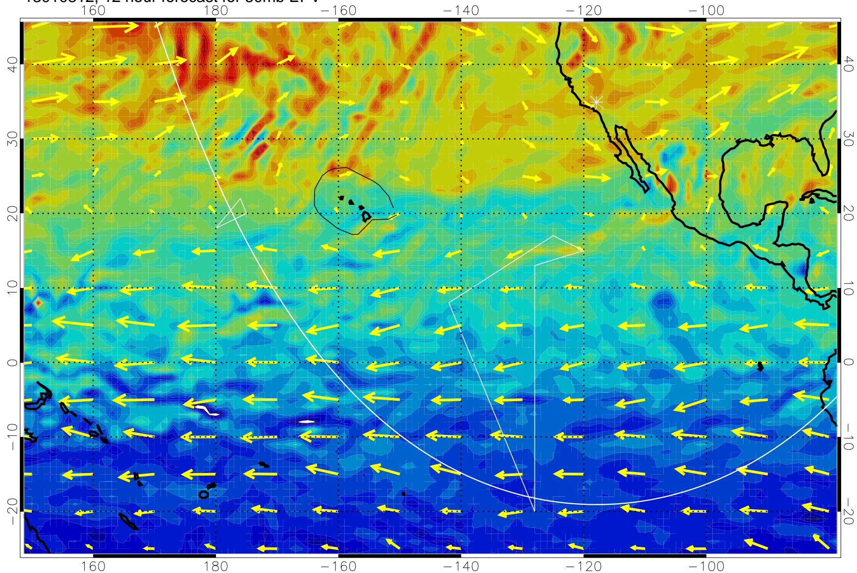
13010812, 12 hour forecast for 50mb EPV
