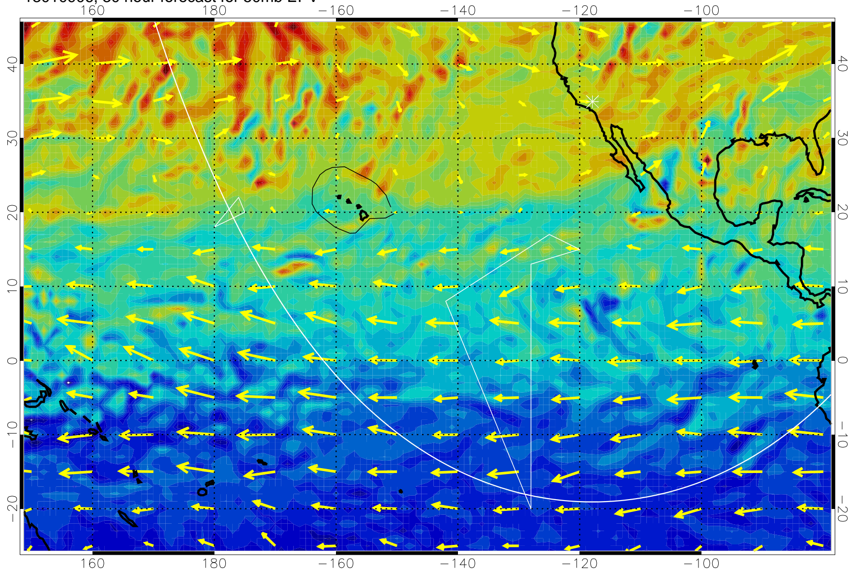
13010906, 30 hour forecast for 50mb EPV
