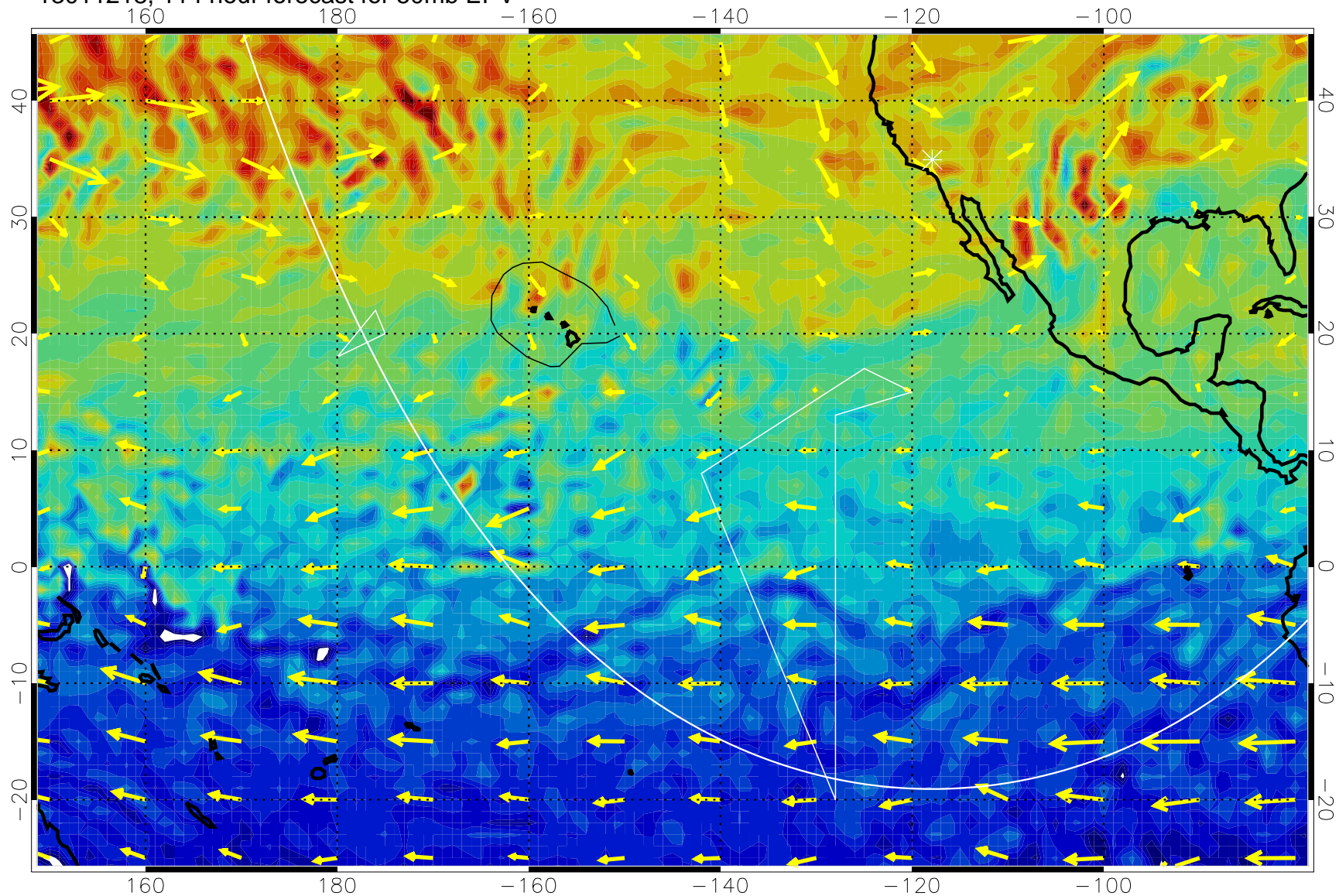
13011218, 114 hour forecast for 50mb EPV
