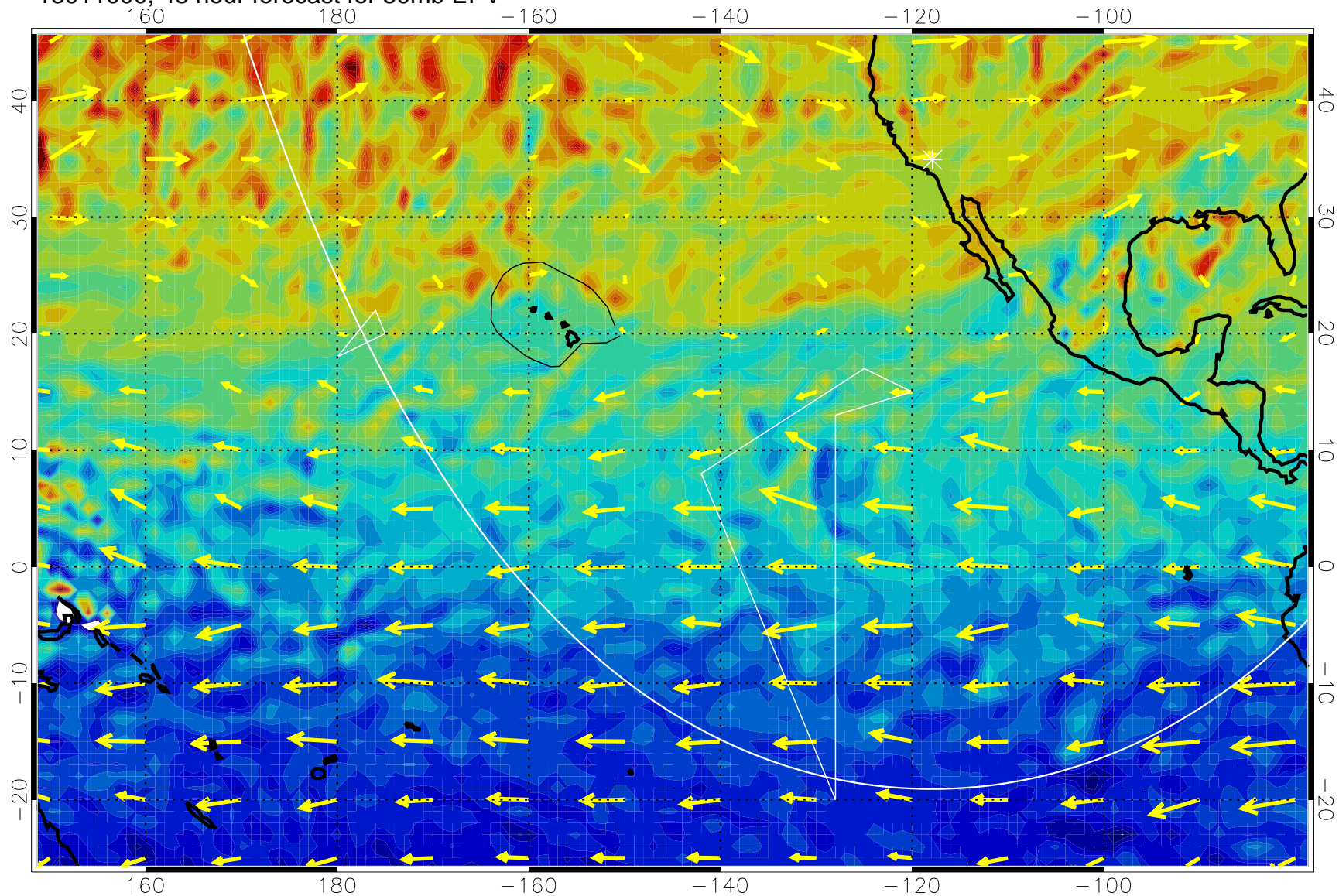
13011000, 48 hour forecast for 50mb EPV
