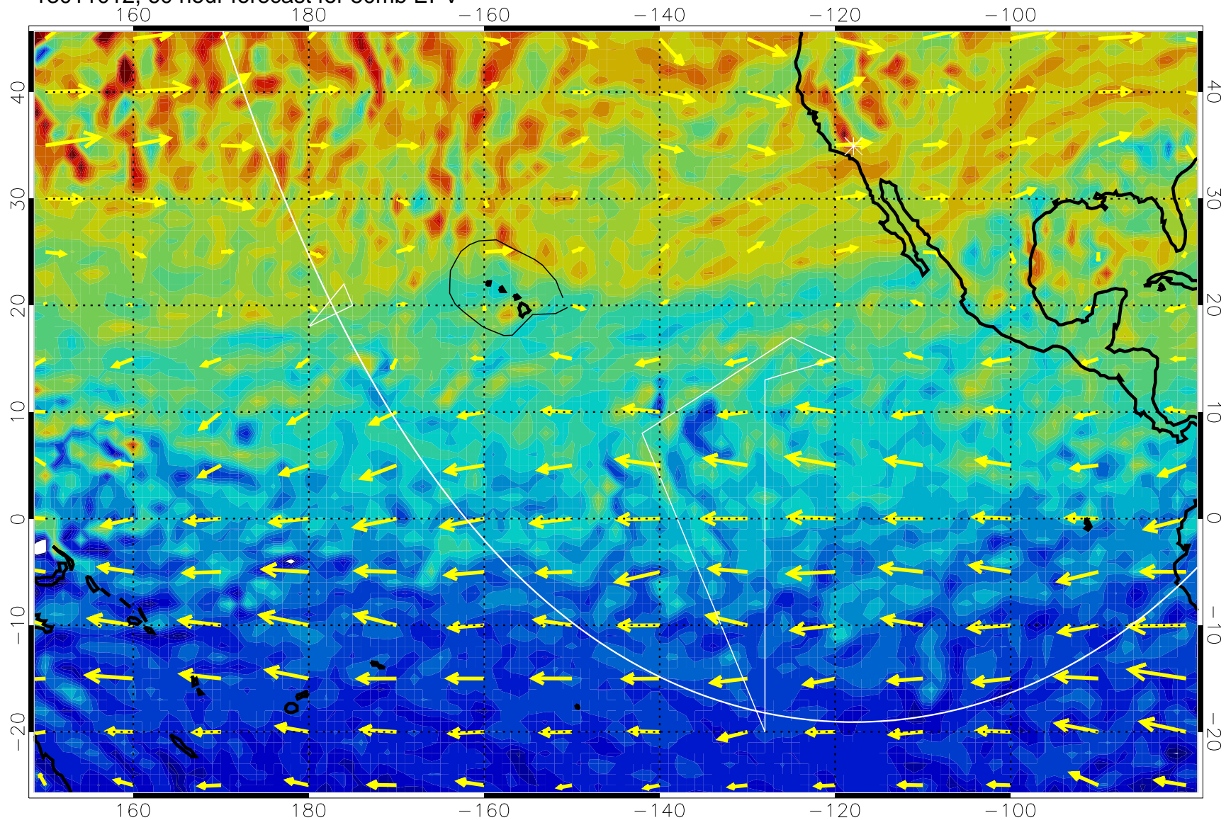
13011012, 60 hour forecast for 50mb EPV
