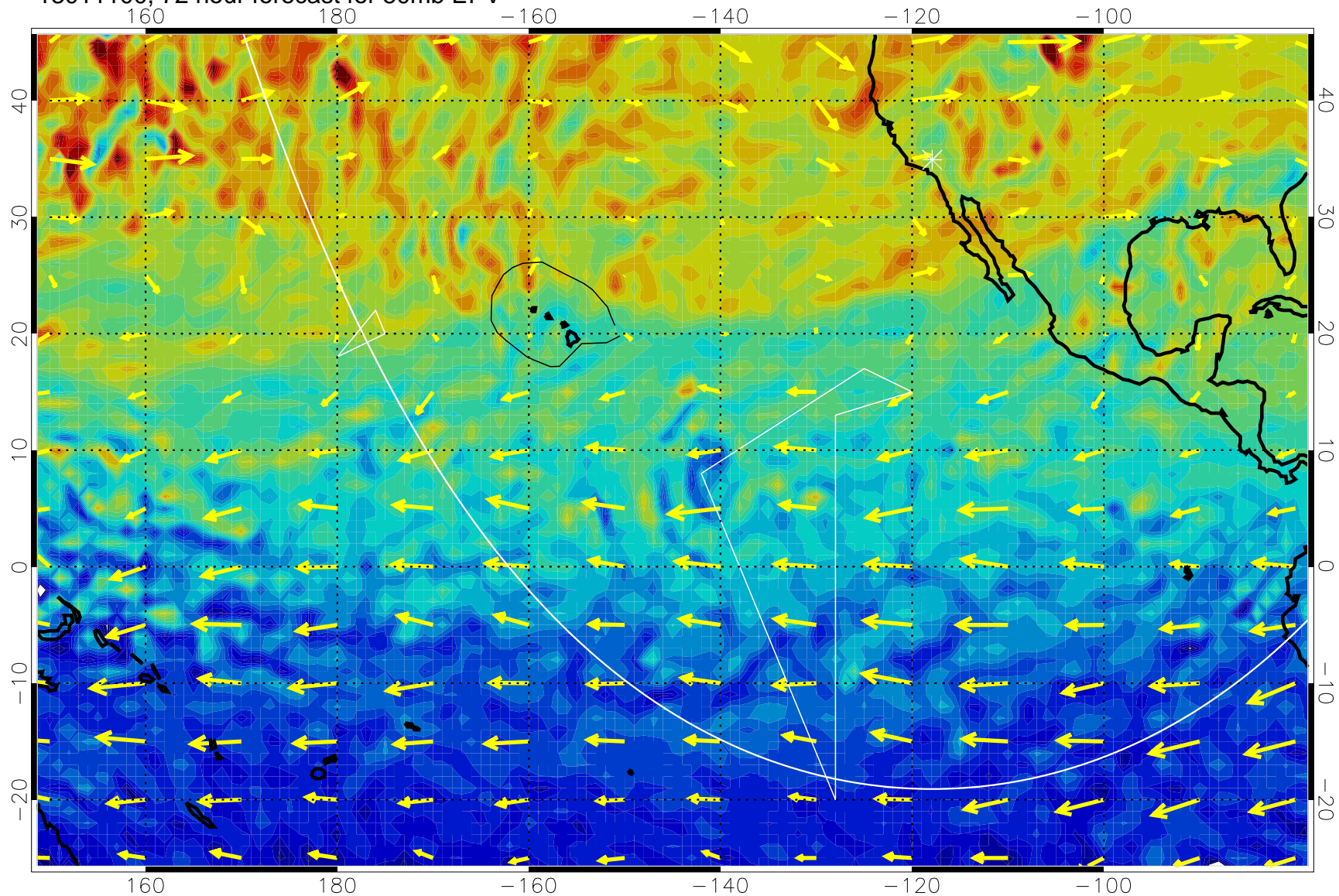
13011100, 72 hour forecast for 50mb EPV
