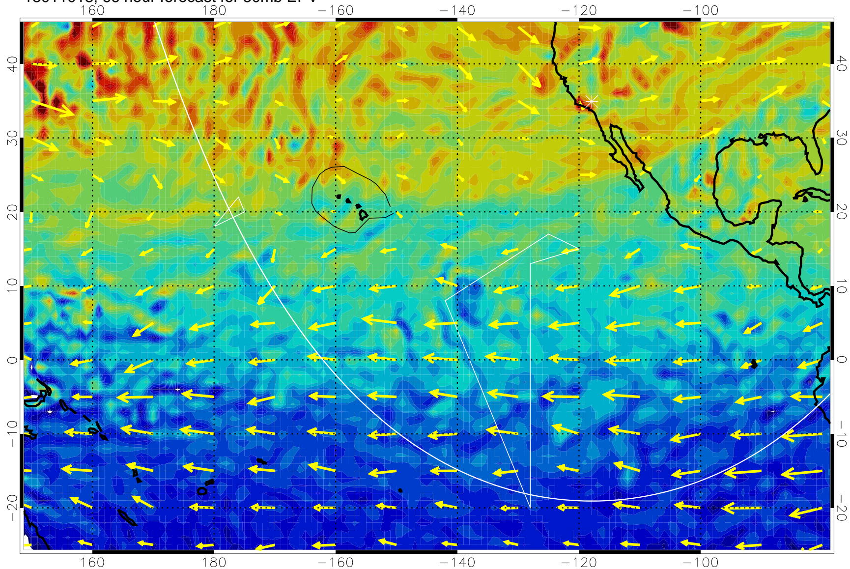
13011018, 66 hour forecast for 50mb EPV
