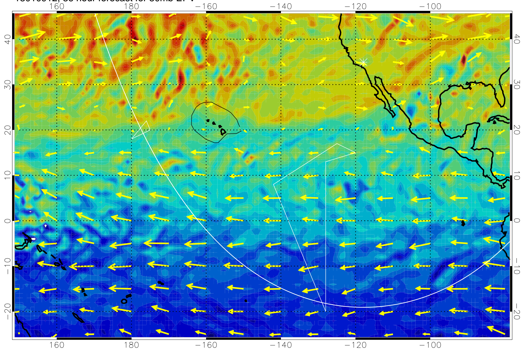
13010912, 36 hour forecast for 50mb EPV
