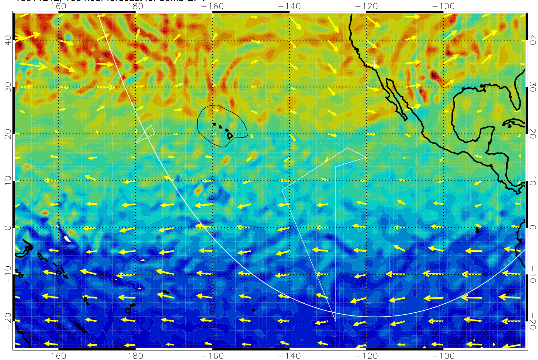
13011212, 108 hour forecast for 50mb EPV
