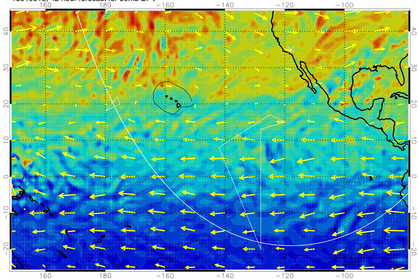
13010918, 42 hour forecast for 50mb EPV
