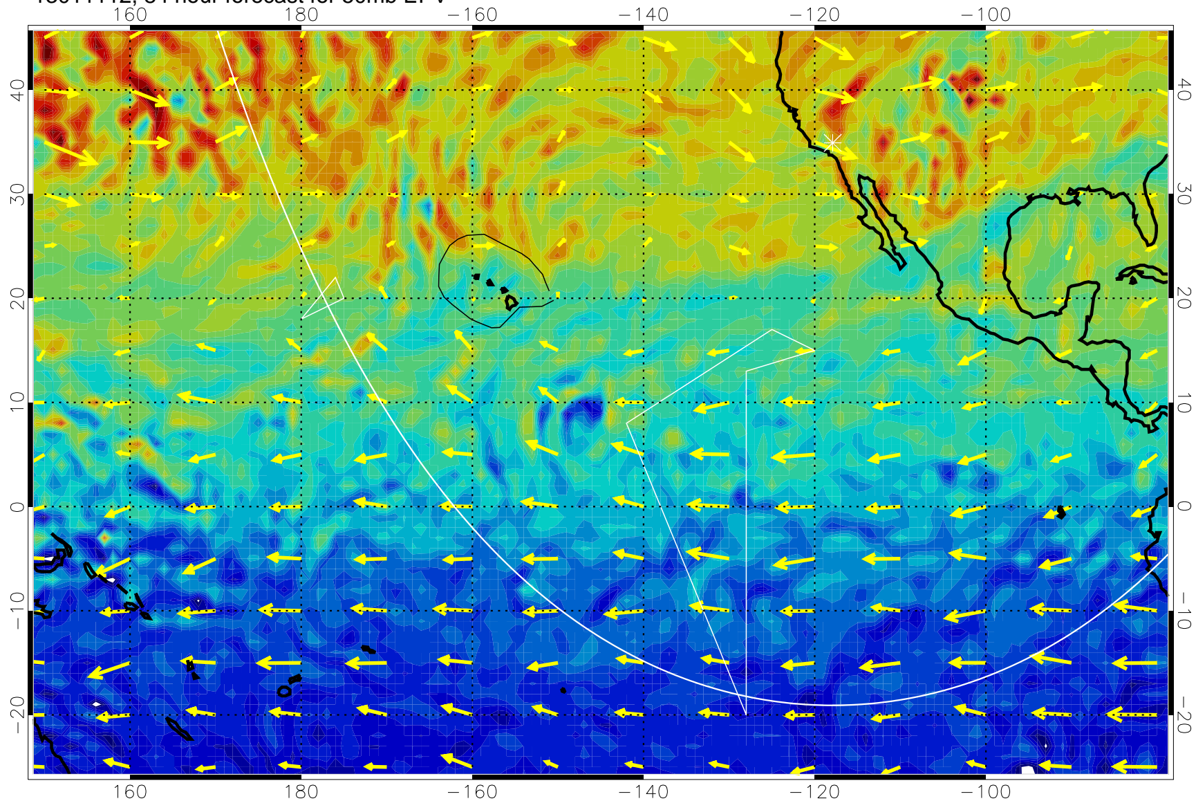
13011112, 84 hour forecast for 50mb EPV
