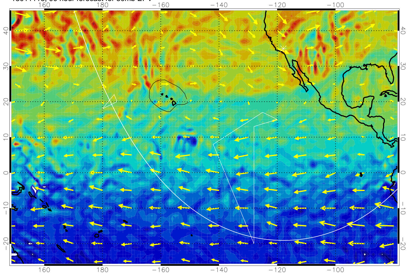
13011118, 90 hour forecast for 50mb EPV
