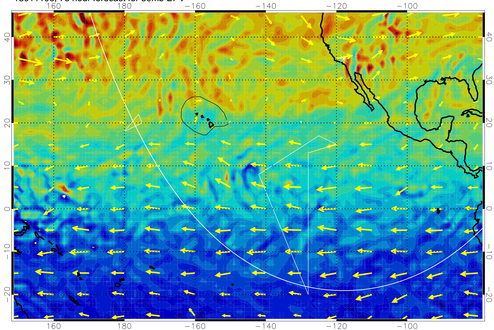
13011106, 78 hour forecast for 50mb EPV
