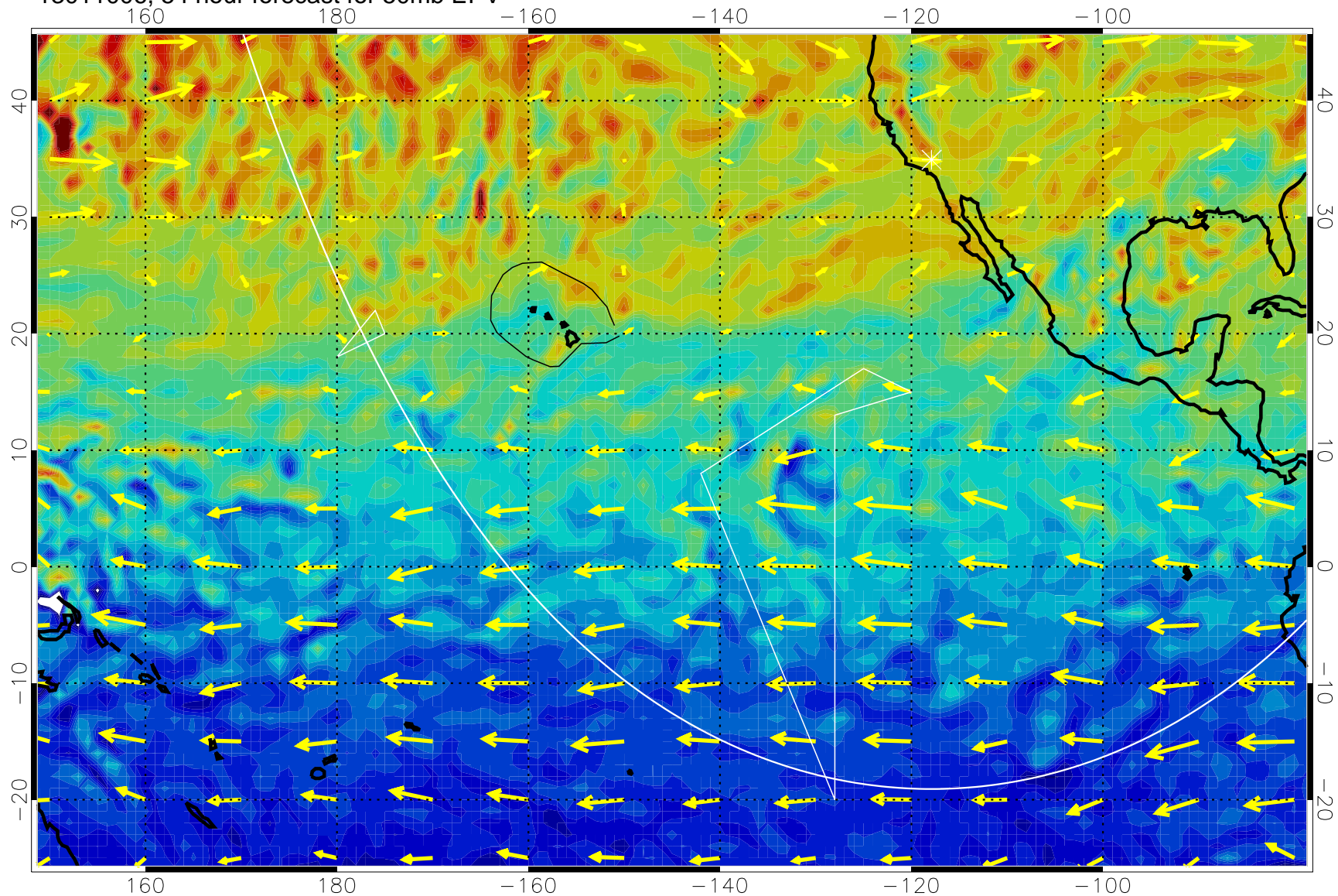
13011006, 54 hour forecast for 50mb EPV
