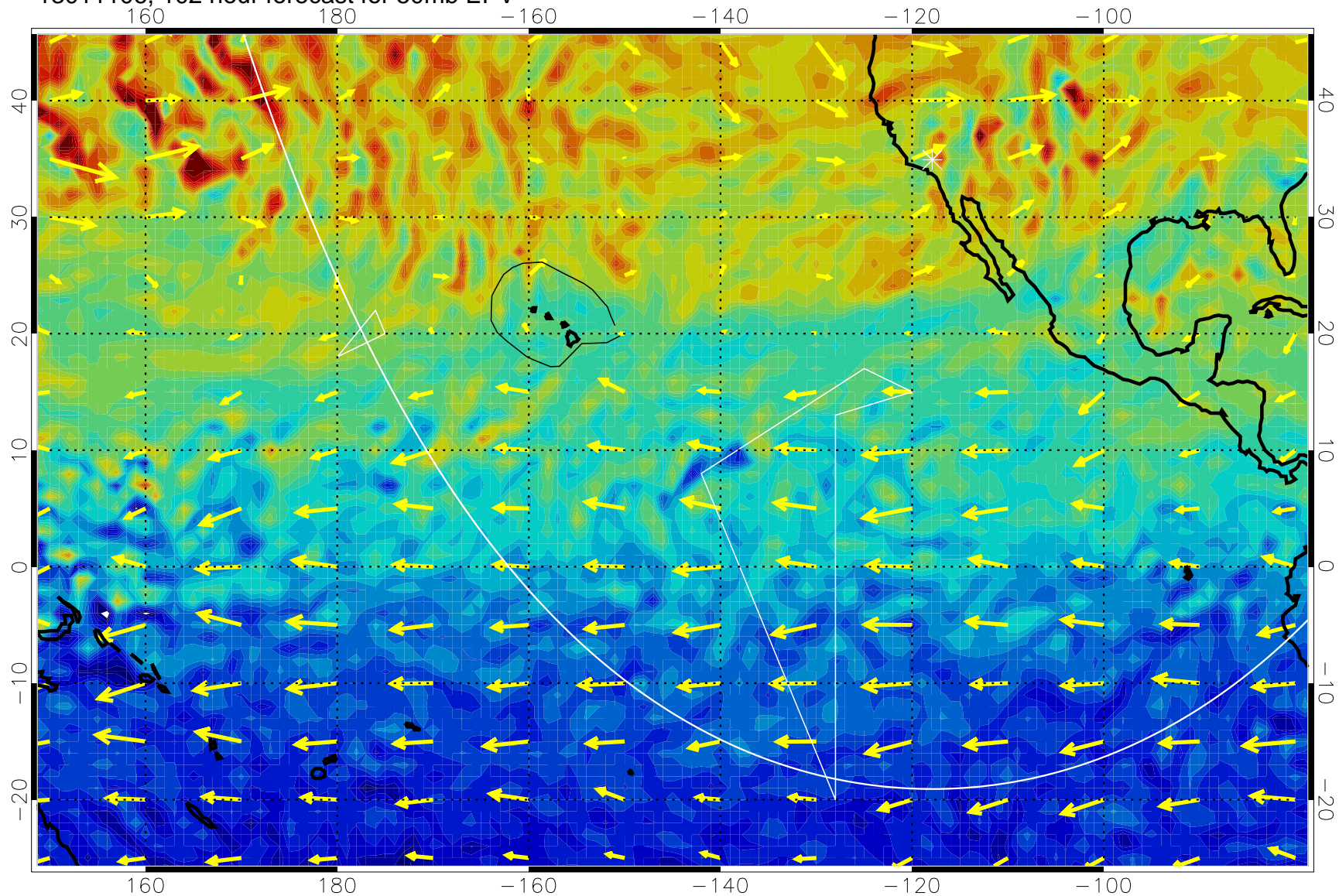
13011106, 102 hour forecast for 50mb EPV
