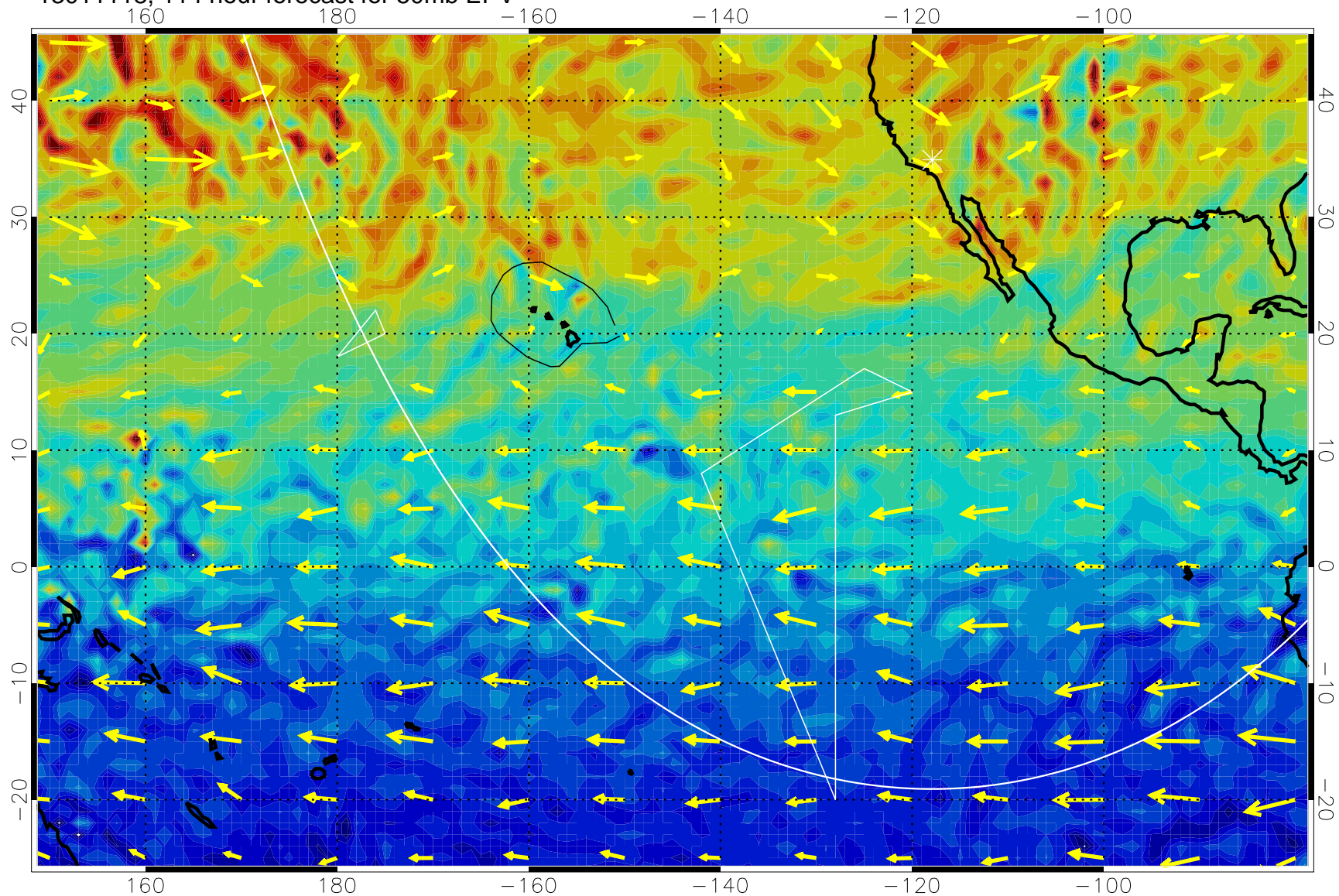
13011118, 114 hour forecast for 50mb EPV
