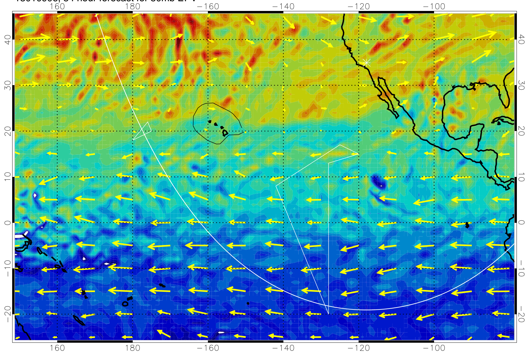
13010906, 54 hour forecast for 50mb EPV
