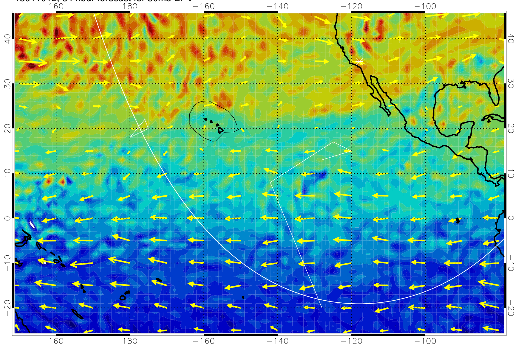
13011012, 84 hour forecast for 50mb EPV
