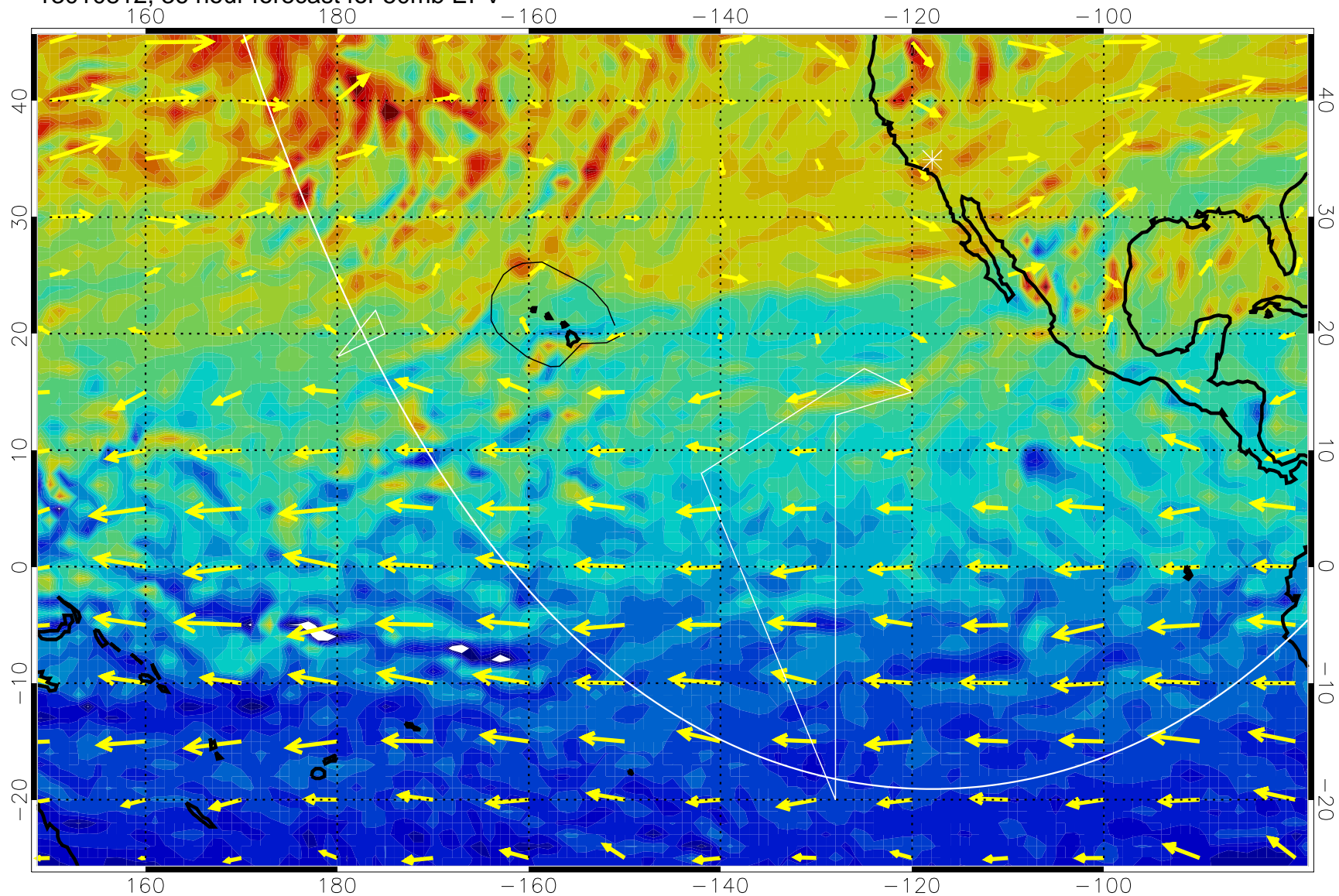
13010812, 36 hour forecast for 50mb EPV
