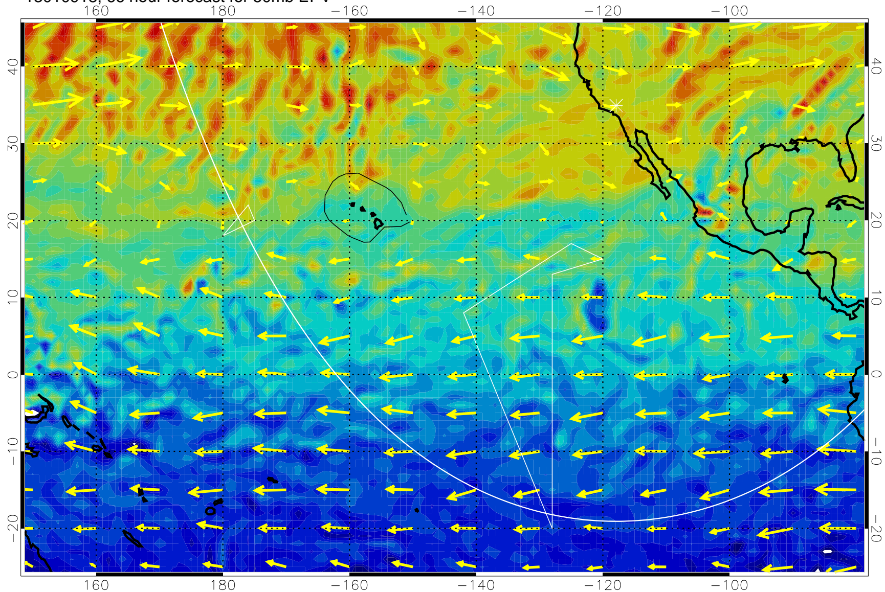
13010918, 66 hour forecast for 50mb EPV
