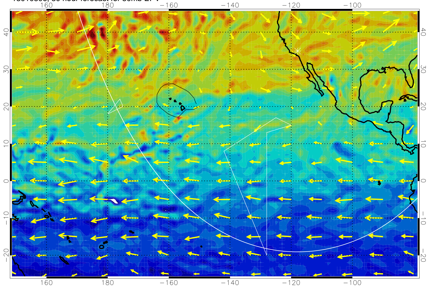
13010806, 30 hour forecast for 50mb EPV
