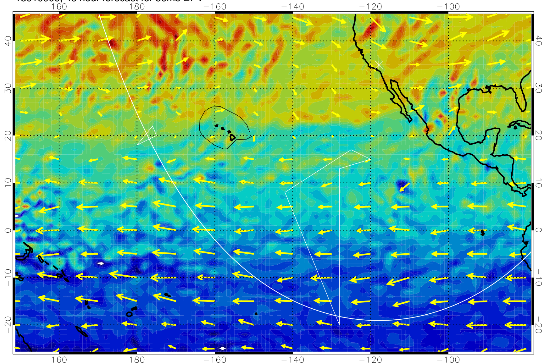
13010900, 48 hour forecast for 50mb EPV
