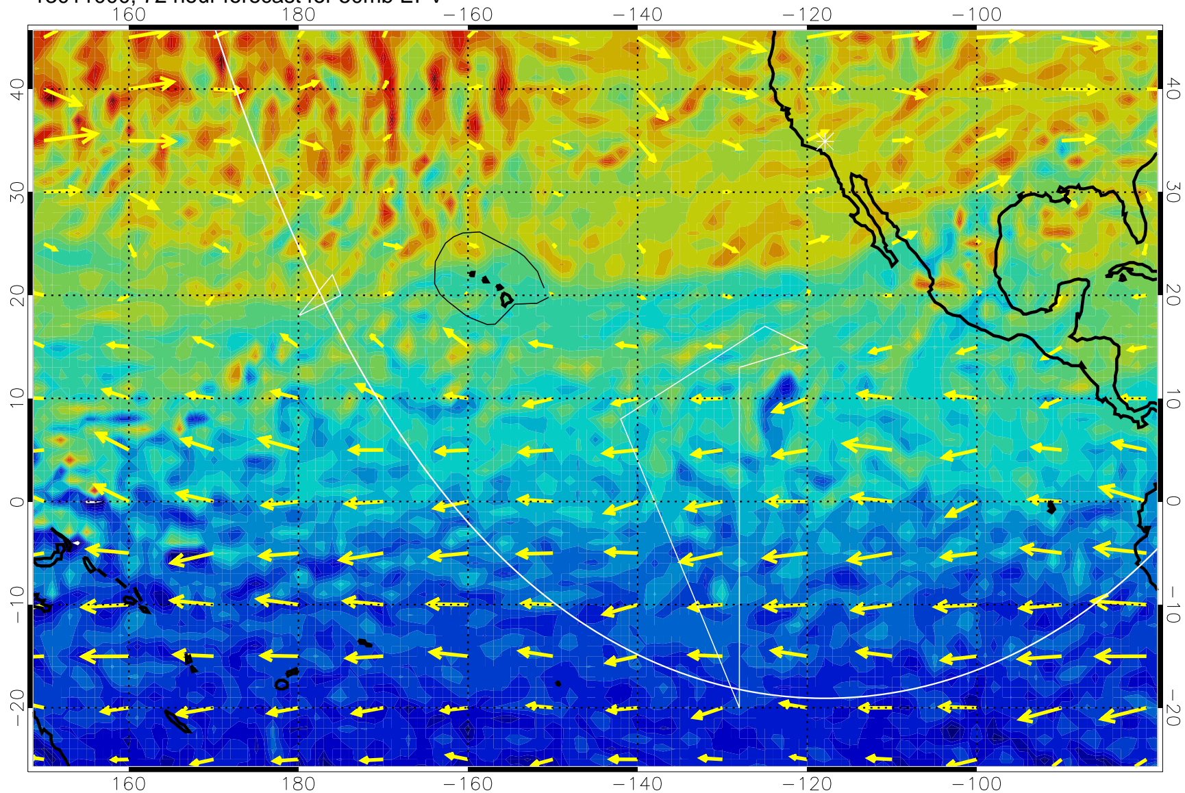
13011000, 72 hour forecast for 50mb EPV
