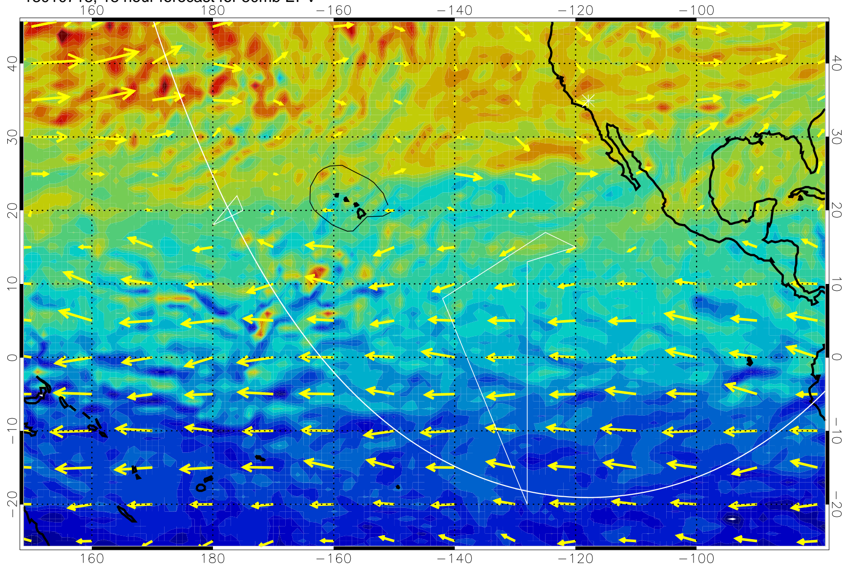
13010718, 18 hour forecast for 50mb EPV
