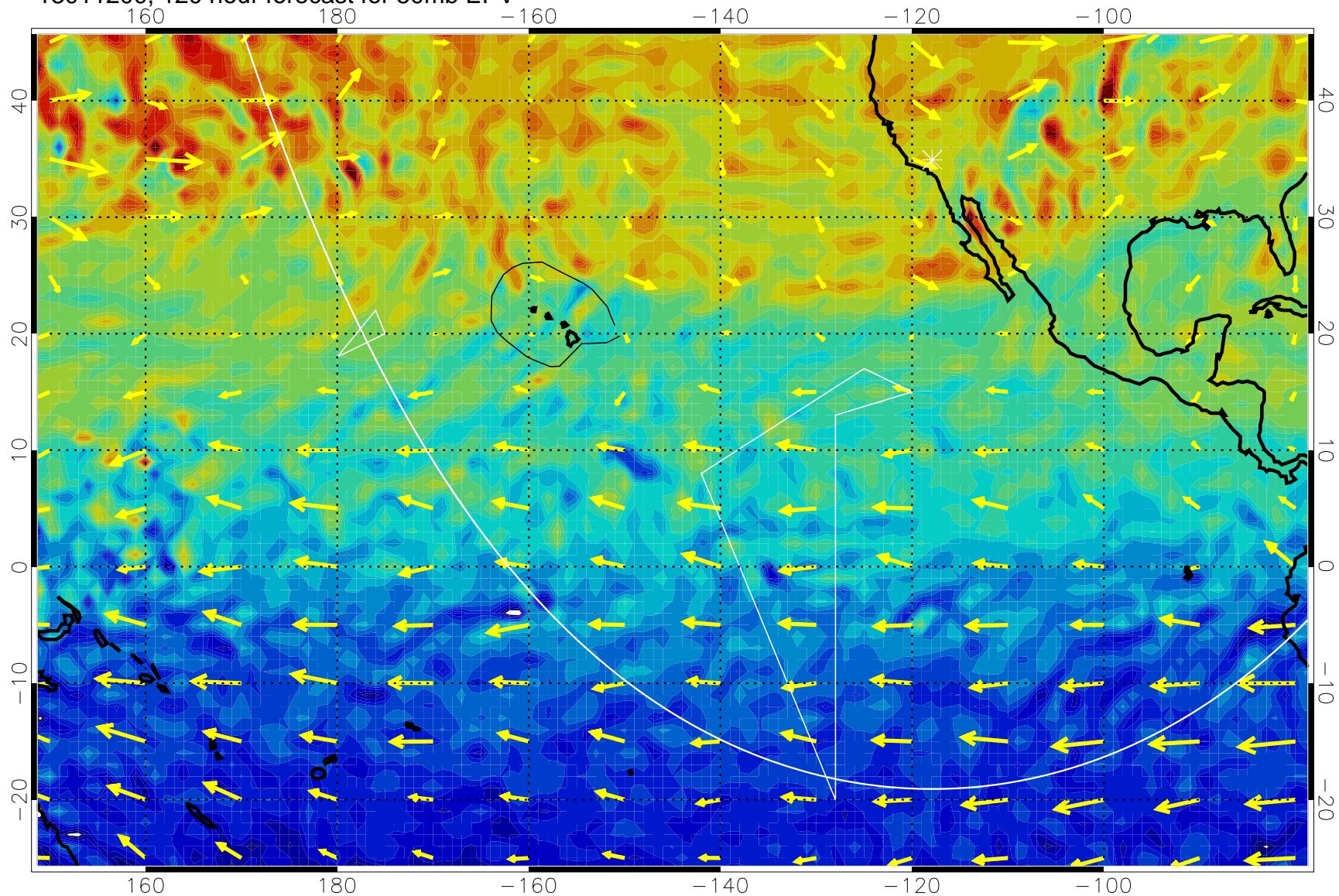
13011200, 120 hour forecast for 50mb EPV
