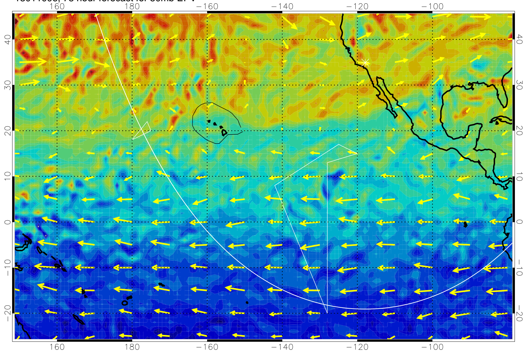
13011006, 78 hour forecast for 50mb EPV
