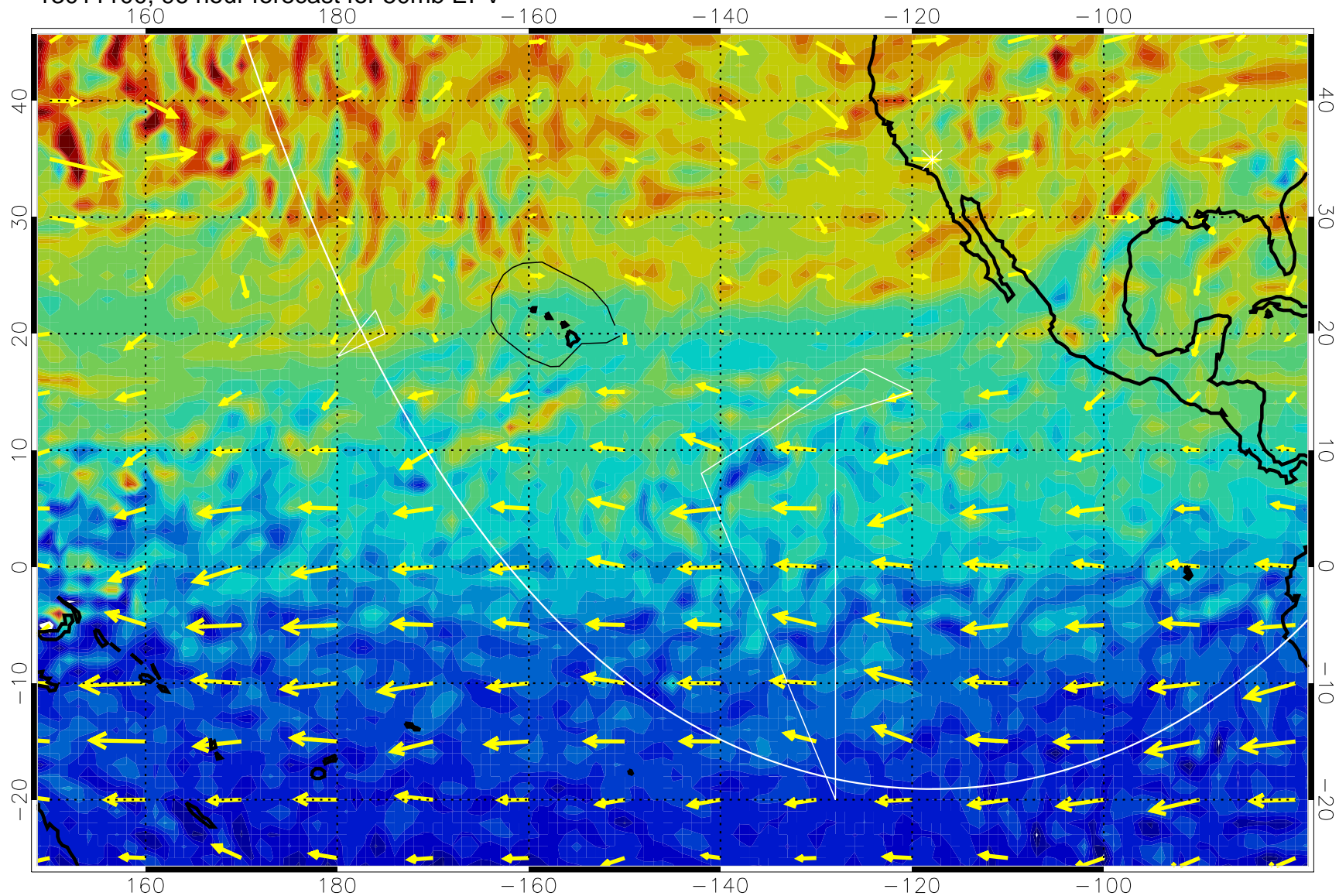
13011100, 96 hour forecast for 50mb EPV
