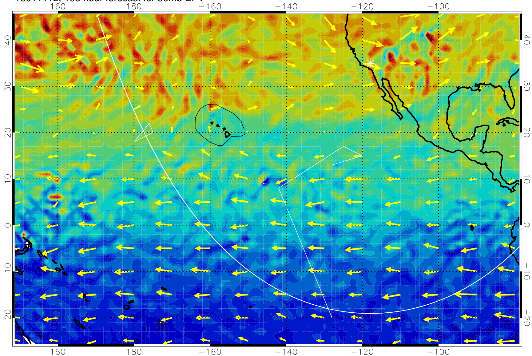
13011112, 108 hour forecast for 50mb EPV
