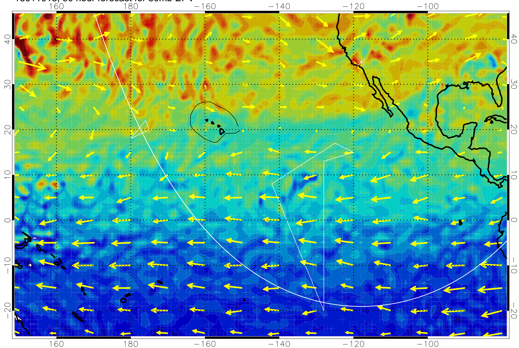
13011018, 90 hour forecast for 50mb EPV
