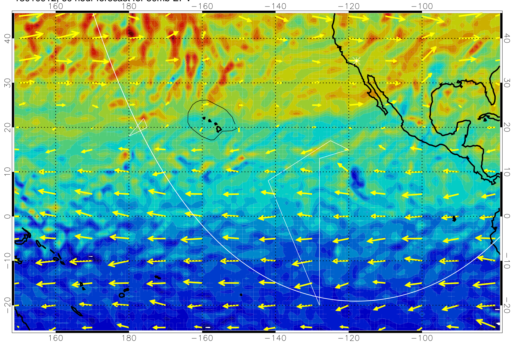
13010912, 60 hour forecast for 50mb EPV
