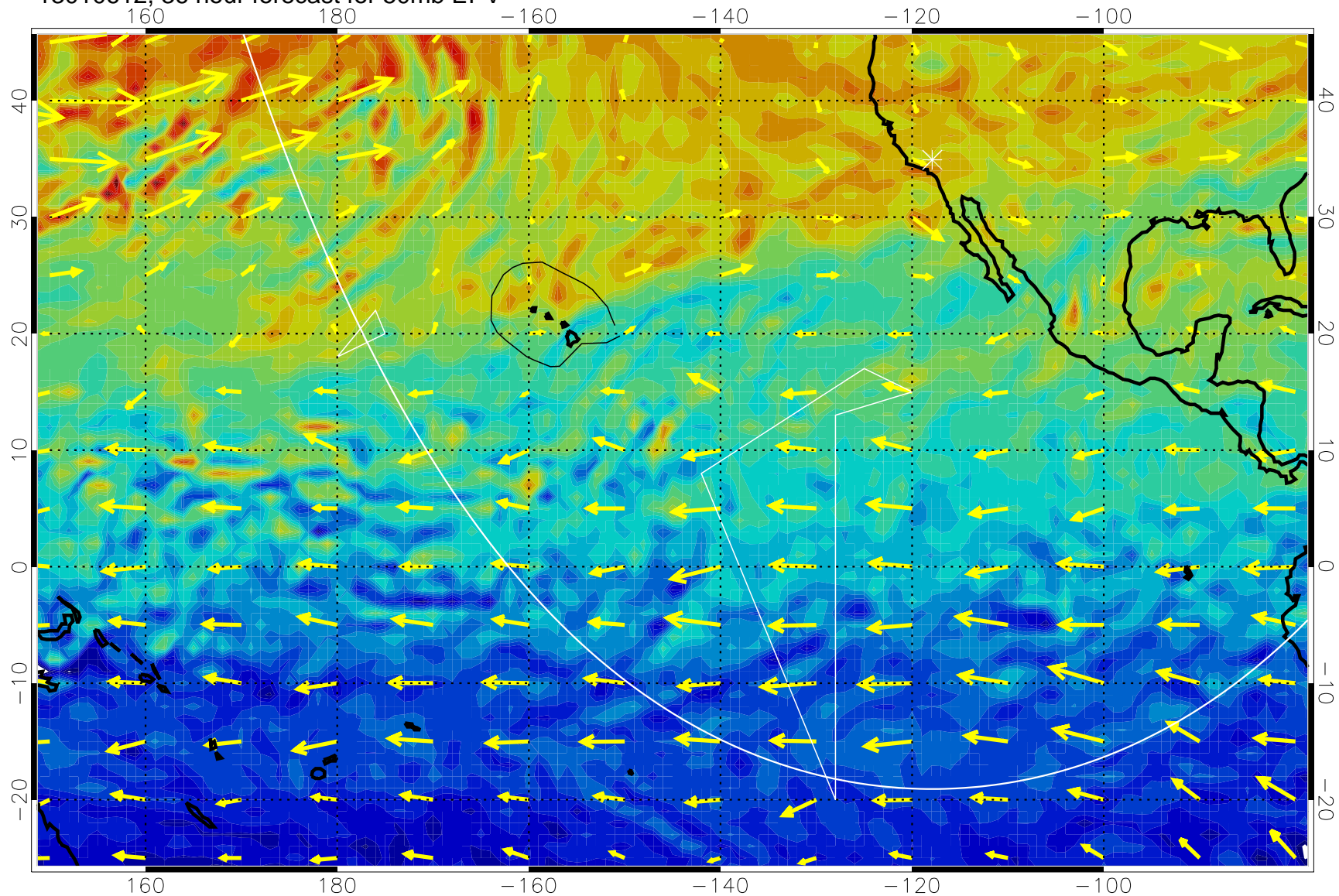
13010612, 36 hour forecast for 50mb EPV
