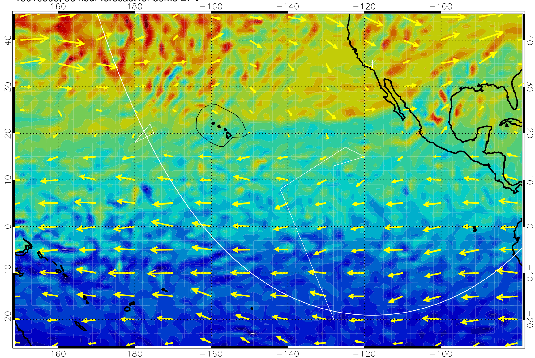
13010900, 96 hour forecast for 50mb EPV
