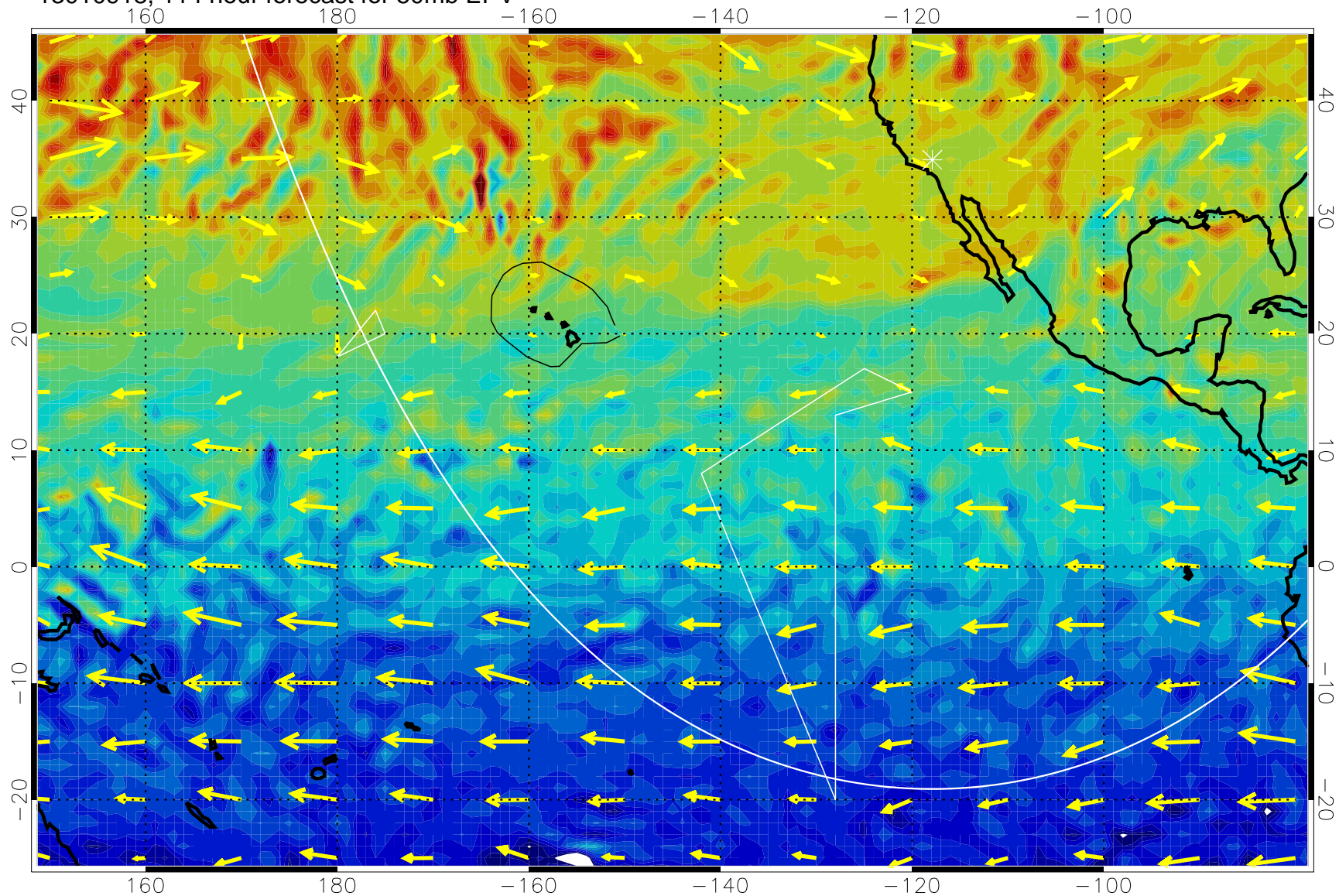
13010918, 114 hour forecast for 50mb EPV
