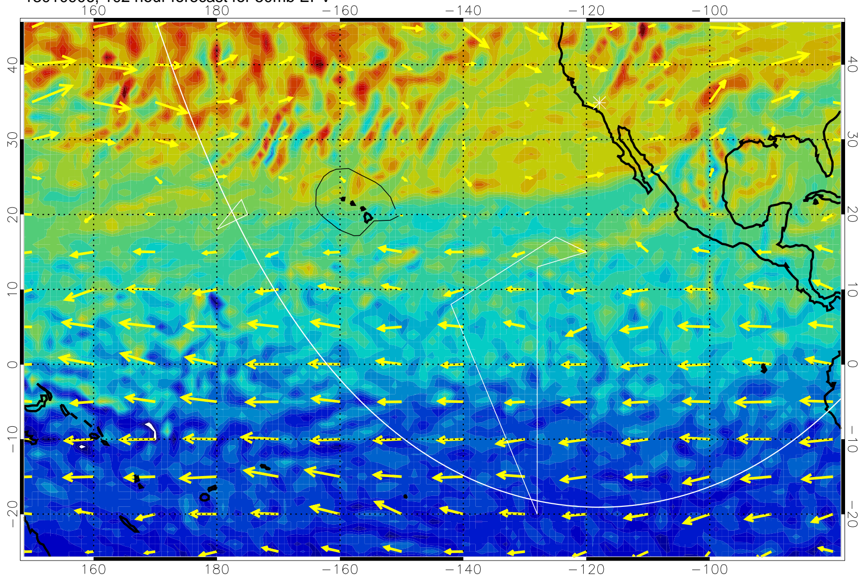
13010906, 102 hour forecast for 50mb EPV
