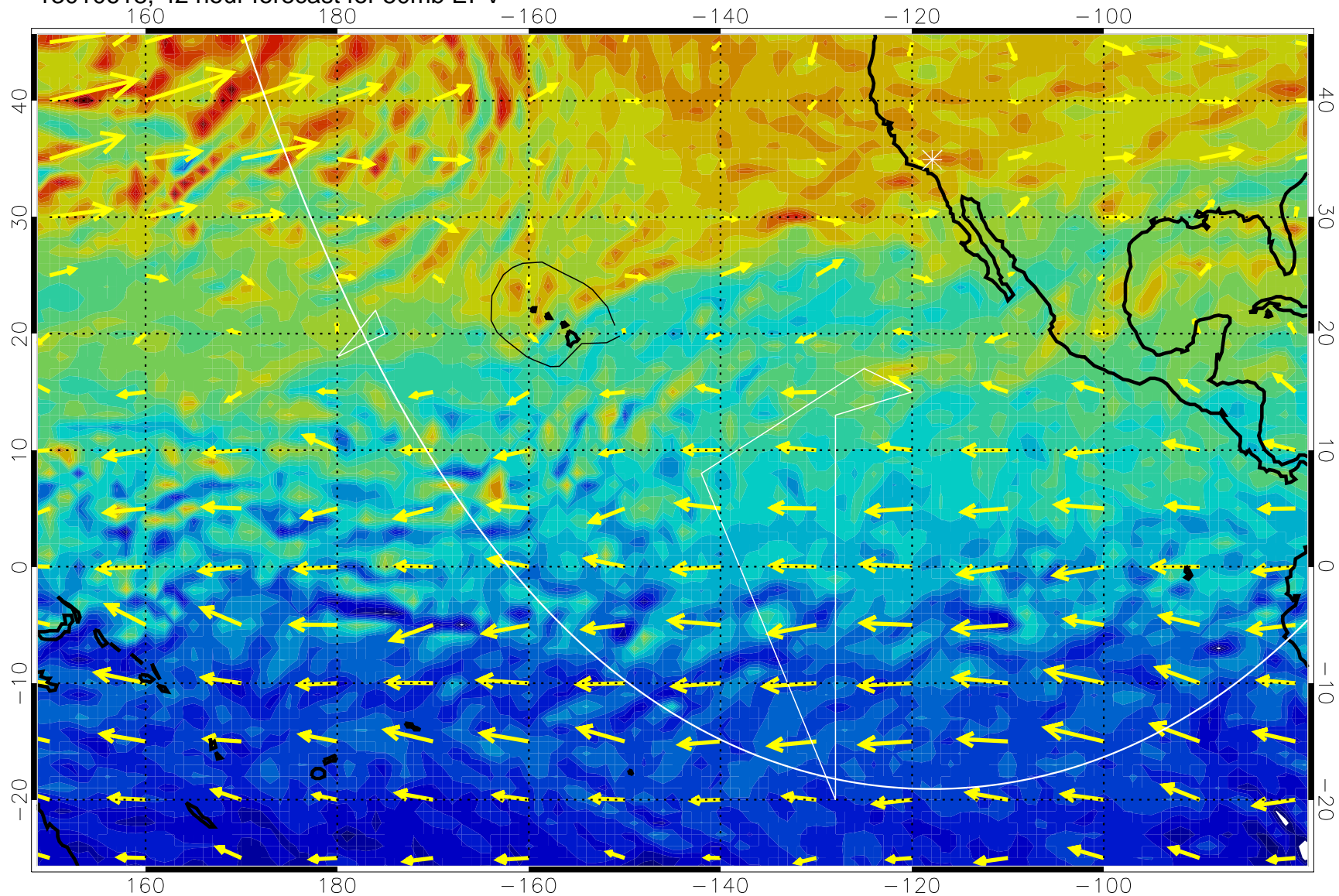
13010618, 42 hour forecast for 50mb EPV
