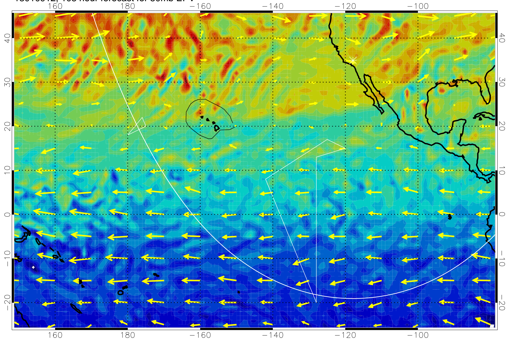
13010912, 108 hour forecast for 50mb EPV
