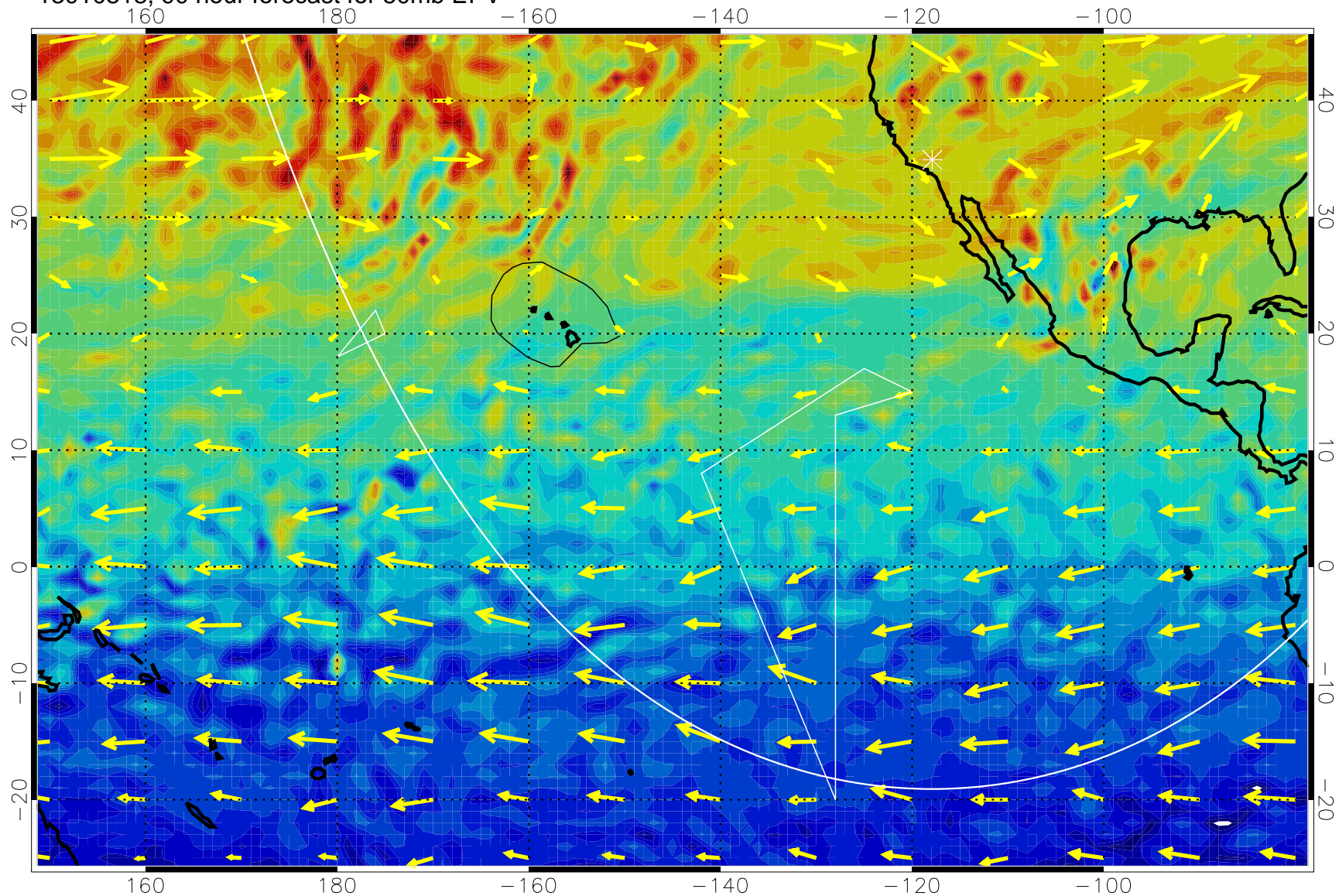
13010818, 90 hour forecast for 50mb EPV
