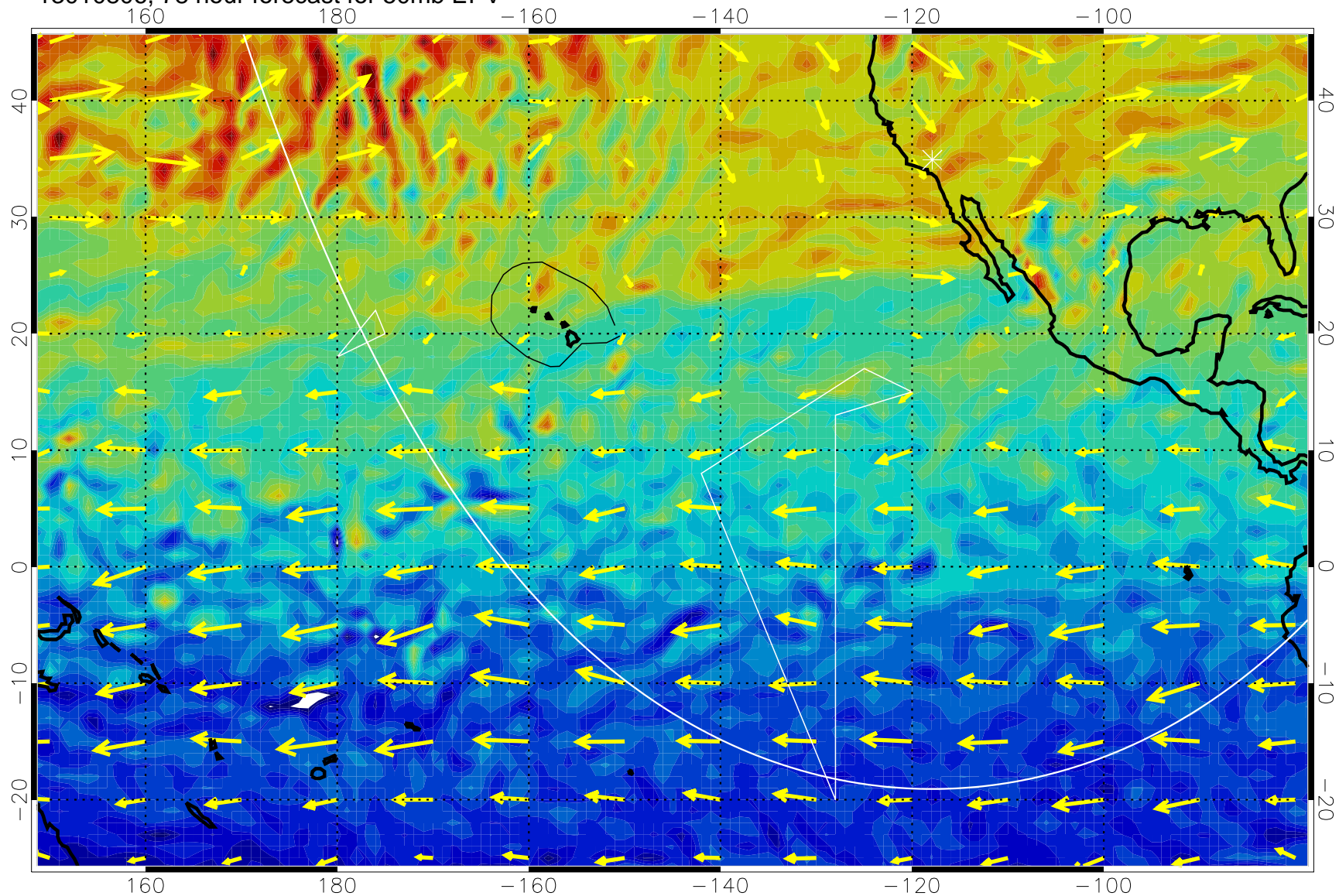
13010806, 78 hour forecast for 50mb EPV
