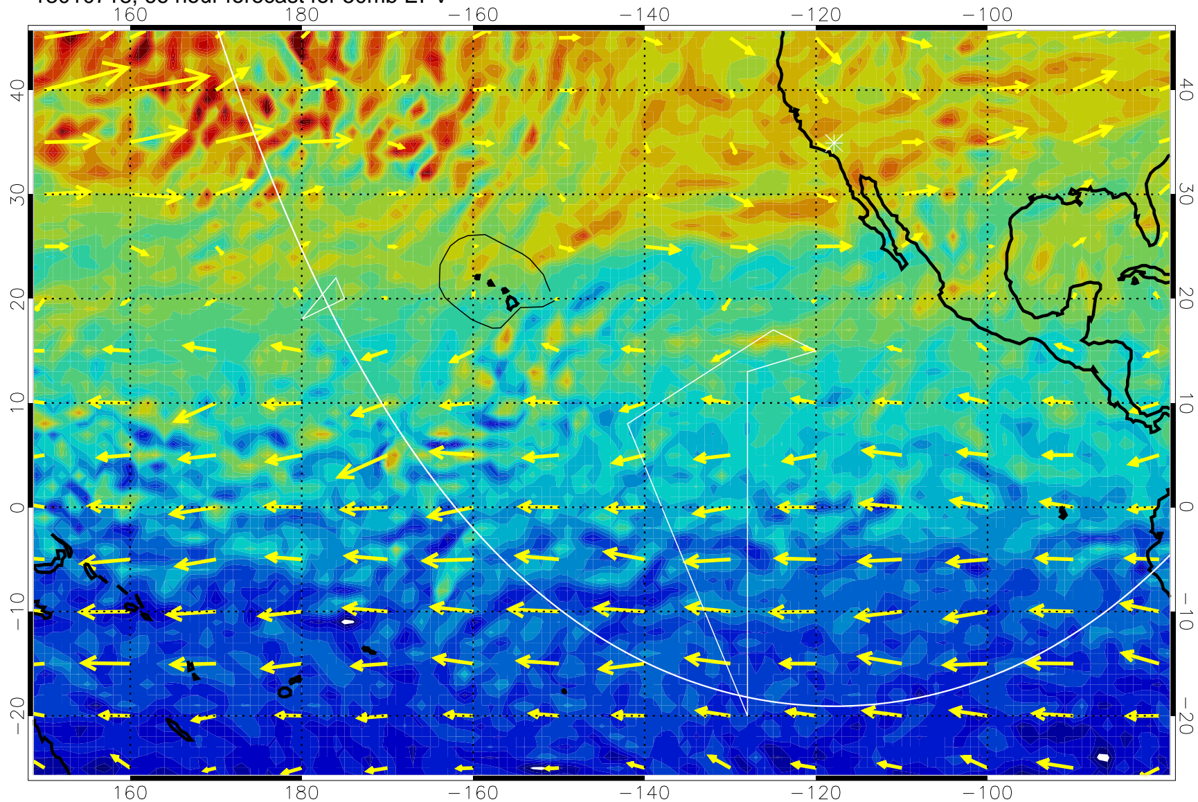
13010718, 66 hour forecast for 50mb EPV
