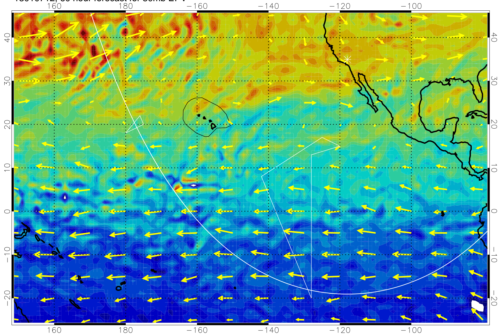
13010712, 60 hour forecast for 50mb EPV
