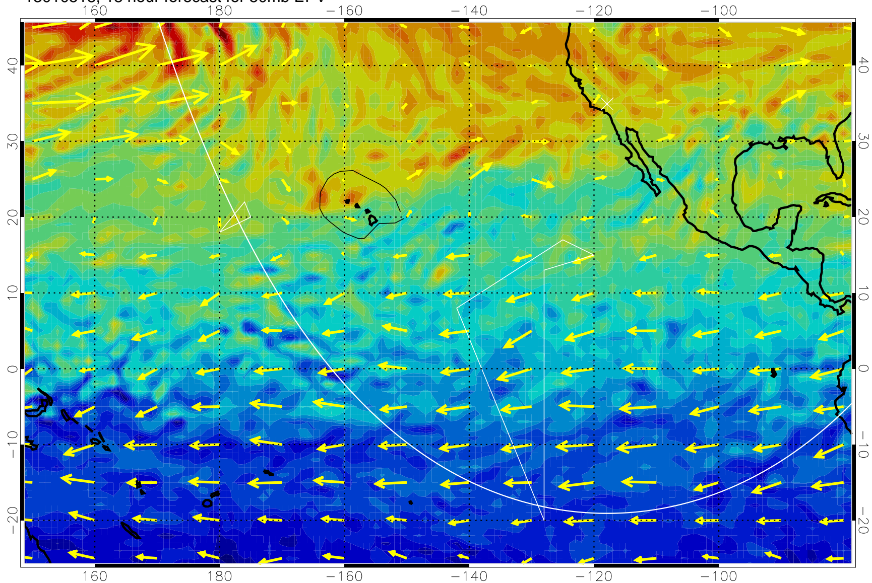
13010518, 18 hour forecast for 50mb EPV
