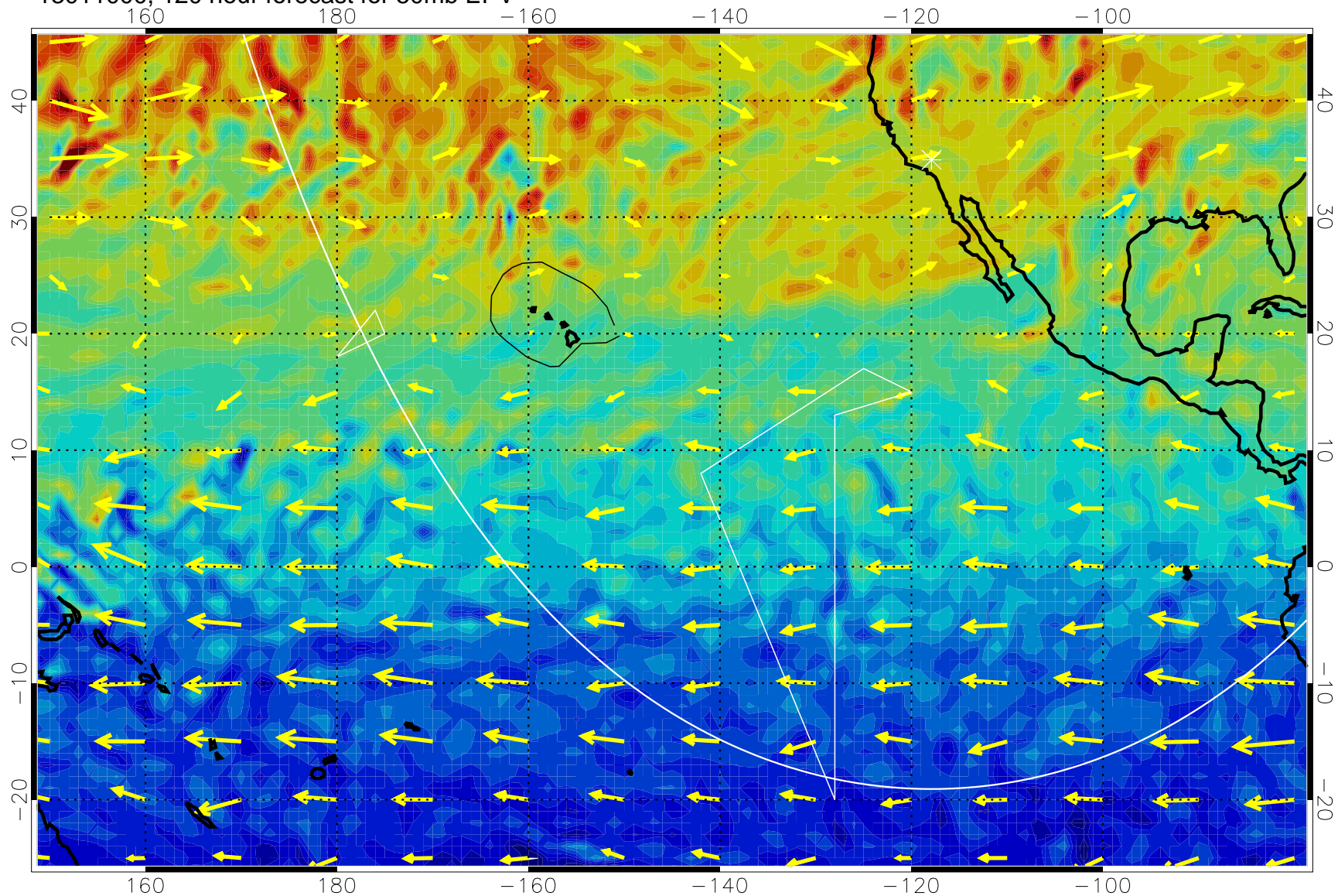
13011000, 120 hour forecast for 50mb EPV
