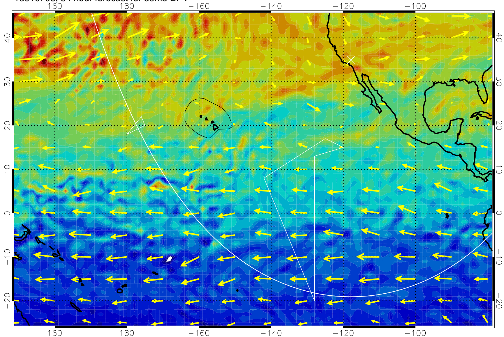
13010706, 54 hour forecast for 50mb EPV
