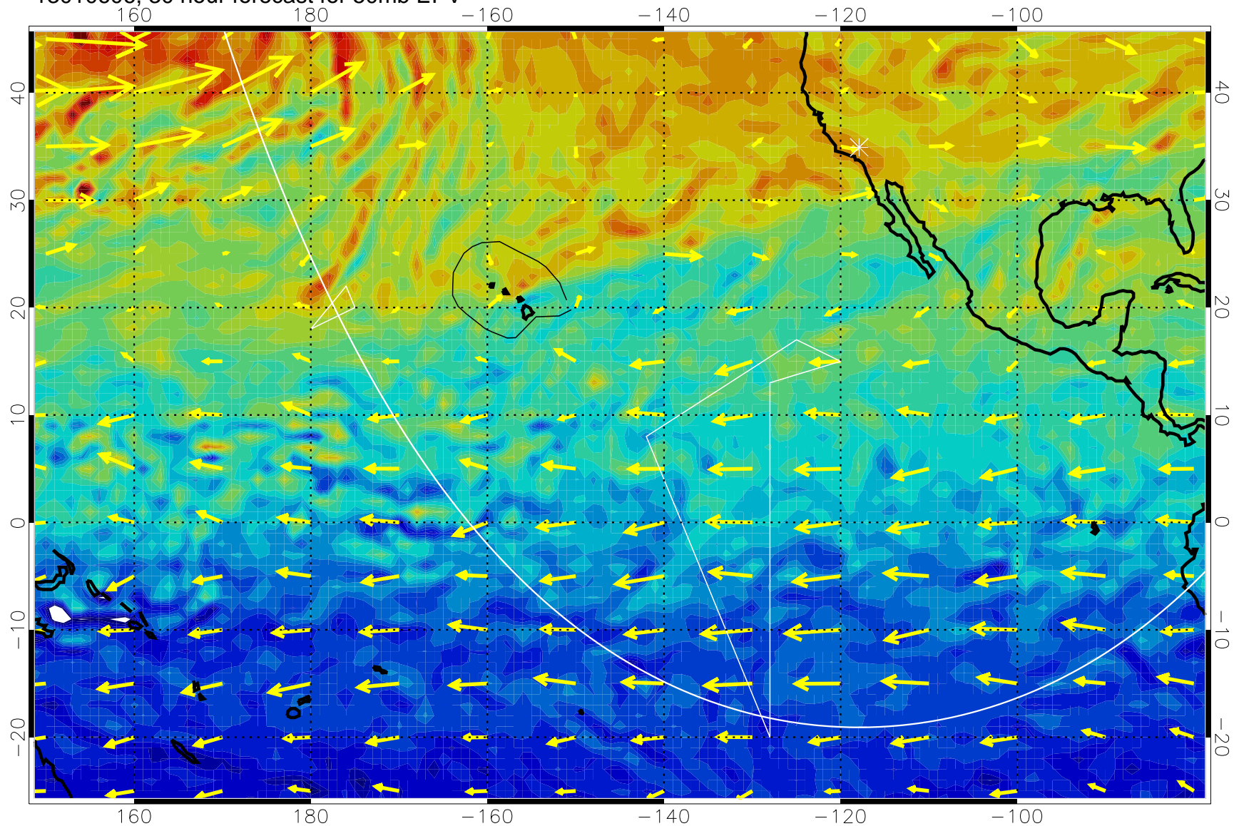
13010606, 30 hour forecast for 50mb EPV
