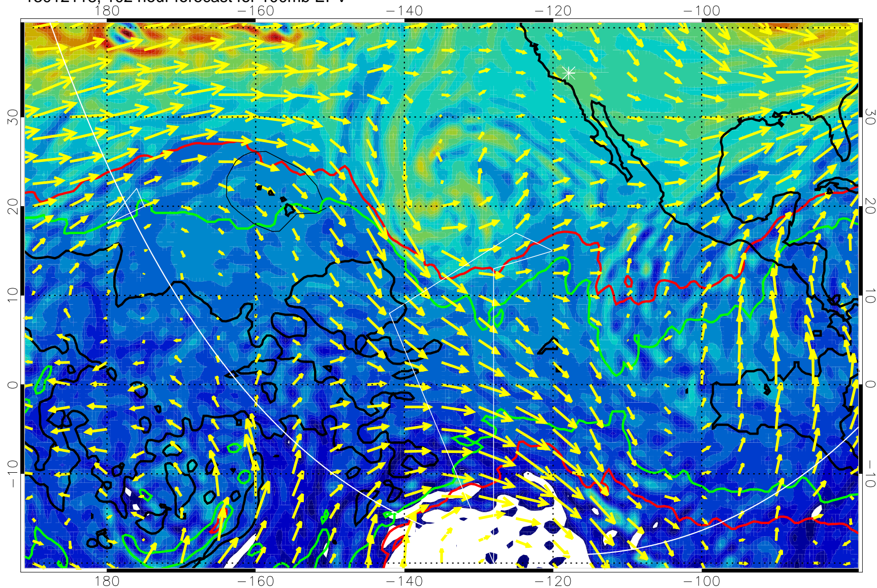
13012118, 102 hour forecast for 100mb EPV
