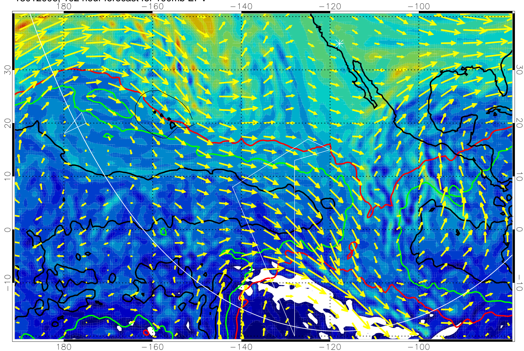
13012006, 102 hour forecast for 100mb EPV
