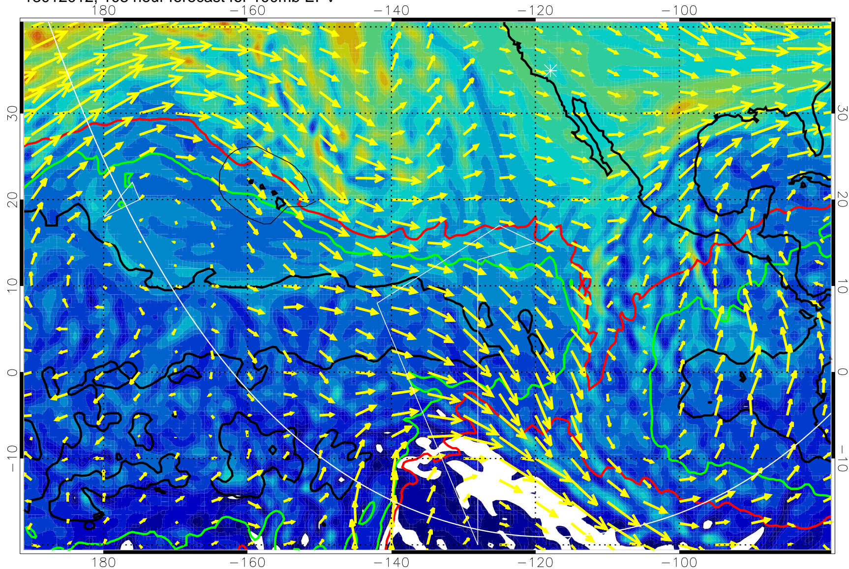
13012012, 108 hour forecast for 100mb EPV
