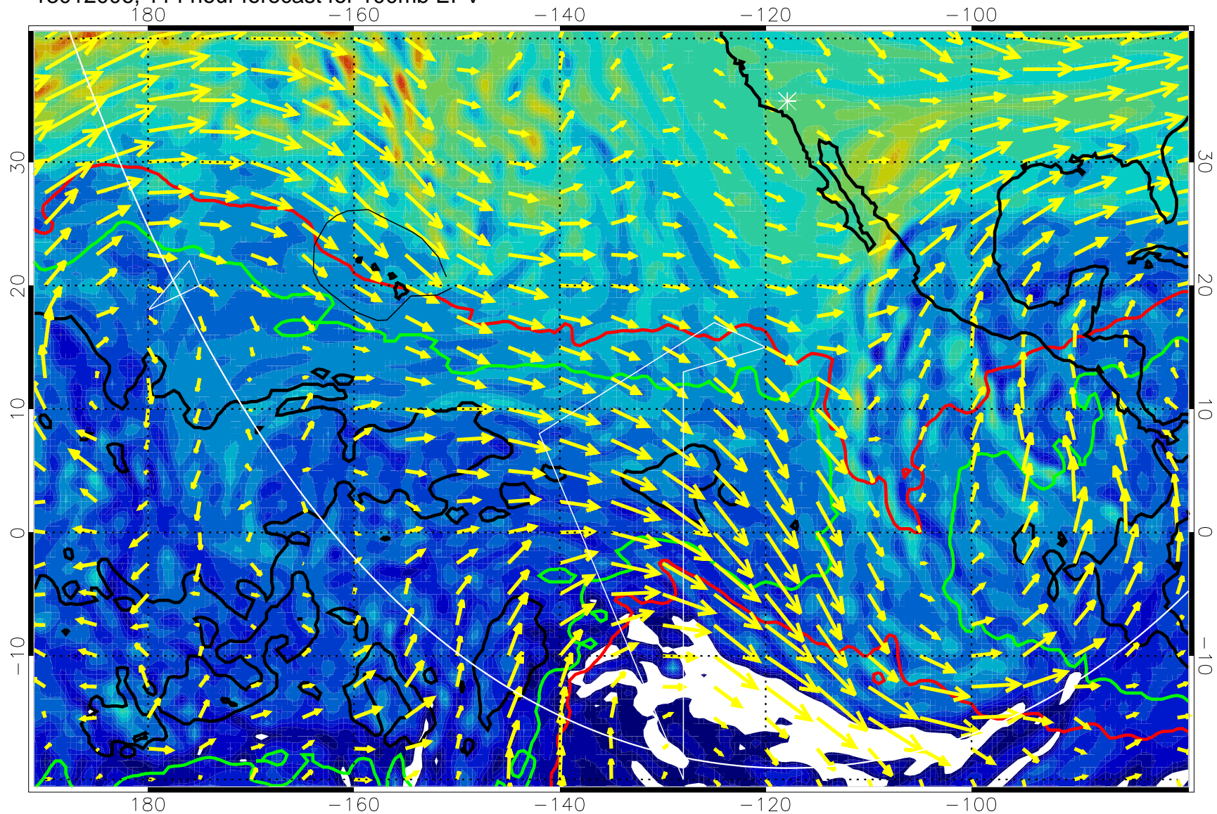
13012006, 114 hour forecast for 100mb EPV
