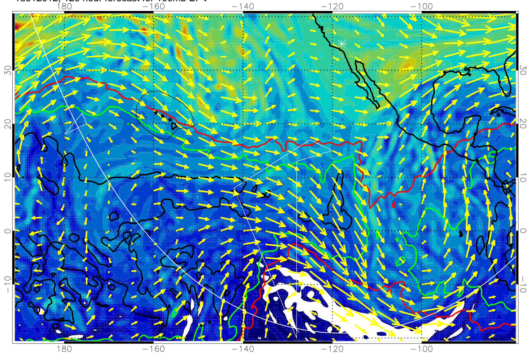
13012012, 120 hour forecast for 100mb EPV
