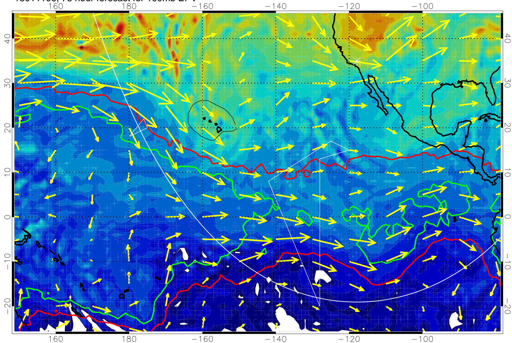
13011106, 78 hour forecast for 100mb EPV
