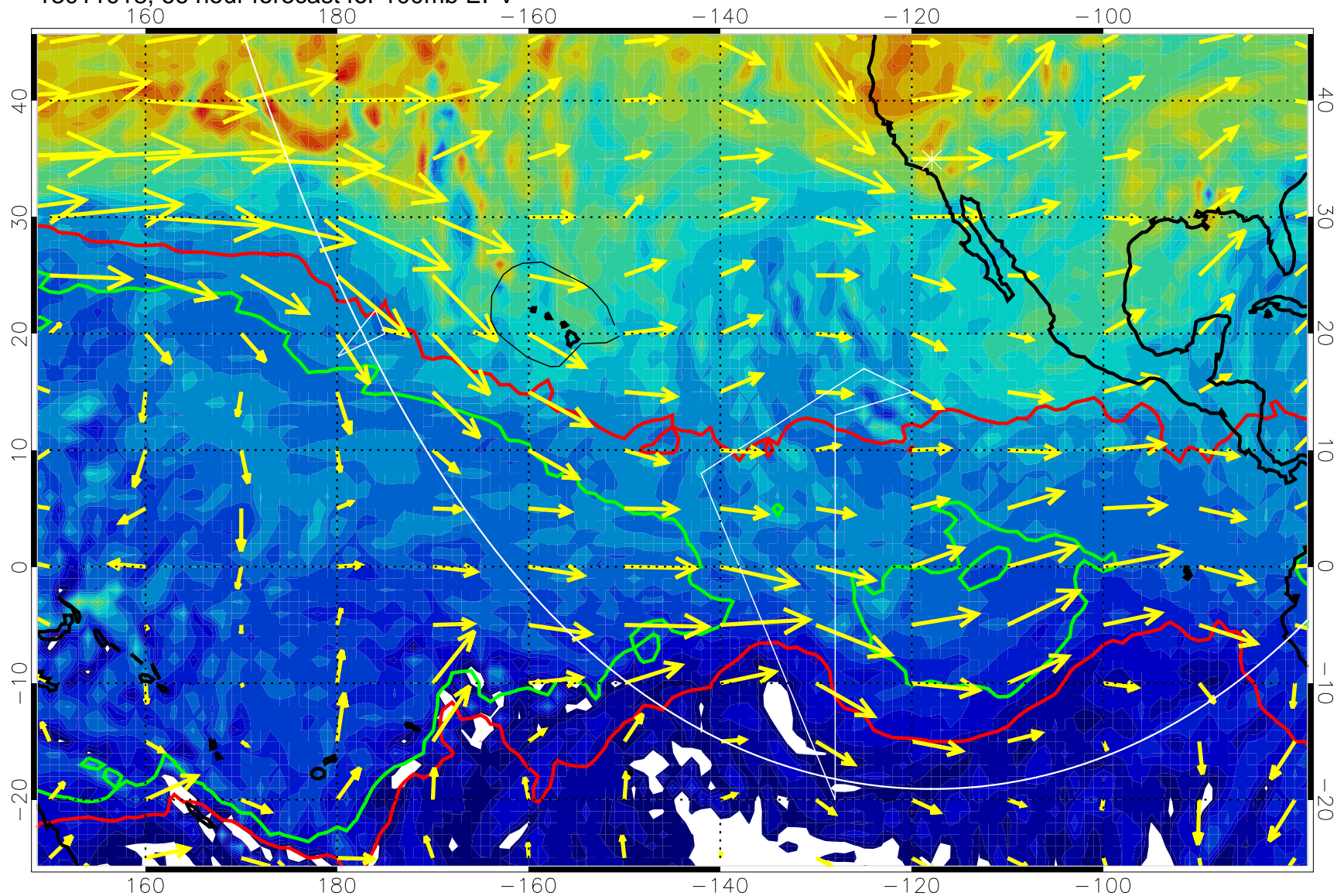
13011018, 66 hour forecast for 100mb EPV
