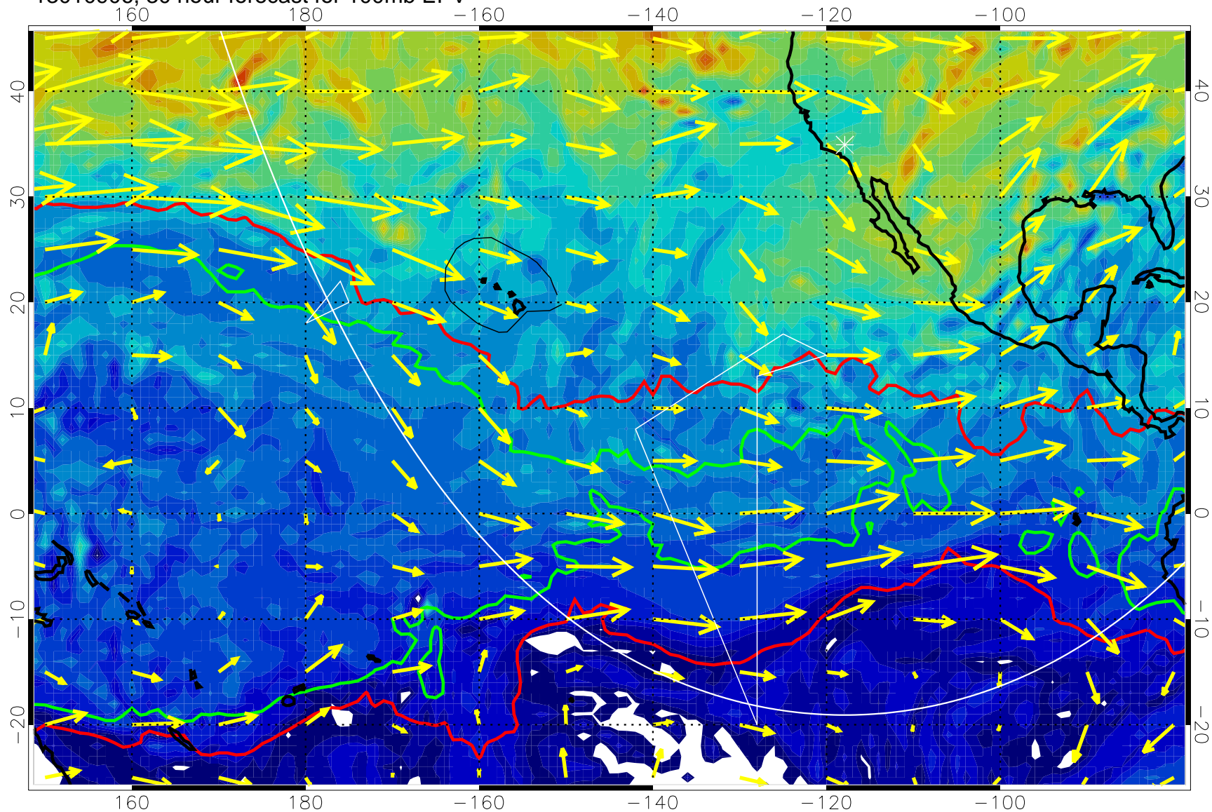
13010906, 30 hour forecast for 100mb EPV
