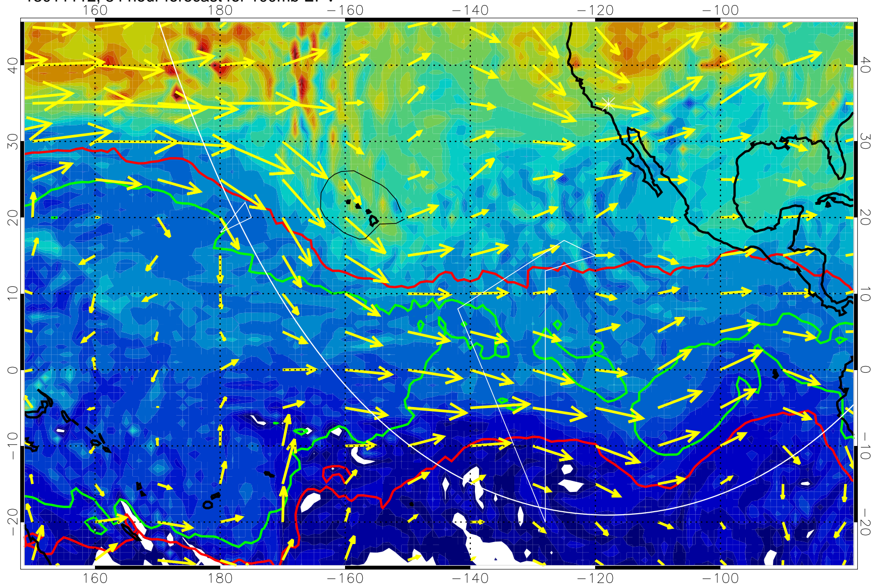
13011112, 84 hour forecast for 100mb EPV
