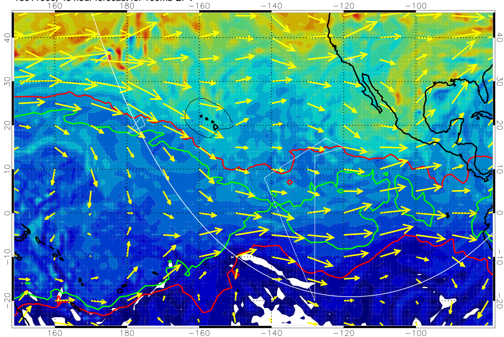
13011000, 48 hour forecast for 100mb EPV
