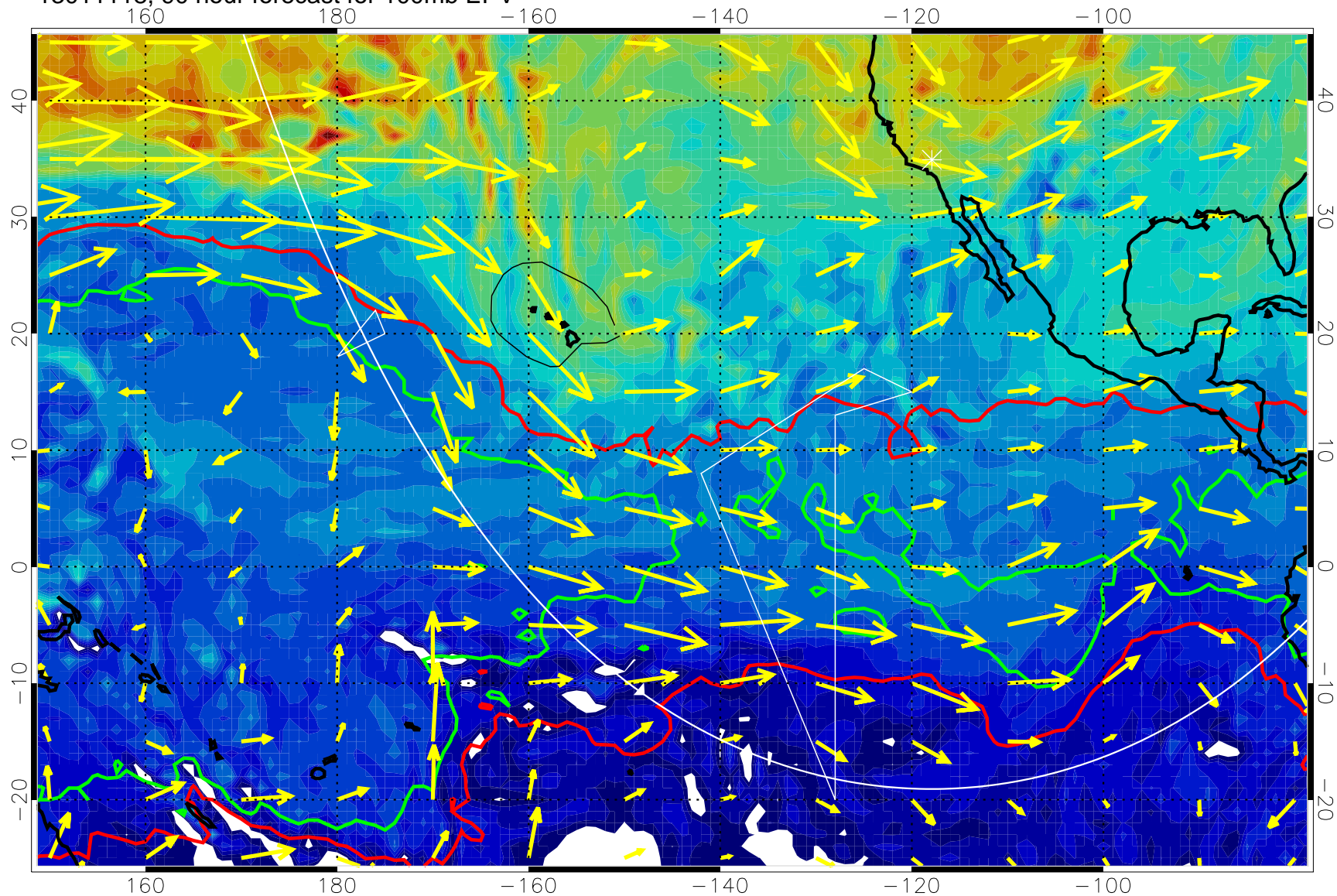
13011118, 90 hour forecast for 100mb EPV
