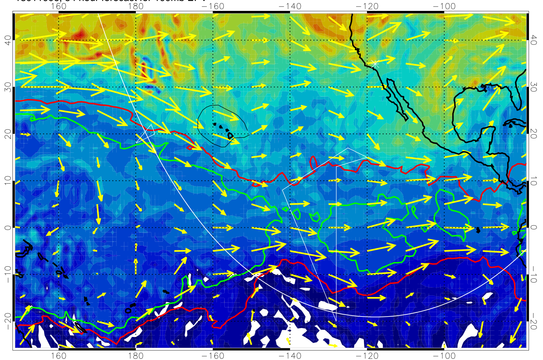
13011006, 54 hour forecast for 100mb EPV
