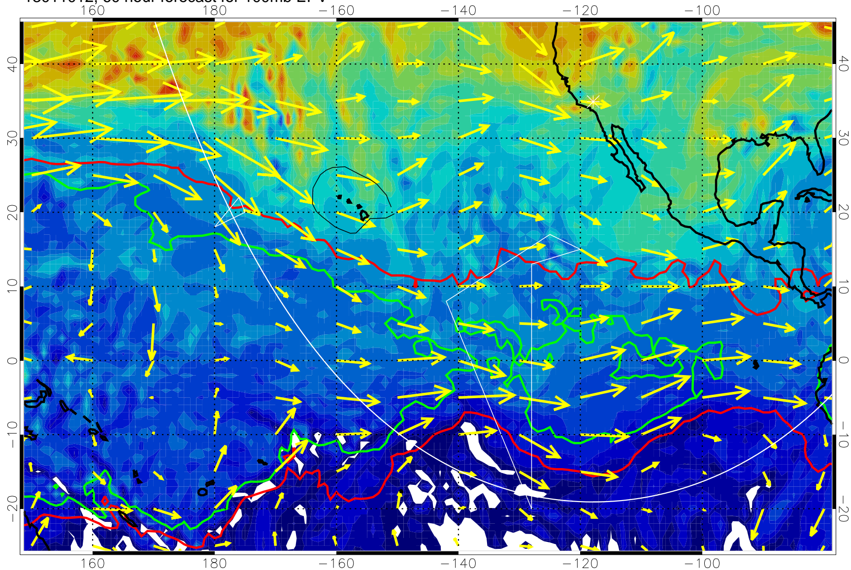
13011012, 60 hour forecast for 100mb EPV
