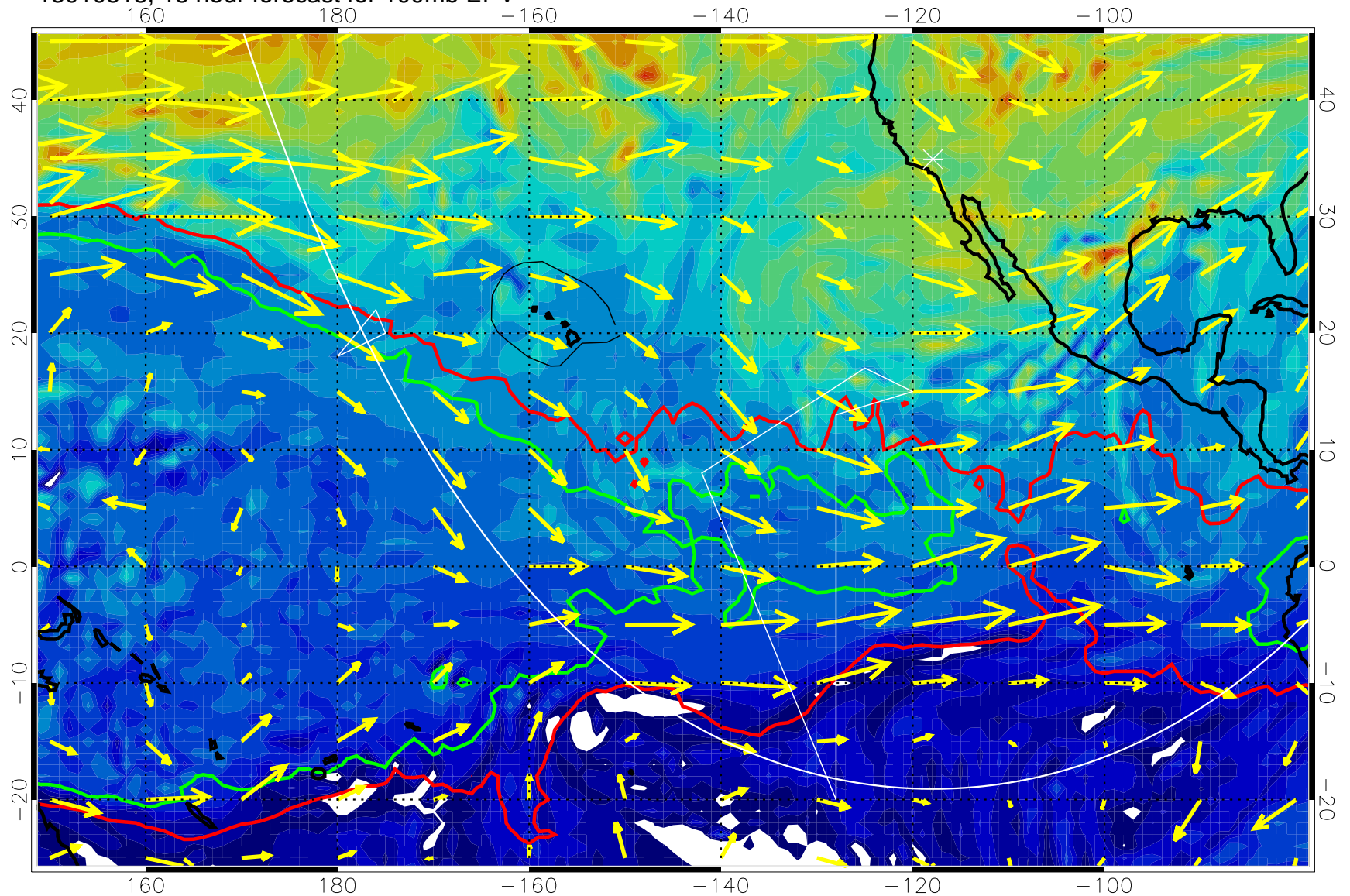
13010818, 18 hour forecast for 100mb EPV
