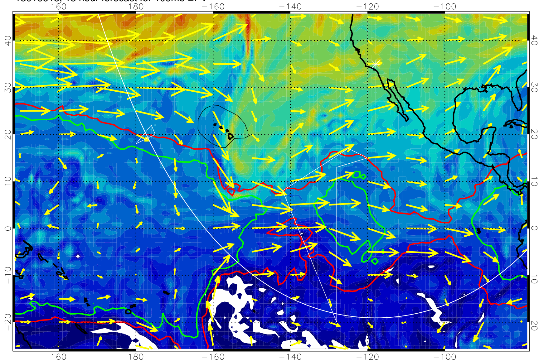
13010618, 18 hour forecast for 100mb EPV
