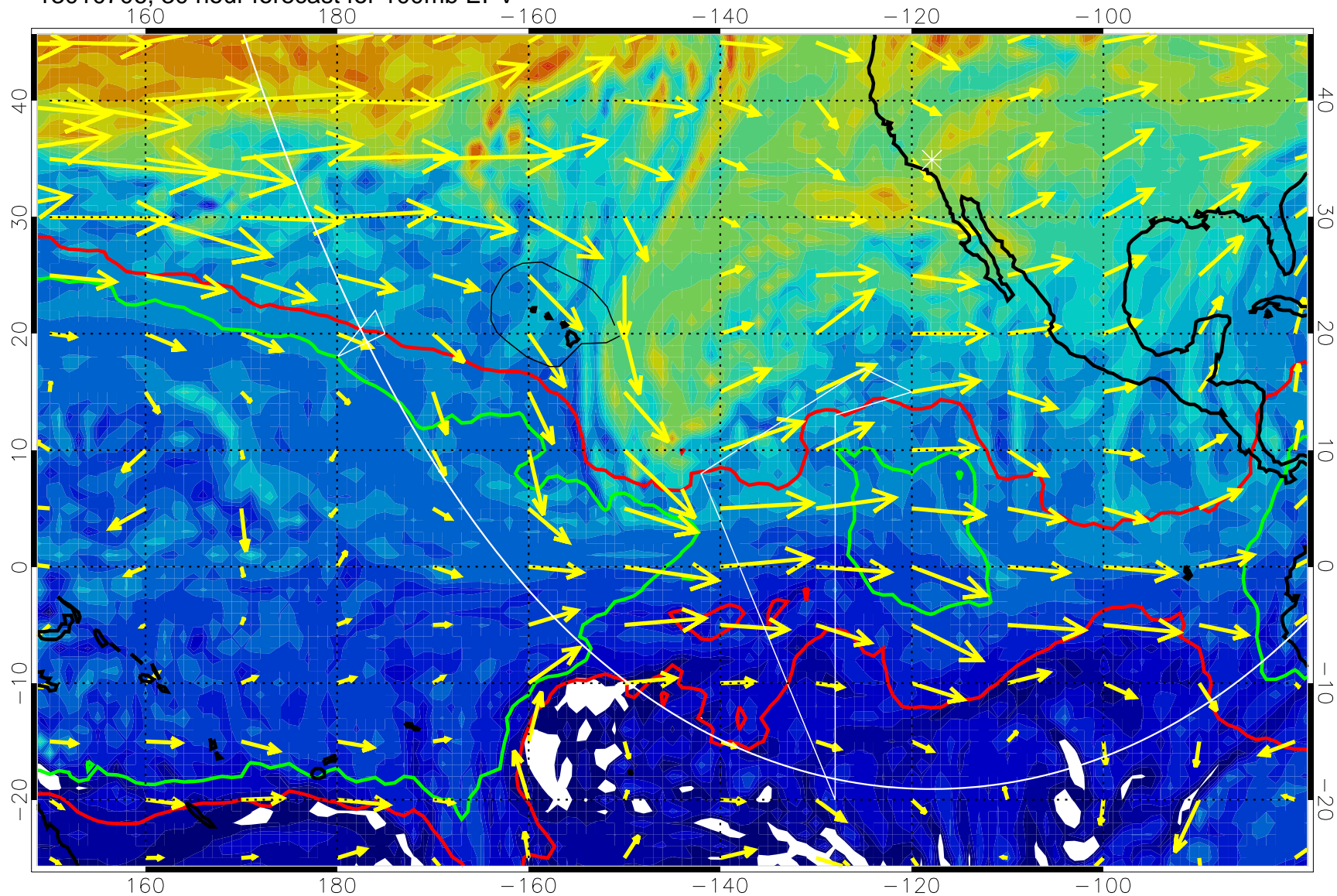
13010706, 30 hour forecast for 100mb EPV
