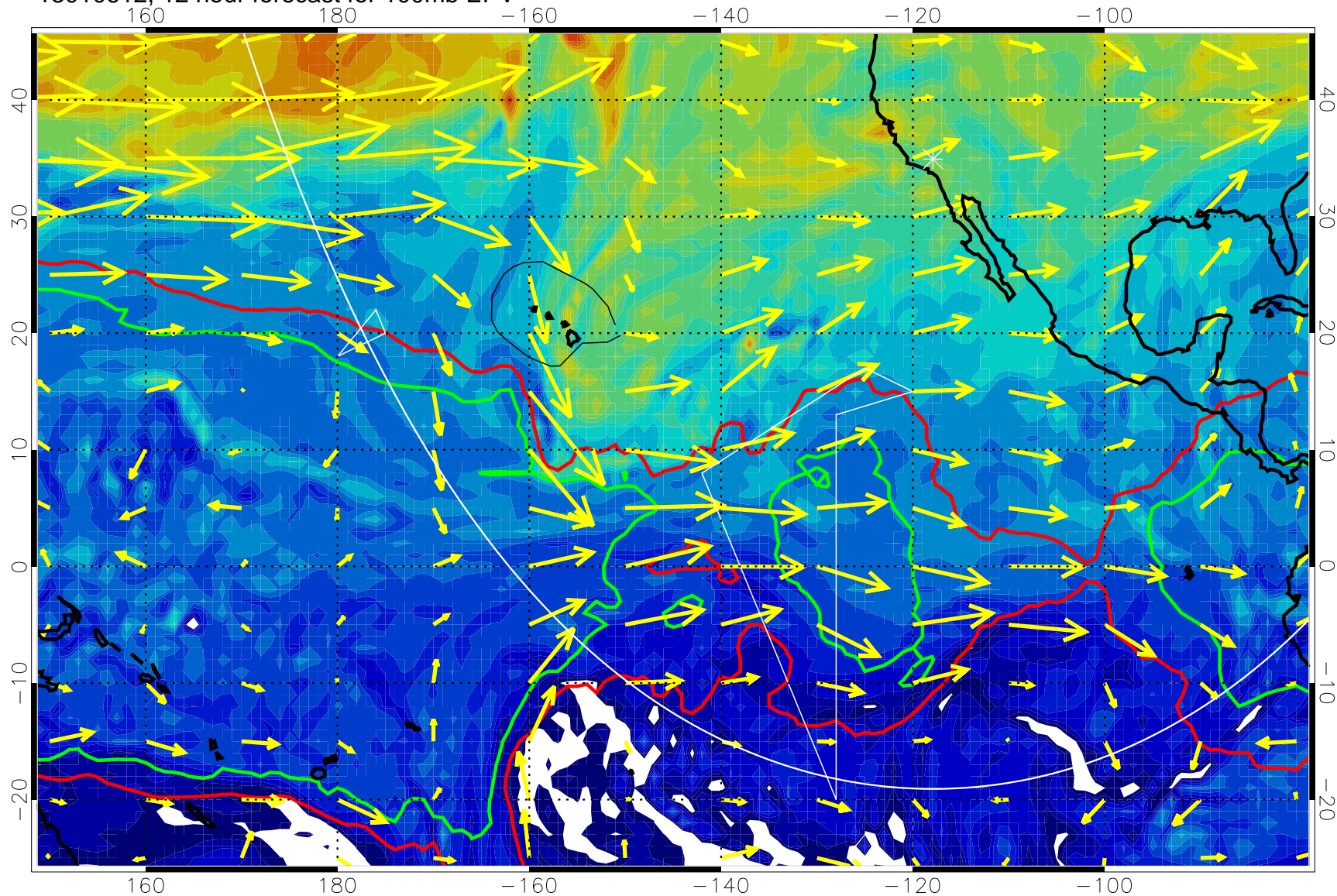
13010612, 12 hour forecast for 100mb EPV
