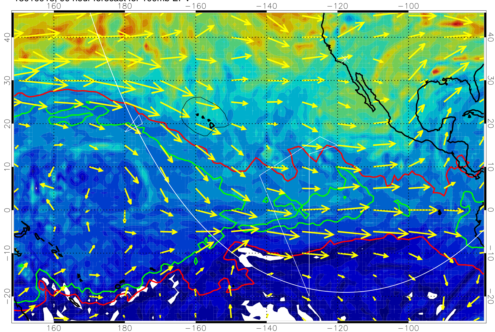
13010918, 90 hour forecast for 100mb EPV
