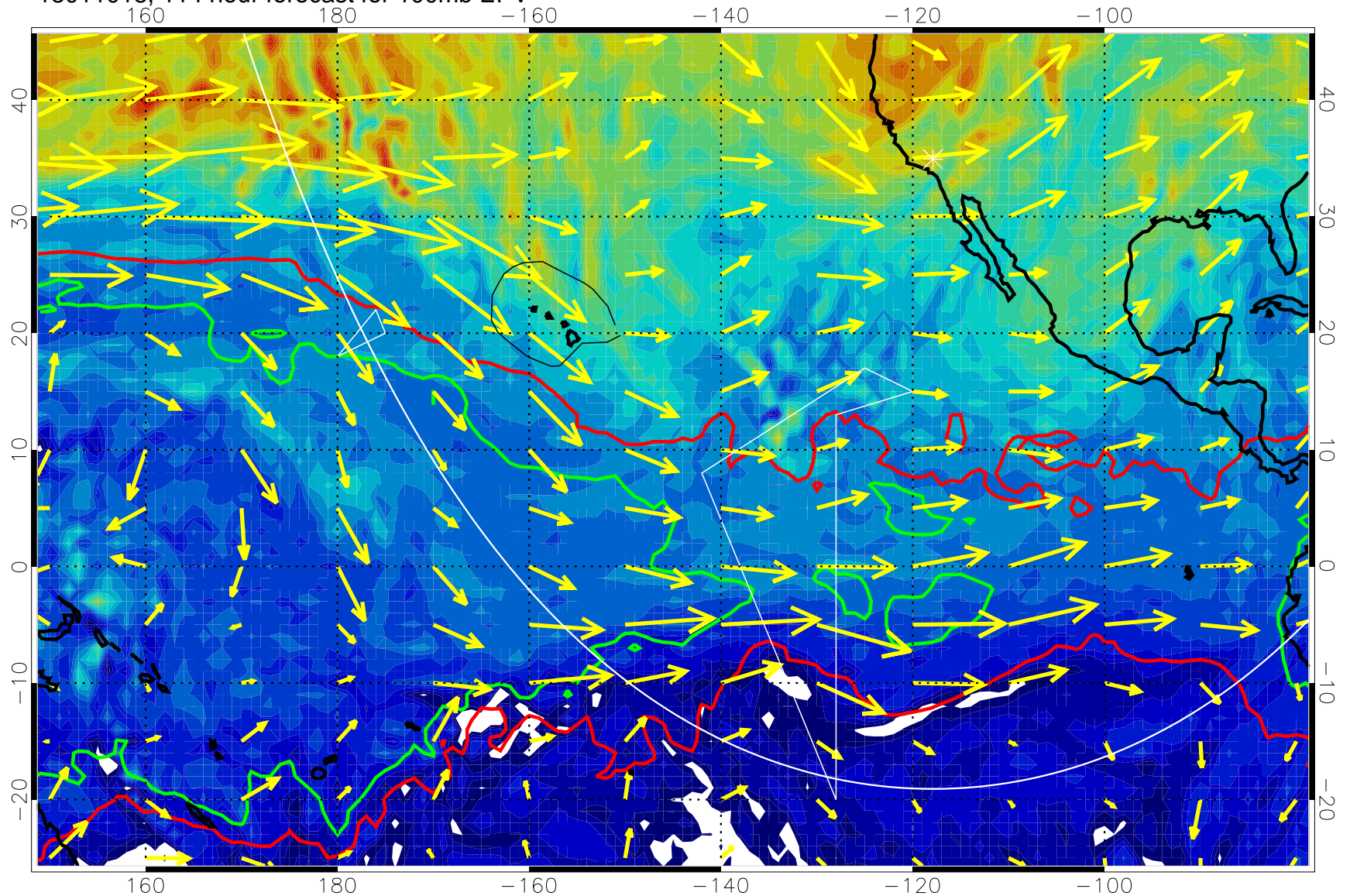
13011018, 114 hour forecast for 100mb EPV
