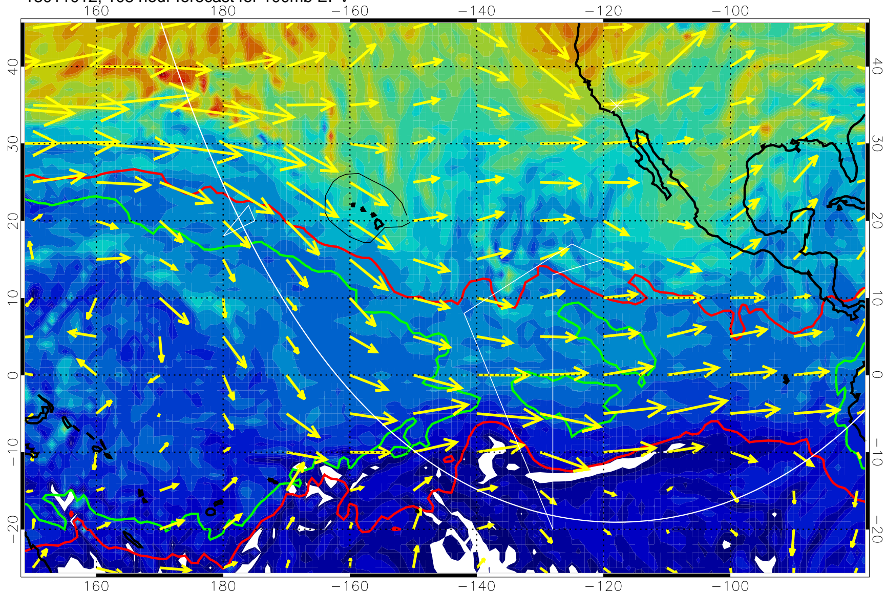
13011012, 108 hour forecast for 100mb EPV
