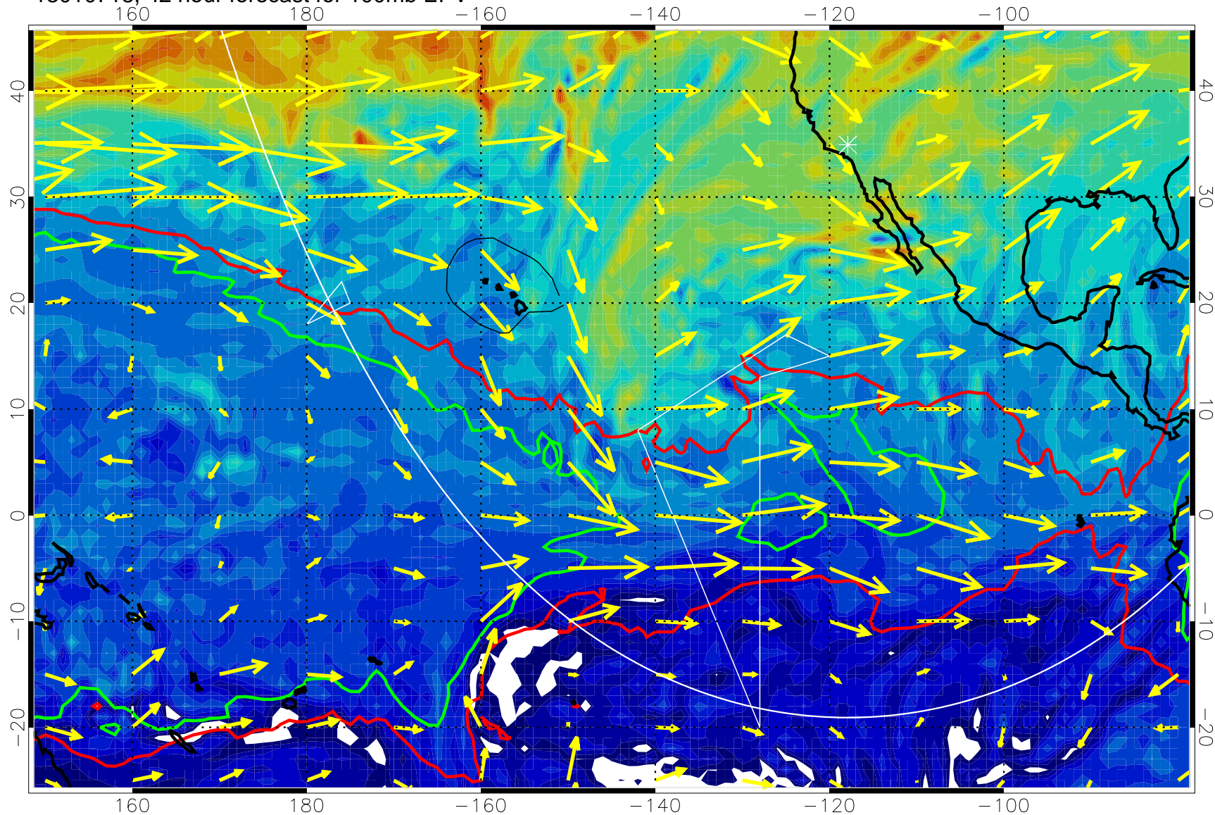
13010718, 42 hour forecast for 100mb EPV
