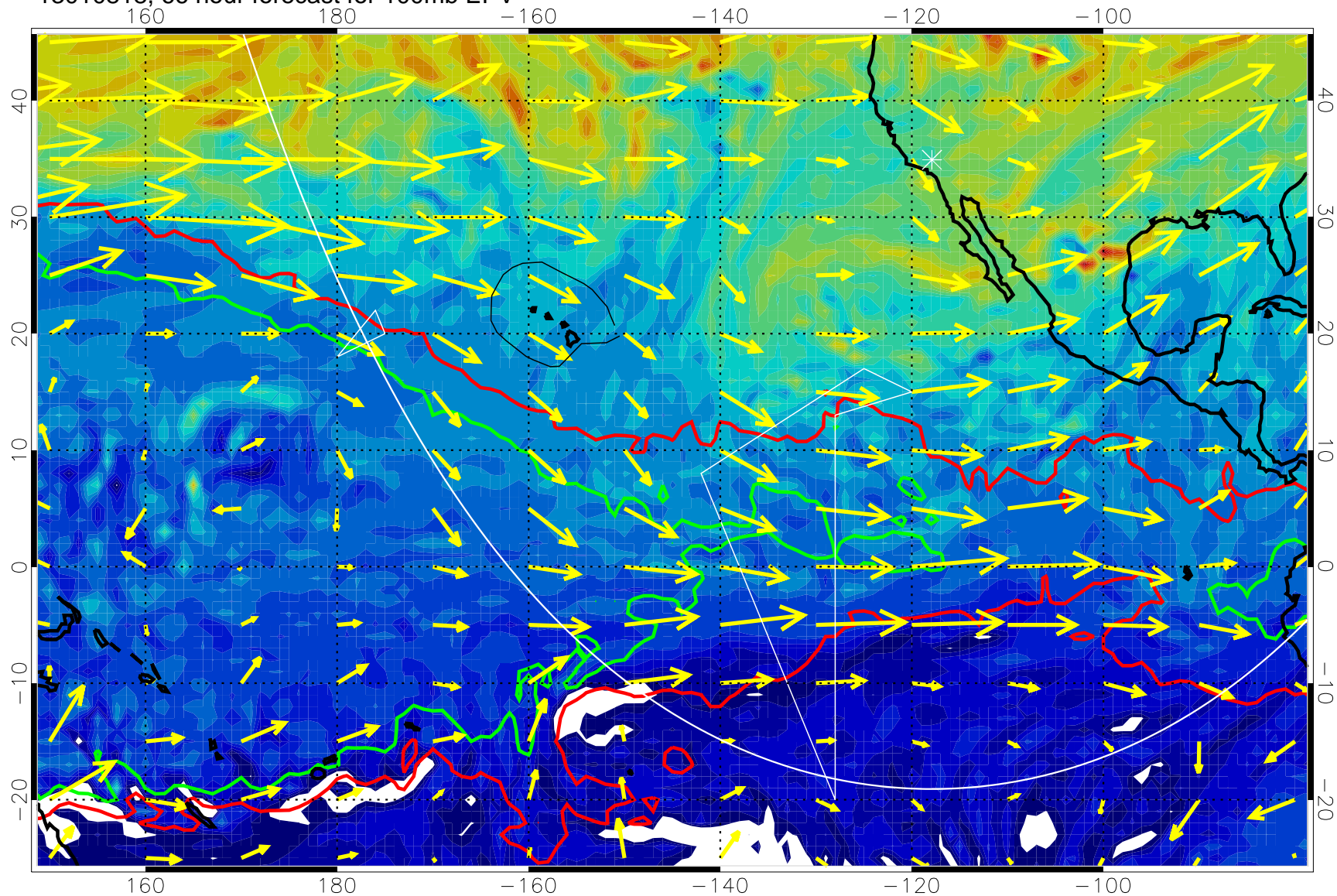
13010818, 66 hour forecast for 100mb EPV
