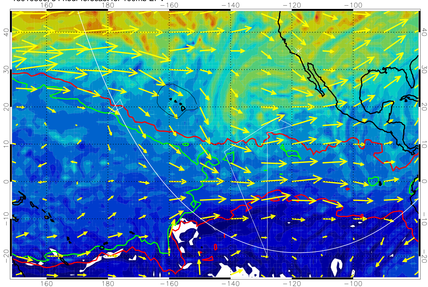
13010806, 54 hour forecast for 100mb EPV
