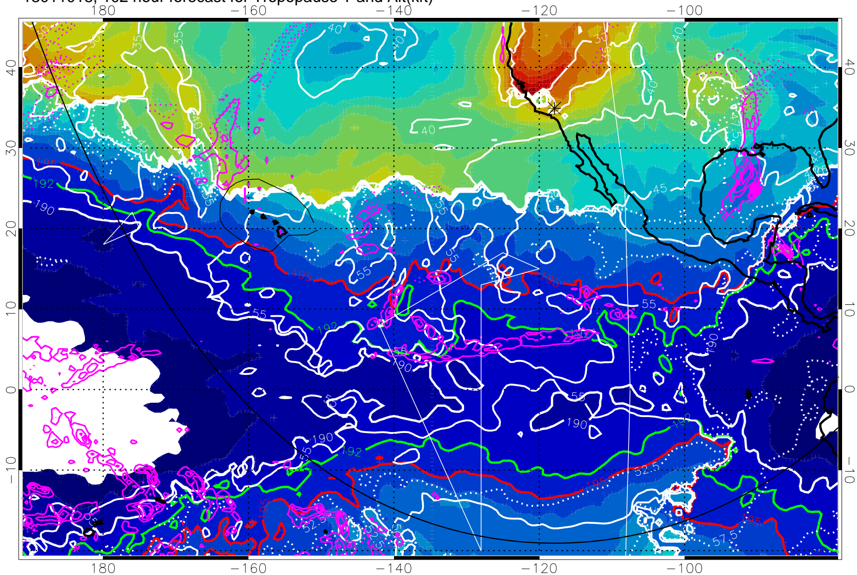
13011018, 102 hour forecast for Tropopause T and Alt(kft)
