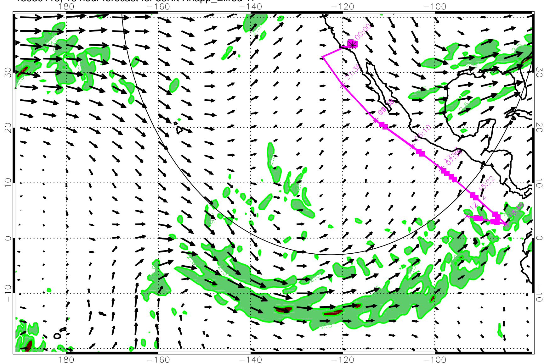
13030118, 18 hour forecast for 53Kft Knapp_Ellrod TI
