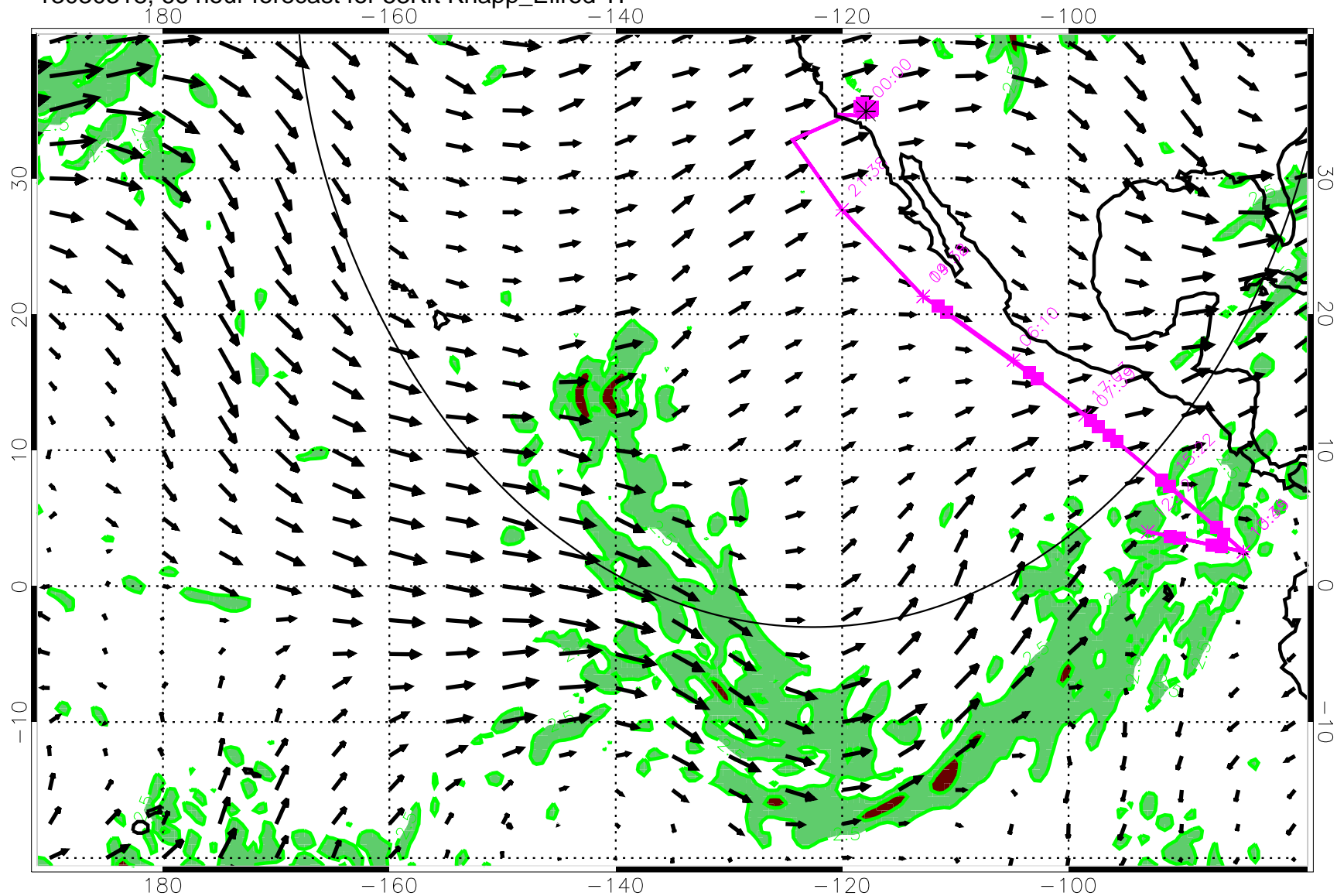
13030318, 66 hour forecast for 53Kft Knapp_Ellrod TI
