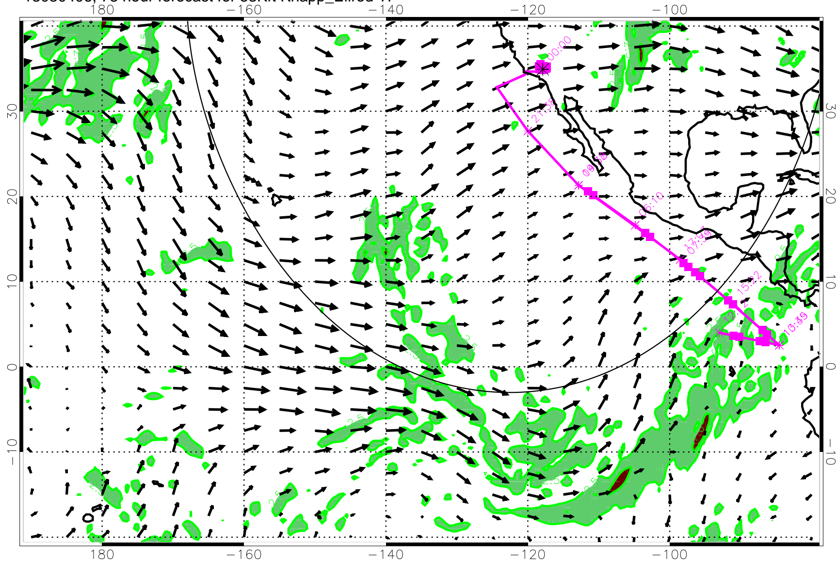
13030406, 78 hour forecast for 53Kft Knapp_Ellrod TI
