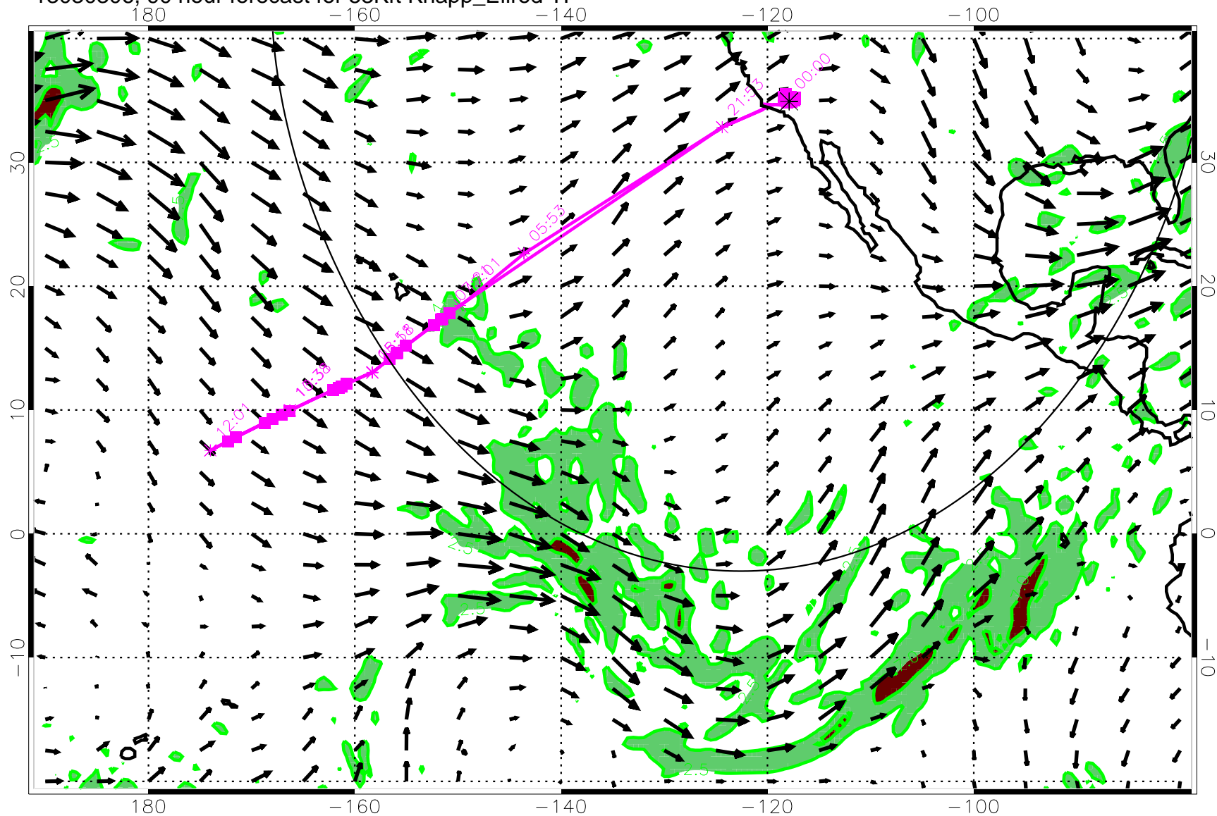
13030306, 90 hour forecast for 53Kft Knapp_Ellrod TI
