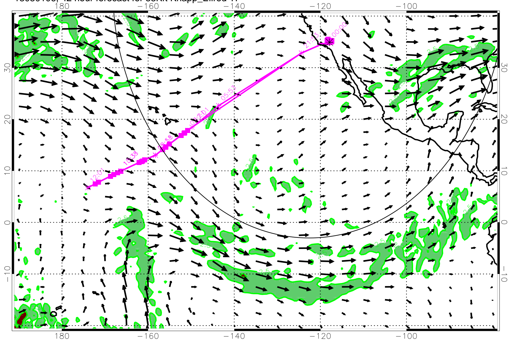
13030106, 42 hour forecast for 53Kft Knapp_Ellrod TI
