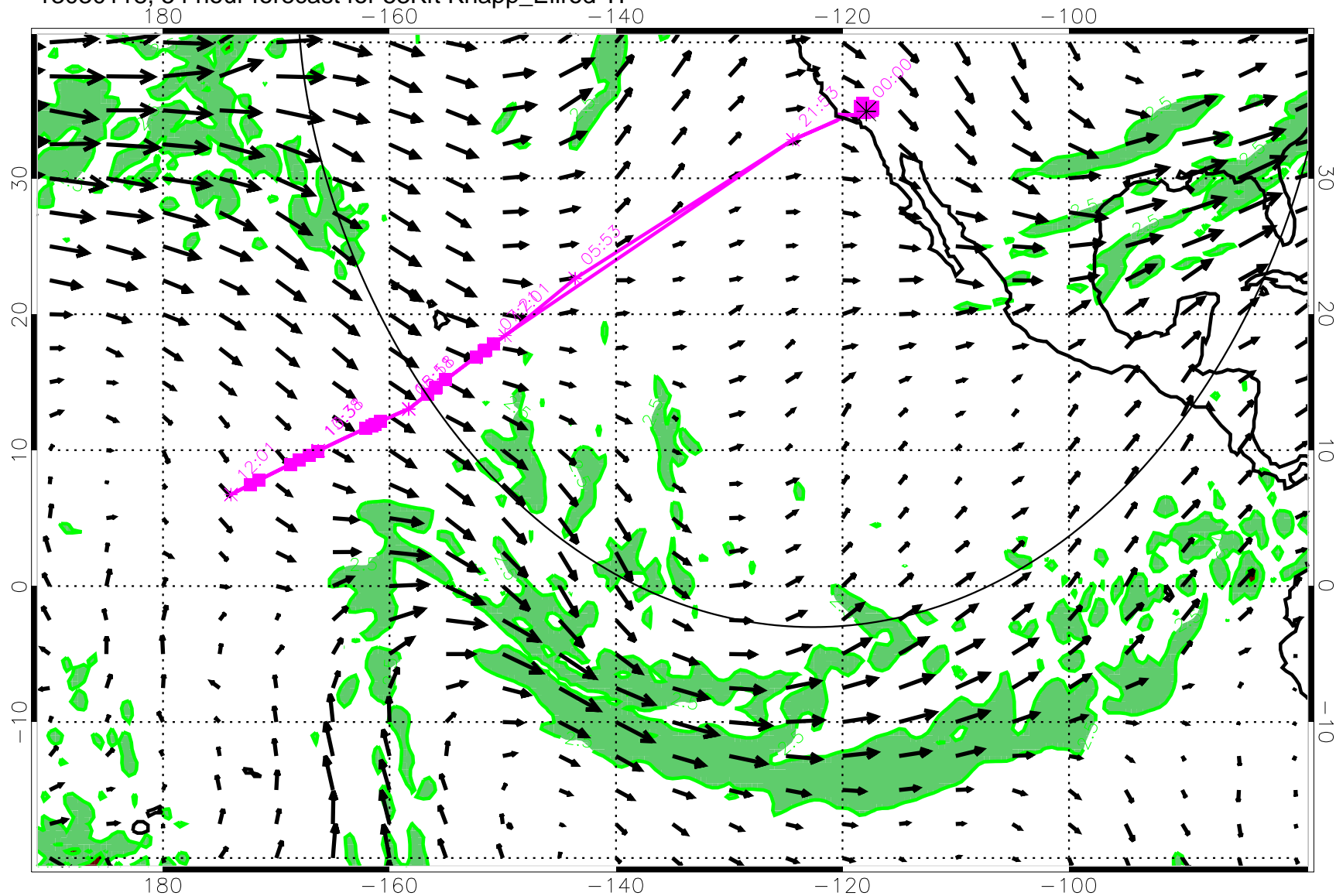
13030118, 54 hour forecast for 53Kft Knapp_Ellrod TI
