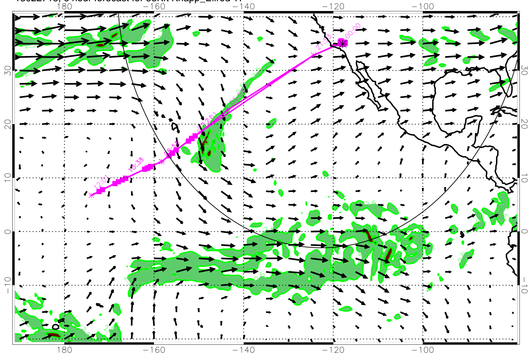
13022718, 6 hour forecast for 53Kft Knapp_Ellrod TI
