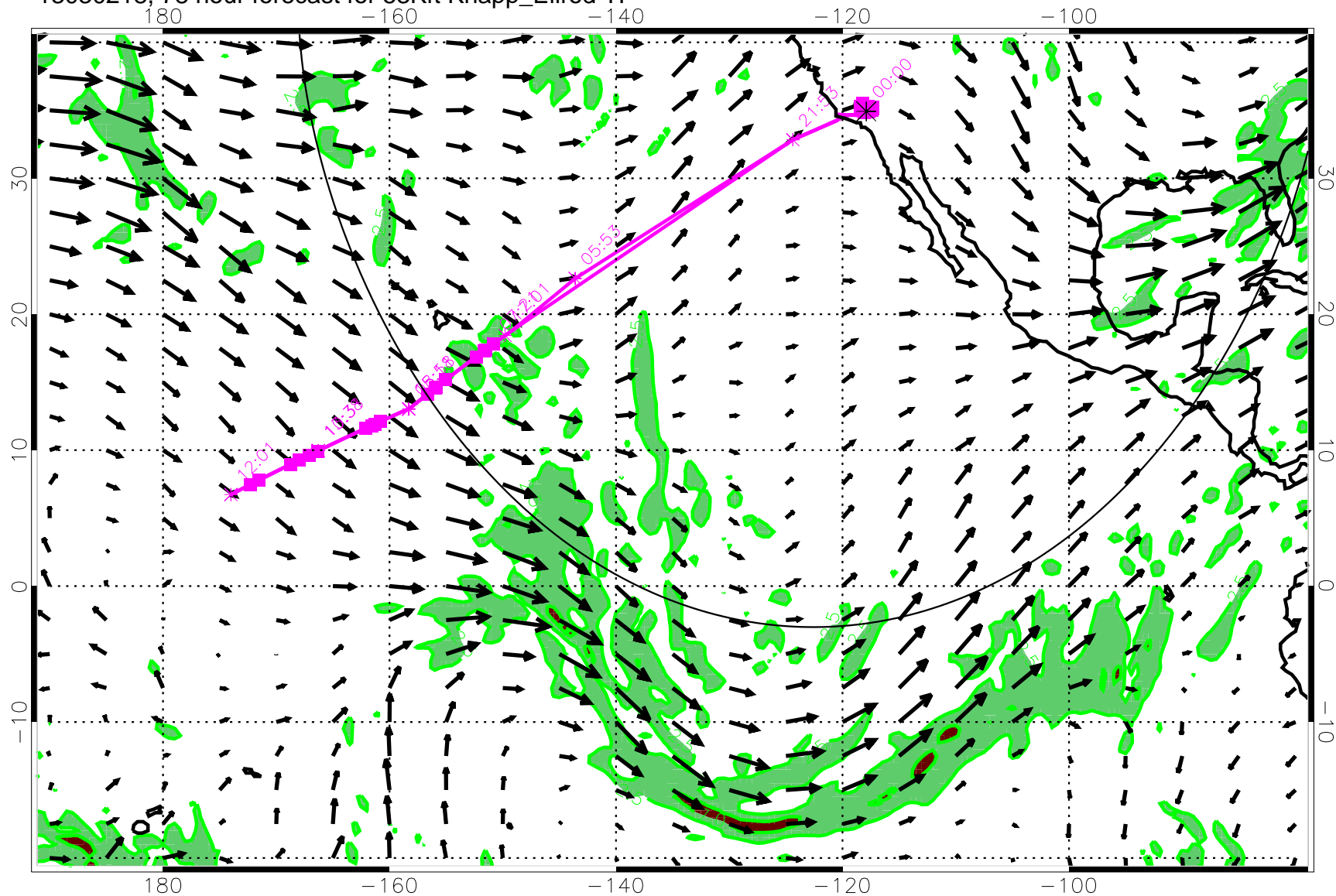
13030218, 78 hour forecast for 53Kft Knapp_Ellrod TI
