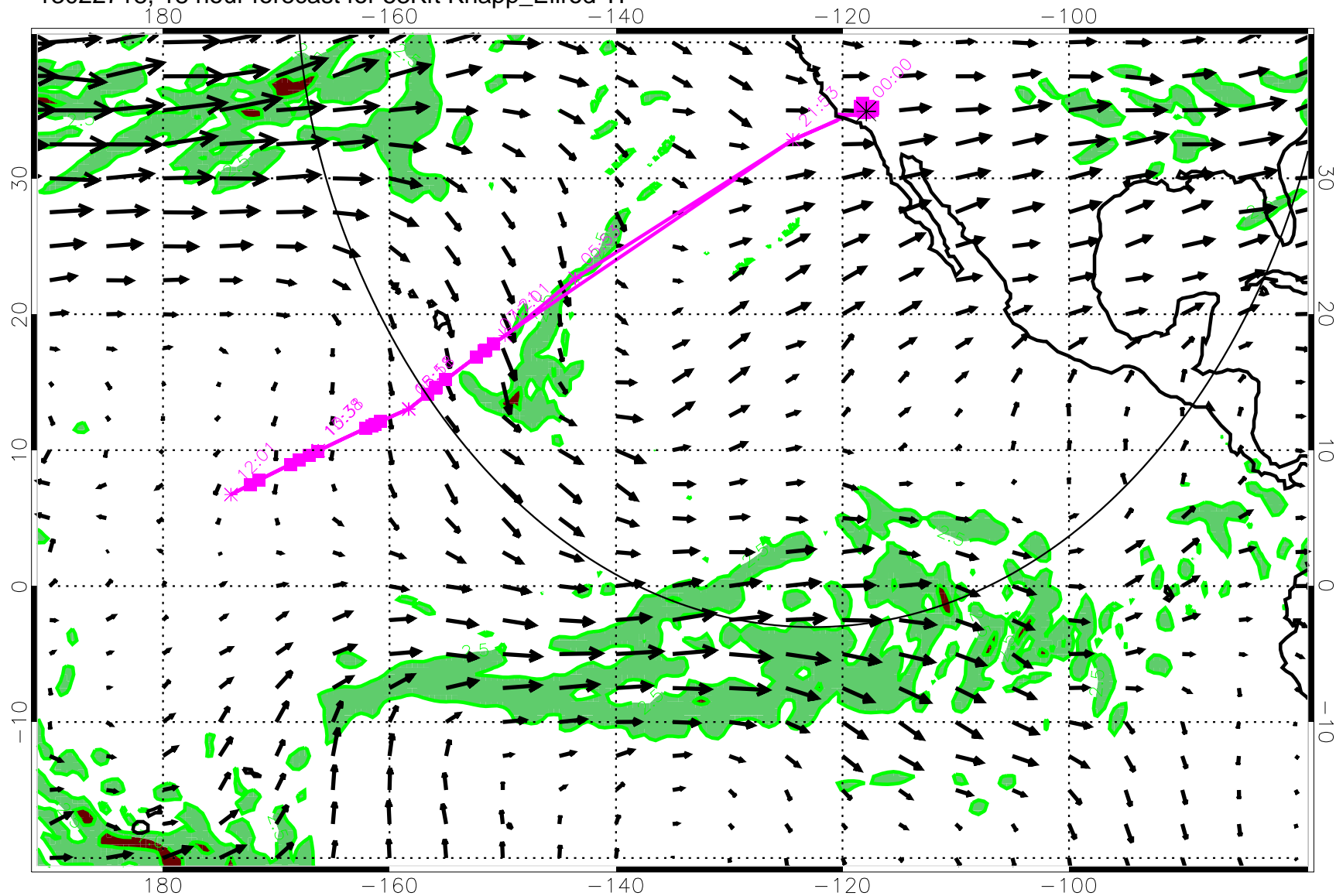
13022718, 18 hour forecast for 53Kft Knapp_Ellrod TI
