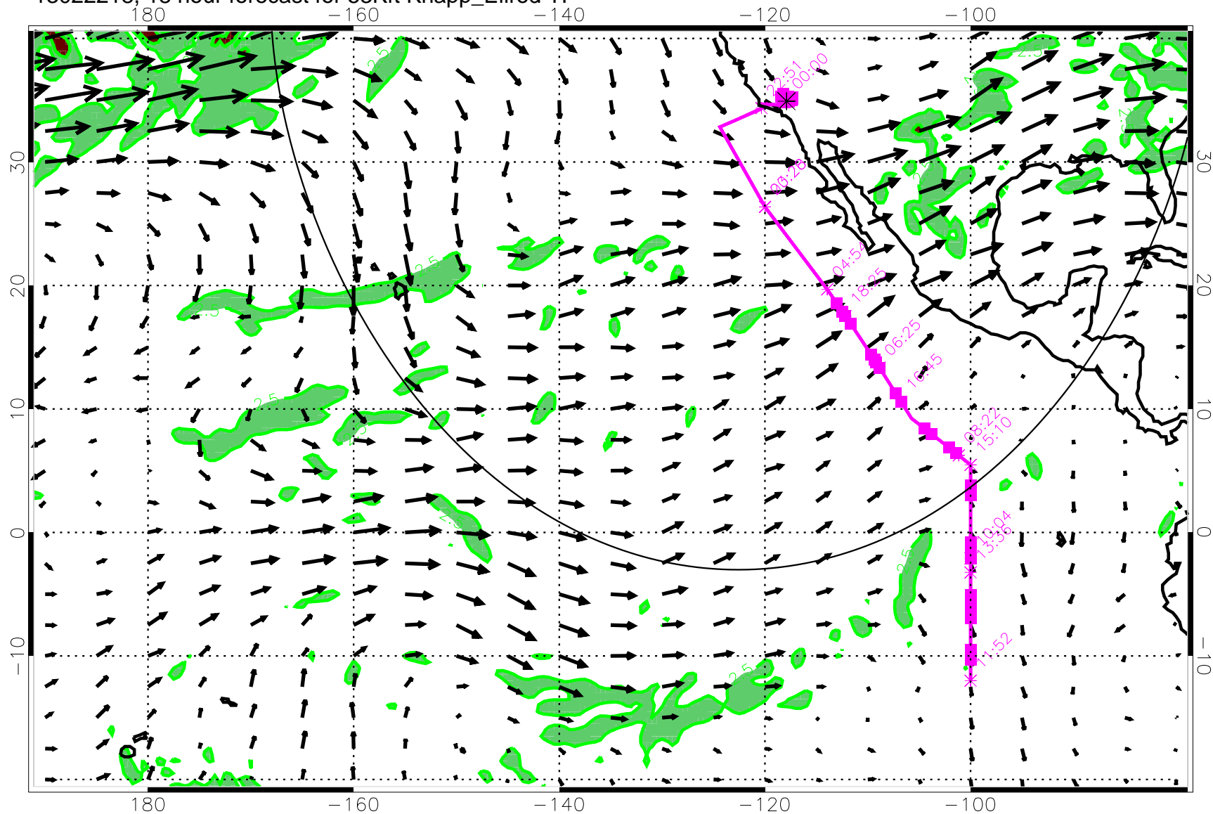
13022218, 18 hour forecast for 53Kft Knapp_Ellrod TI
