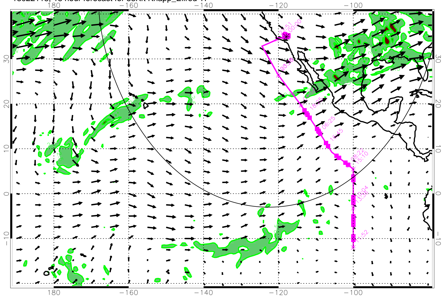
13022118, 18 hour forecast for 53Kft Knapp_Ellrod TI
