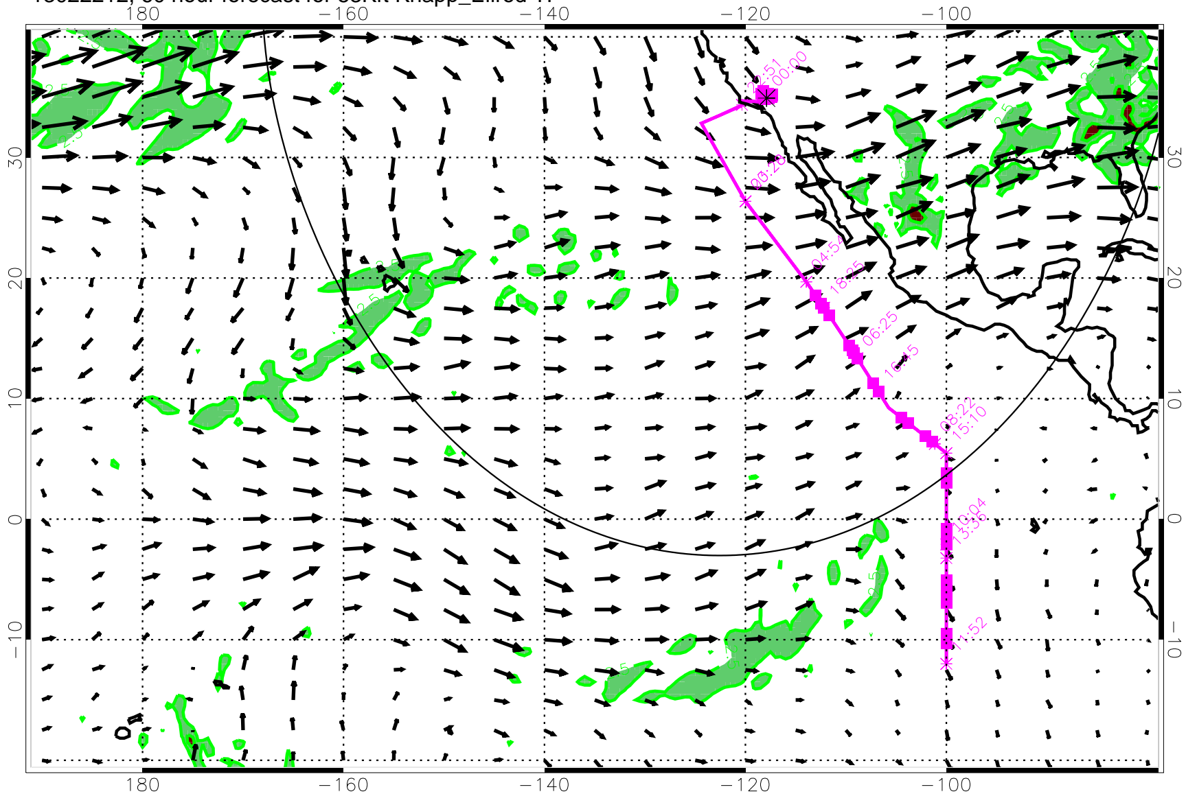
13022212, 60 hour forecast for 53Kft Knapp_Ellrod TI
