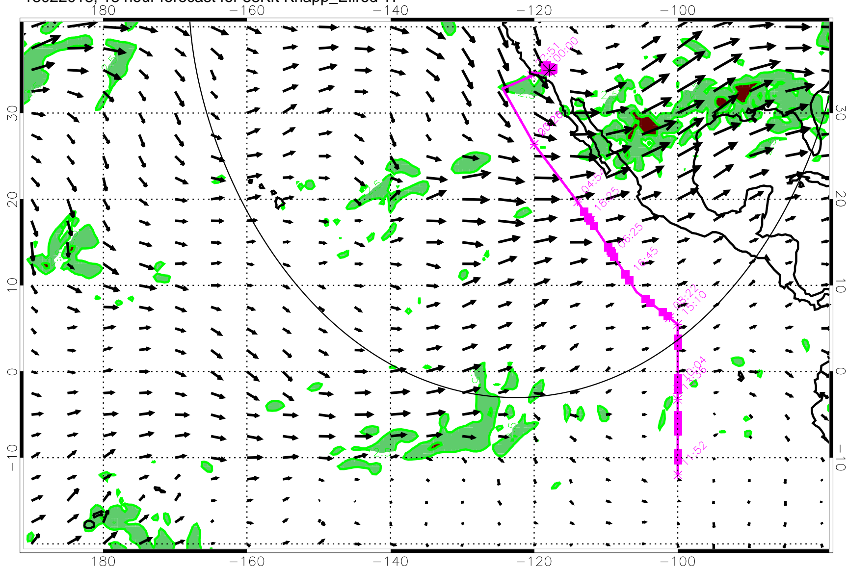
13022018, 18 hour forecast for 53Kft Knapp_Ellrod TI
