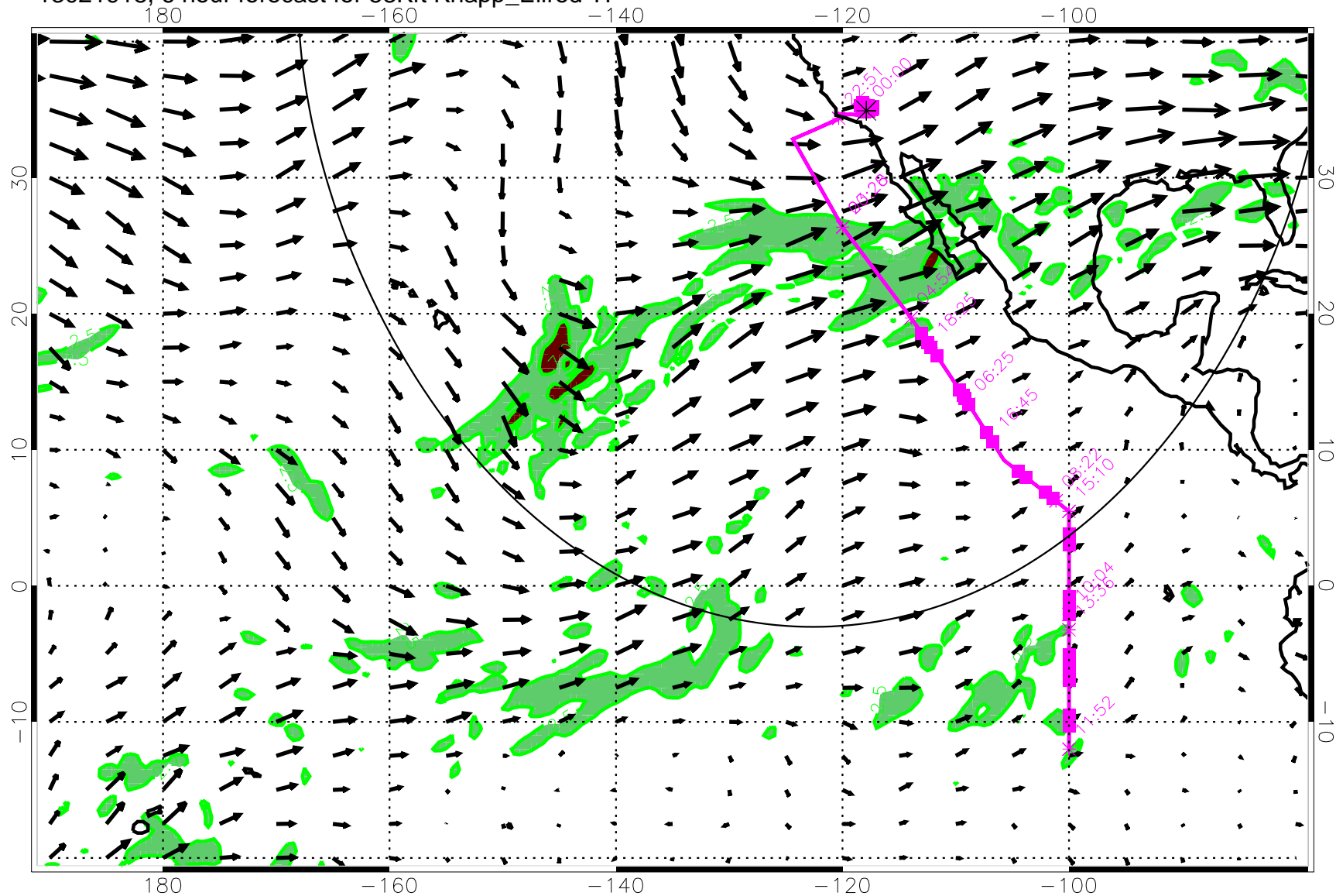
13021918, 6 hour forecast for 53Kft Knapp_Ellrod TI
