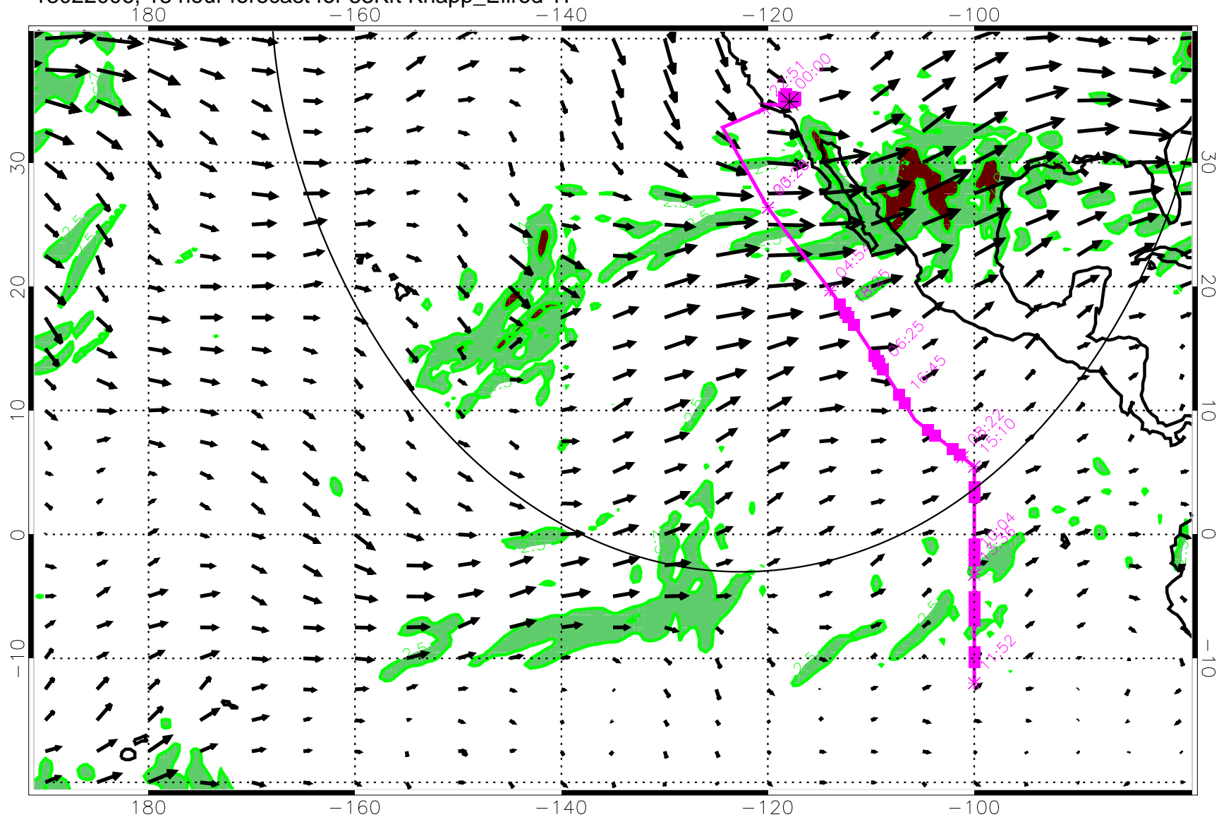
13022006, 18 hour forecast for 53Kft Knapp_Ellrod TI
