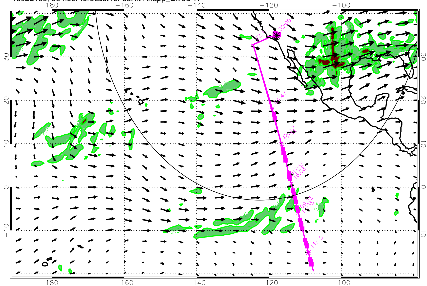
13022106, 66 hour forecast for 53Kft Knapp_Ellrod TI
