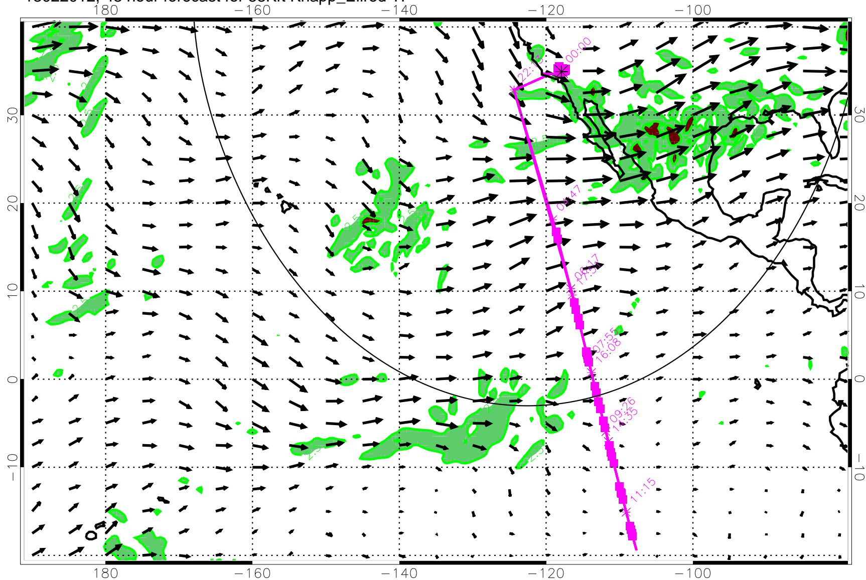
13022012, 48 hour forecast for 53Kft Knapp_Ellrod TI
