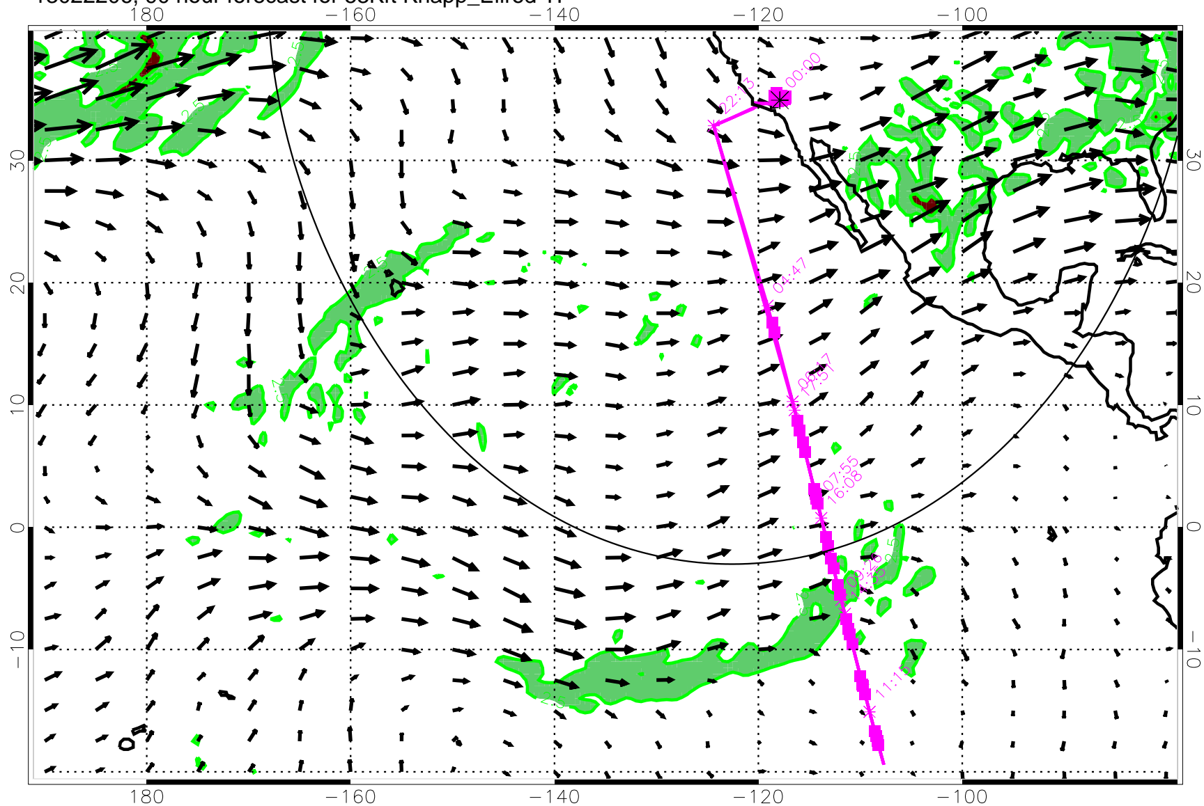
13022206, 90 hour forecast for 53Kft Knapp_Ellrod TI
