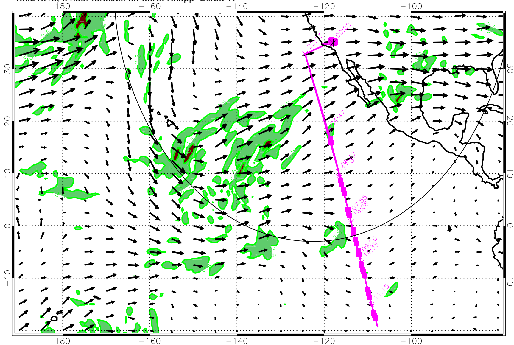
13021818, 6 hour forecast for 53Kft Knapp_Ellrod TI
