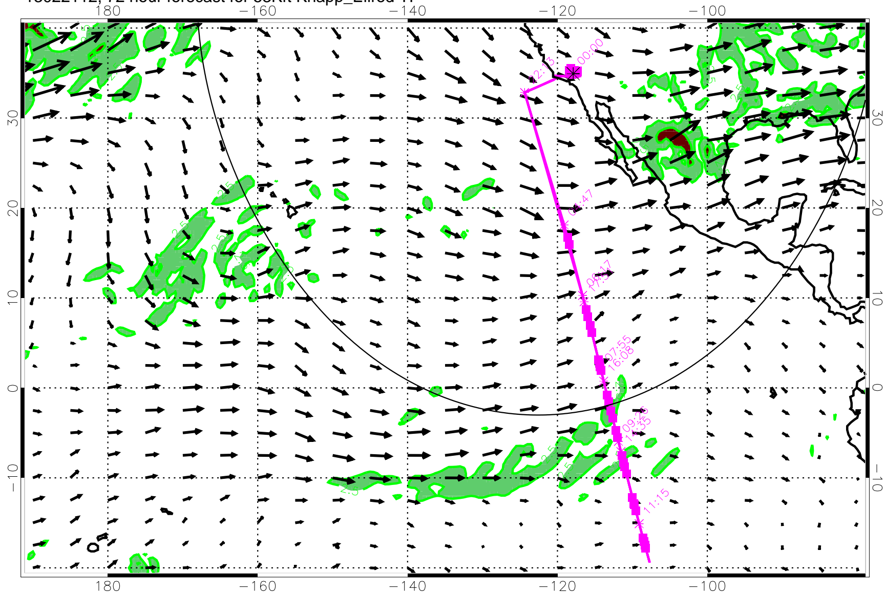
13022112, 72 hour forecast for 53Kft Knapp_Ellrod TI
