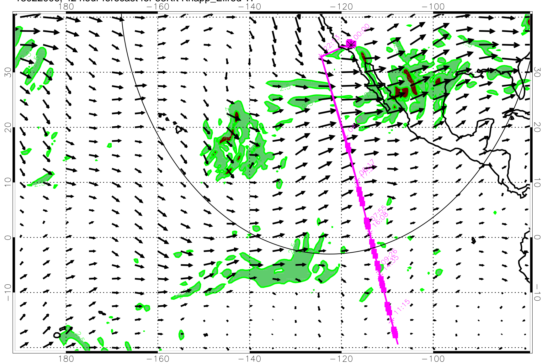
13022006, 42 hour forecast for 53Kft Knapp_Ellrod TI
