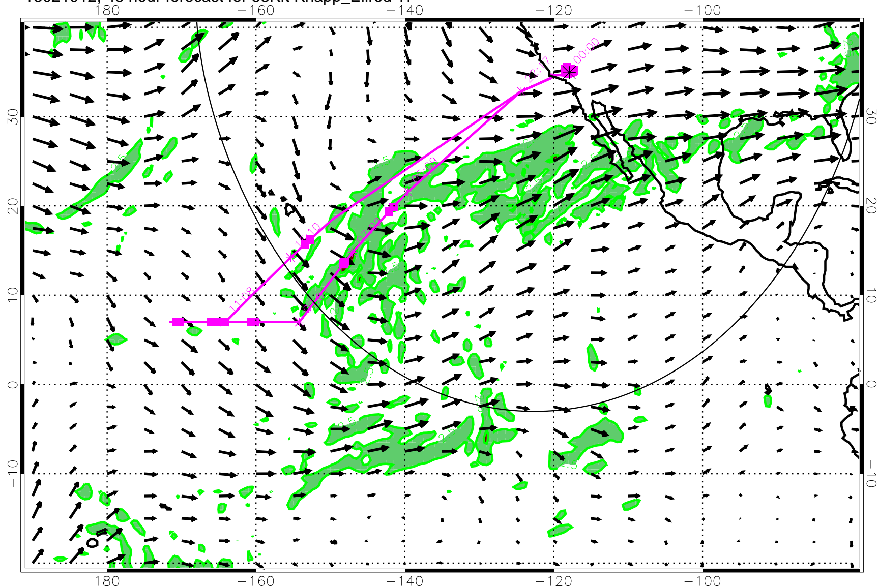
13021912, 48 hour forecast for 53Kft Knapp_Ellrod TI
