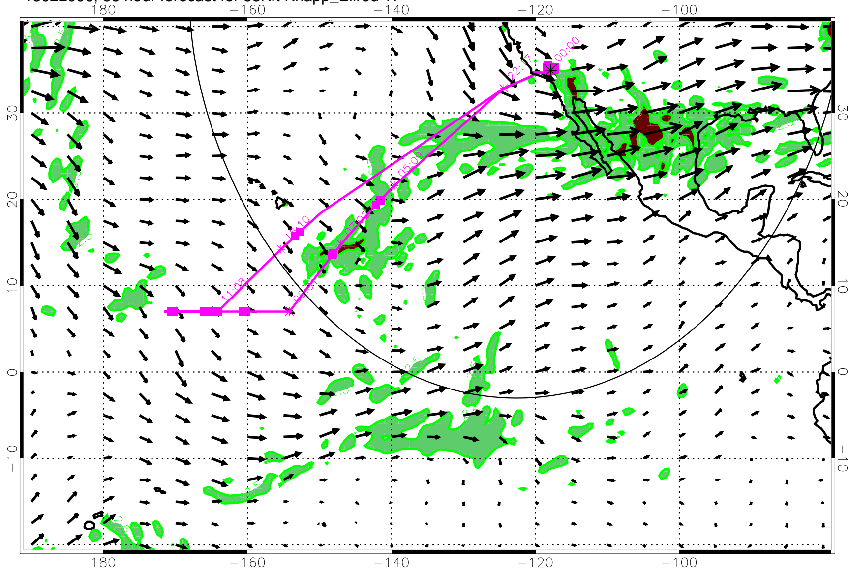
13022006, 66 hour forecast for 53Kft Knapp_Ellrod TI
