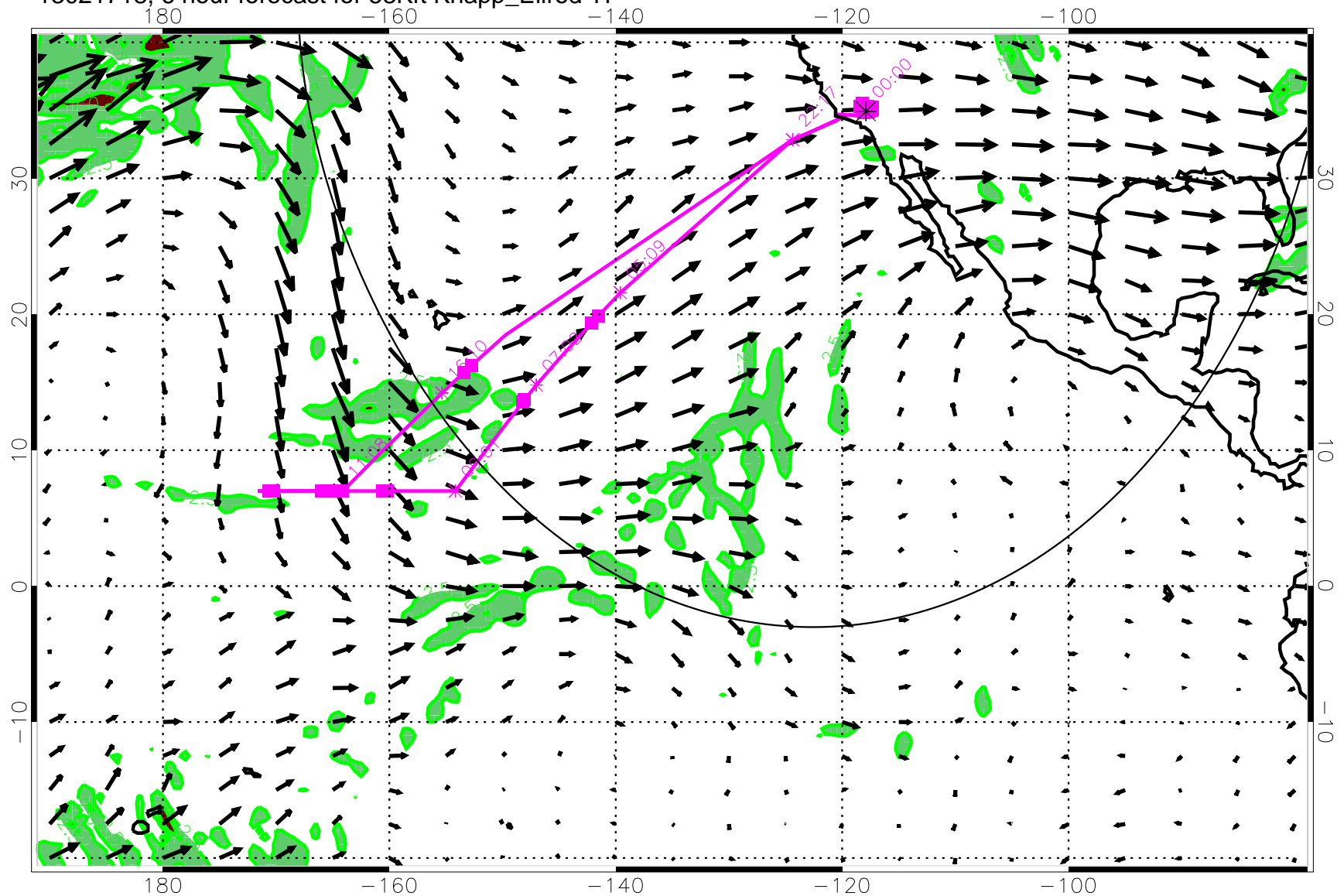
13021718, 6 hour forecast for 53Kft Knapp_Ellrod TI
