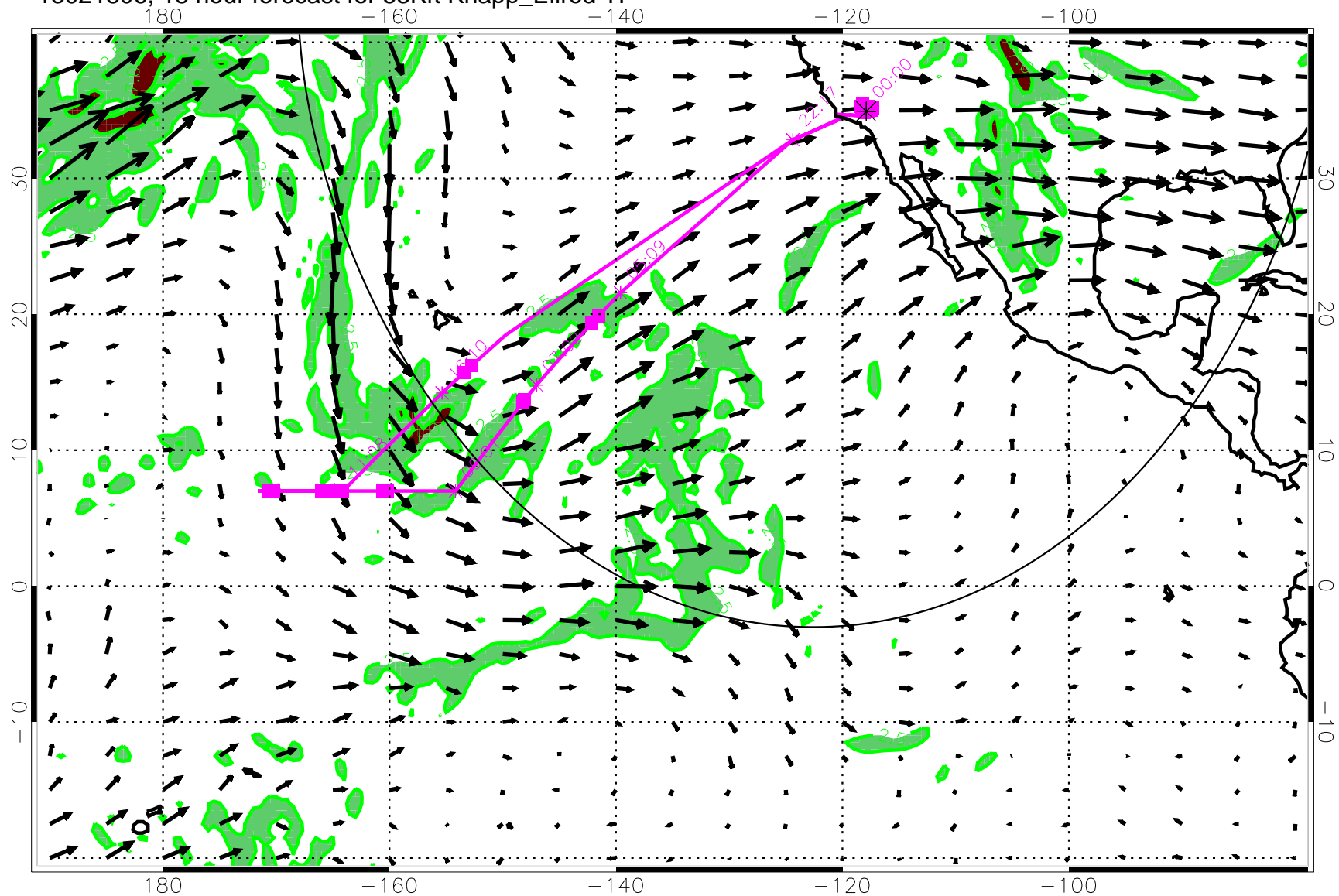
13021806, 18 hour forecast for 53Kft Knapp_Ellrod TI
