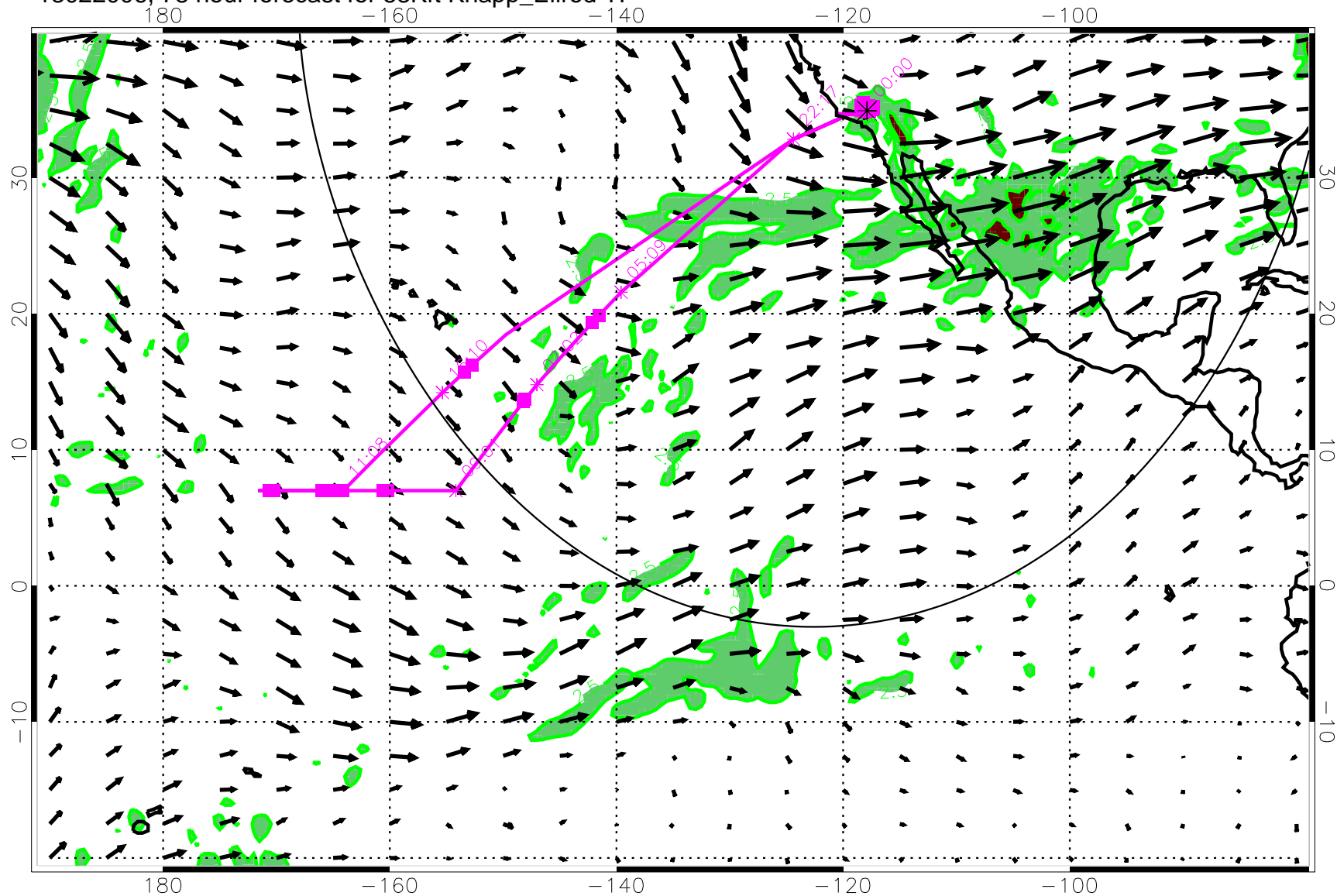
13022006, 78 hour forecast for 53Kft Knapp_Ellrod TI
