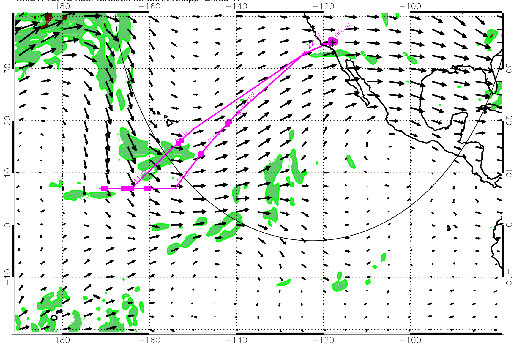
13021712, 12 hour forecast for 53Kft Knapp_Ellrod TI
