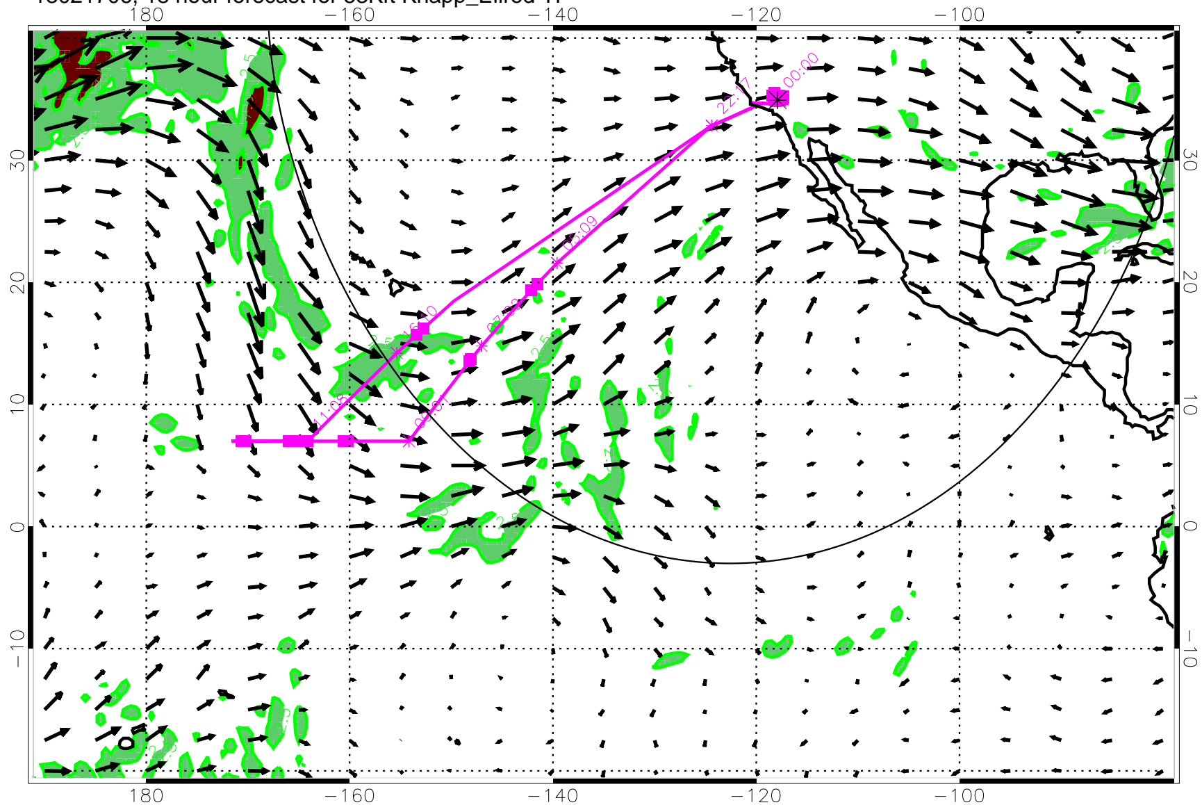
13021706, 18 hour forecast for 53Kft Knapp_Ellrod TI
