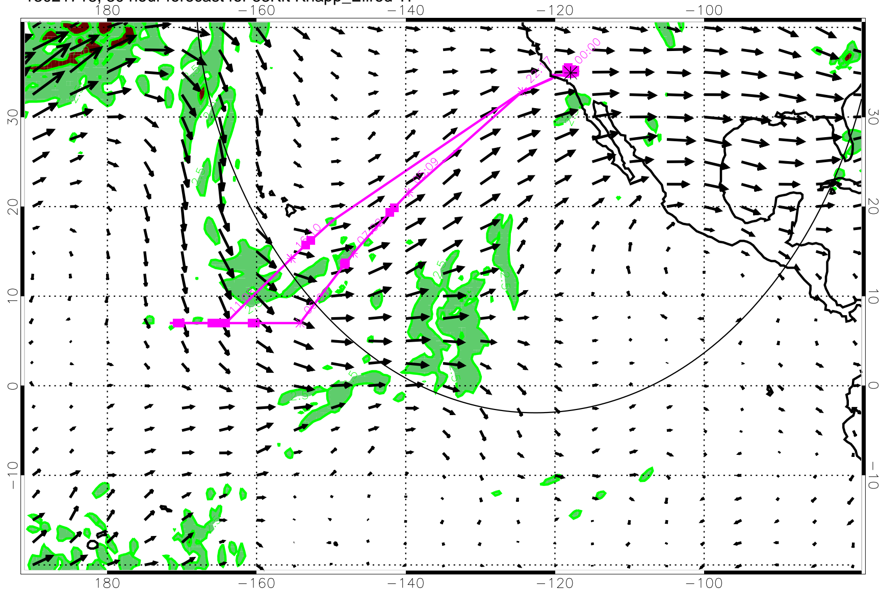
13021718, 30 hour forecast for 53Kft Knapp_Ellrod TI
