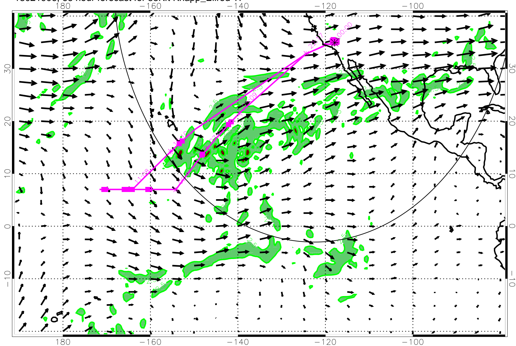
13021906, 66 hour forecast for 53Kft Knapp_Ellrod TI
