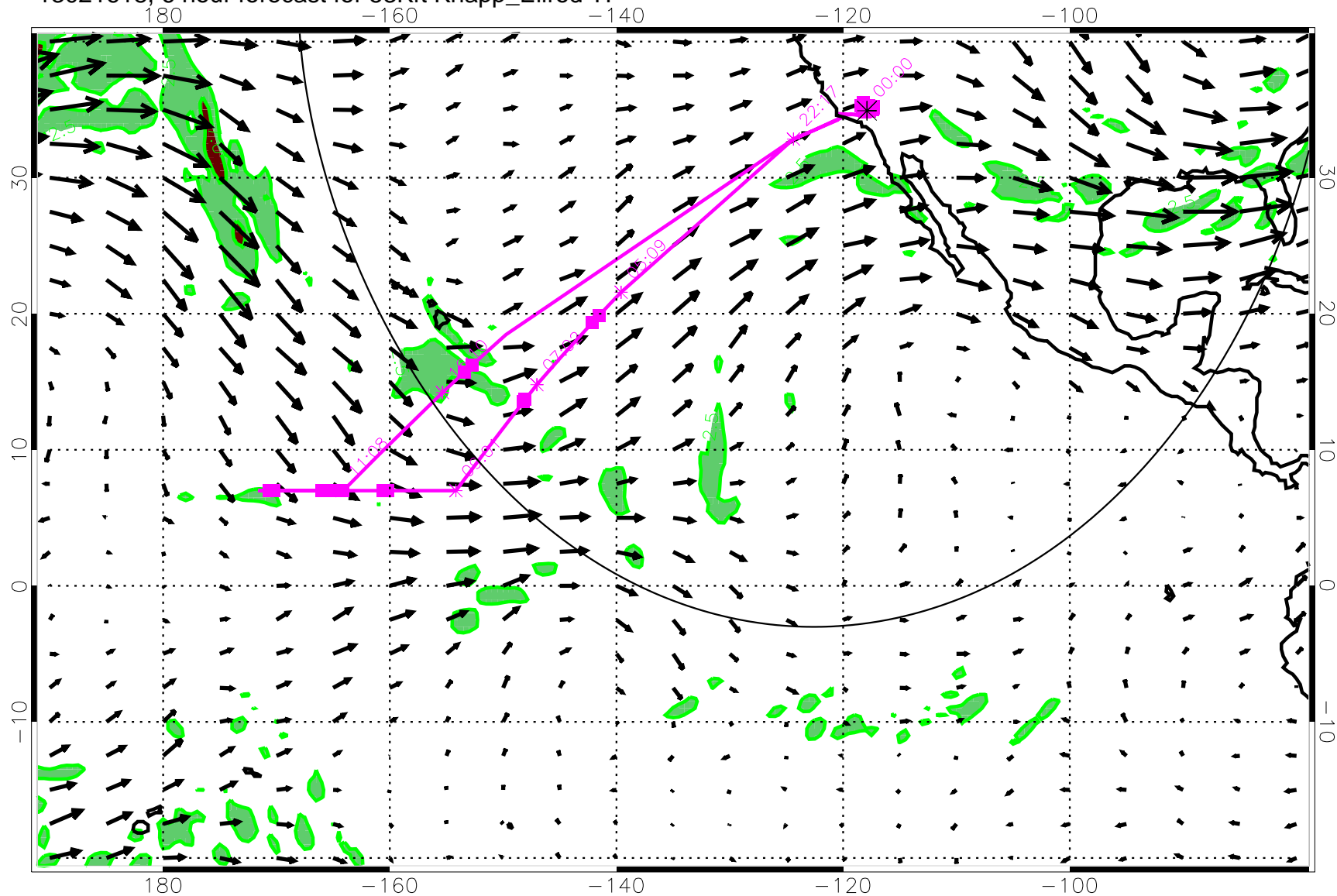
13021618, 6 hour forecast for 53Kft Knapp_Ellrod TI
