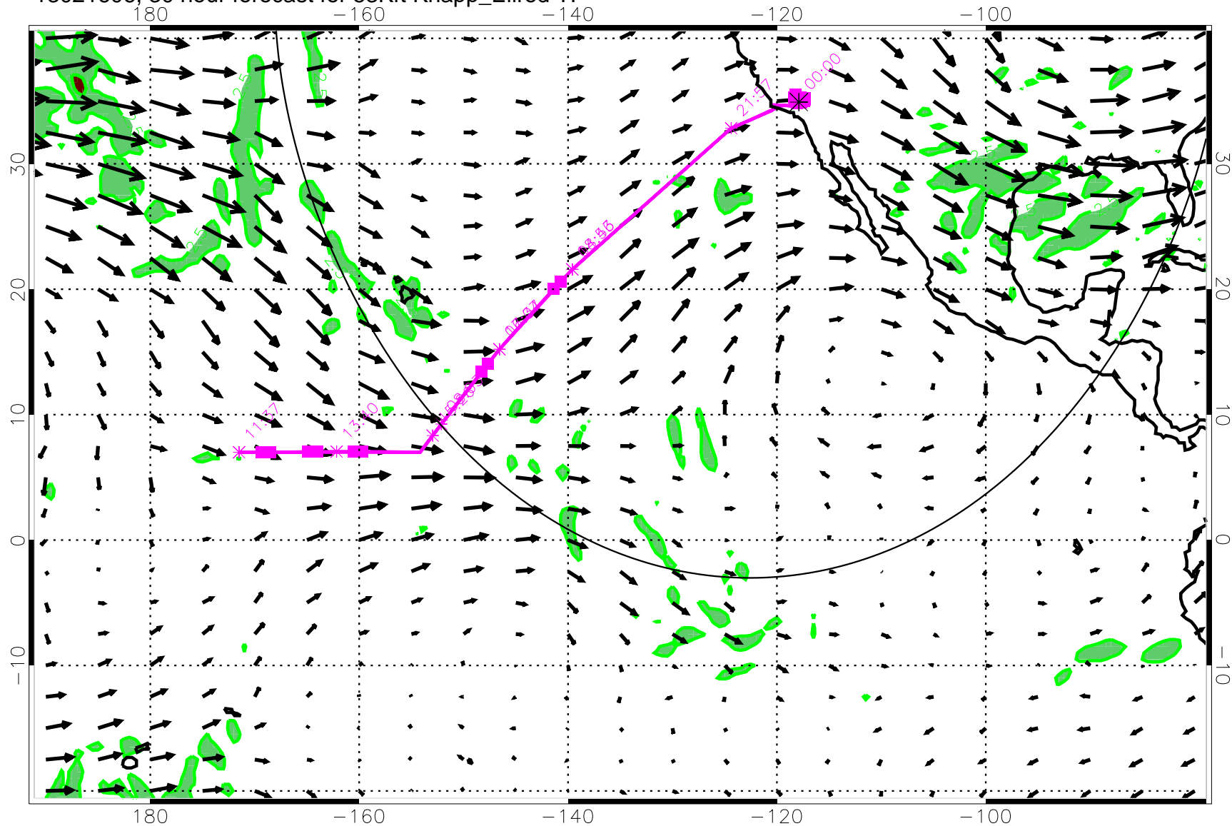
13021606, 30 hour forecast for 53Kft Knapp_Ellrod TI
