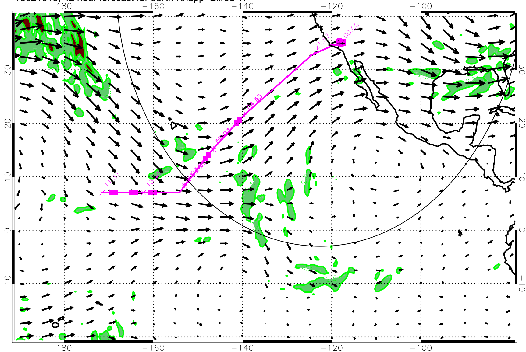
13021618, 42 hour forecast for 53Kft Knapp_Ellrod TI
