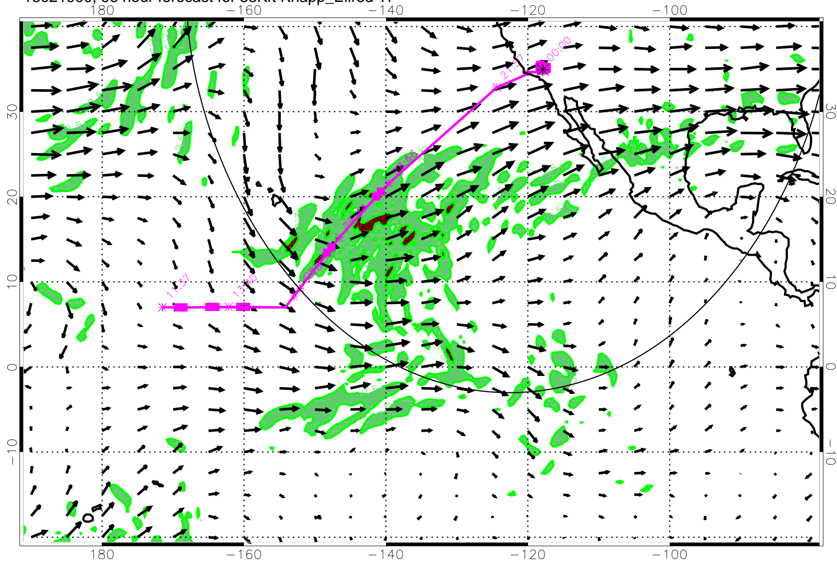
13021900, 96 hour forecast for 53Kft Knapp_Ellrod TI
