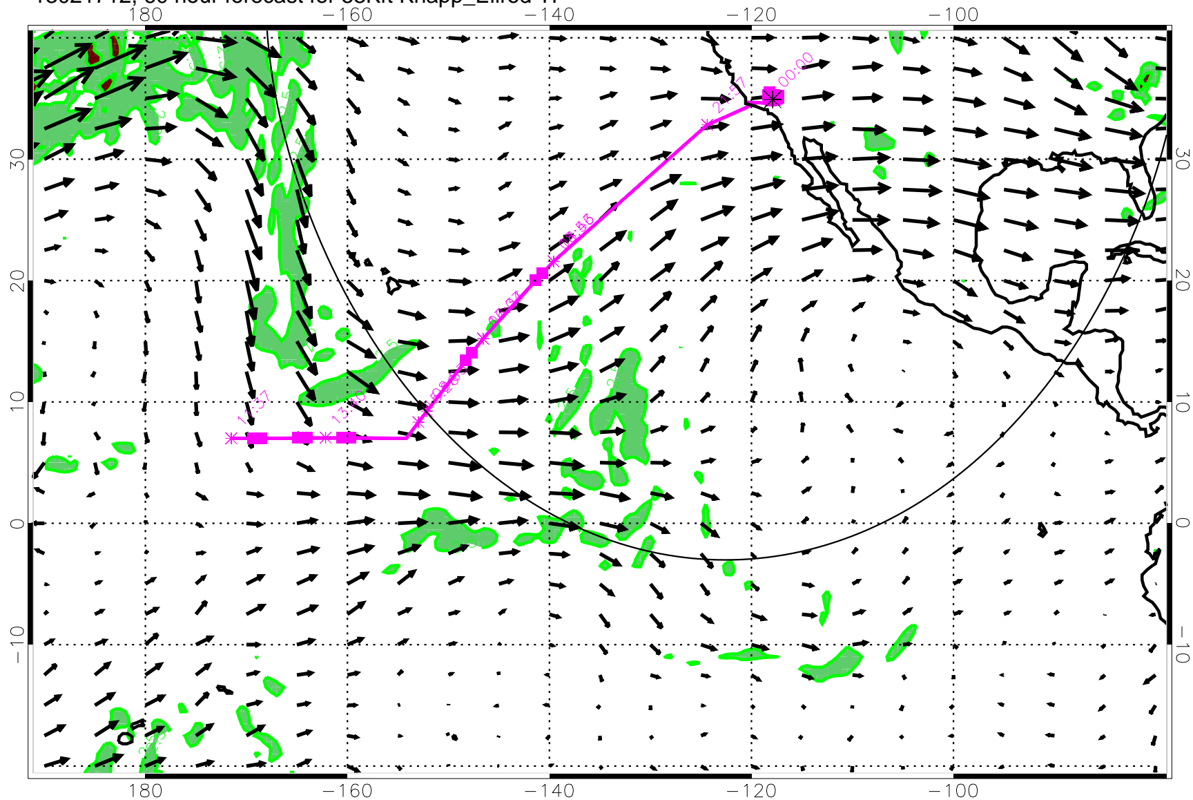
13021712, 60 hour forecast for 53Kft Knapp_Ellrod TI
