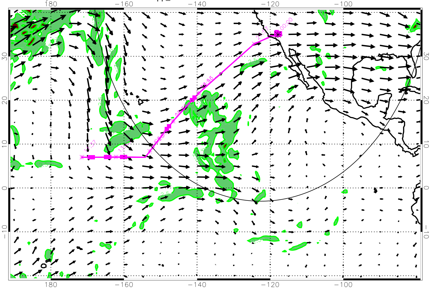
13021718, 66 hour forecast for 53Kft Knapp_Ellrod TI
