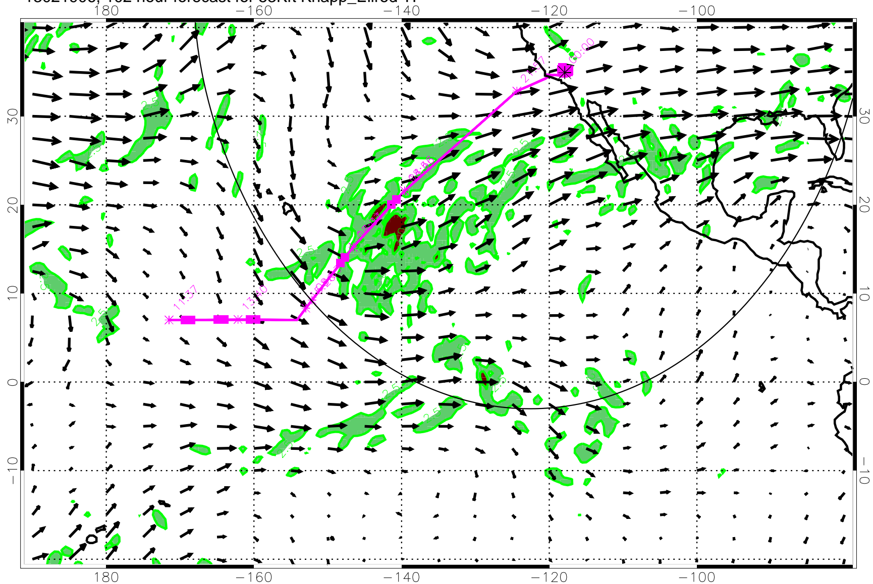
13021906, 102 hour forecast for 53Kft Knapp_Ellrod TI
