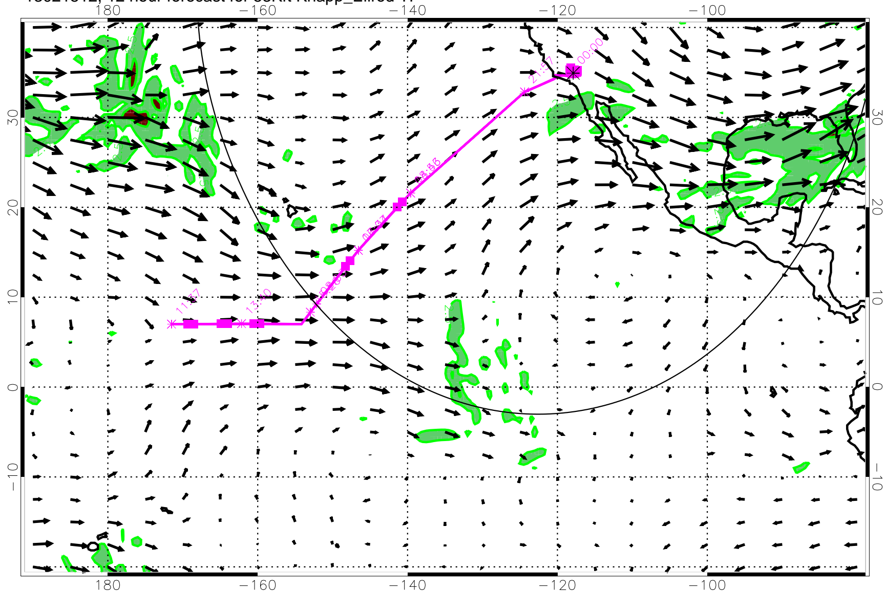
13021512, 12 hour forecast for 53Kft Knapp_Ellrod TI
