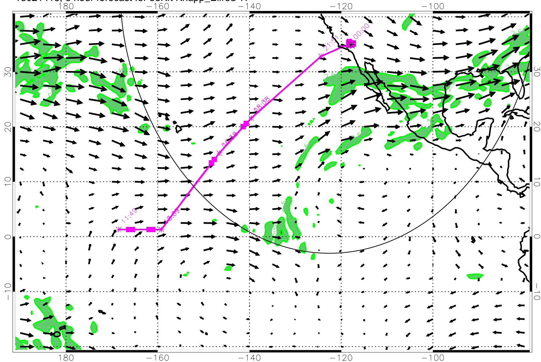
13021418, 6 hour forecast for 53Kft Knapp_Ellrod TI
