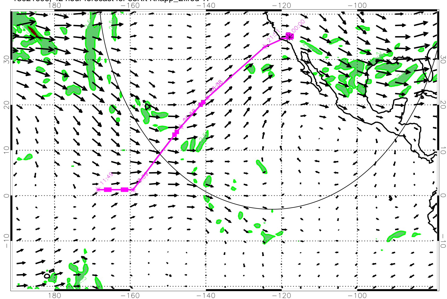
13021606, 42 hour forecast for 53Kft Knapp_Ellrod TI
