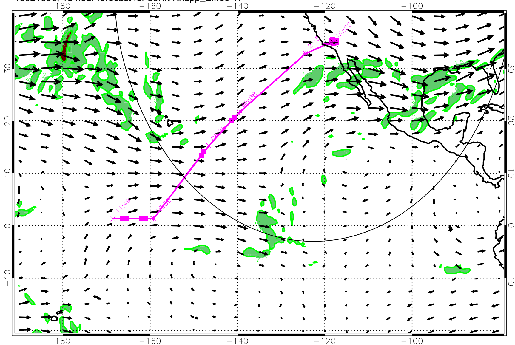
13021506, 18 hour forecast for 53Kft Knapp_Ellrod TI
