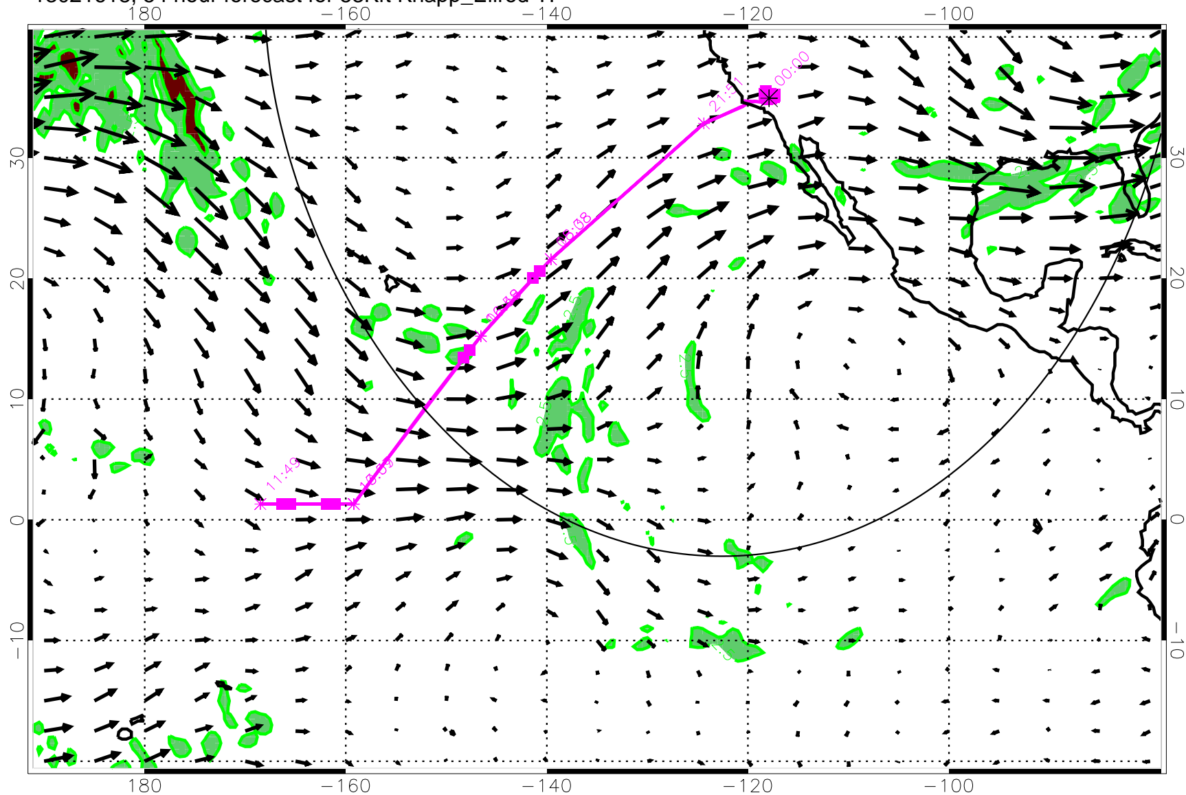
13021618, 54 hour forecast for 53Kft Knapp_Ellrod TI
