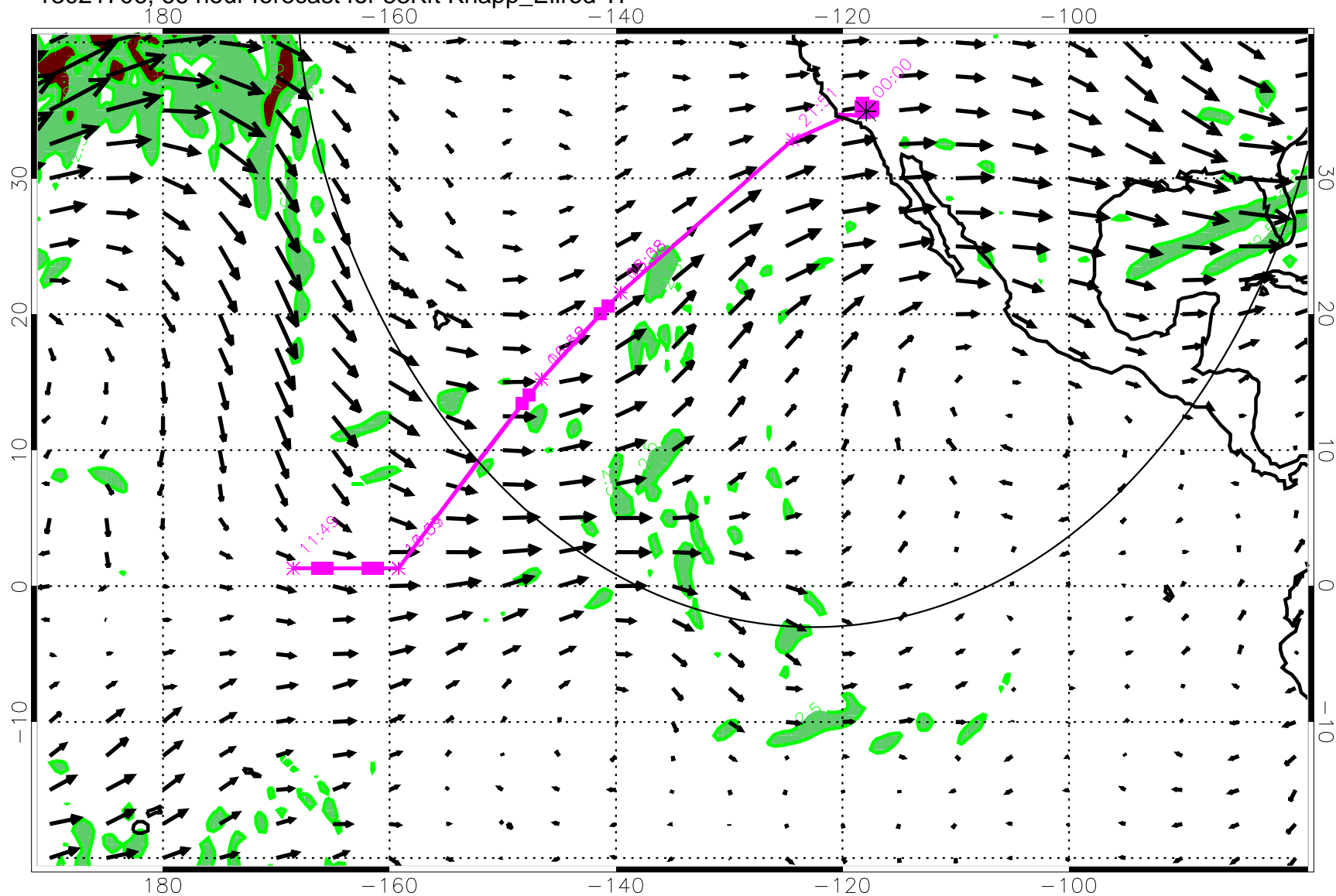
13021706, 66 hour forecast for 53Kft Knapp_Ellrod TI
