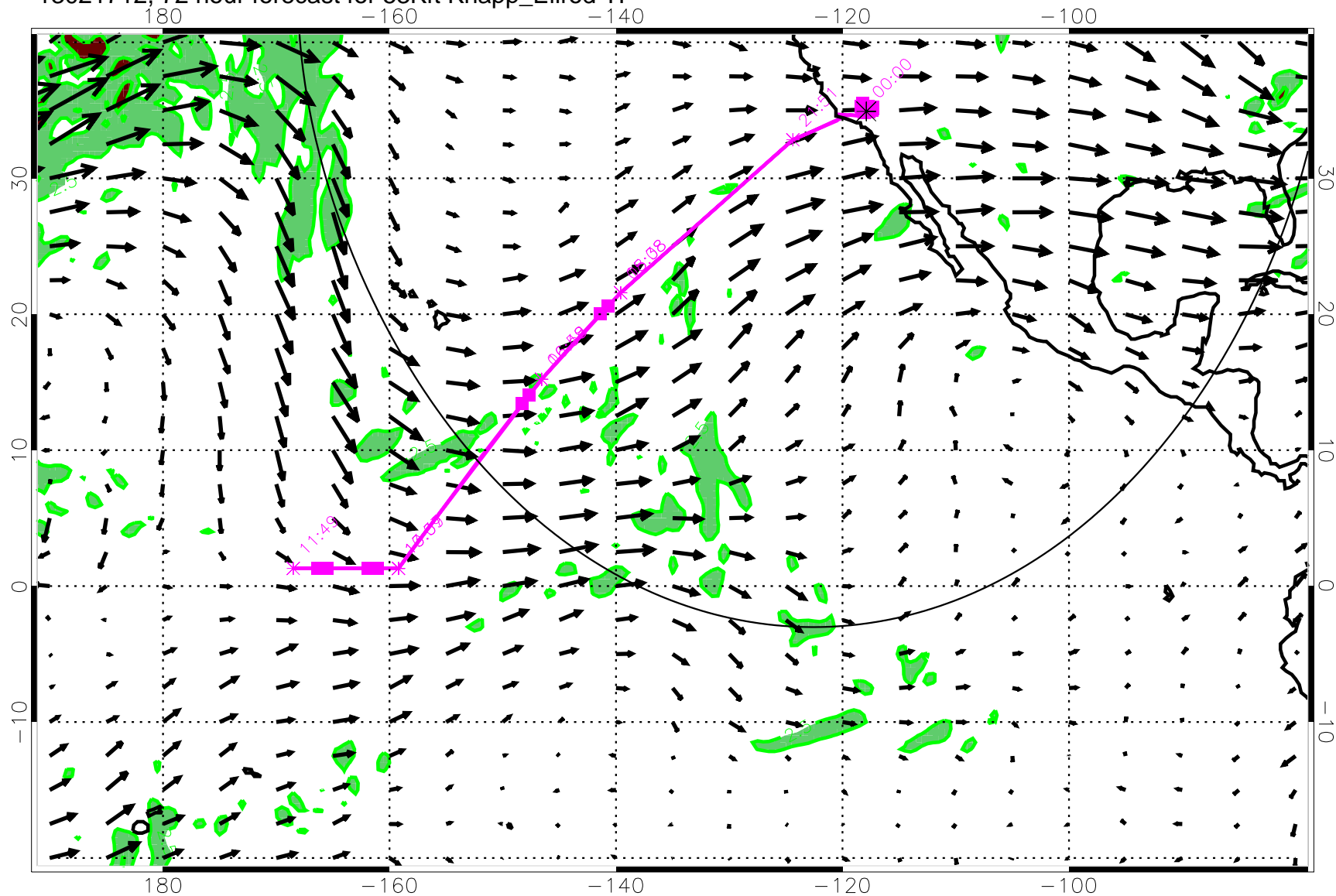
13021712, 72 hour forecast for 53Kft Knapp_Ellrod TI
