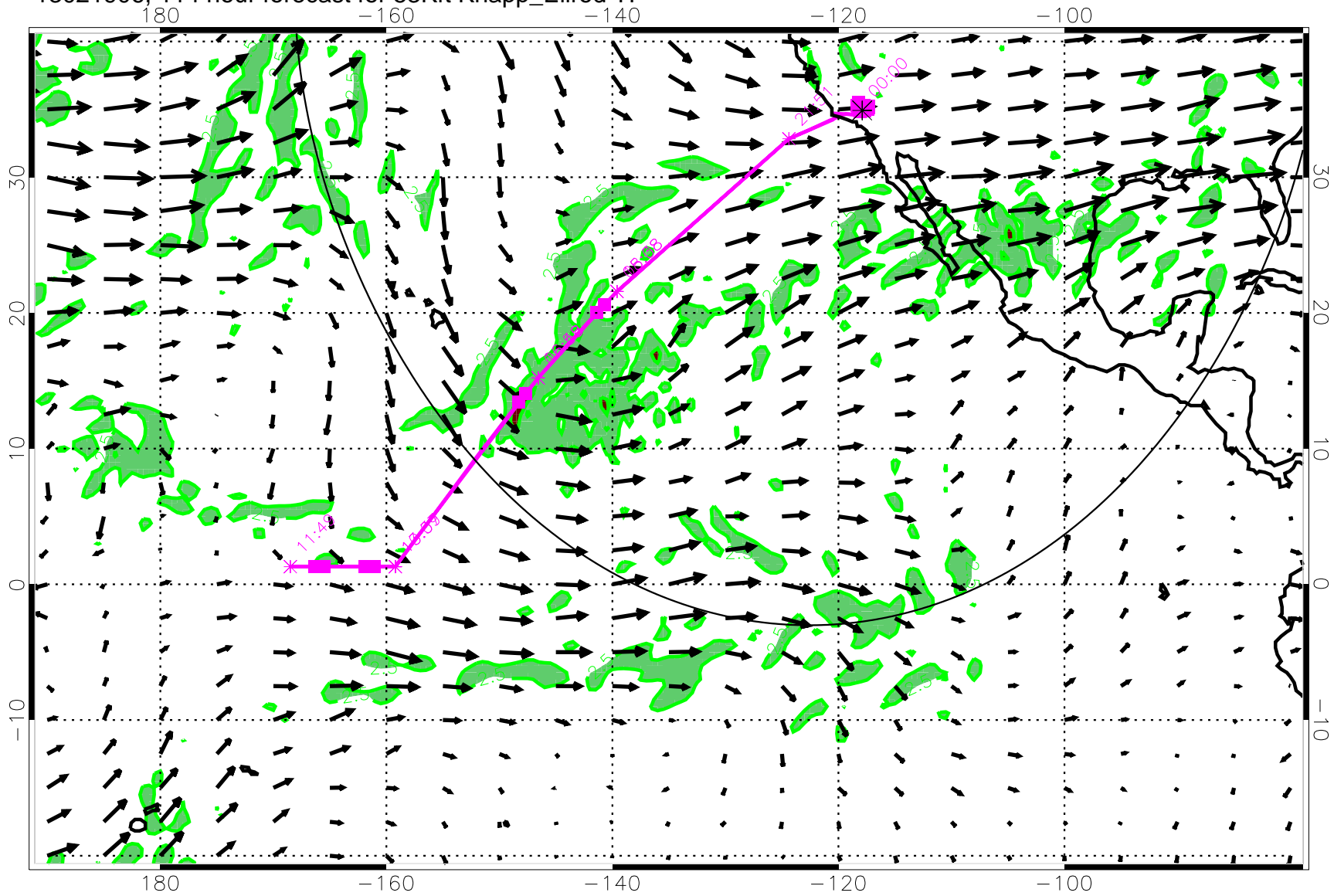
13021906, 114 hour forecast for 53Kft Knapp_Ellrod T1
