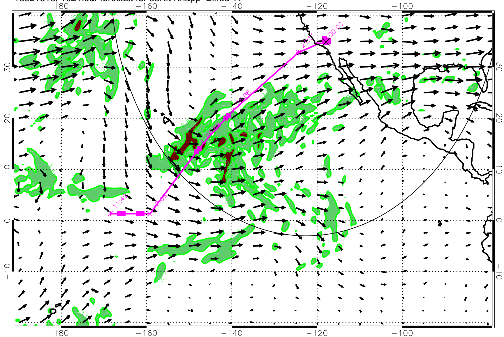
13021818, 102 hour forecast for 53Kft Knapp_Ellrod T1
