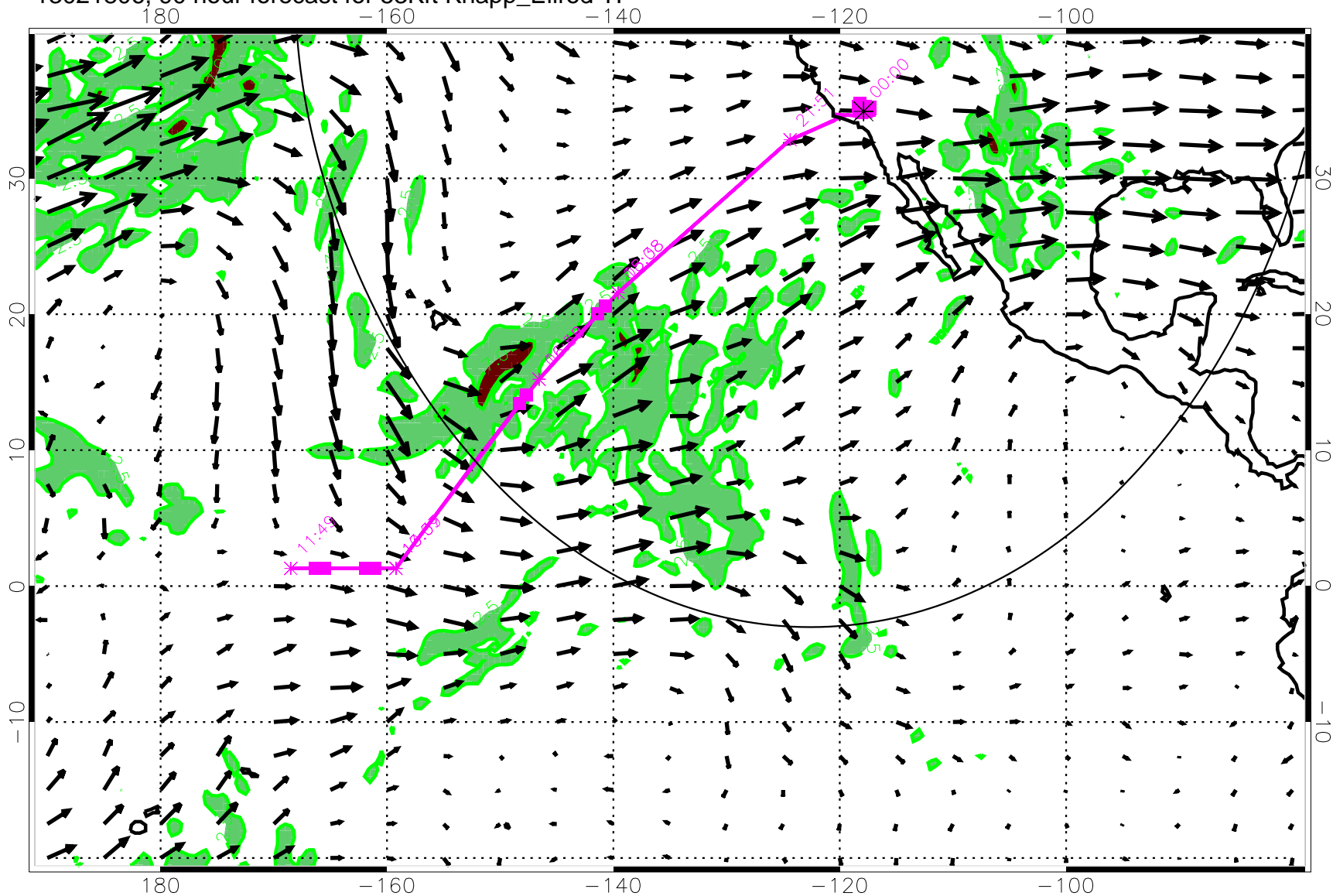
13021806, 90 hour forecast for 53Kft Knapp_Ellrod TI
