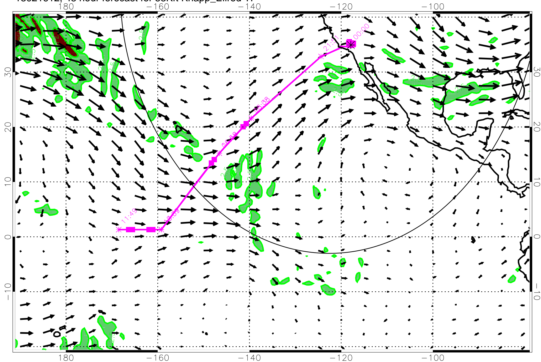
13021612, 48 hour forecast for 53Kft Knapp_Ellrod TI
