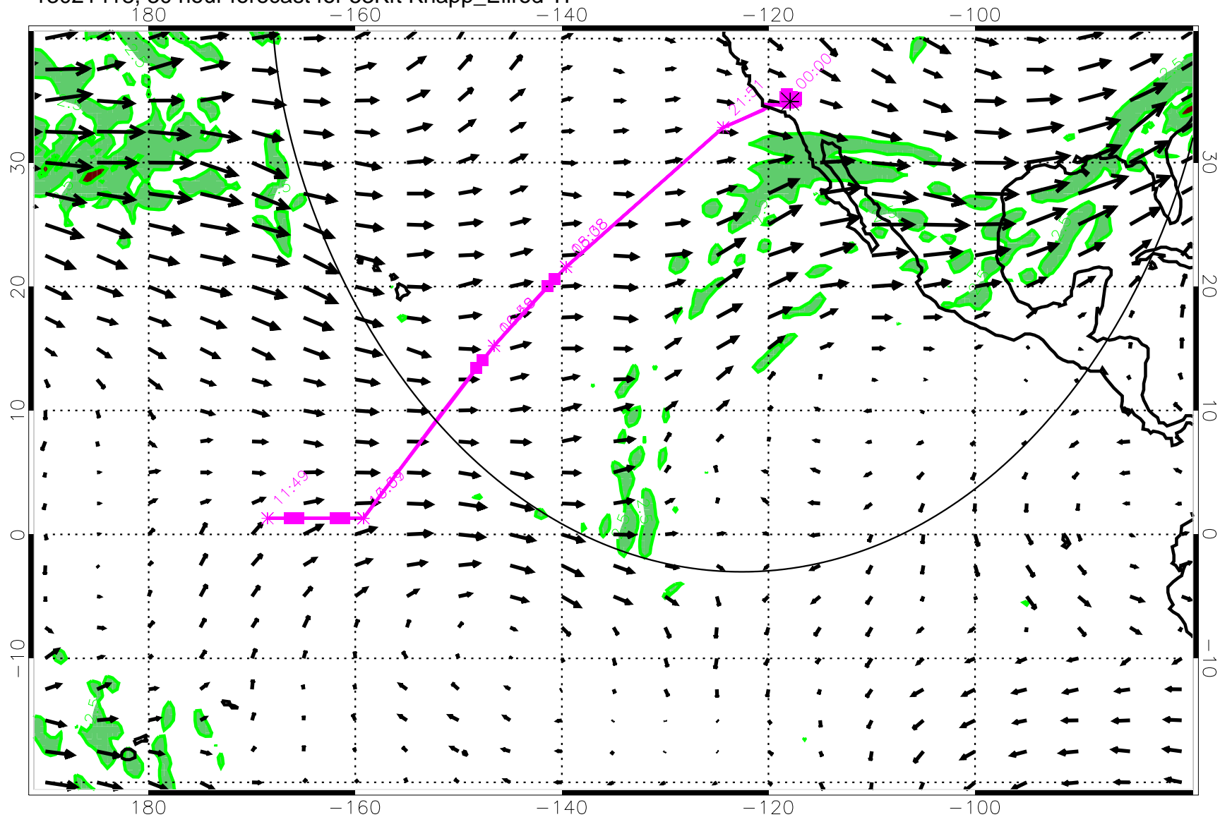
13021418, 30 hour forecast for 53Kft Knapp_Ellrod T1
