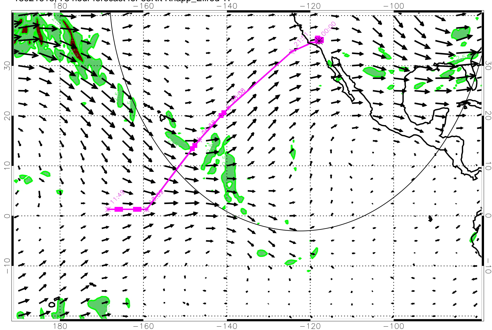
13021618, 78 hour forecast for 53Kft Knapp_Ellrod TI
