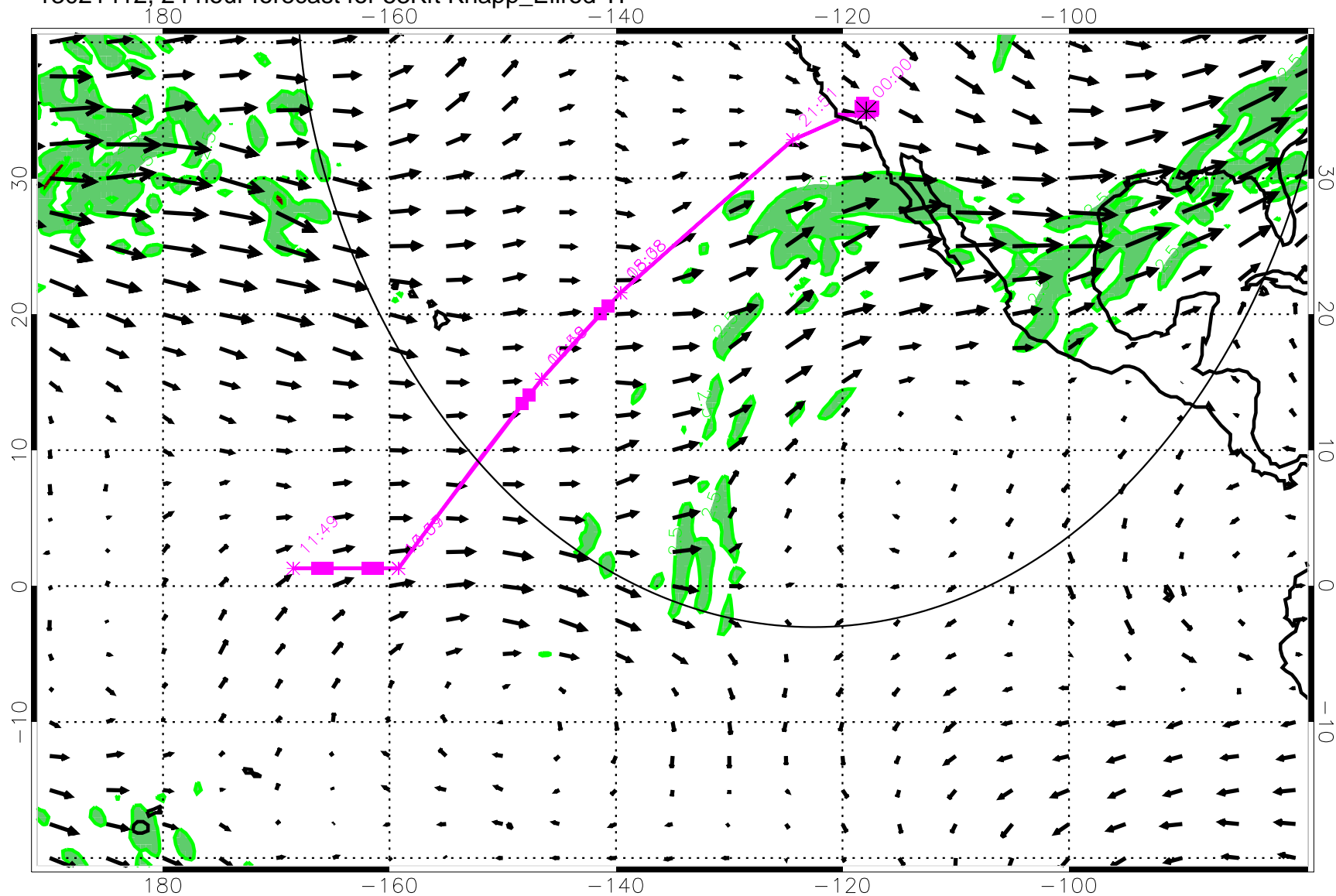
13021412, 24 hour forecast for 53Kft Knapp_Ellrod TI
