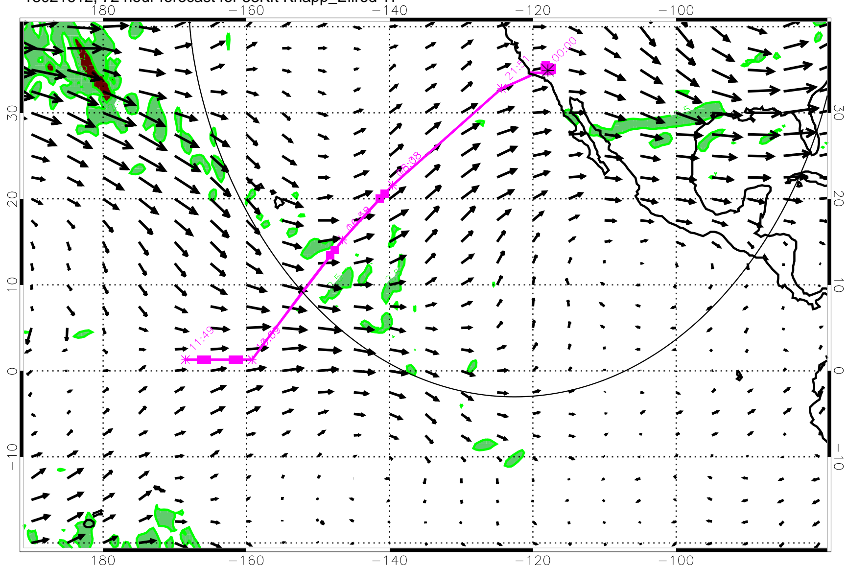
13021612, 72 hour forecast for 53Kft Knapp_Ellrod TI
