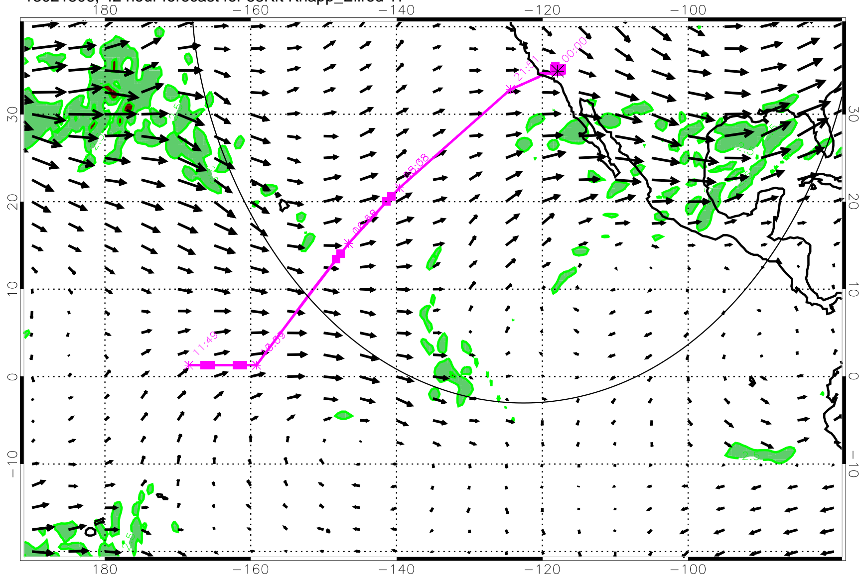
13021506, 42 hour forecast for 53Kft Knapp_Ellrod TI
