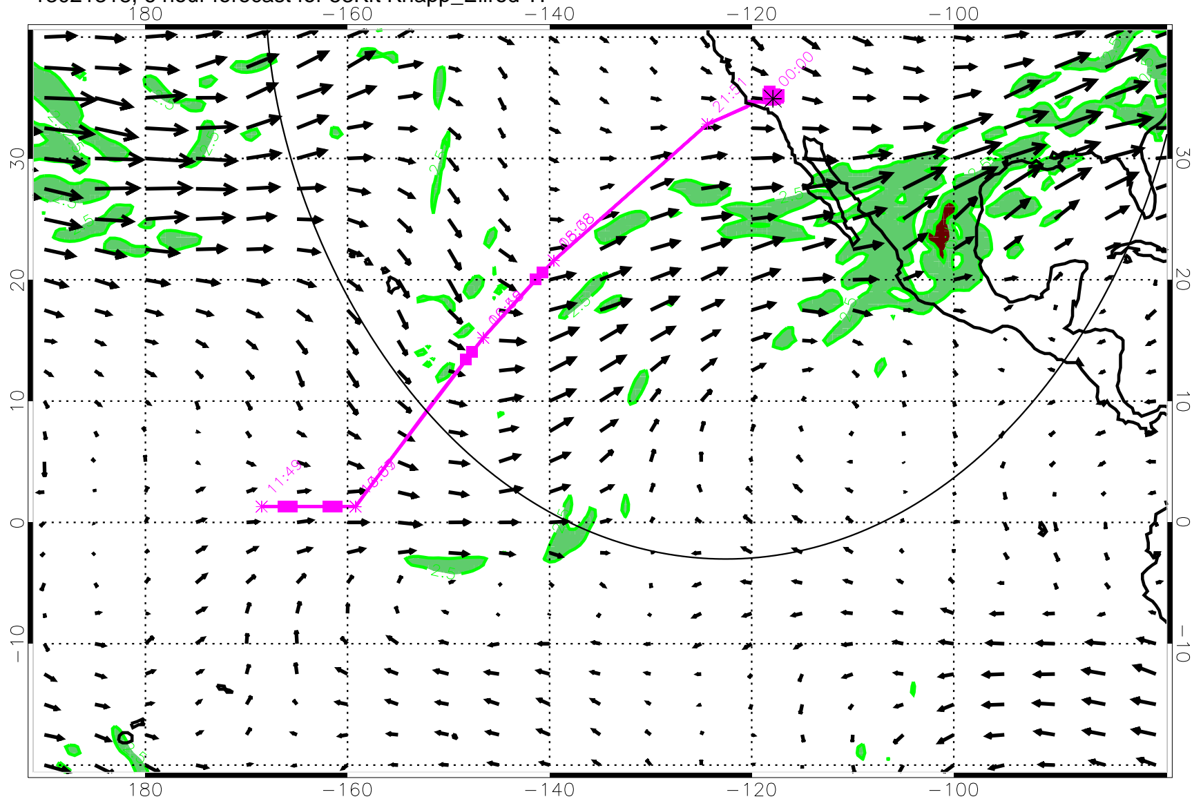
13021318, 6 hour forecast for 53Kft Knapp_Ellrod TI
