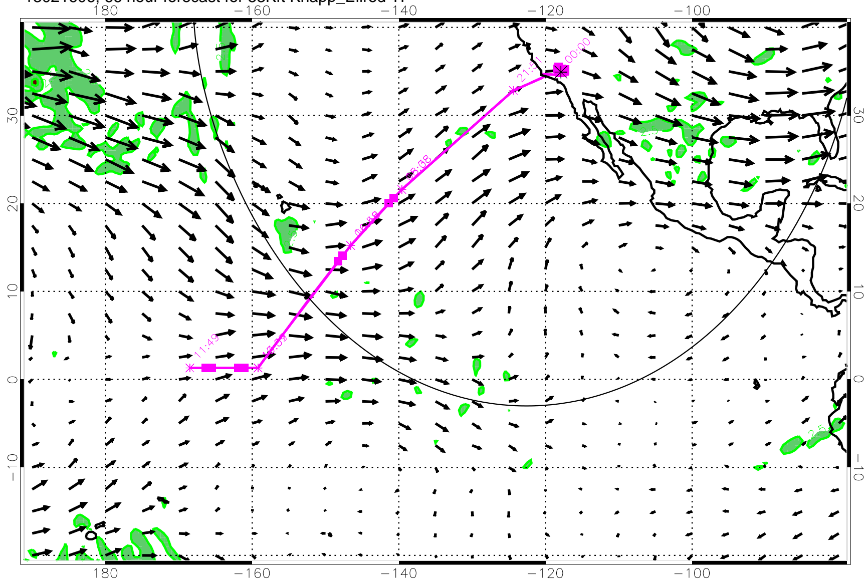
13021606, 66 hour forecast for 53Kft Knapp_Ellrod TI
